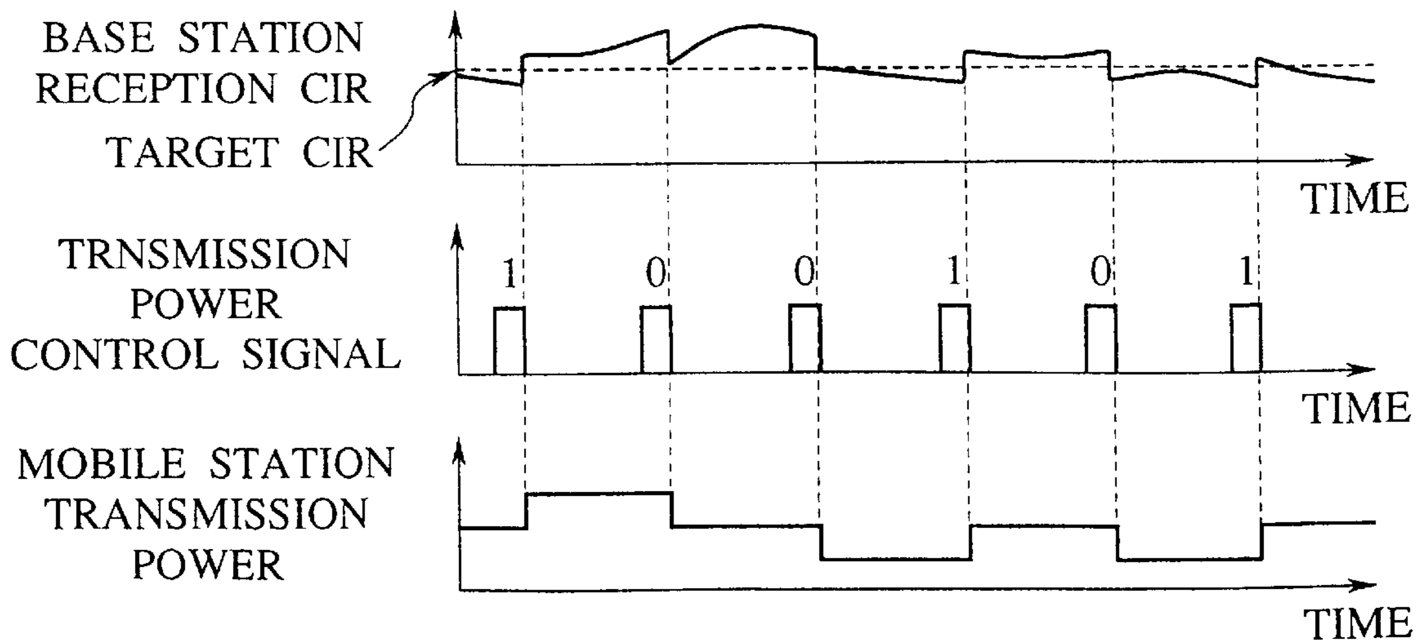
FIG.2 PRIOR ART
