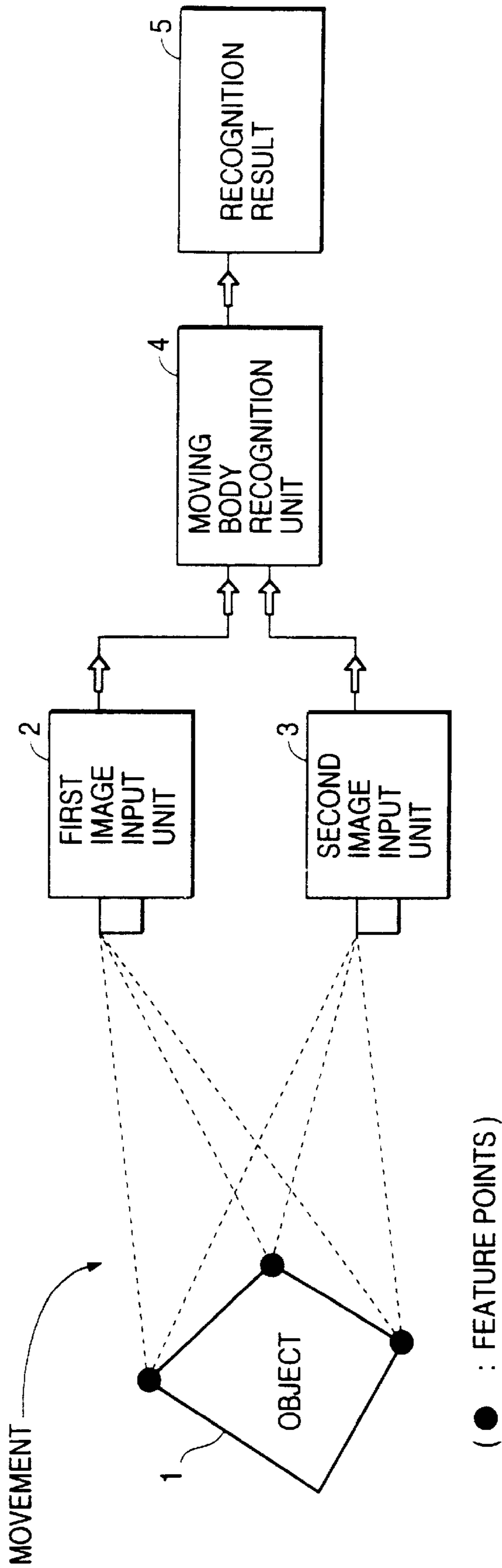
FIG. 1 (PRIOR ART)
