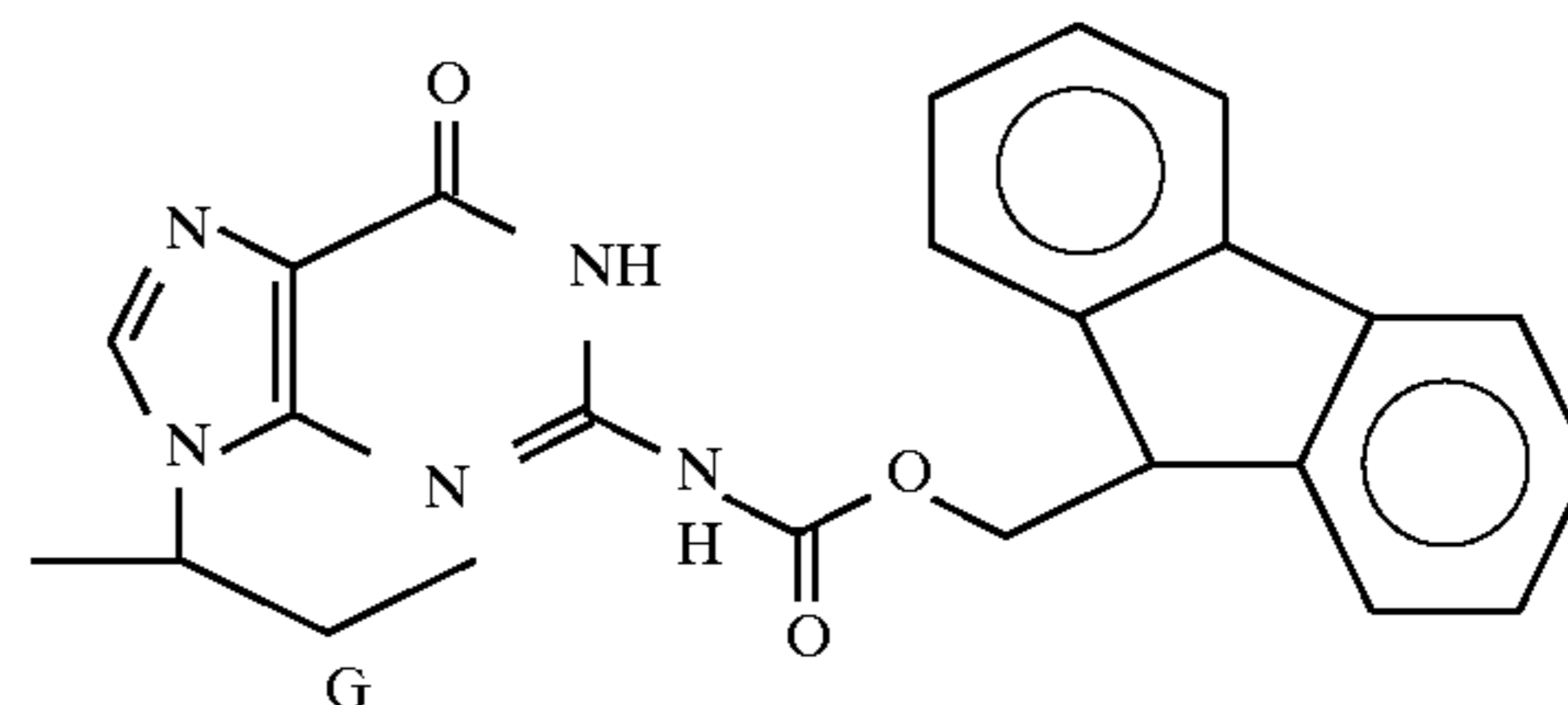
Guanine (G)
