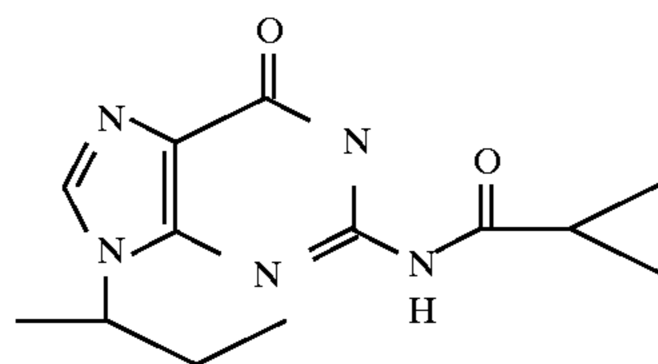
Guanine (G)
