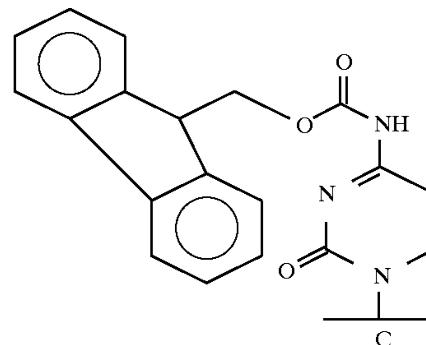
Cytosine (C)
