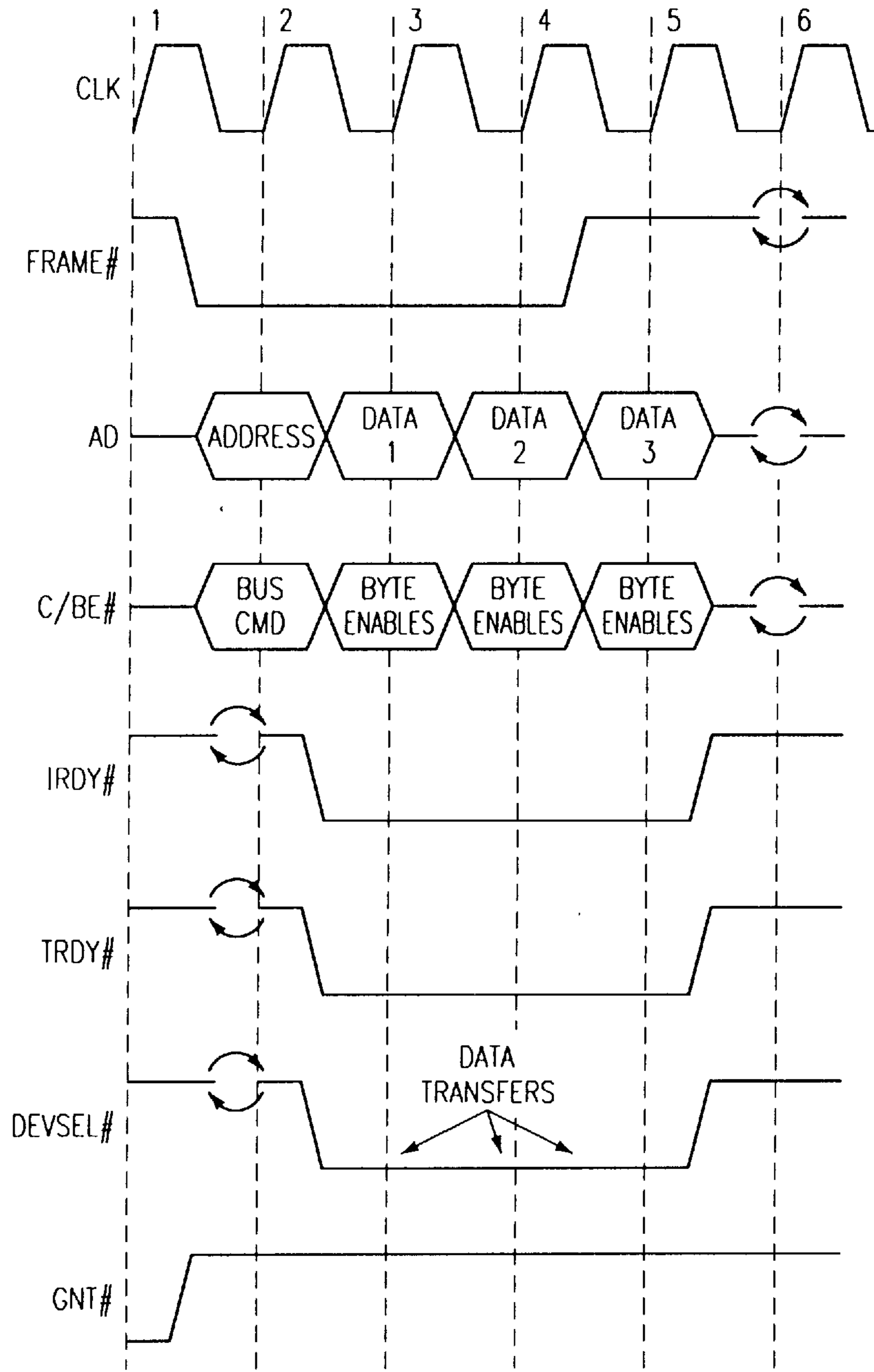
PCI BUS WRITE
