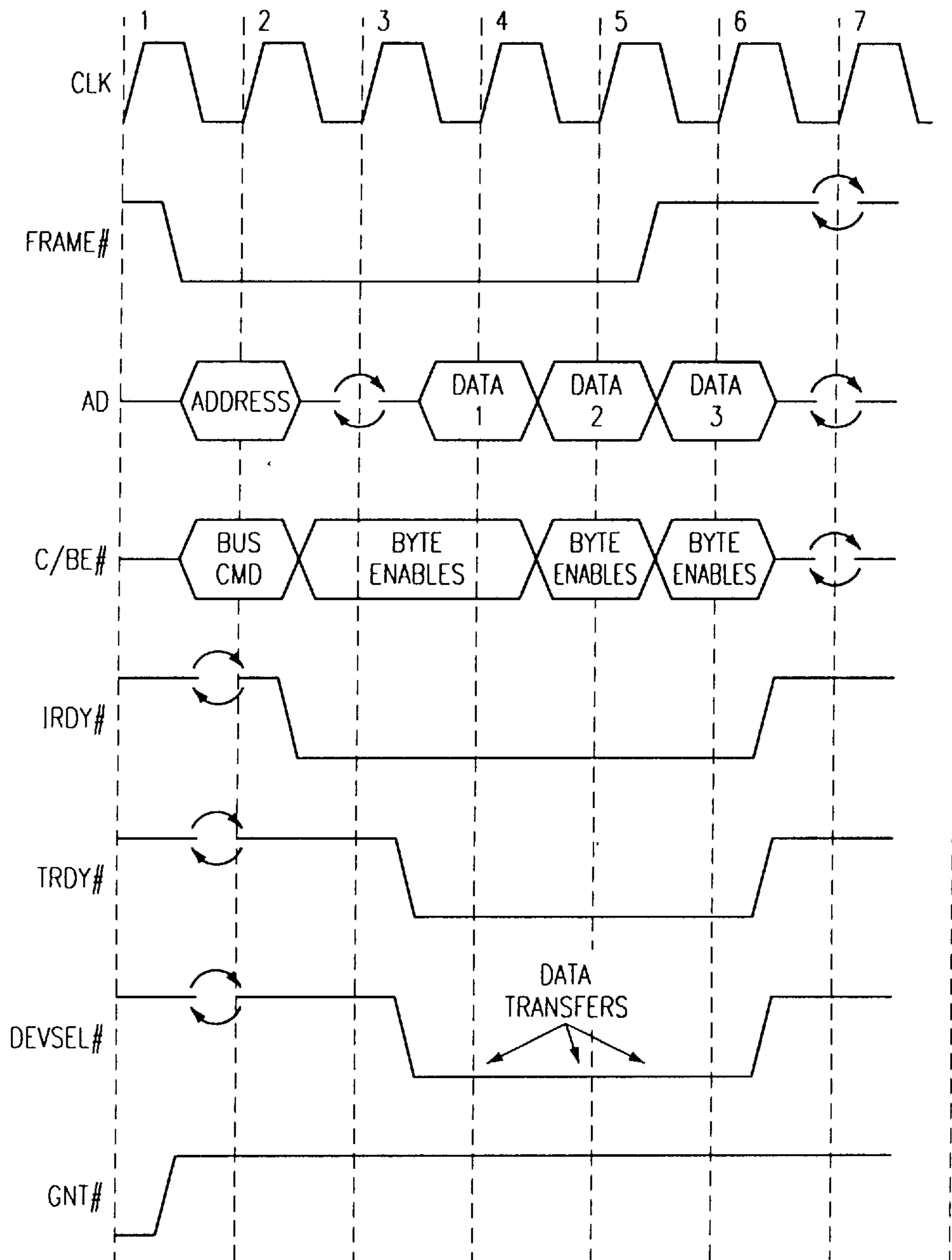
PCI BUS READ
