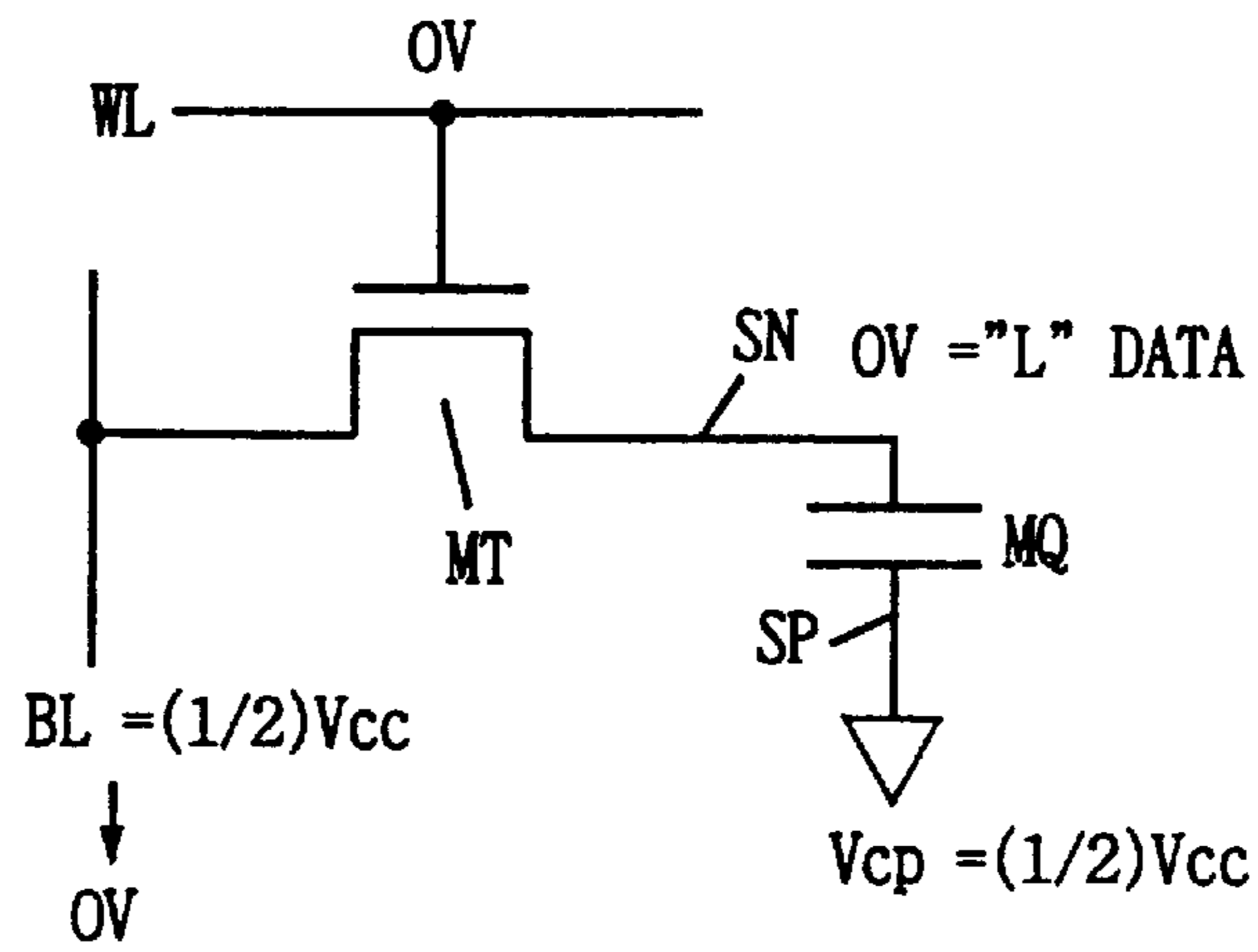
FIG. 70 PRIOR ART
