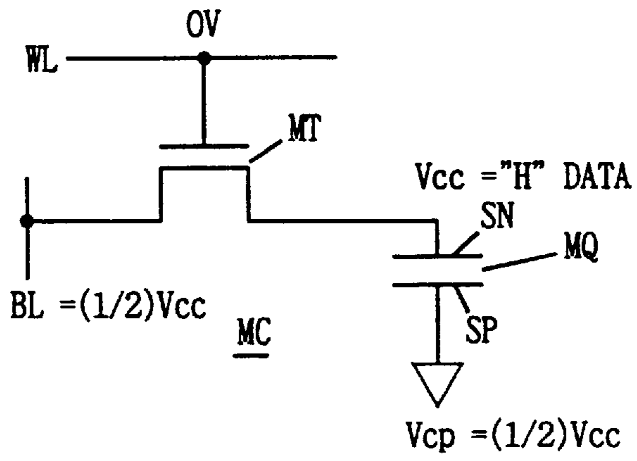
FIG. 68 PRIOR ART
