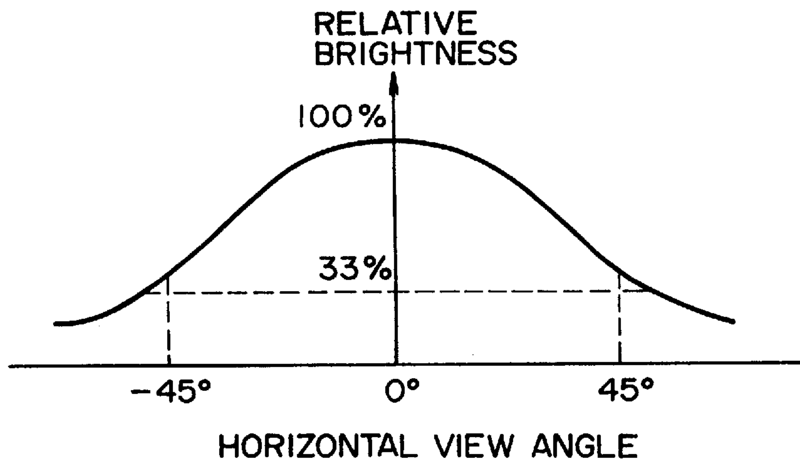
FIG. 8 PRIOR ART
