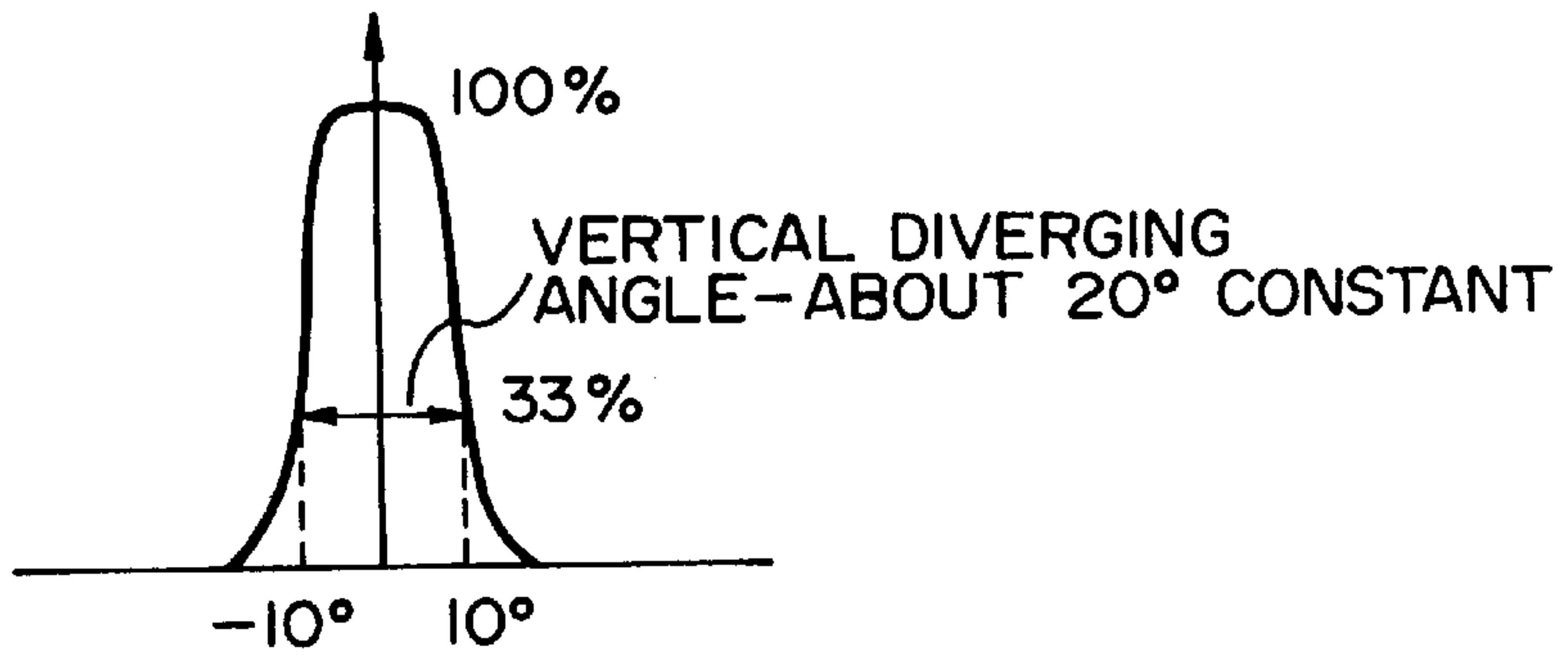
FIG. 9 PRIOR ART
