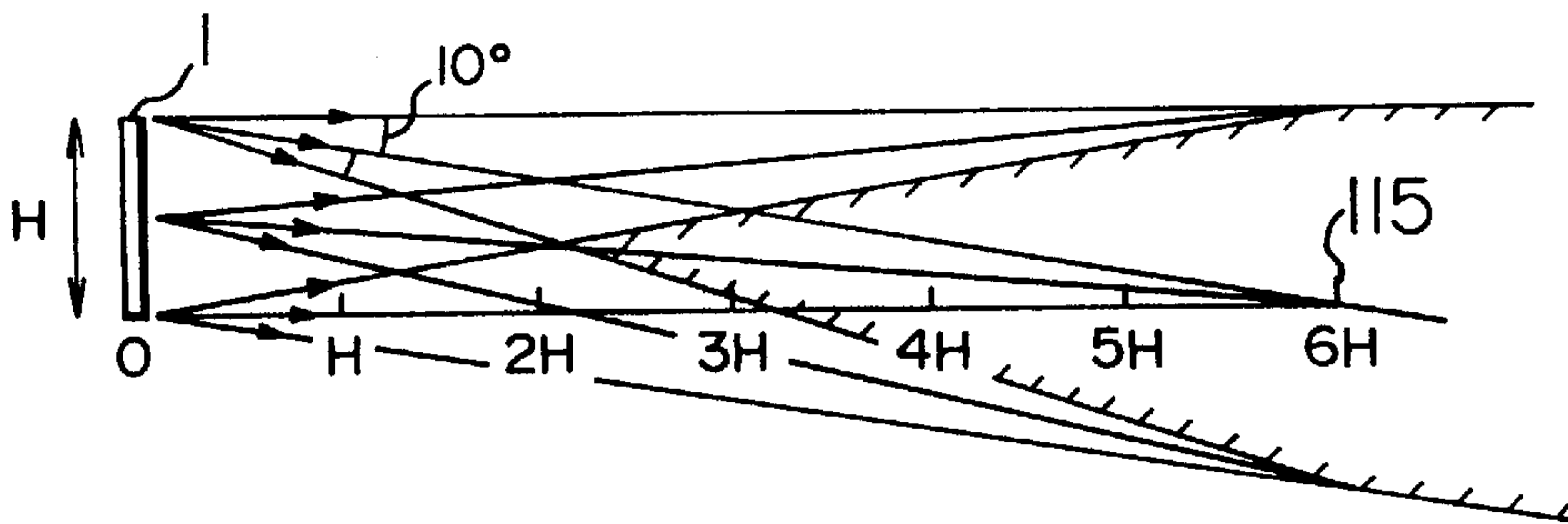
FIG. 10 PRIOR ART
