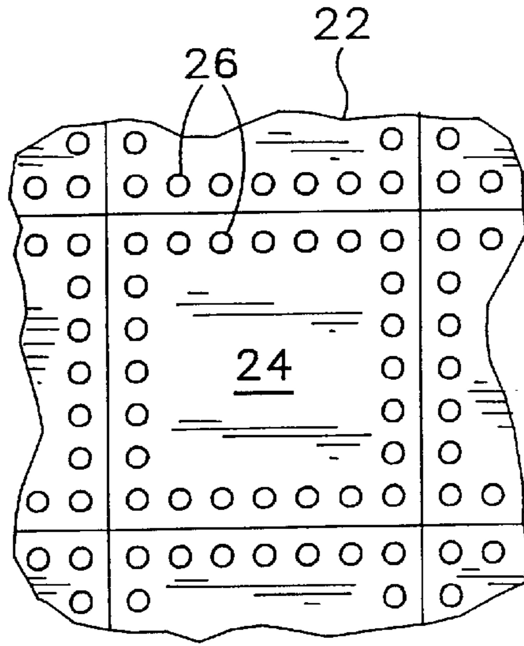
Fig. 2 (PRIOR ART)
