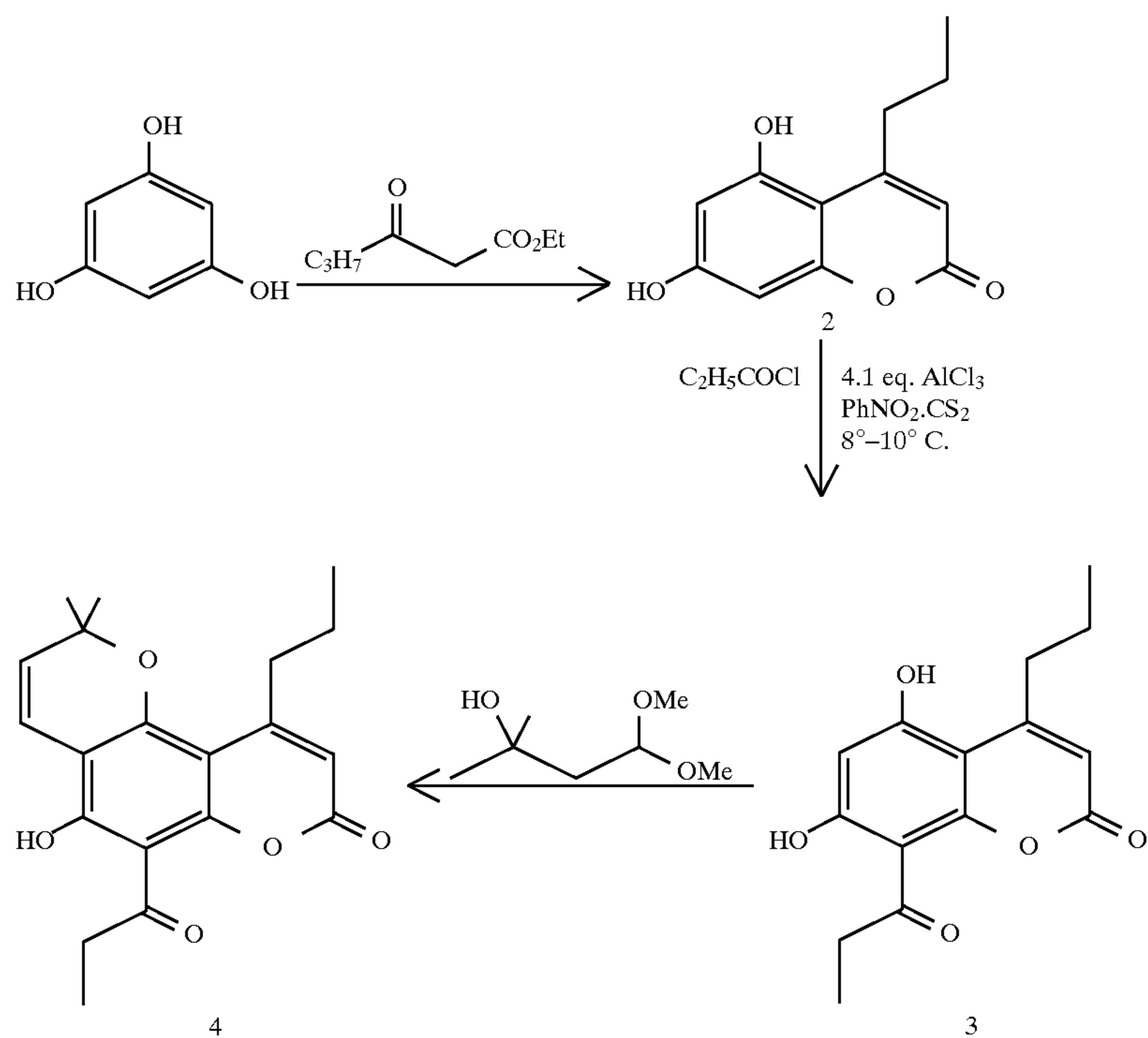
SCHEME I
