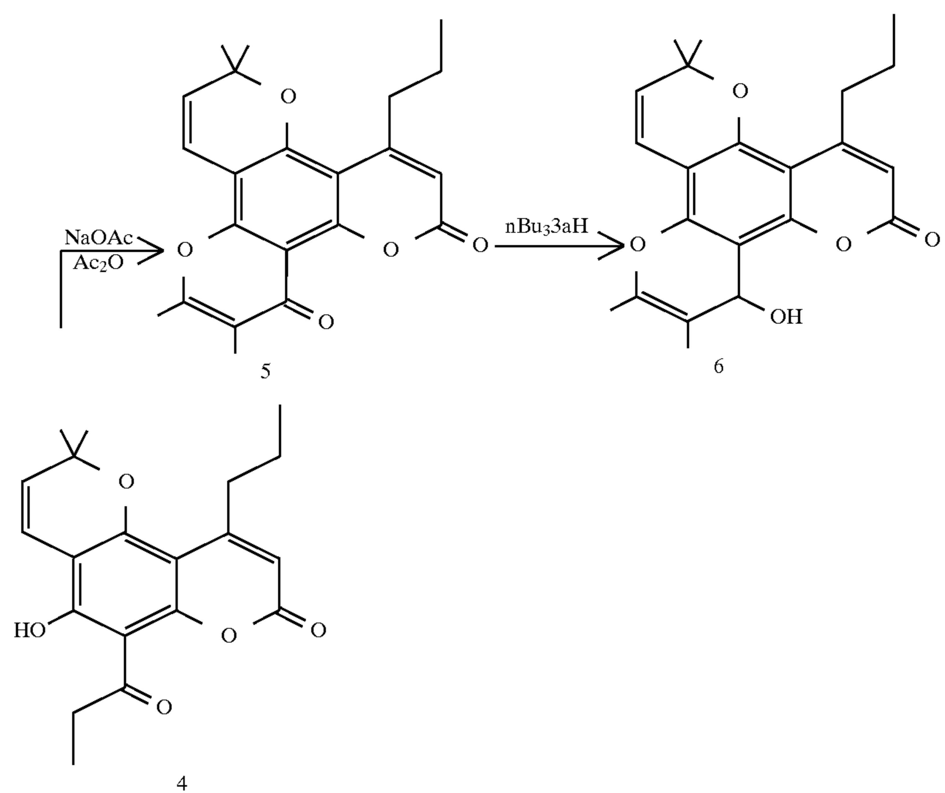
SCHEME II
