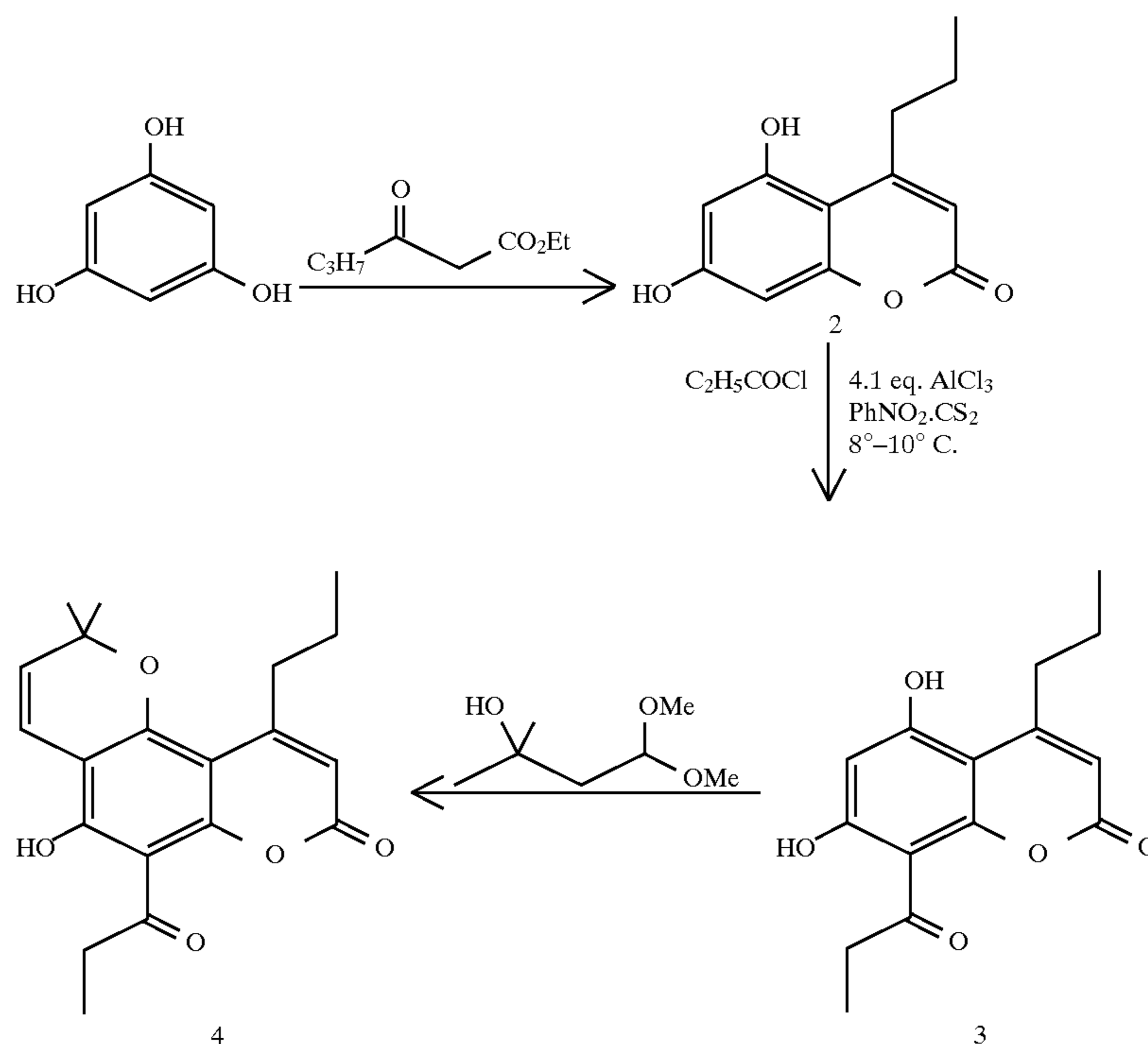
SCHEME I
