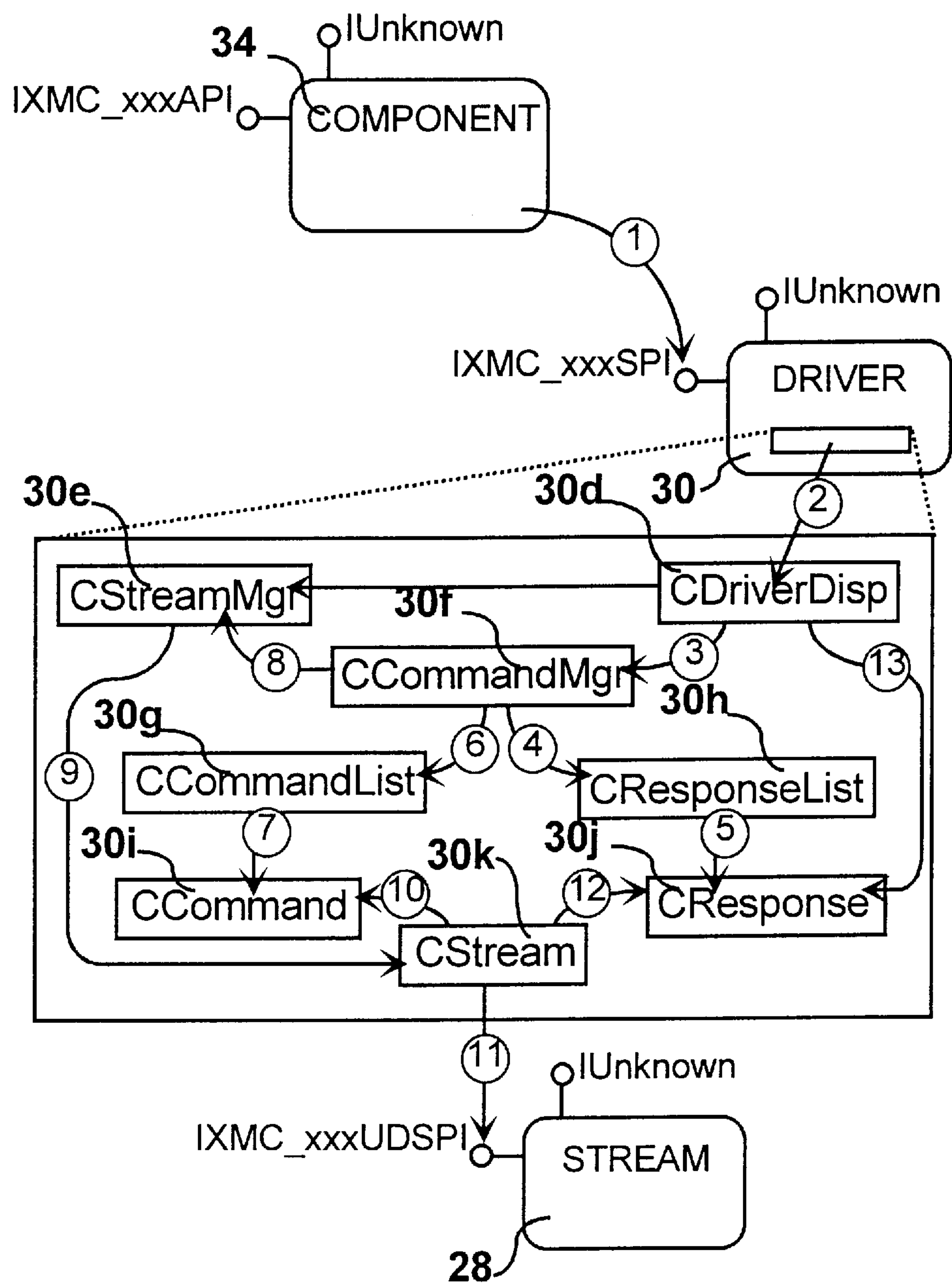
FIG. 19 Scenario-Map - Command Operations
