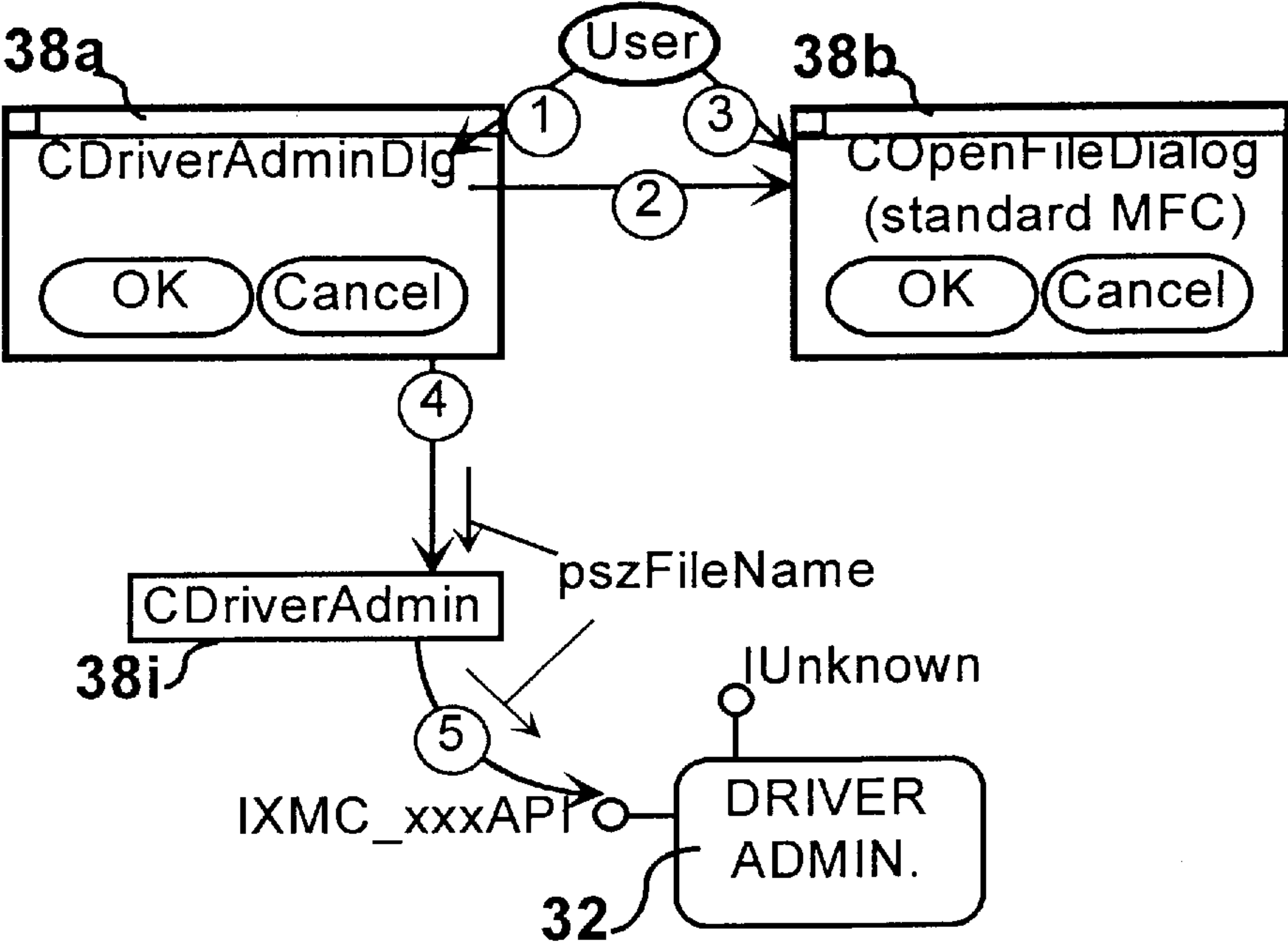
FIG. 55 Scenario-Map - Adding a Driver
