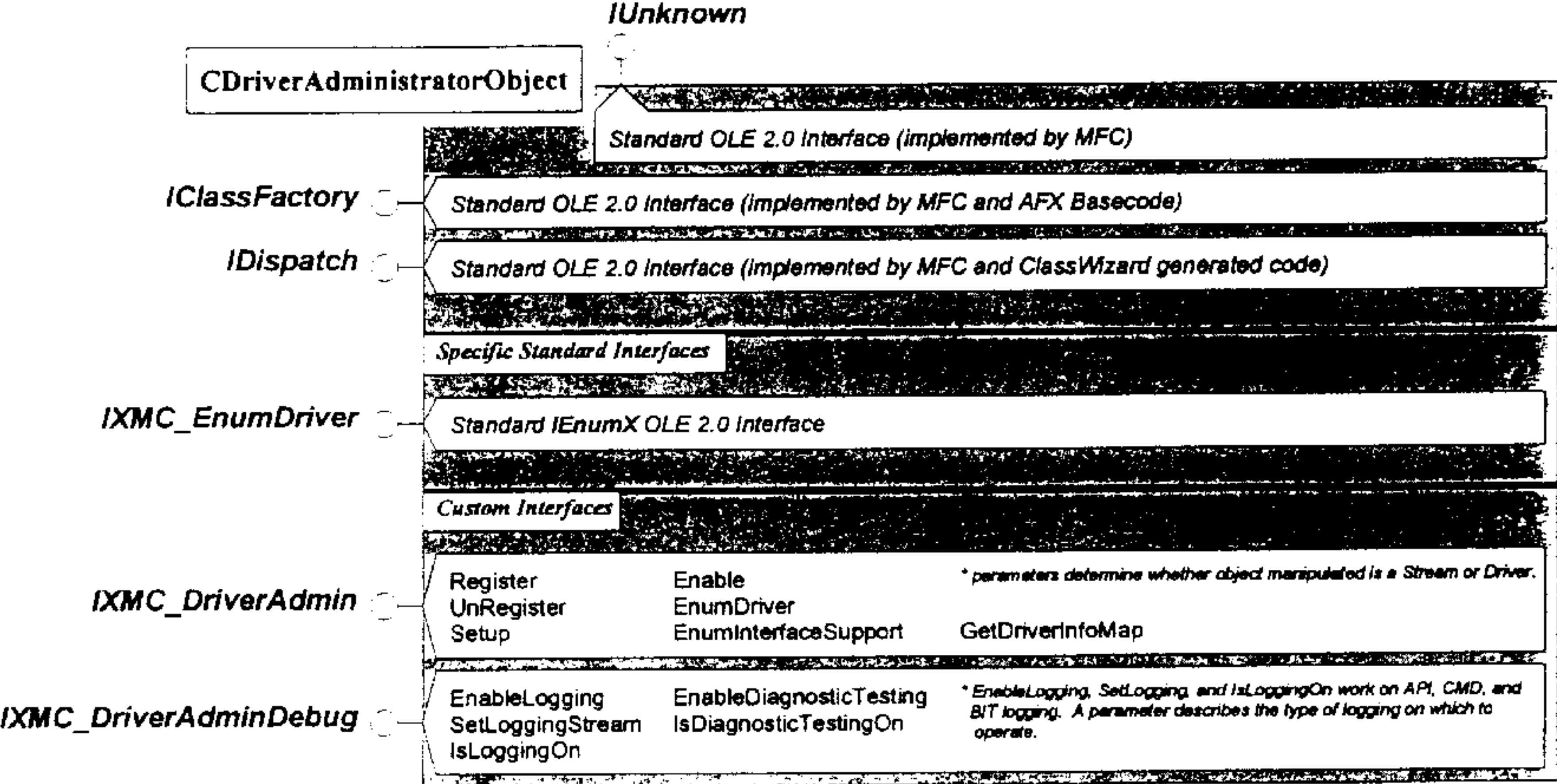
Figure 11 Interface-Map. For more information on the standard OLE interfaces see the OLE 2 Programmer's Reference . And, for more information on the custom XMC API interfaces, see the XMC API Reference .
