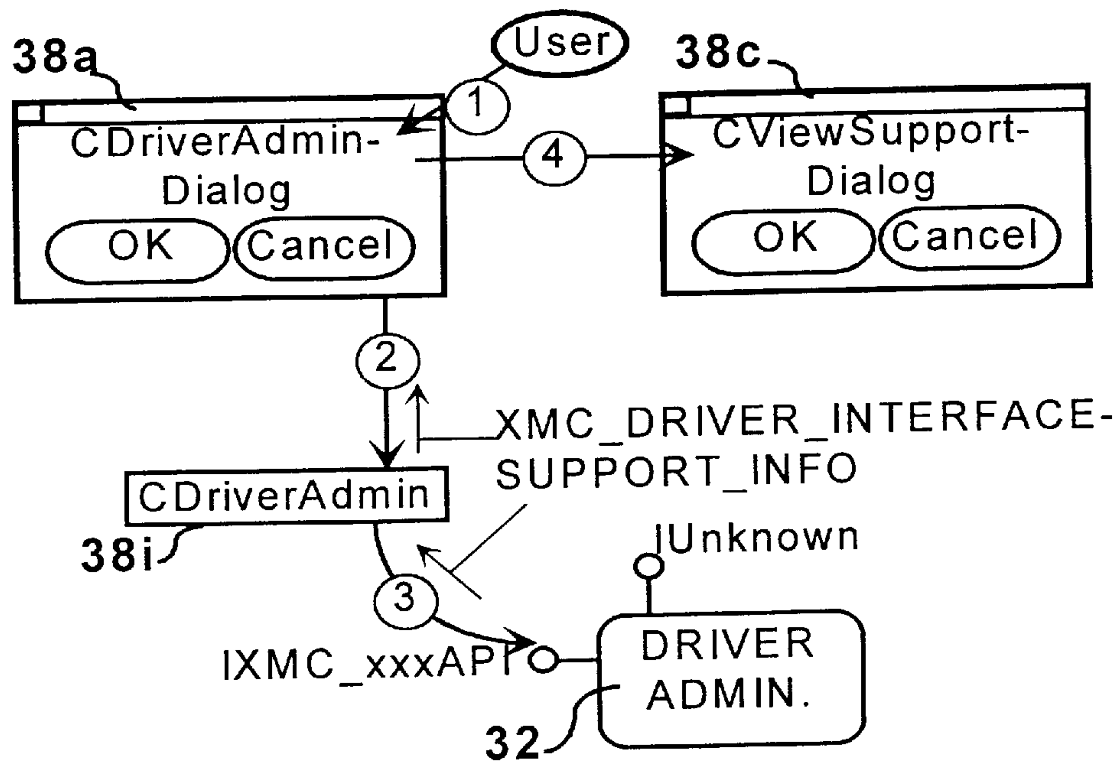
FIG. 57 Scenario-Map - View Support
