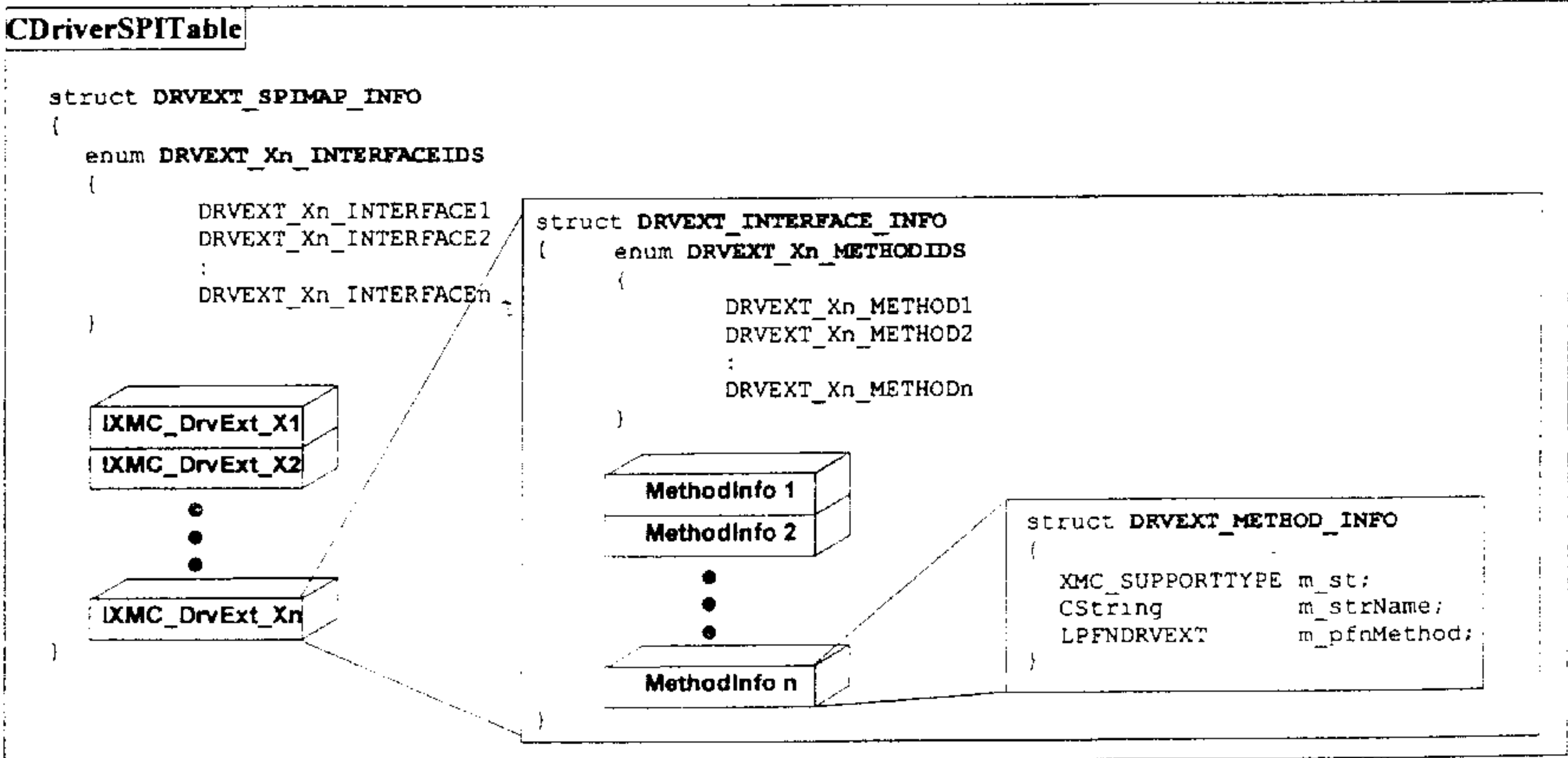
Figure 9 Data-Map - CDriver class with XMCSPi table.
