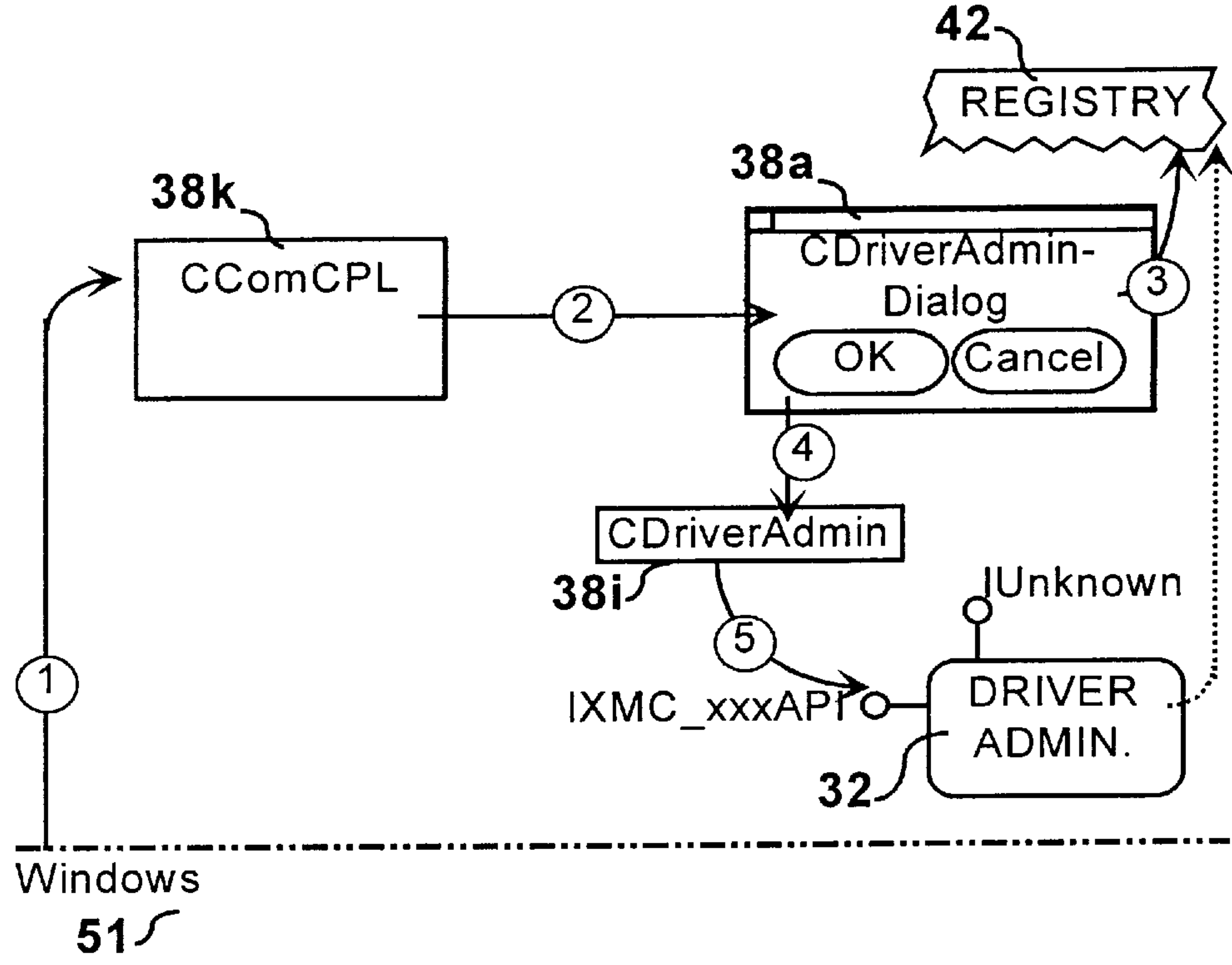
FIG. 53 Scenario-Map - Initializing the App.
