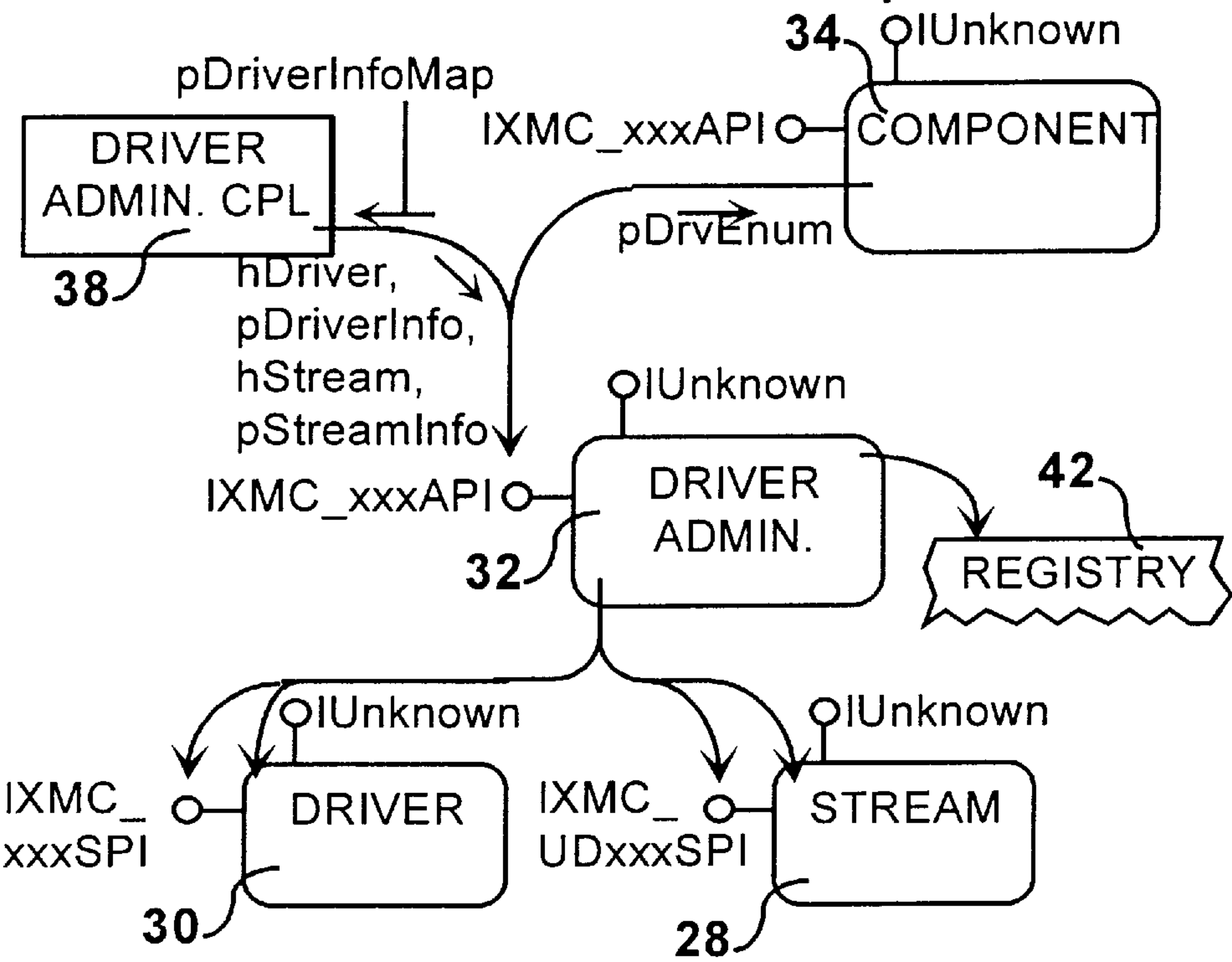
FIG. 40 Module Interaction-Map
