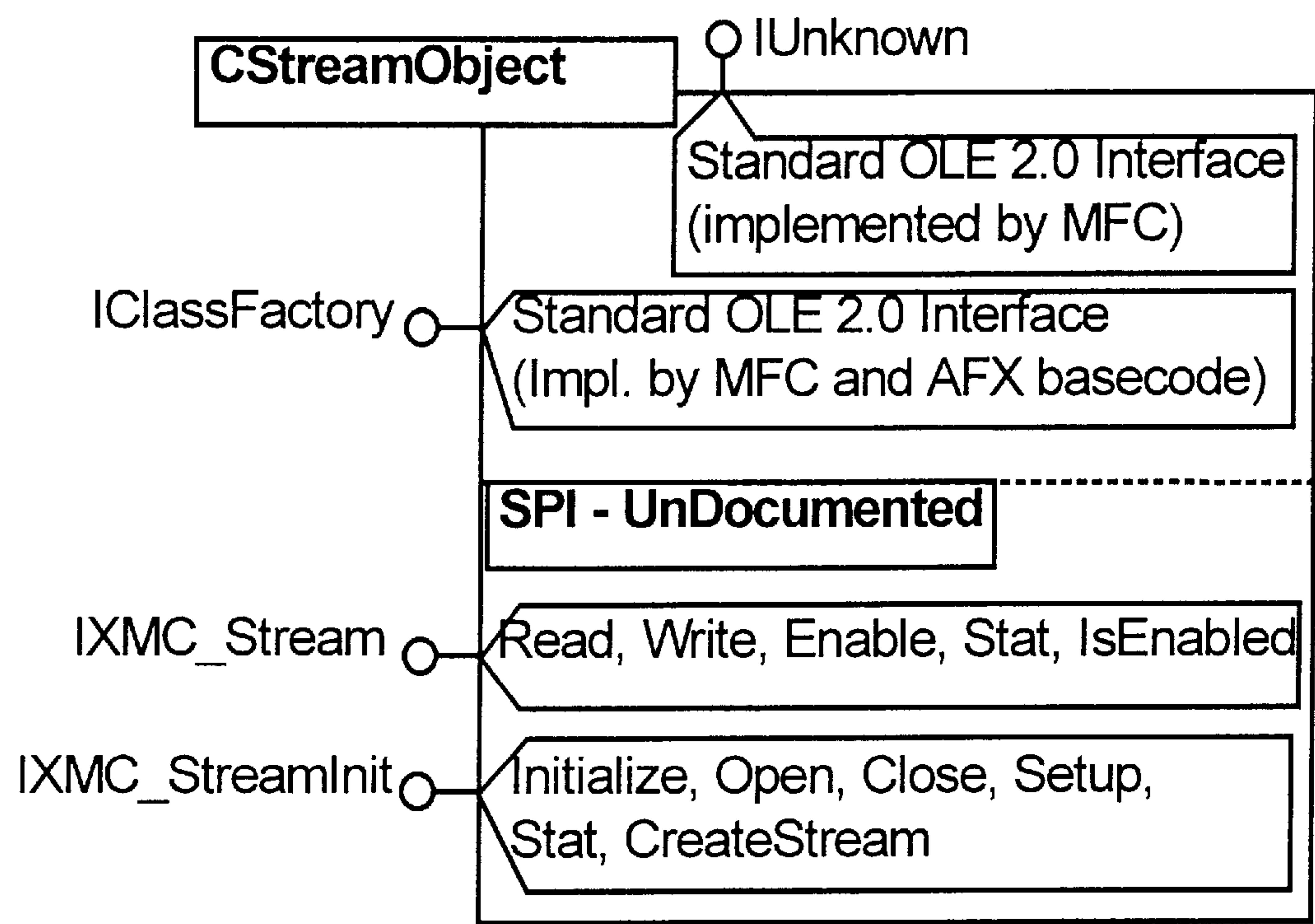
FIG. 33 Interface-Map
