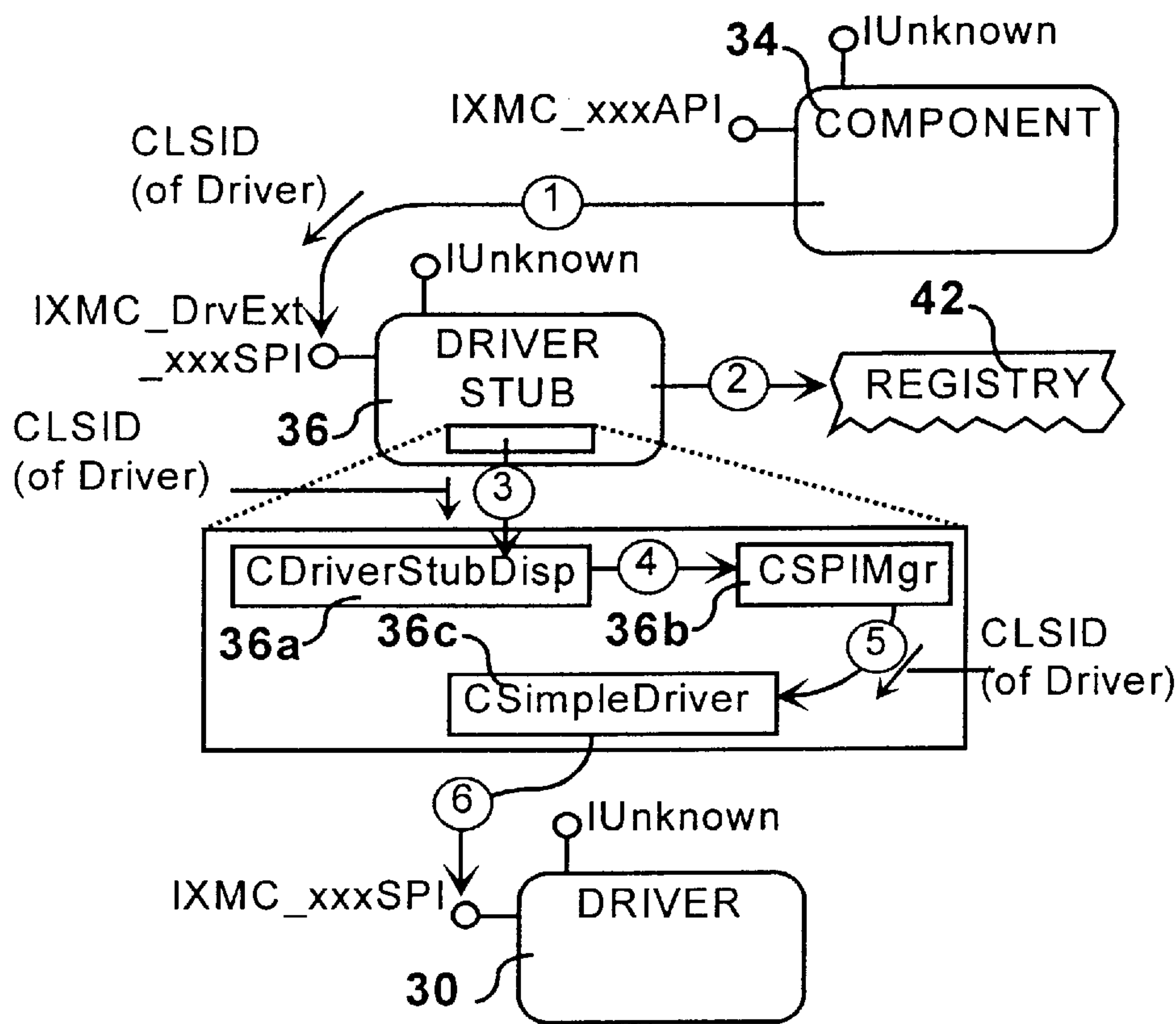
FIG. 36 Scenario-Map - Initialization
