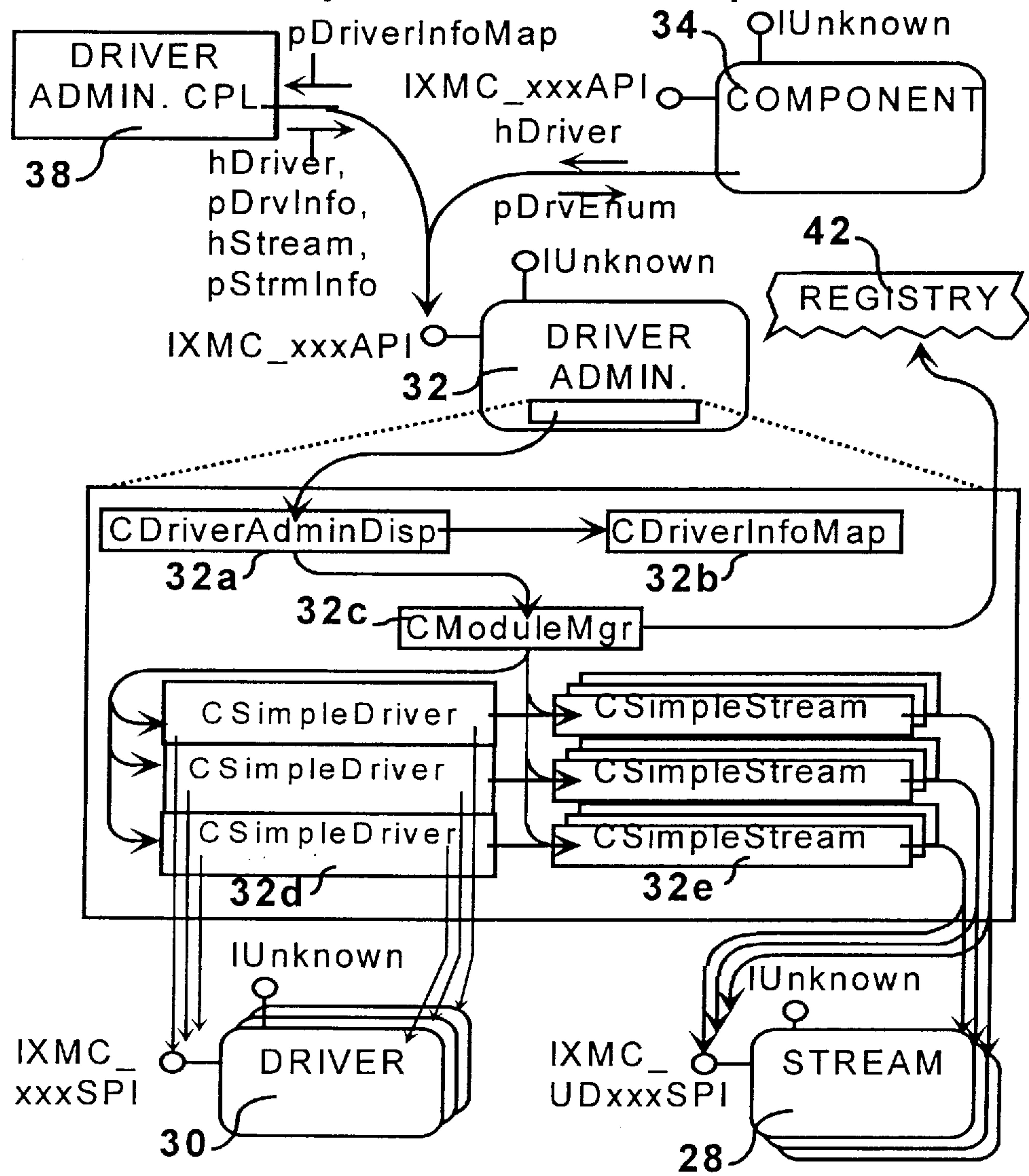
FIG. 41 Object Interaction-Map
