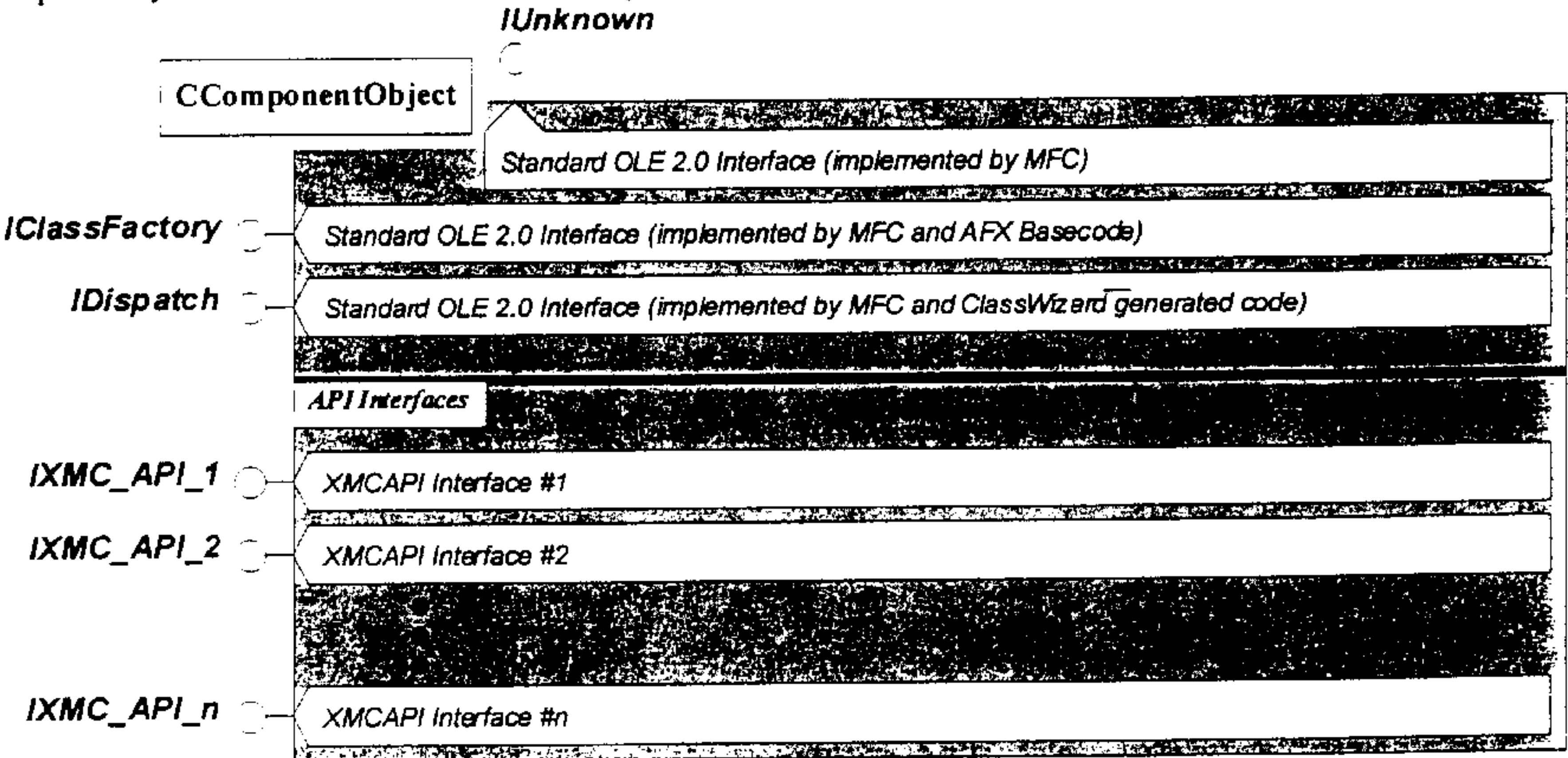
Figure 8 Interface-Map. For more information on the standard OLE interfaces see the OLE 2 Programmer's Reference . And, for more information on the custom XMC API interfaces, see the XMC API Reference .
