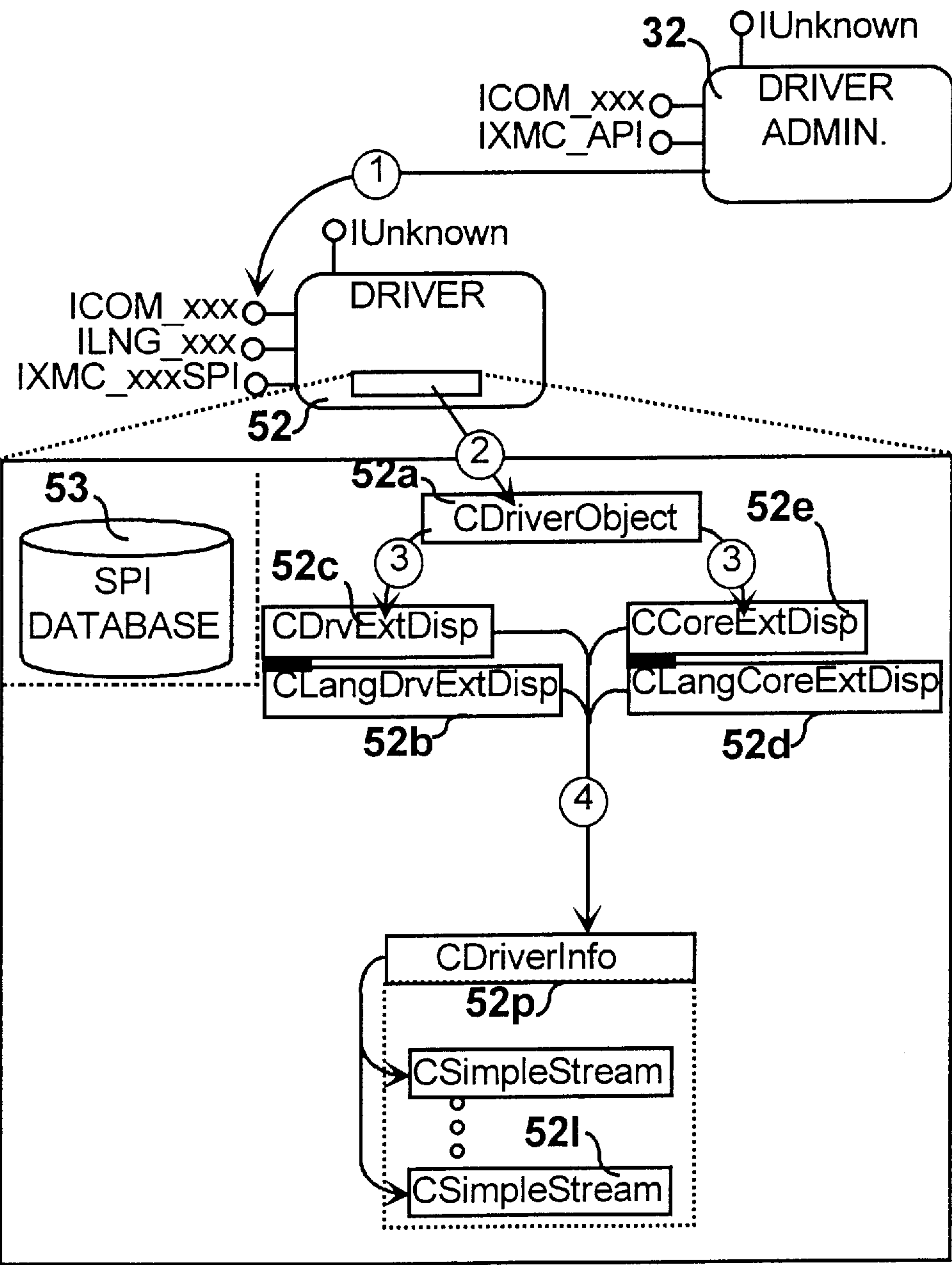
FIG. 62 Scenario-Map - Query Operation
