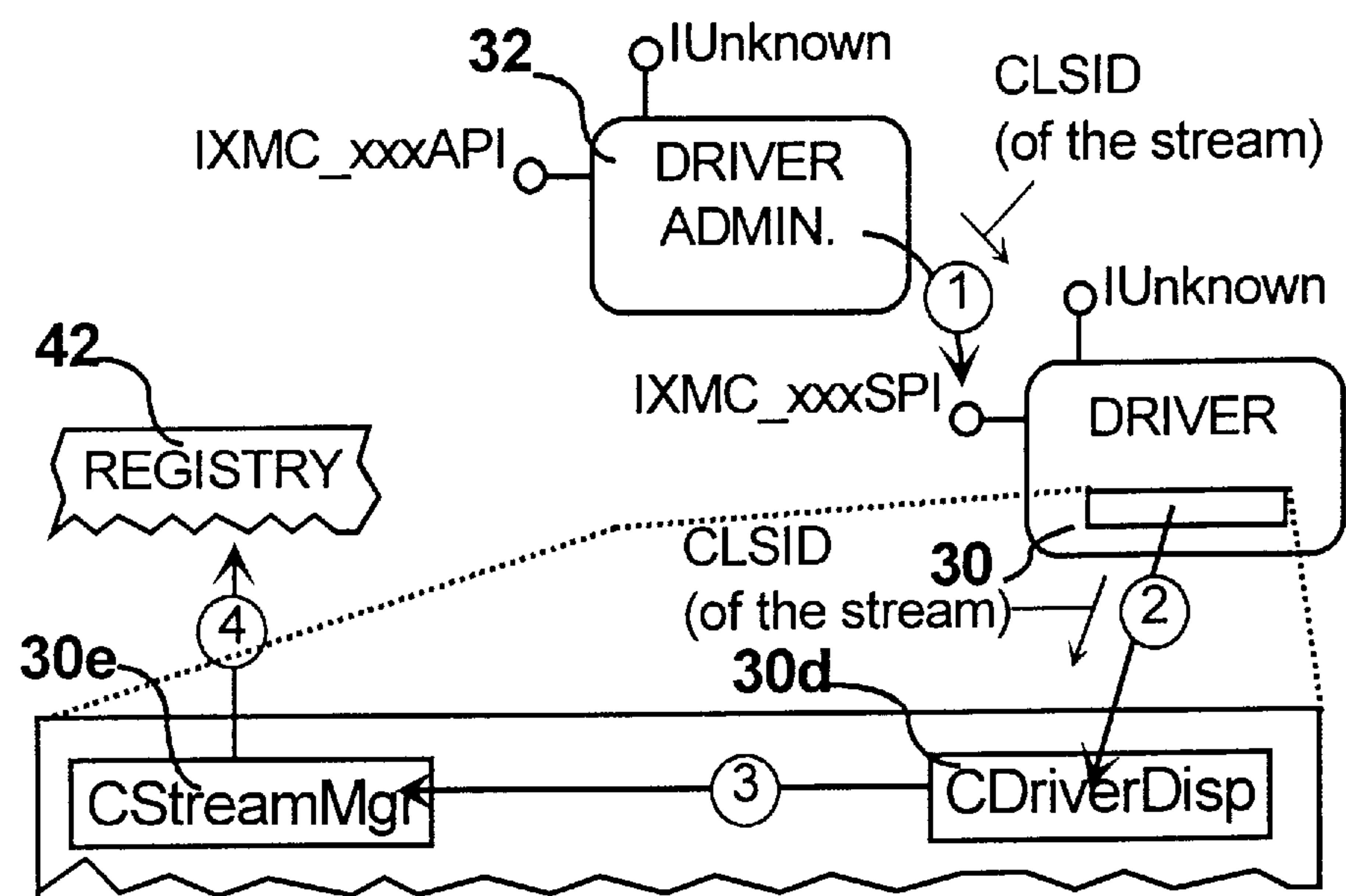
FIG. 15 Scenario-Map - Adding a Stream
