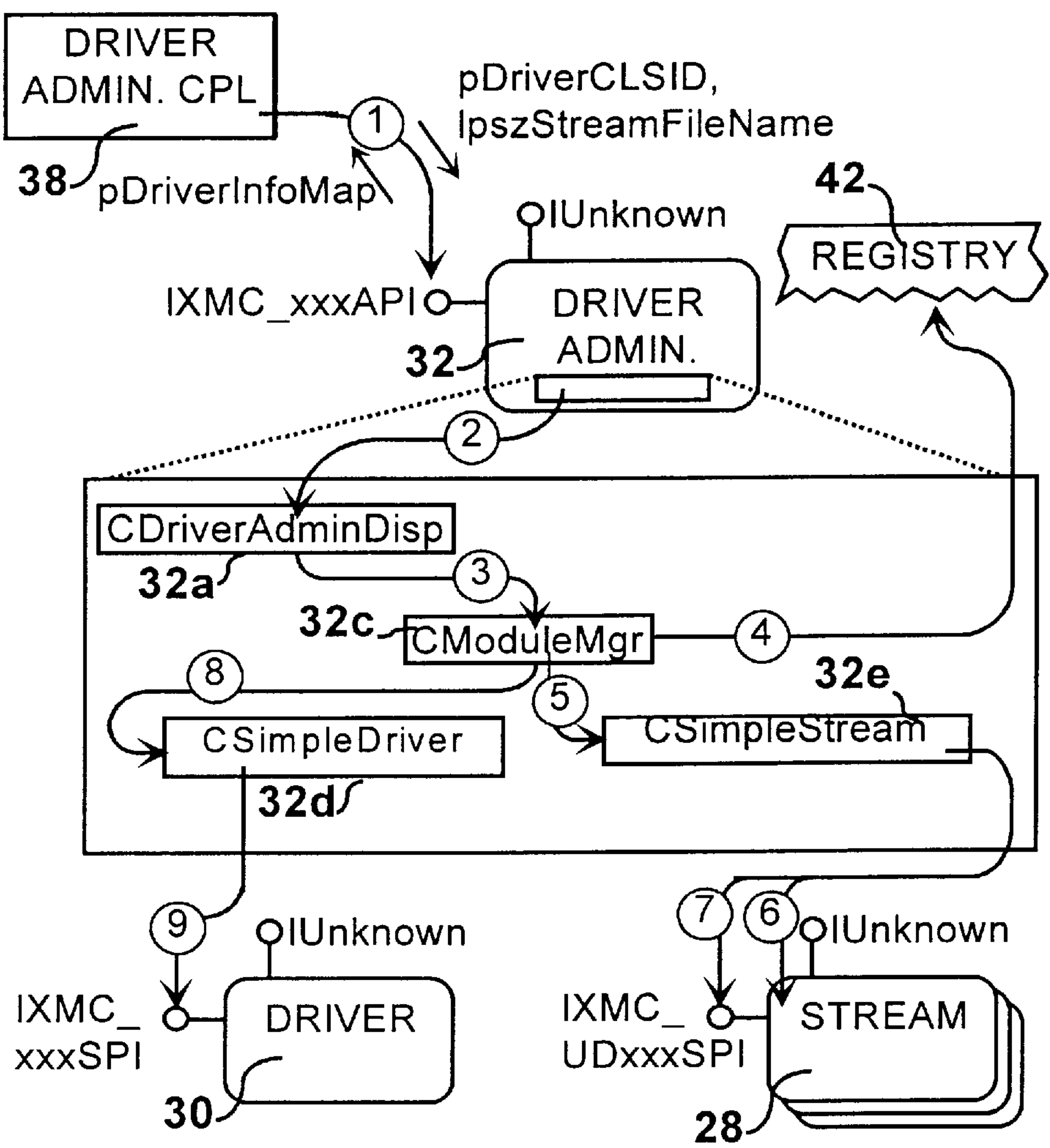
FIG. 44 Scenario-Map - Registering a Stream
