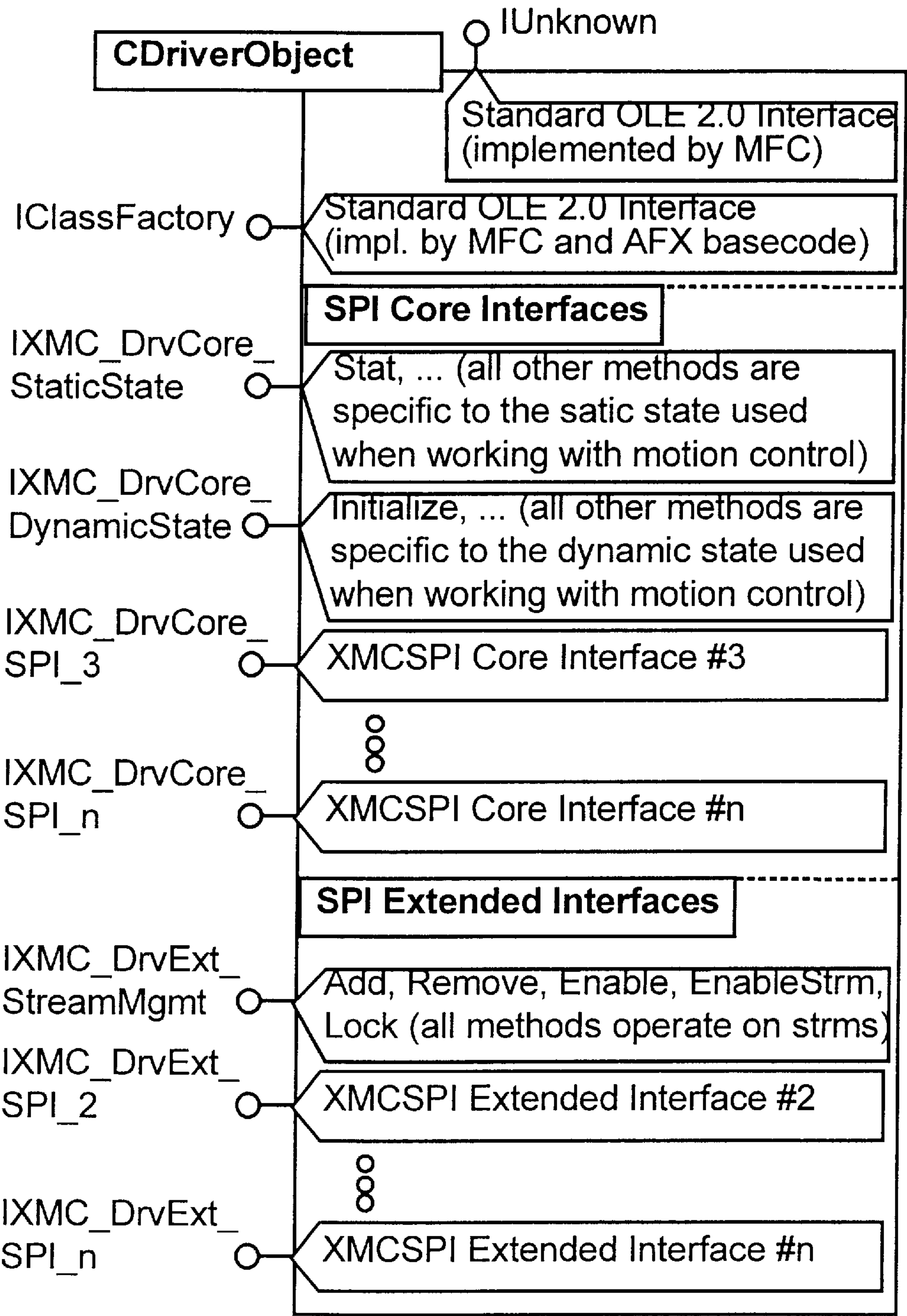
FIG. 21 Interface-Map
