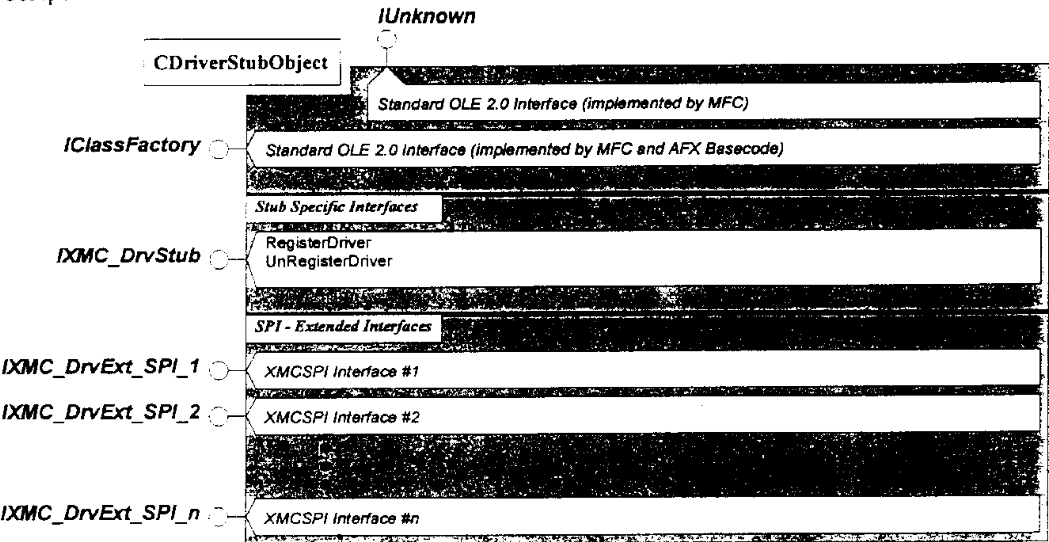
Figure 6 Interface-Map.
