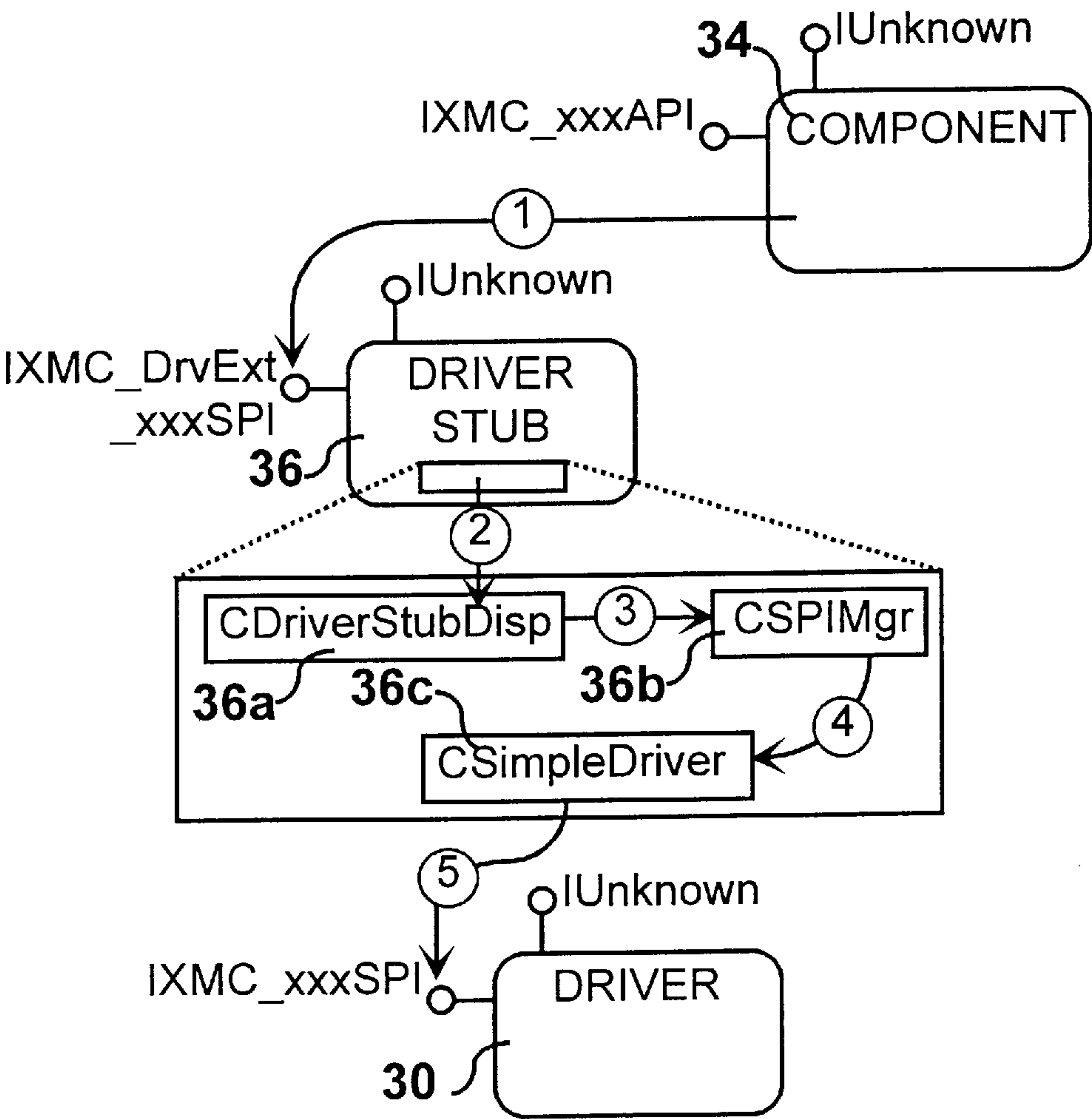
FIG. 38 Scenario-Map - Clean-up
