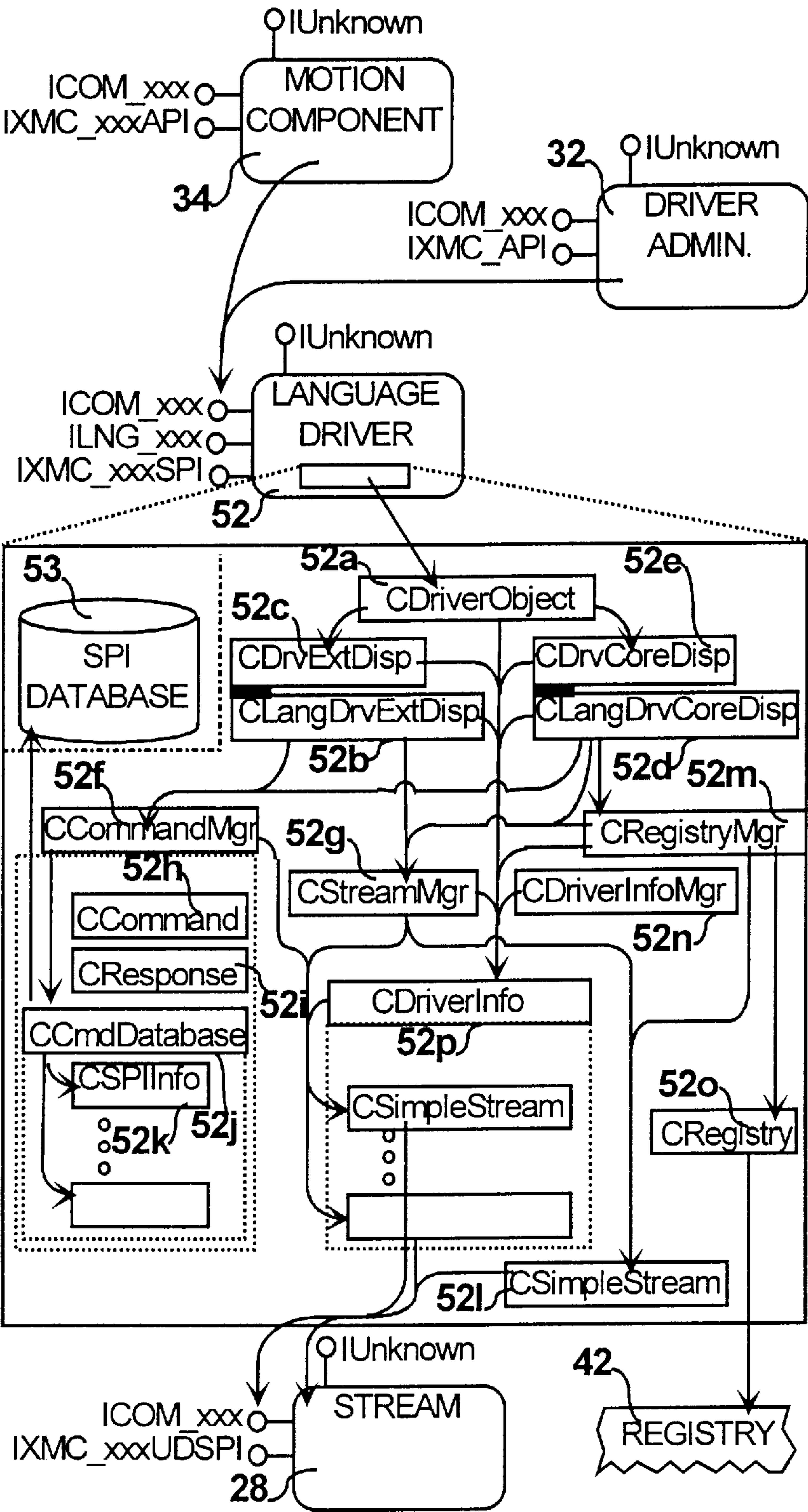
FIG. 59 Object Interaction-Map
