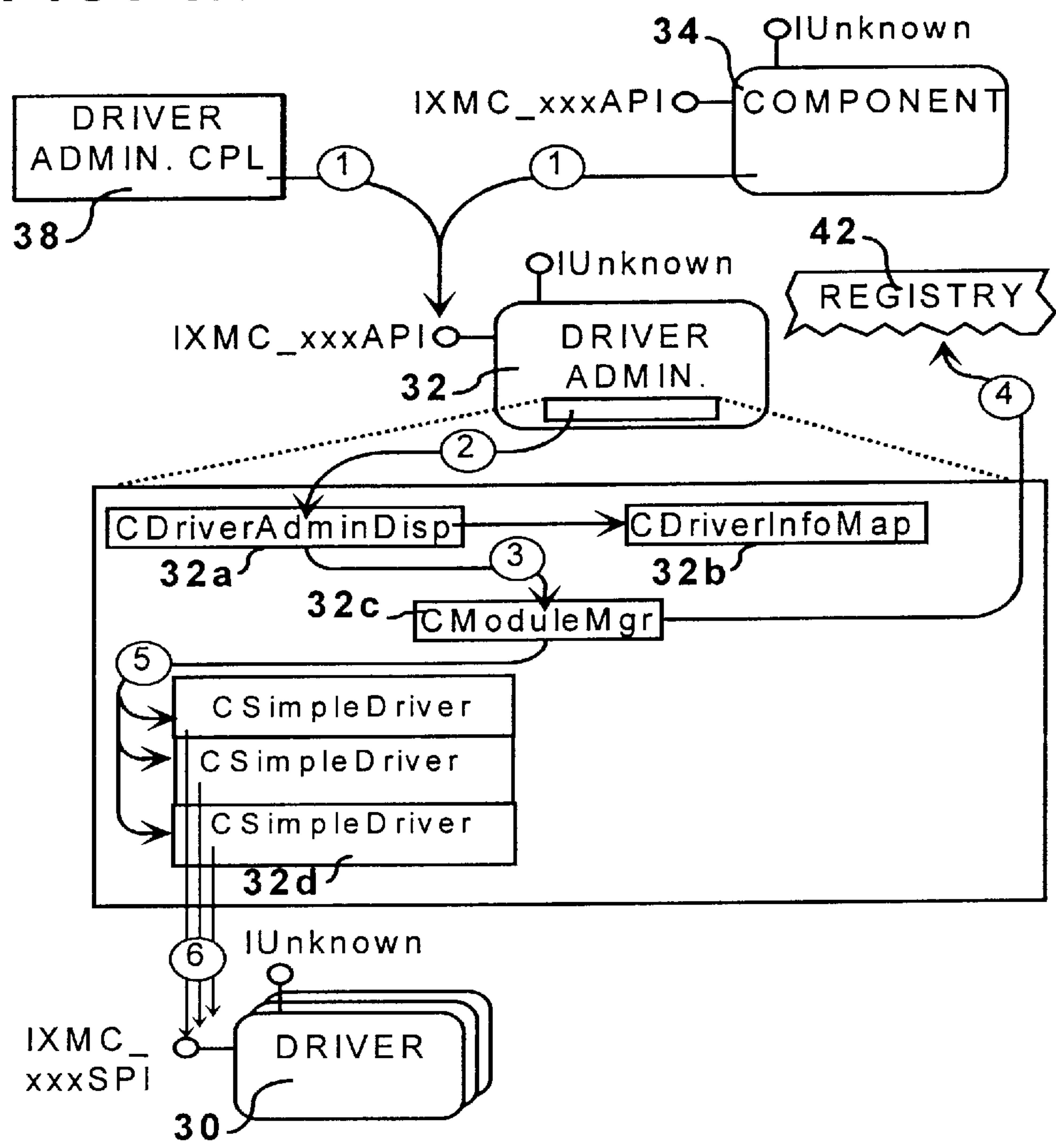
FIG. 42 Scenario-Map - Initialization
