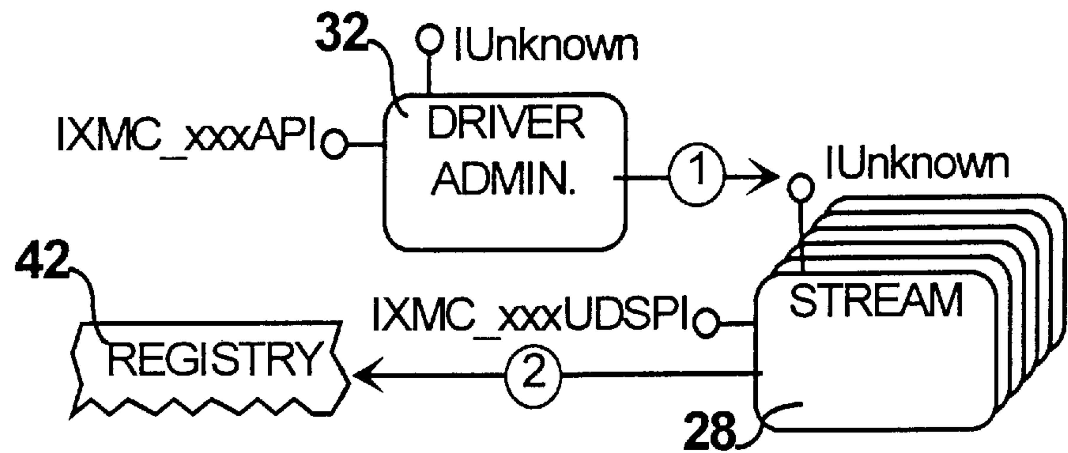
FIG. 25 Scenario-Map - Registration
