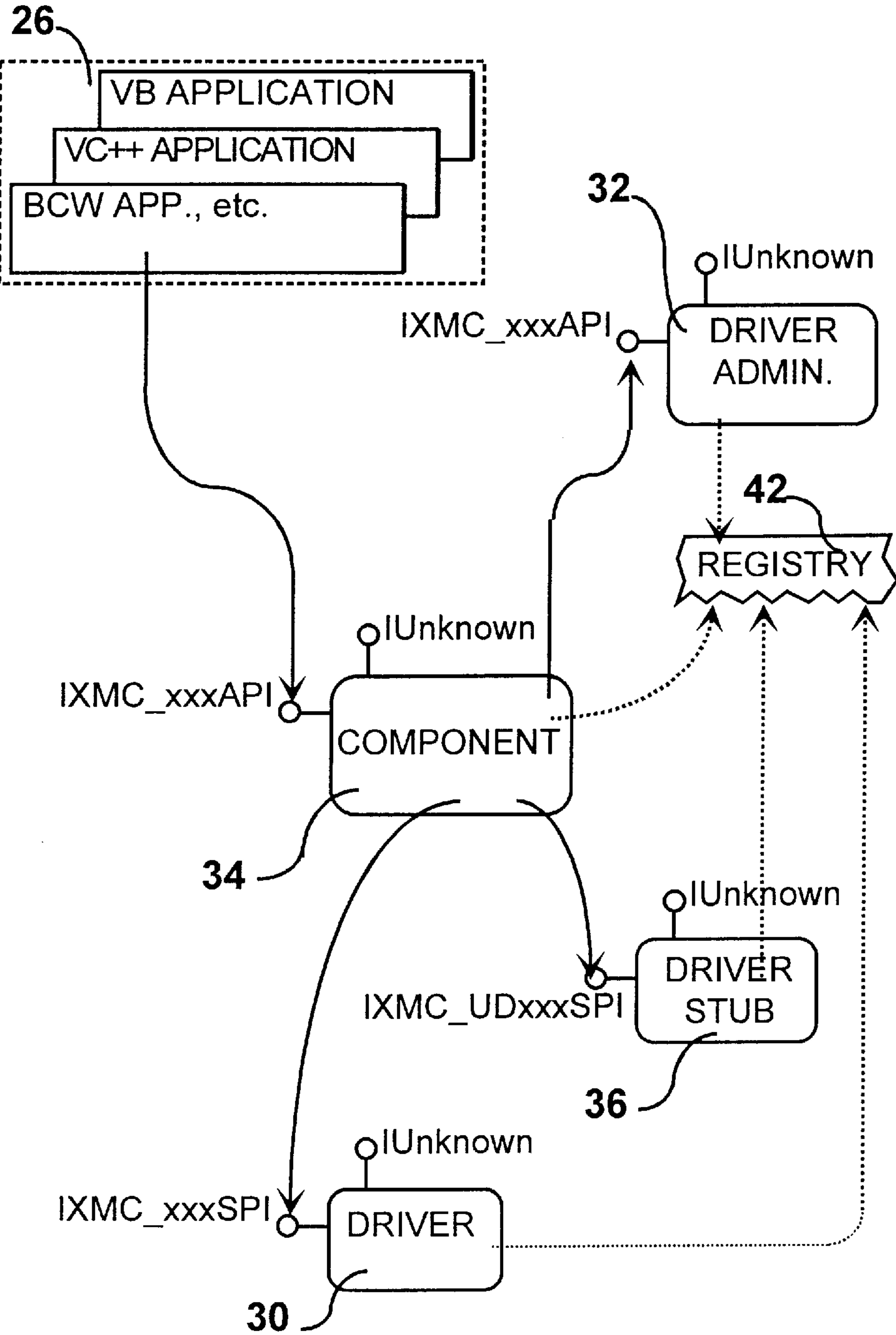
FIG. 2 Module Interaction-Map
