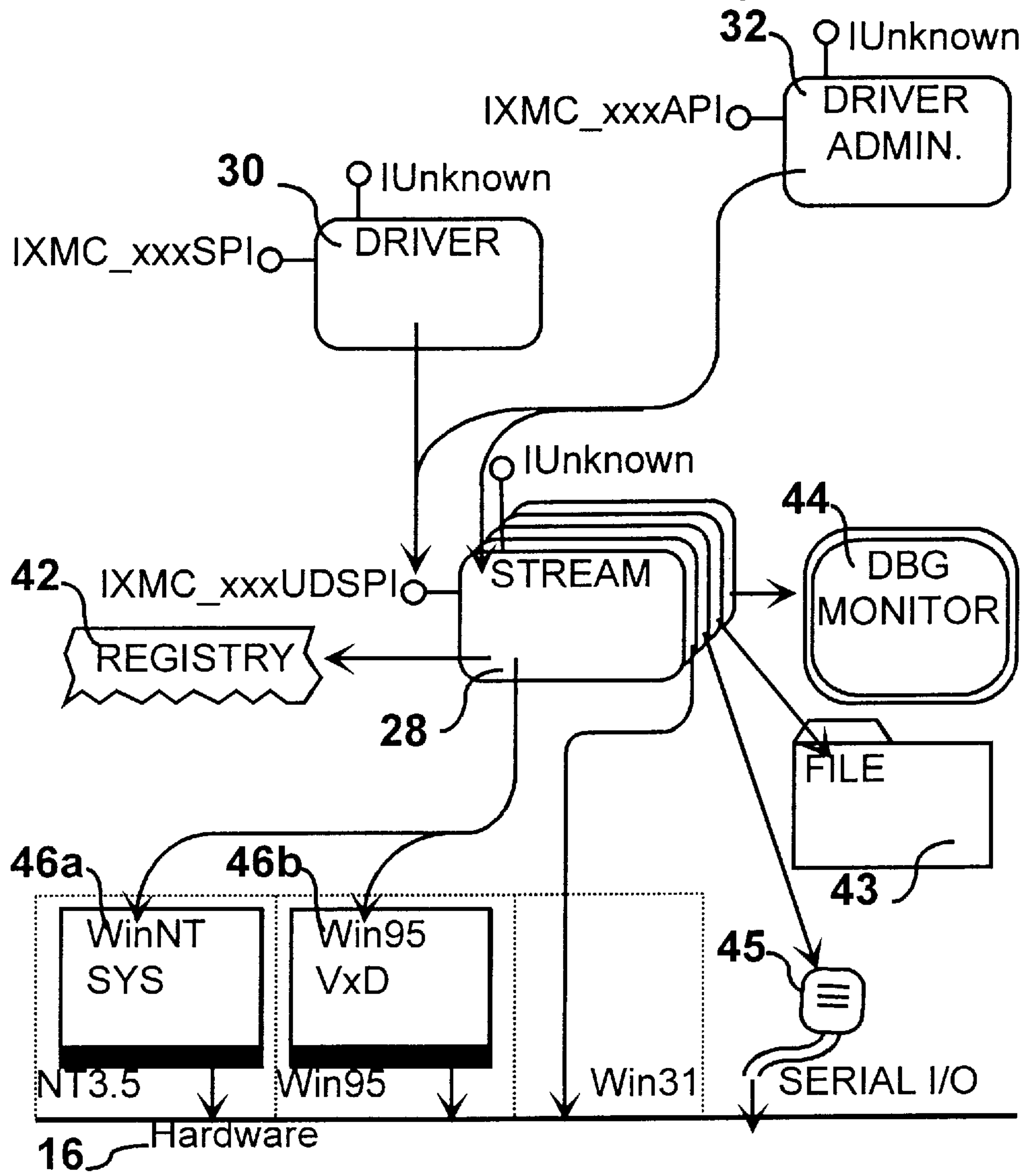
FIG. 22 Module Interaction-Map
