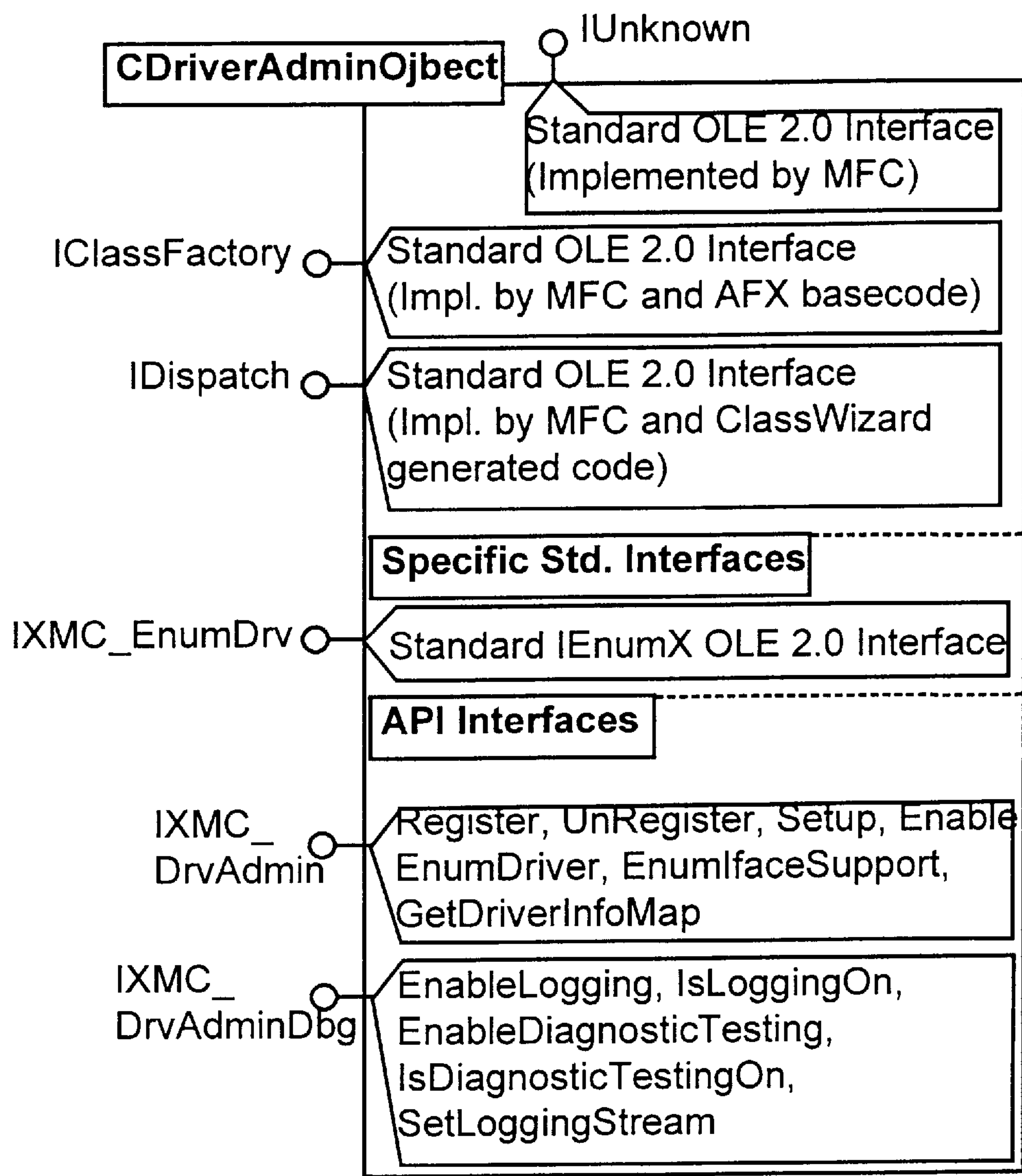
FIG. 50 Interface-Map.
