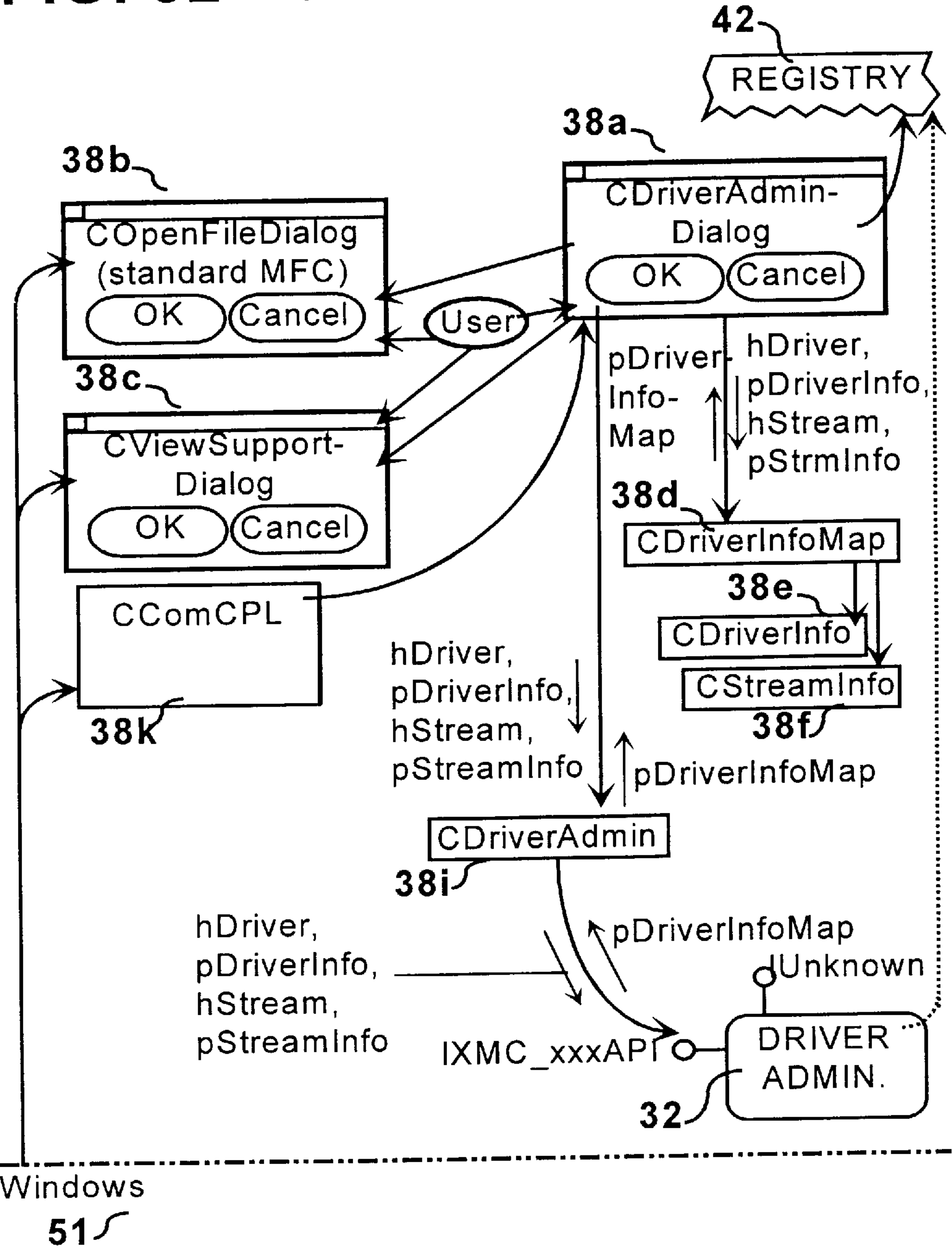
FIG. 52 Object Interaction-Map
