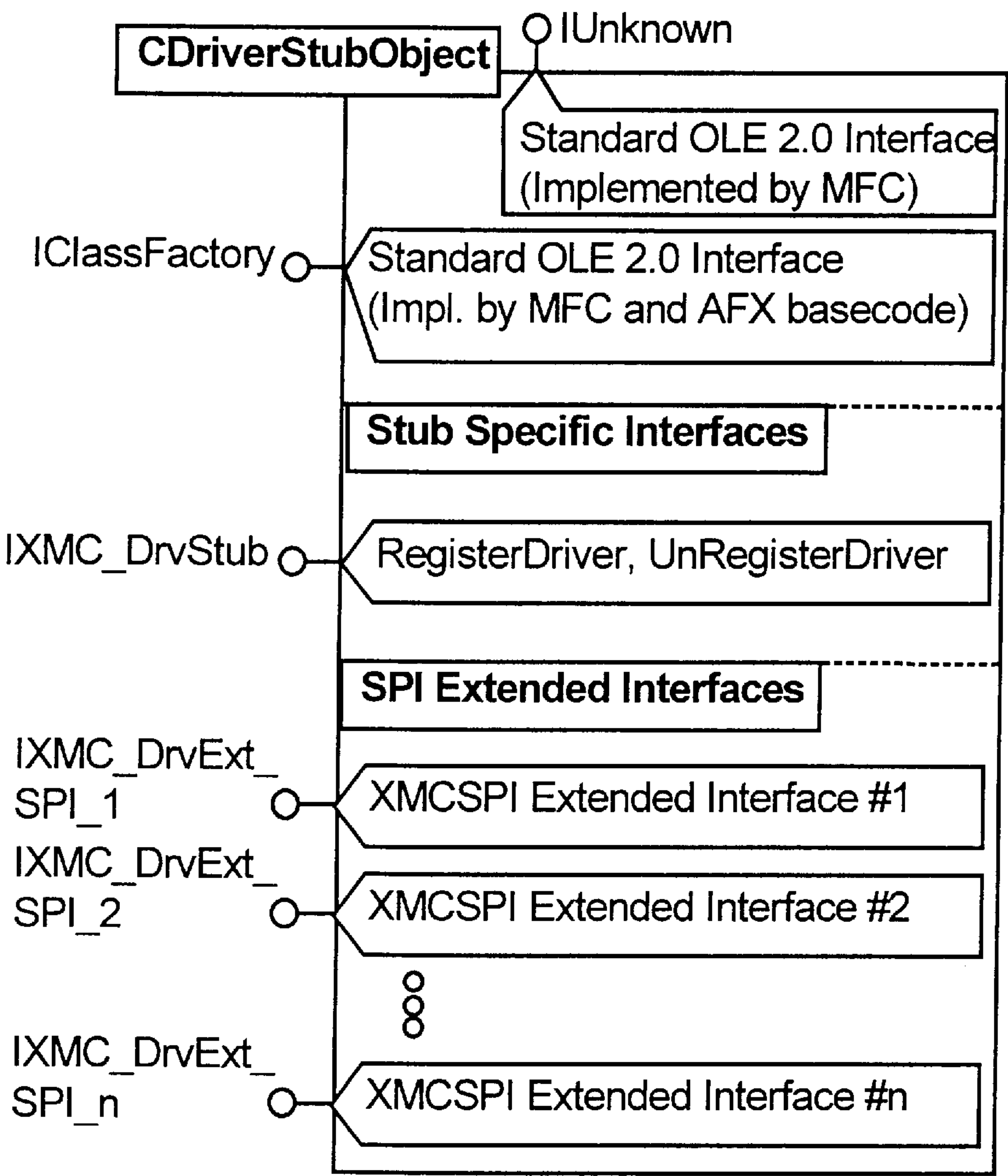
FIG. 39 Interface-Map
