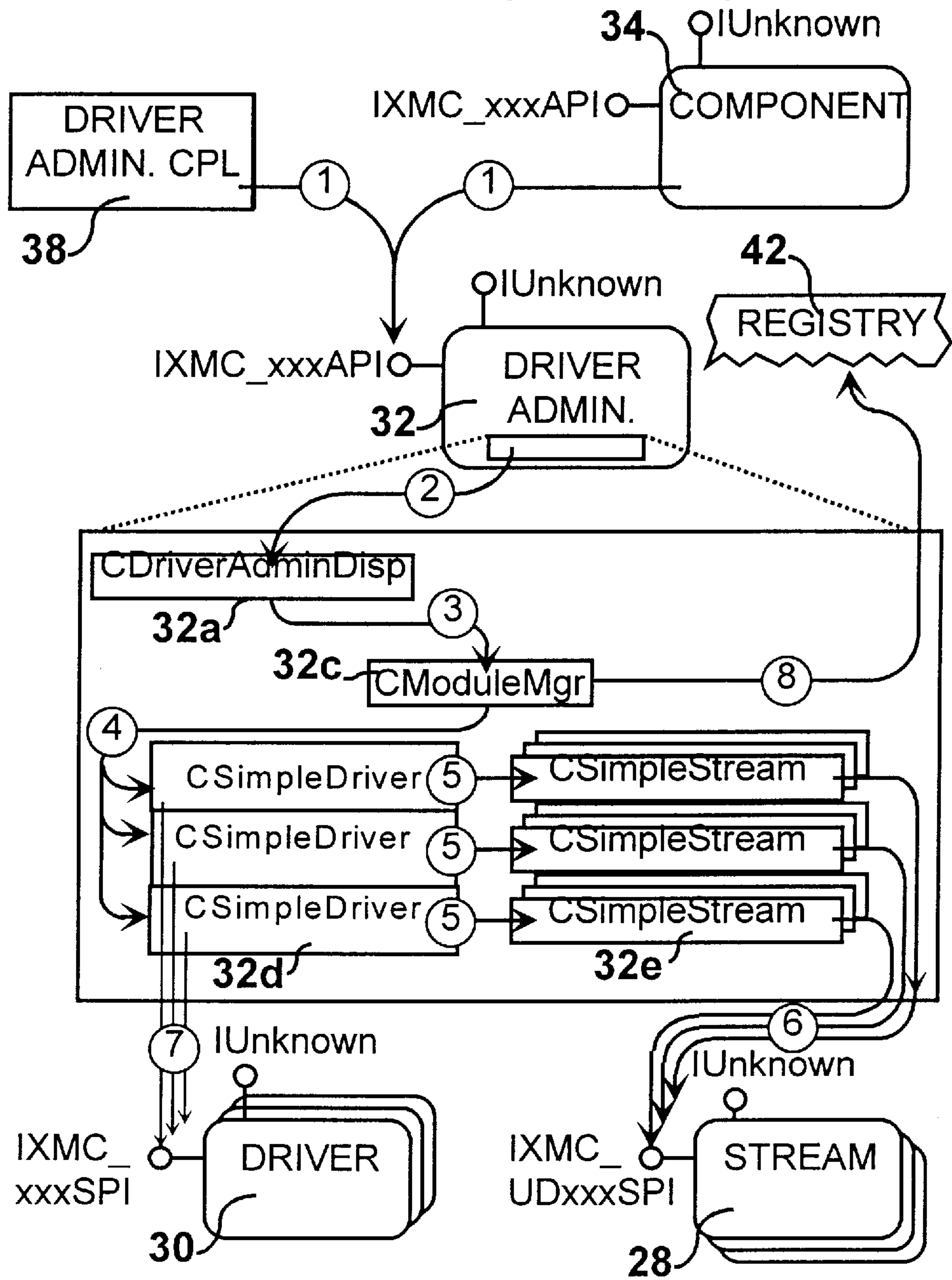
FIG. 49 Scenario-Map - Clean-up
