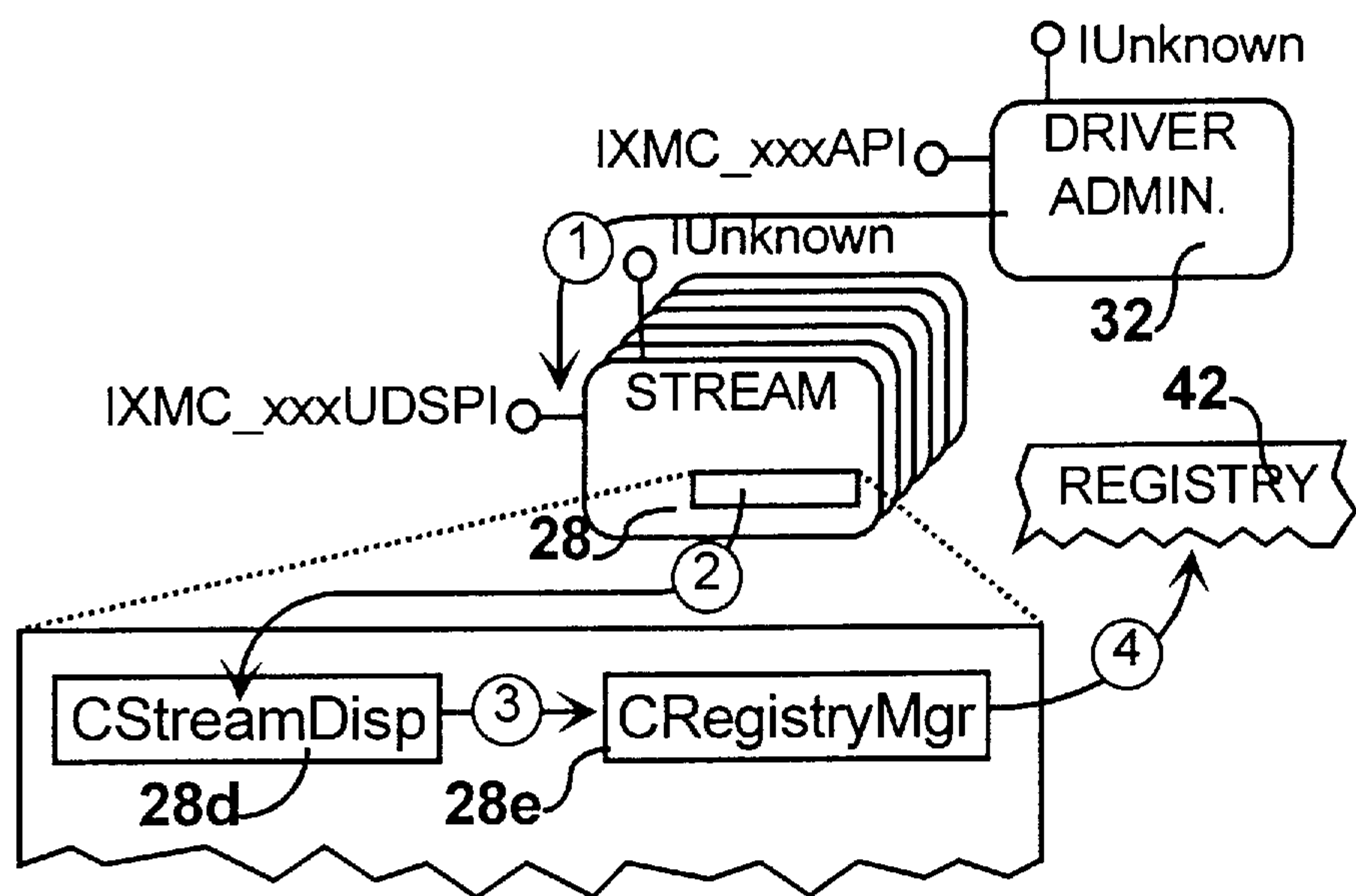
FIG. 27 Scenario-Map - Clean-up
