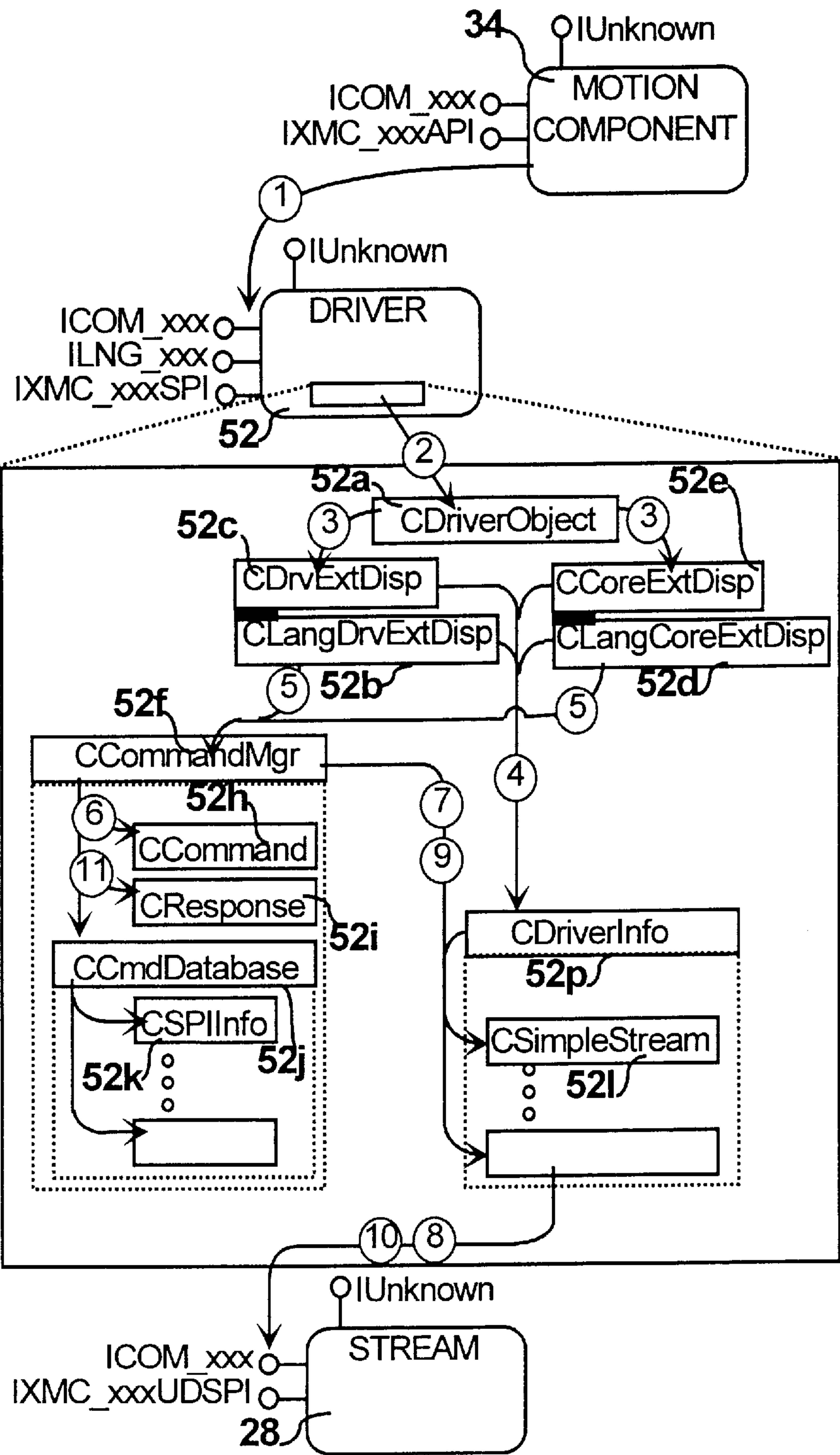
FIG. 65 Scenario-Map - Command Operation
