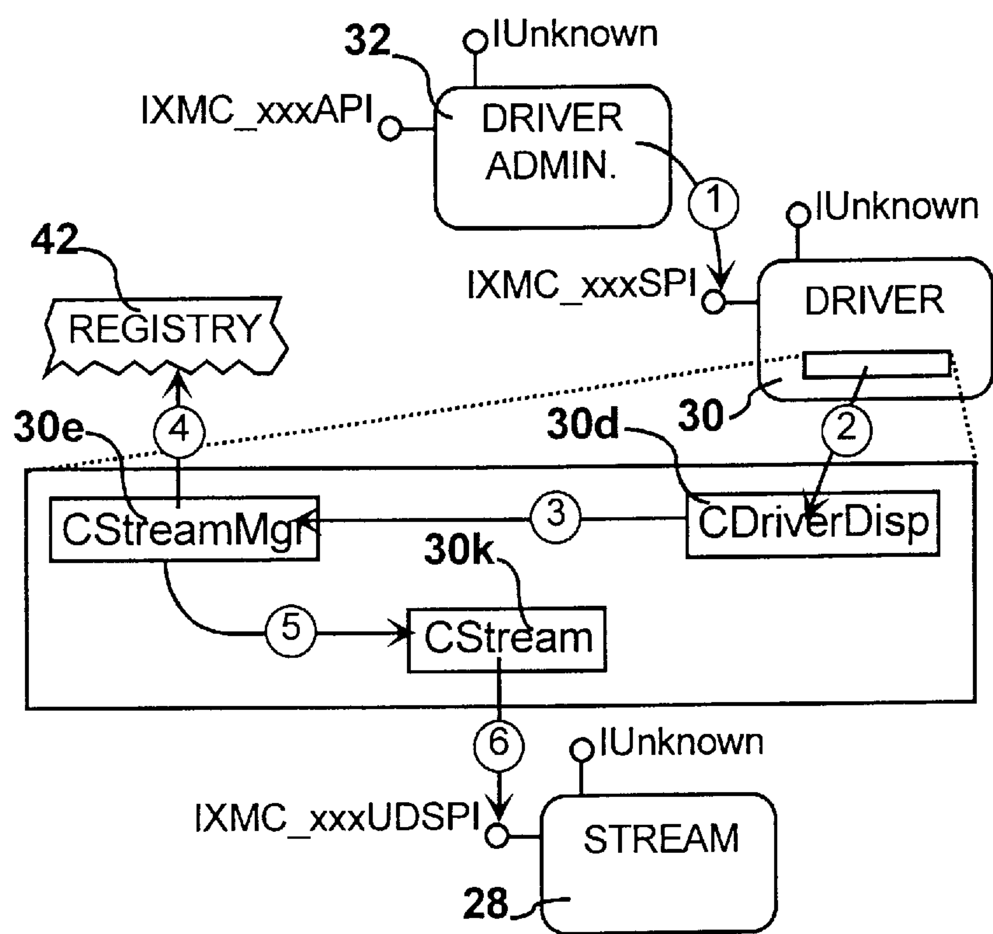
FIG. 16 Scenario-Map - Query Operation
