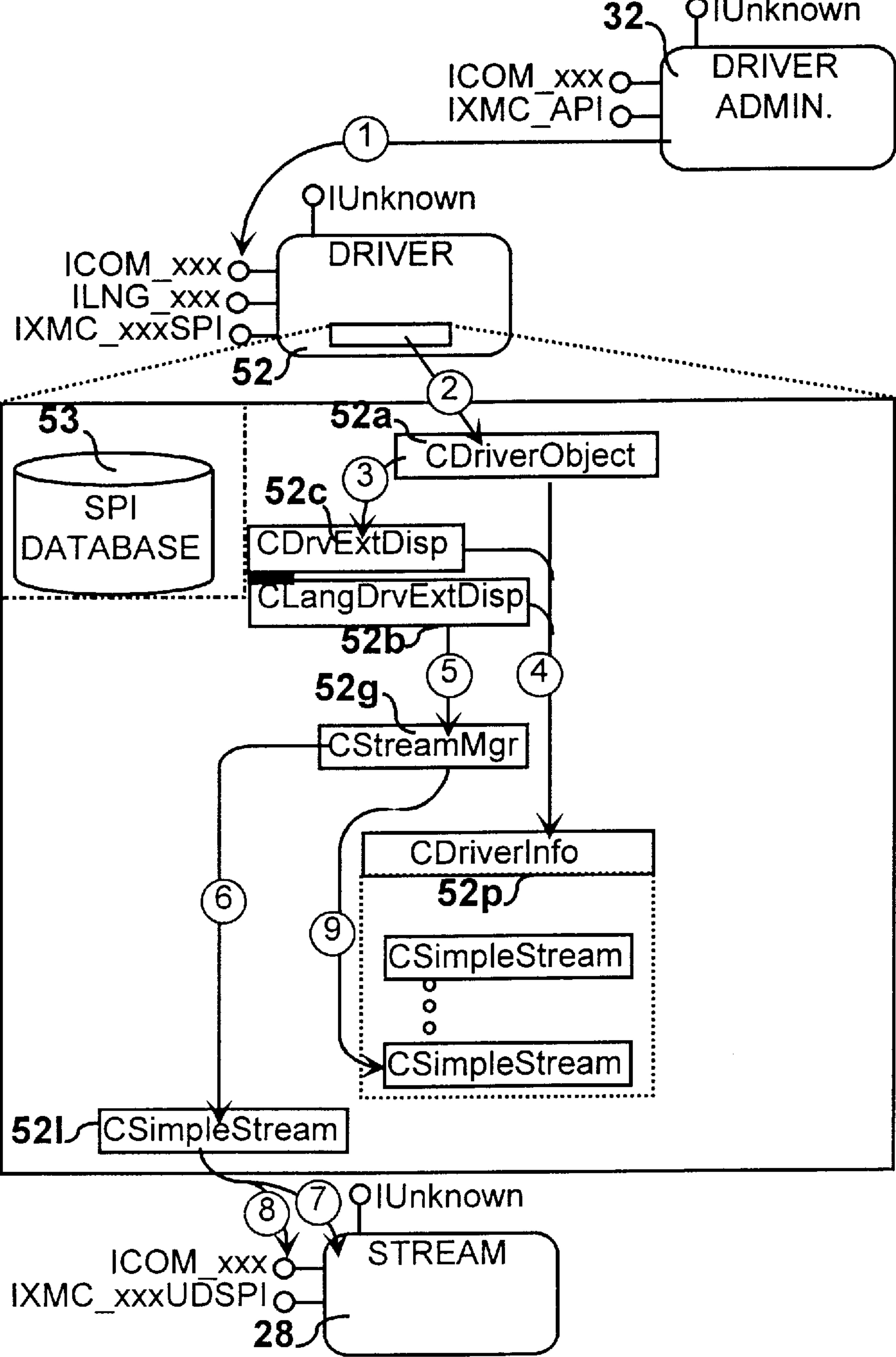
FIG. 61 Scenario-Map - Adding a Stream
