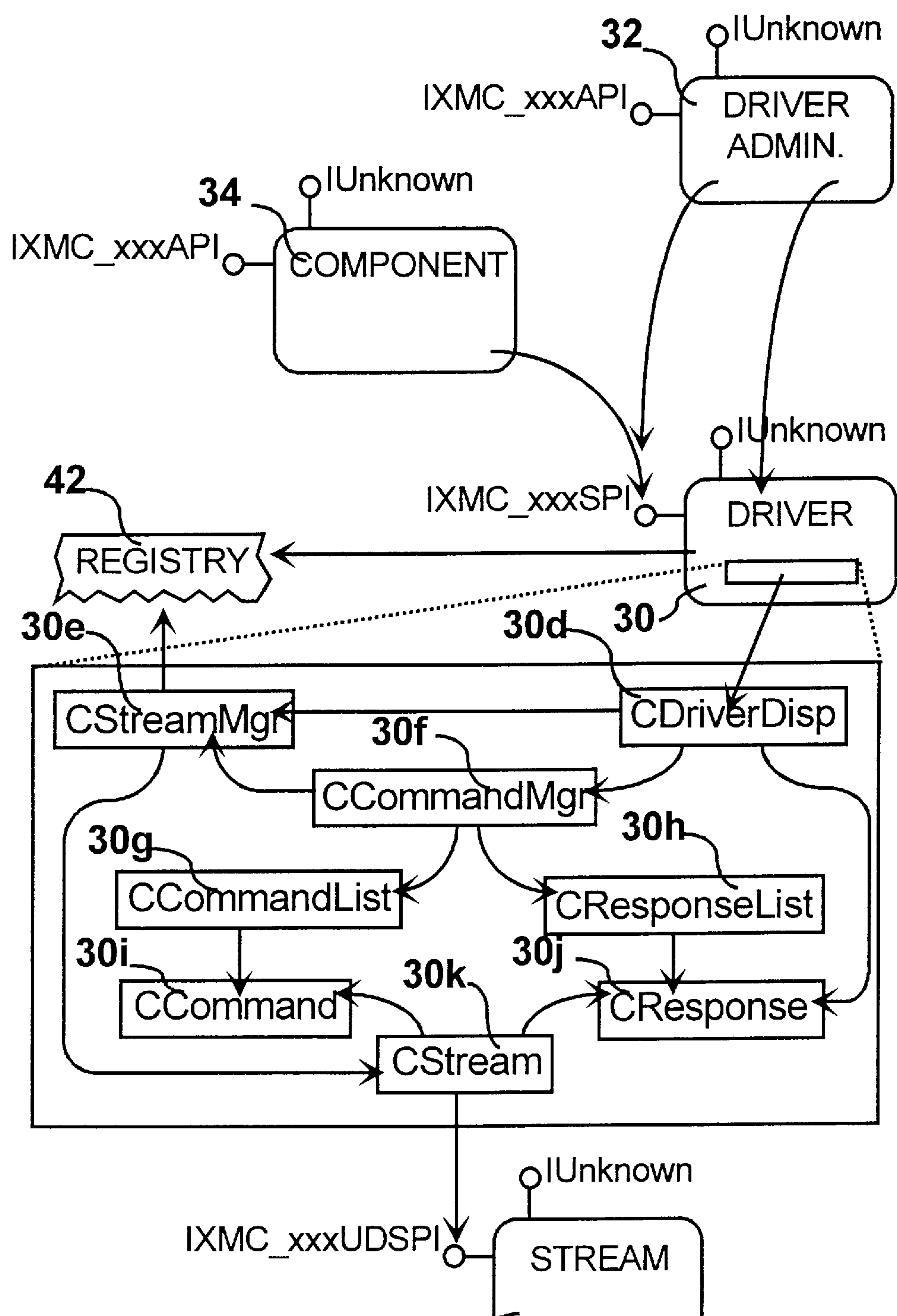
FIG. 12 Object Interaction-Map
