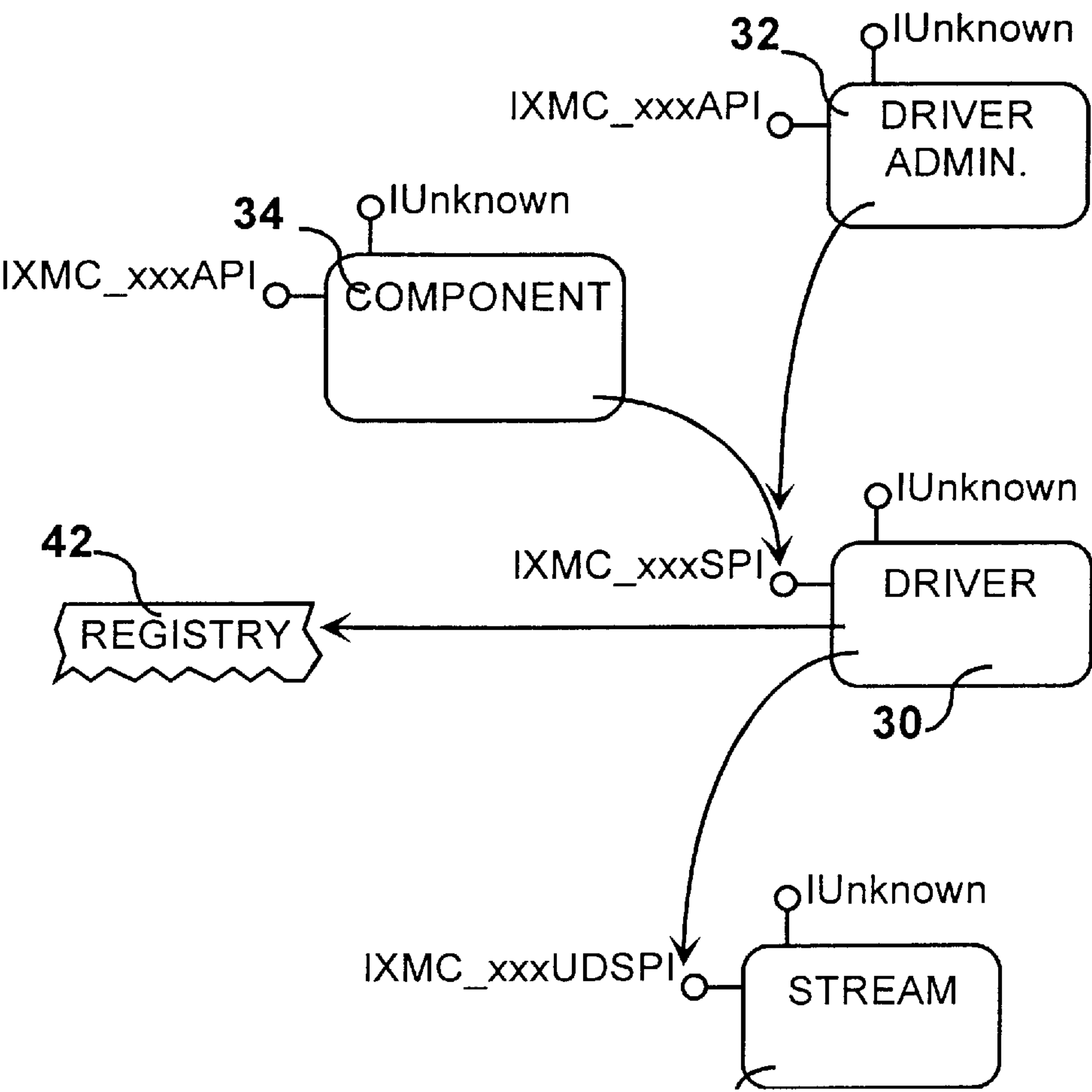
FIG. 11 Module Interaction-Map
