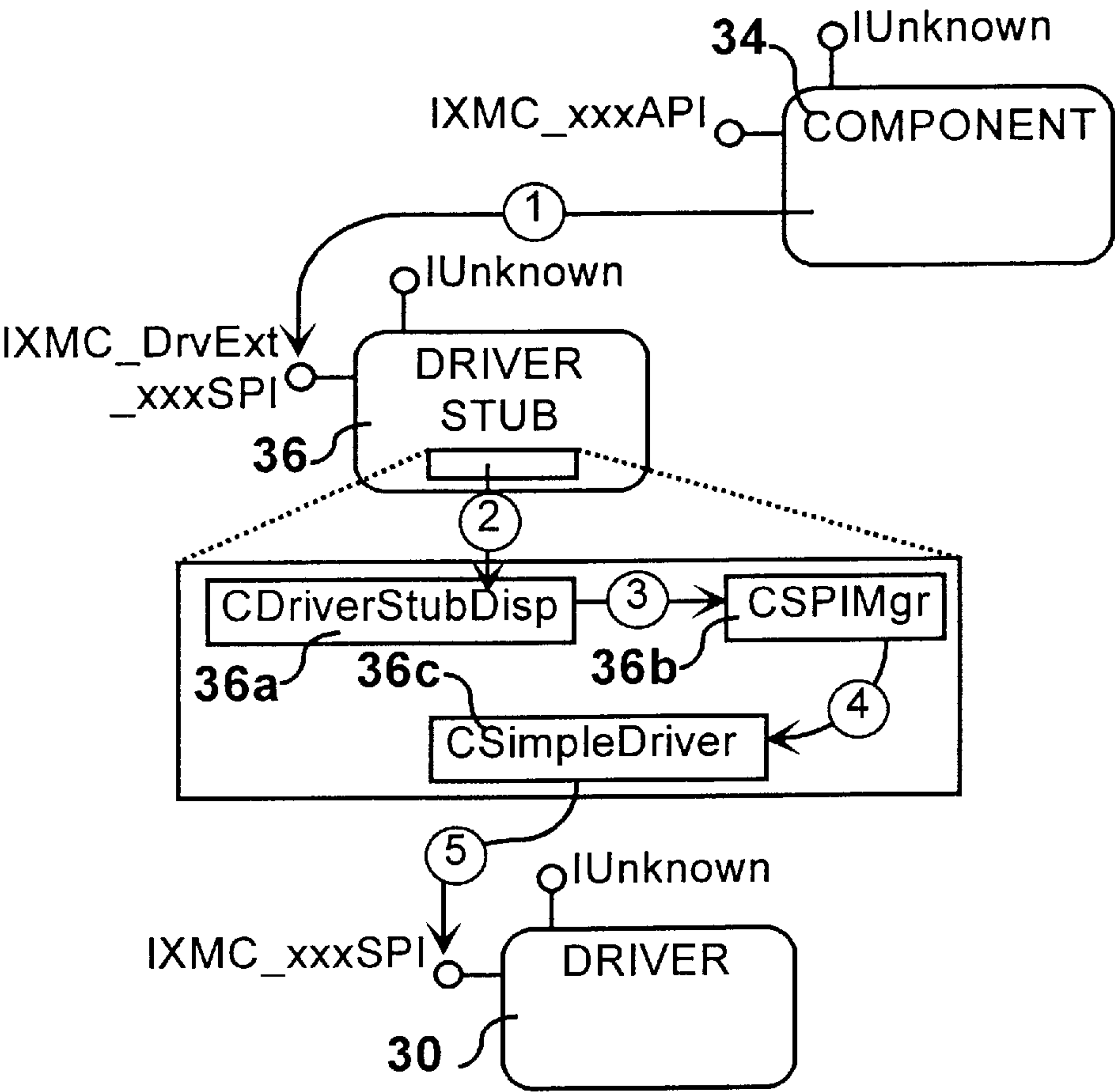
FIG. 37 Scenario-Map - Operations
