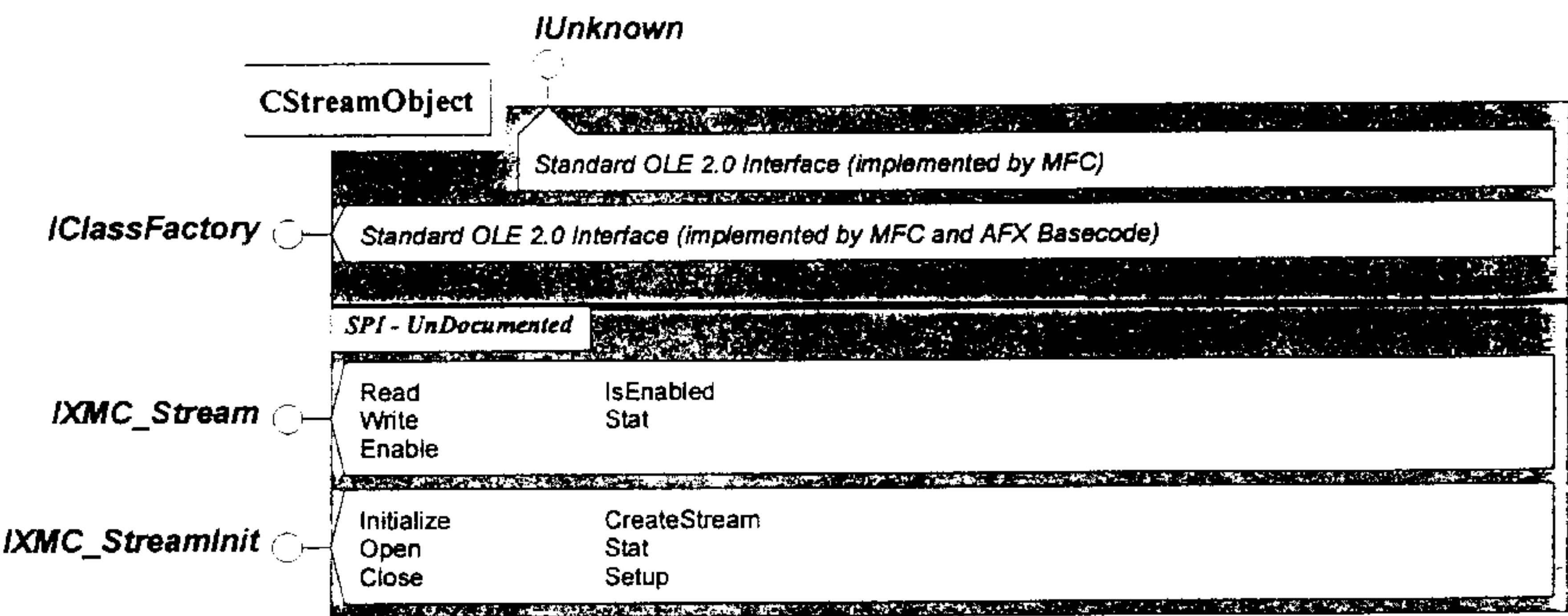
Figure 12 Interface-Map.
