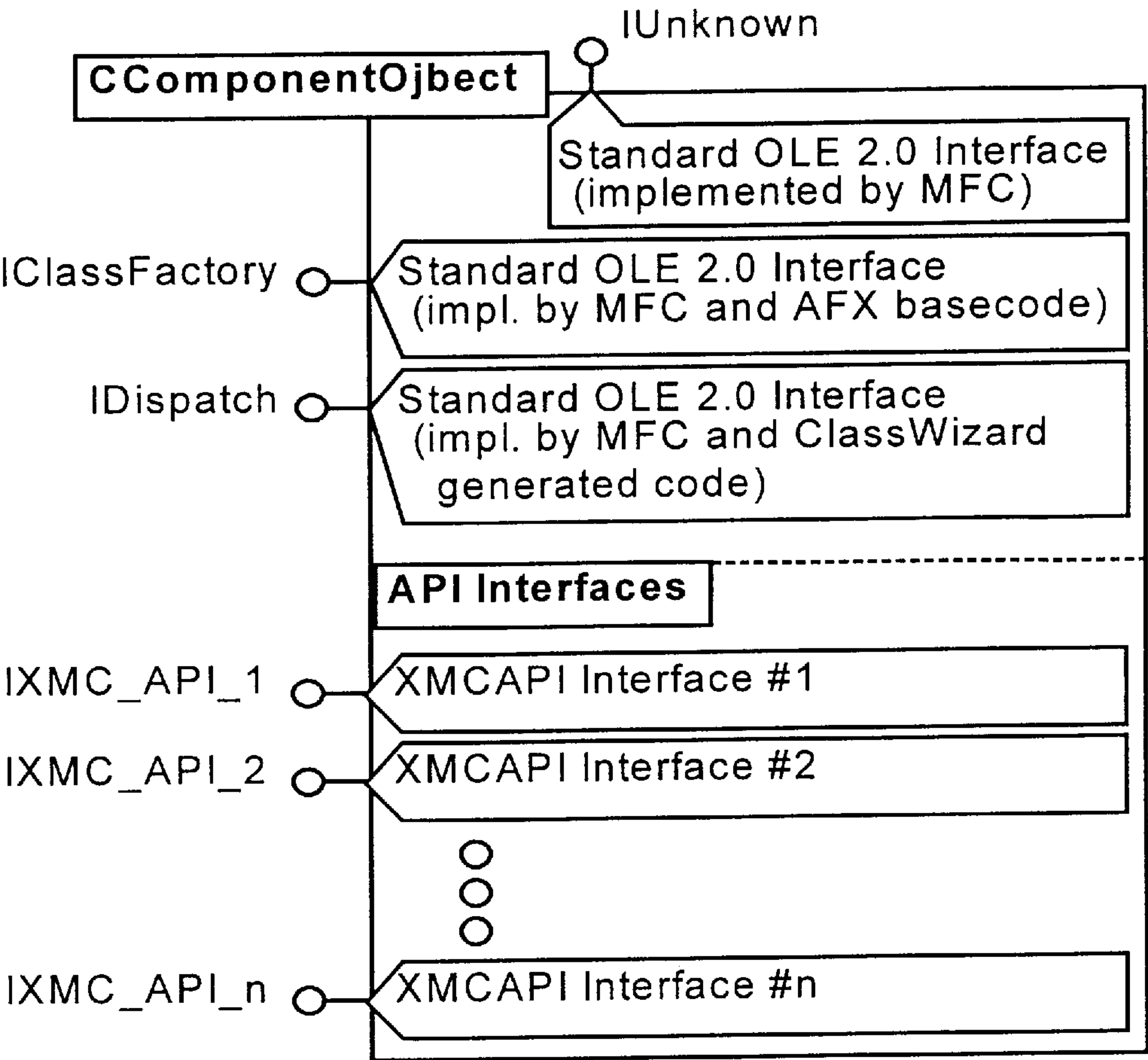
FIG. 9 Interface-Map
