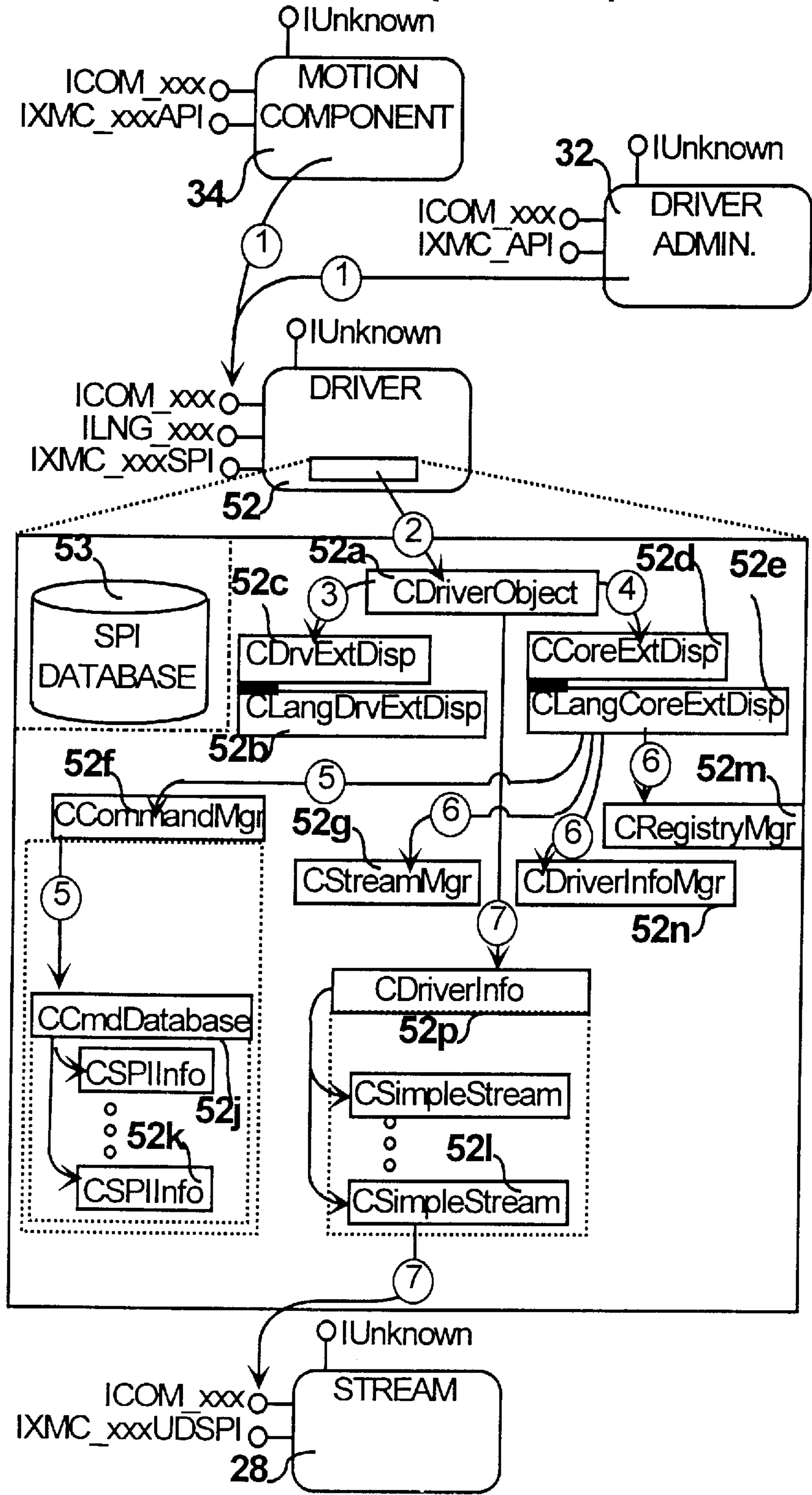
FIG. 64 Scenario-Map - Clean-up
