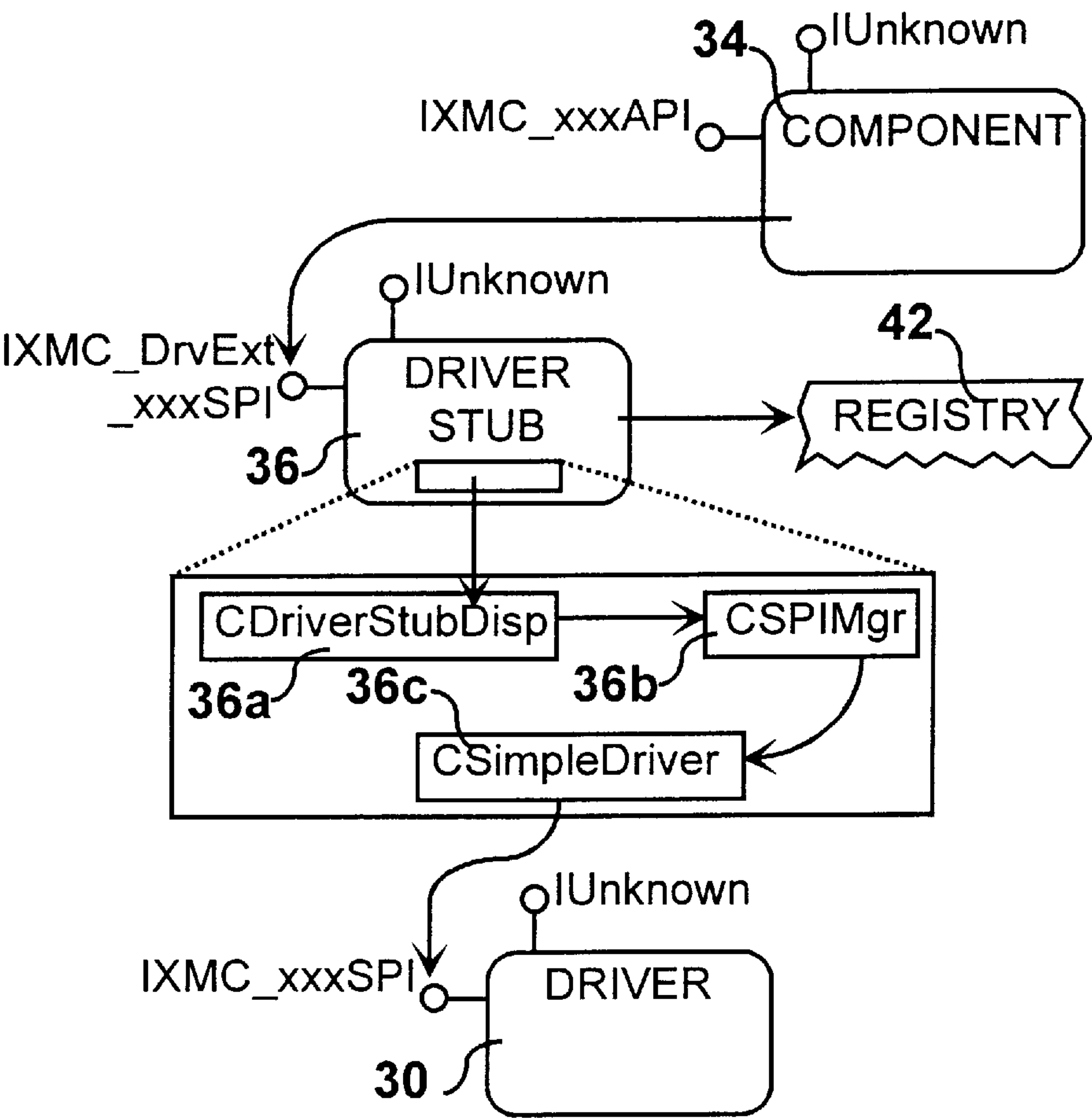
FIG. 35 Object Interaction-Map
