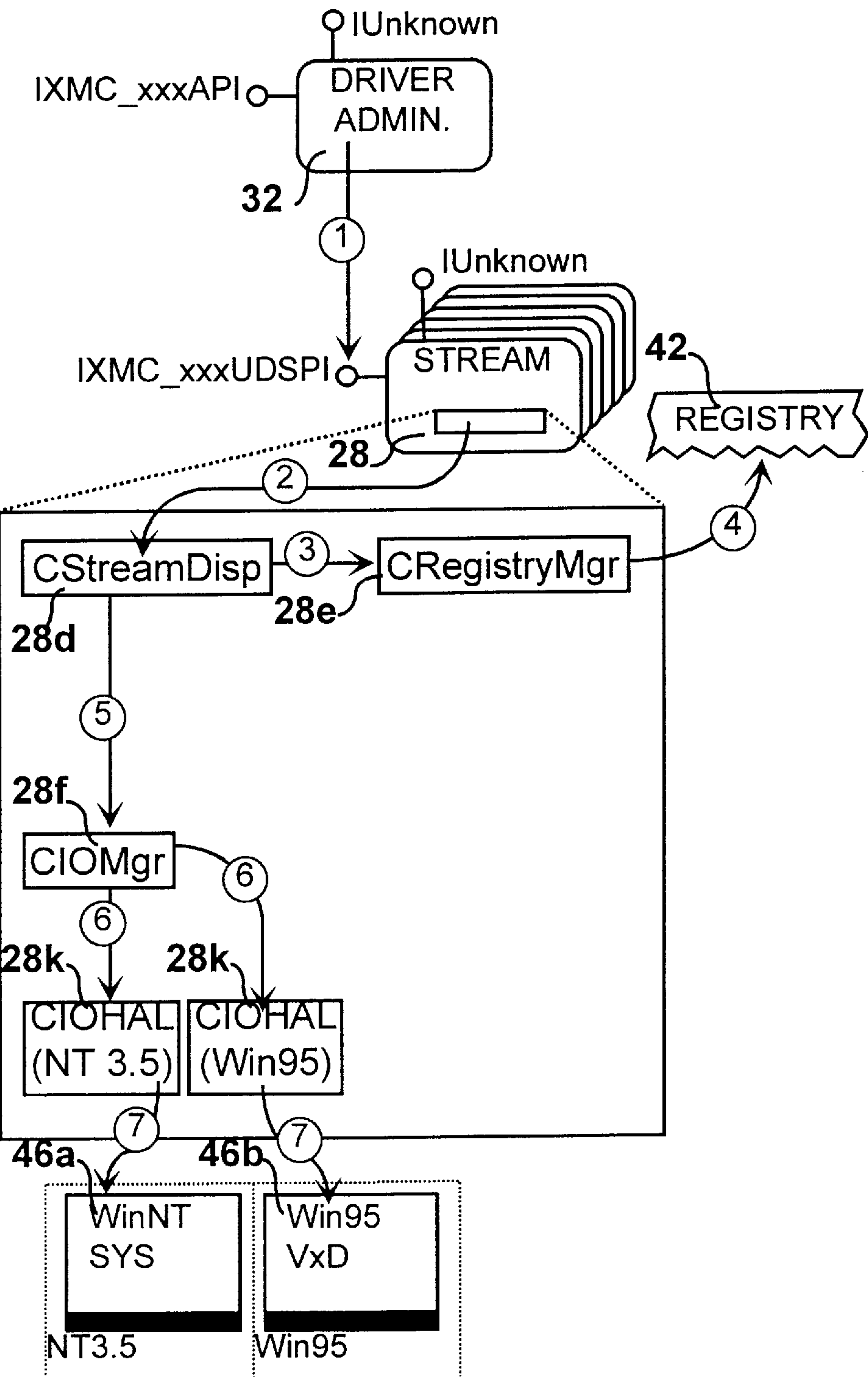
FIG. 24 Scenario-Map - Initialization
