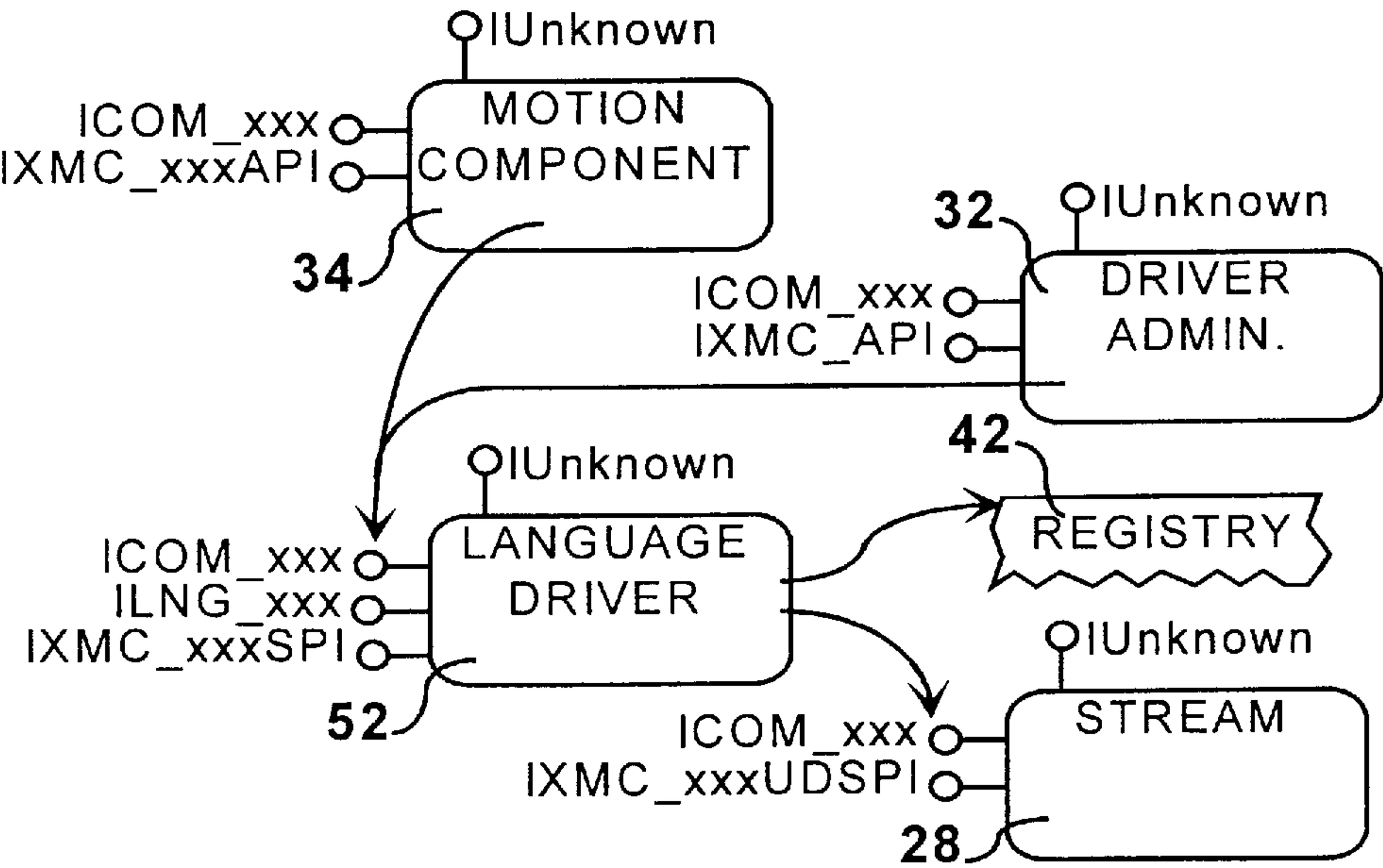
FIG. 58 Module Interaction-Map
