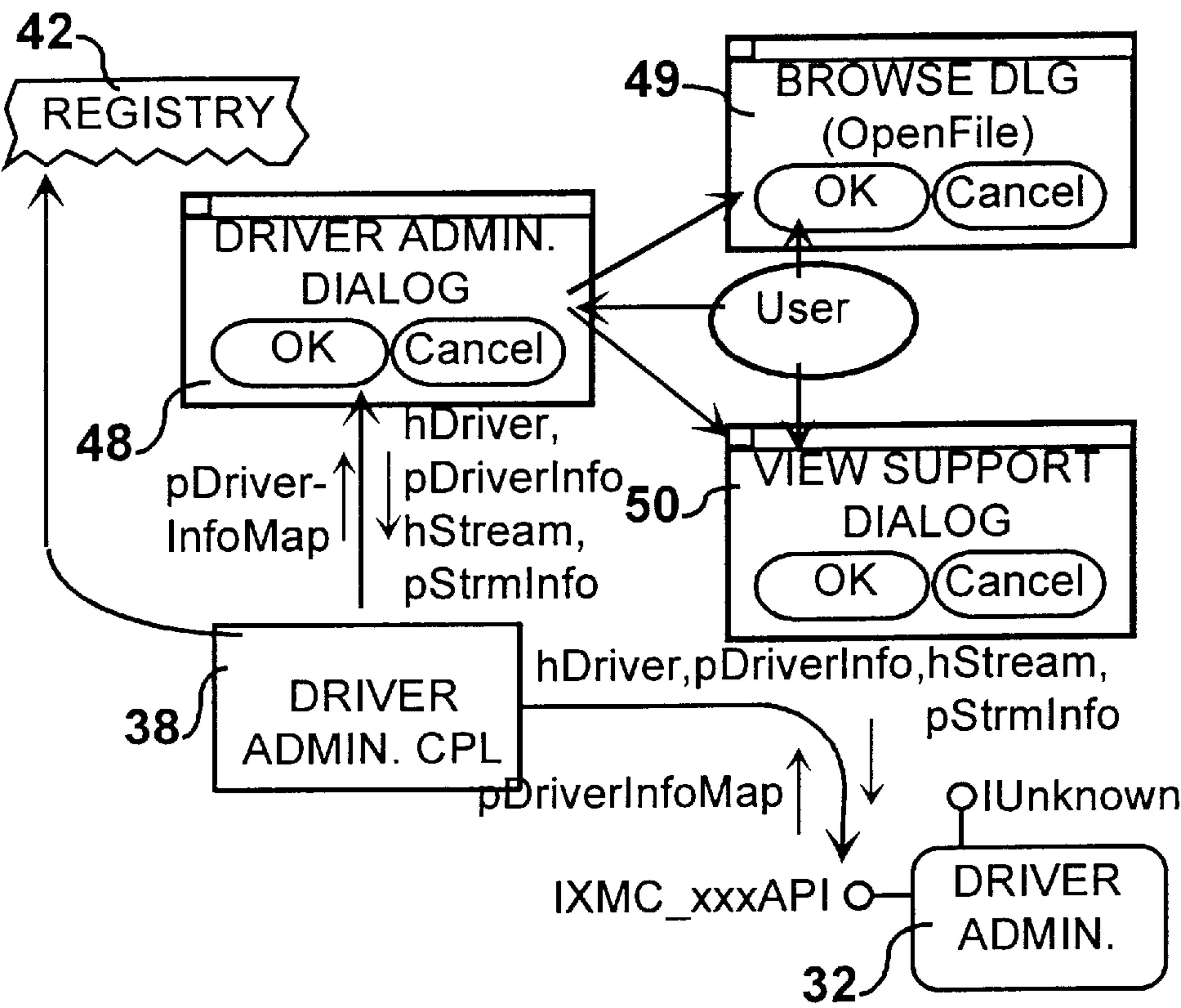
FIG. 51 Module Interaction-Map
