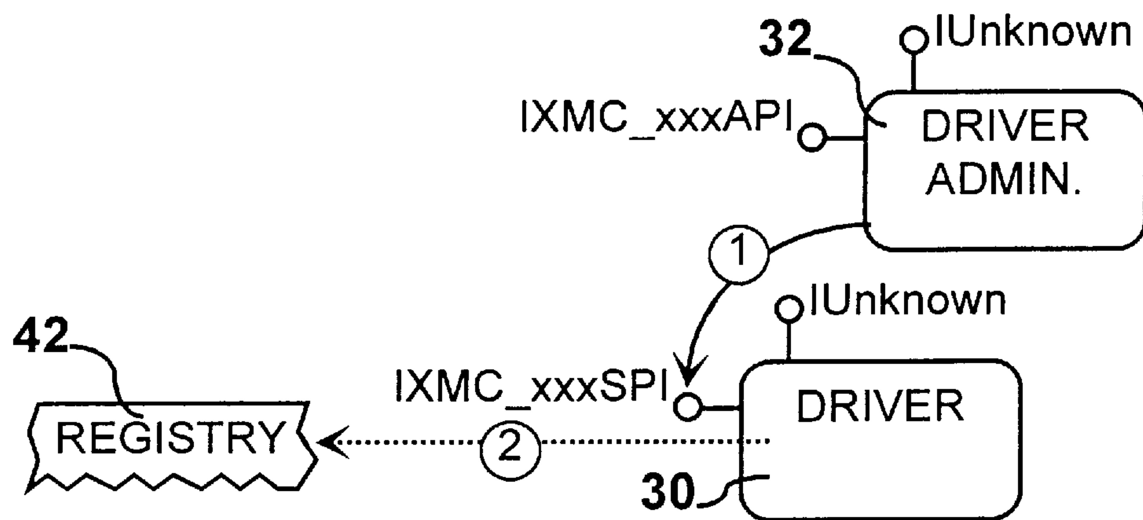
FIG. 13 Scenario-Map - Registration
