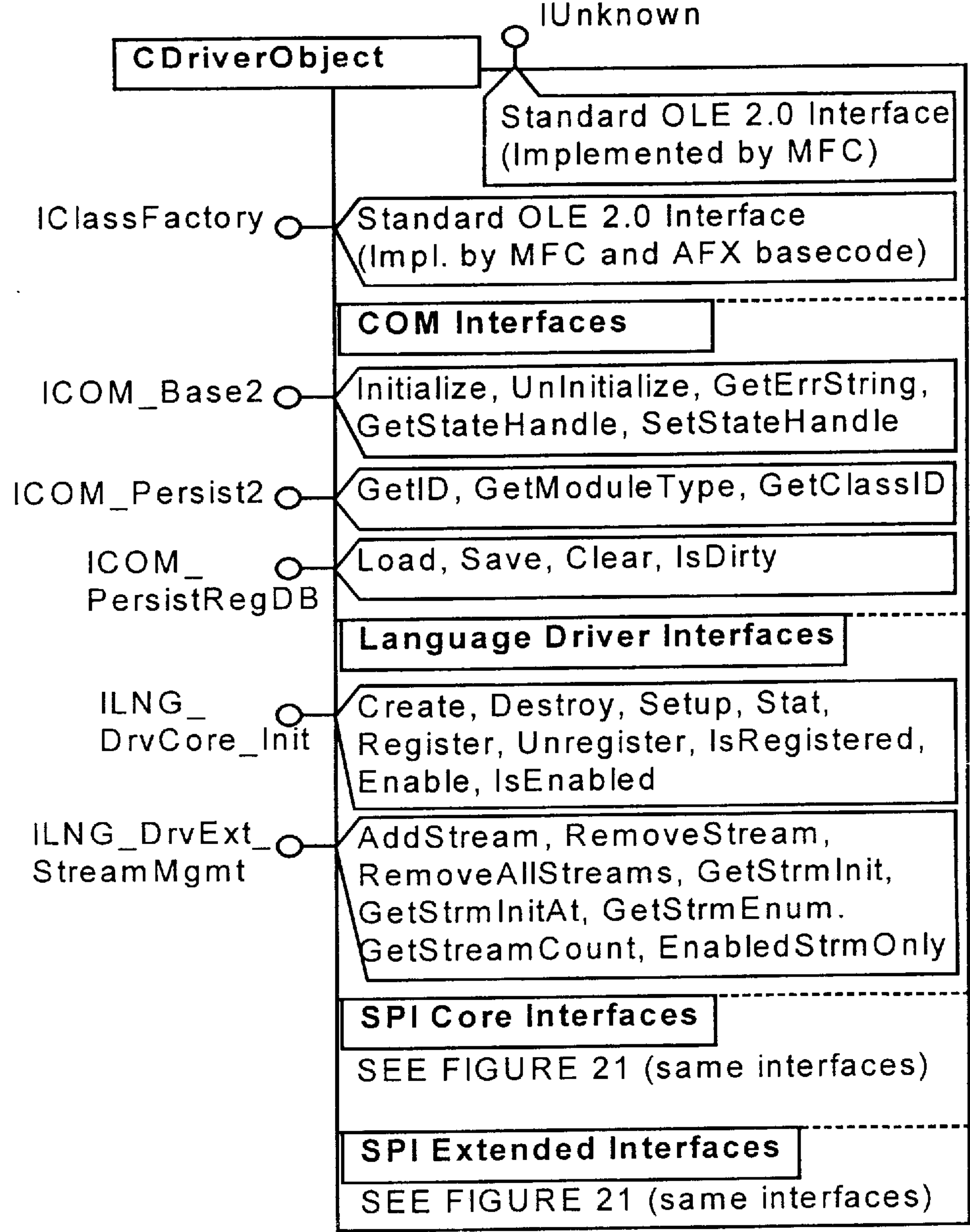
FIG. 66 Interface-Map
