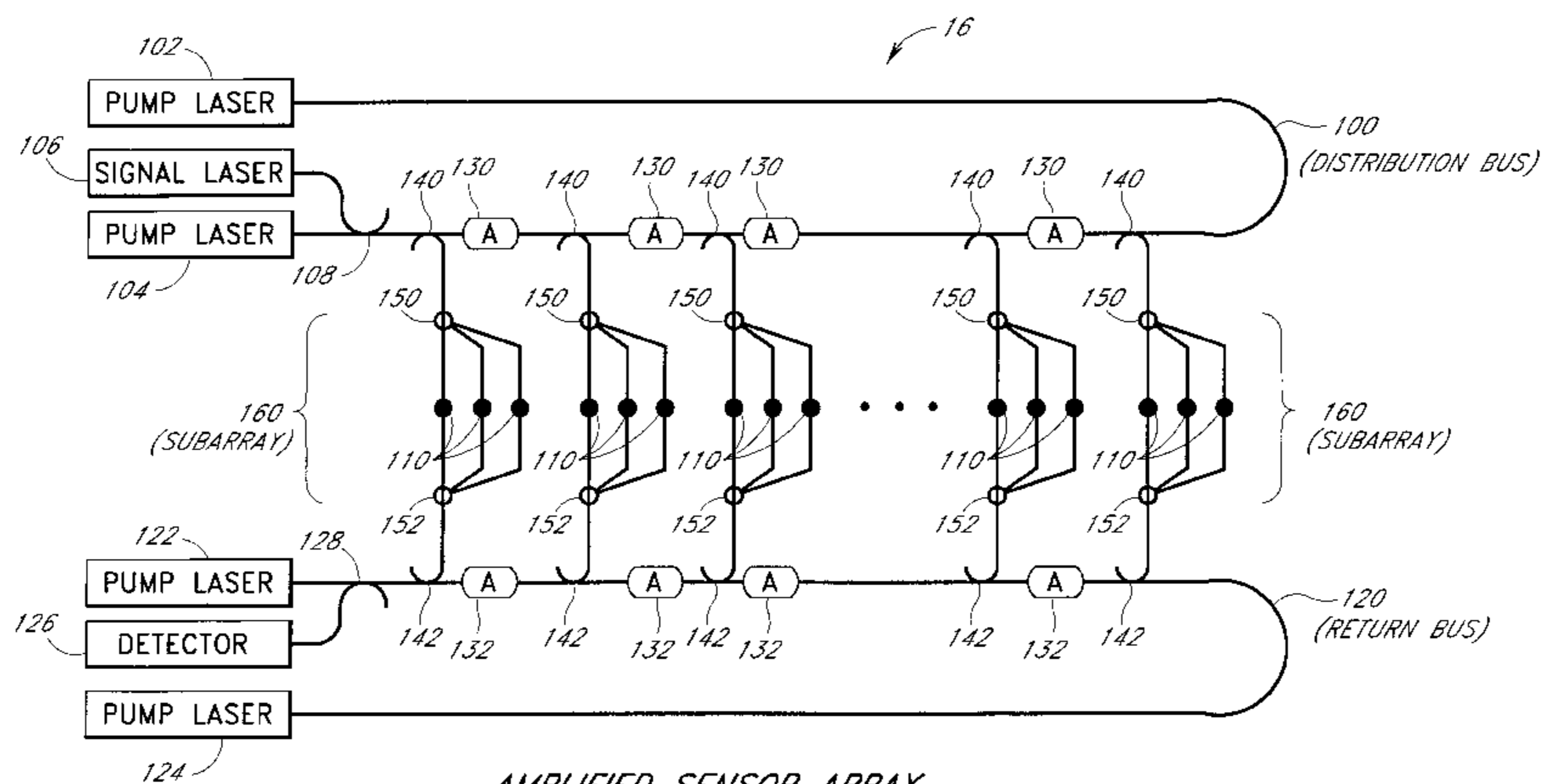
AMPLIFIED SENSOR ARRAY WITH 3 SENSORS PER SUB-ARRAY
