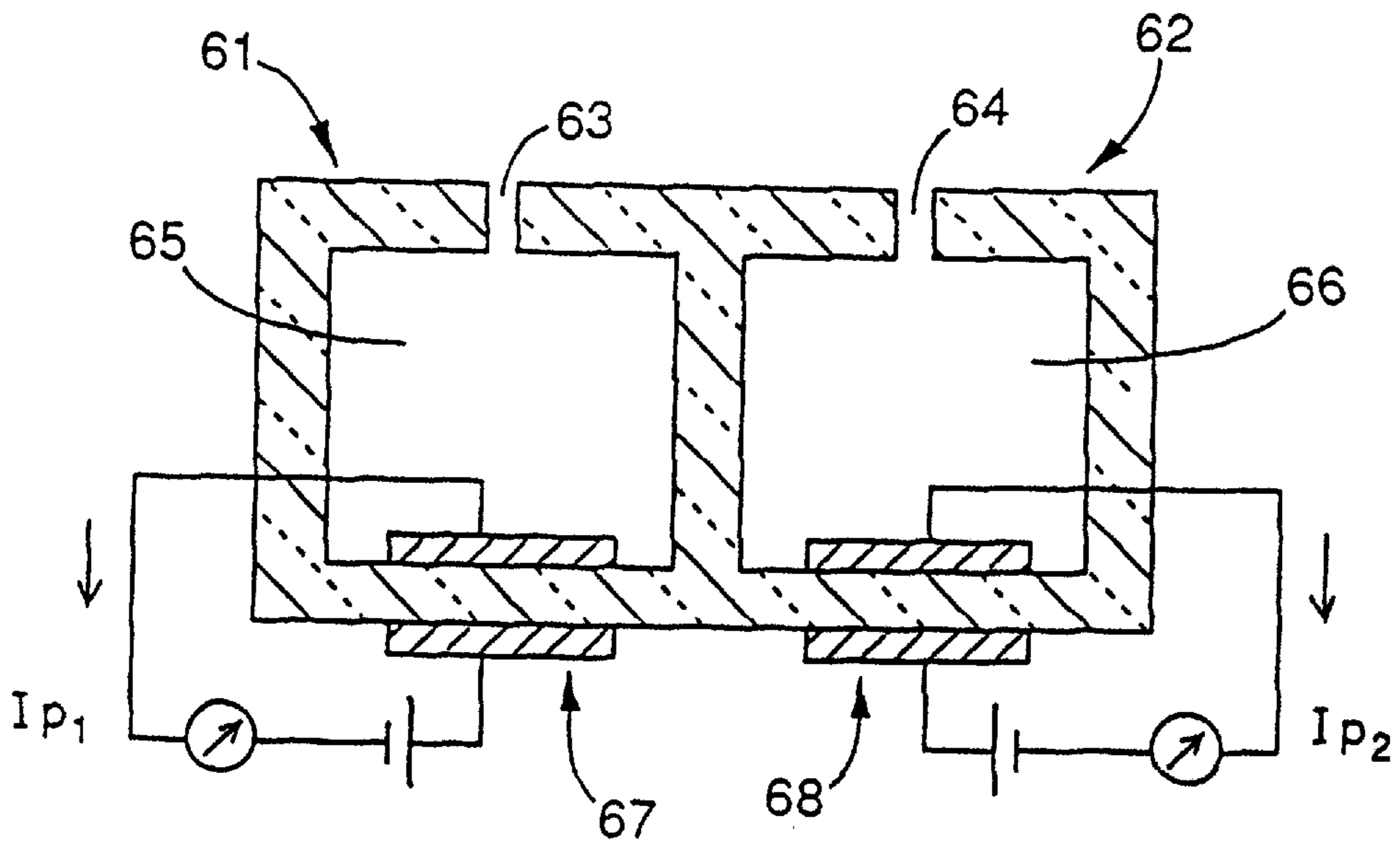
FIG. 25 PRIOR ART
