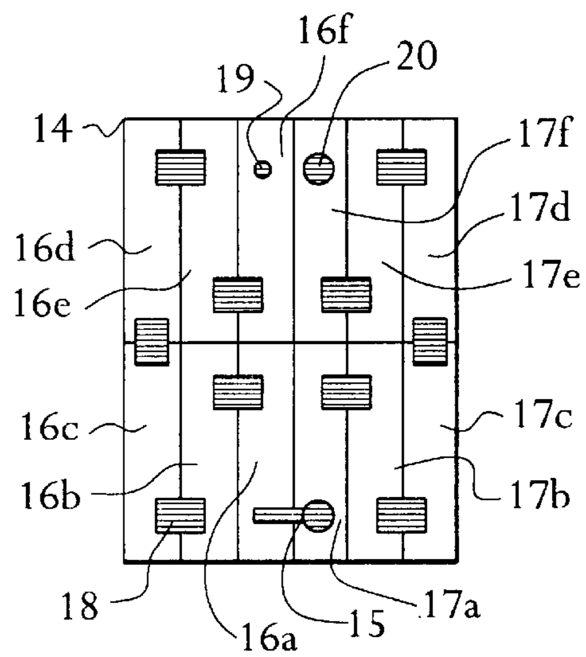
FIG. 3 Prior Art
