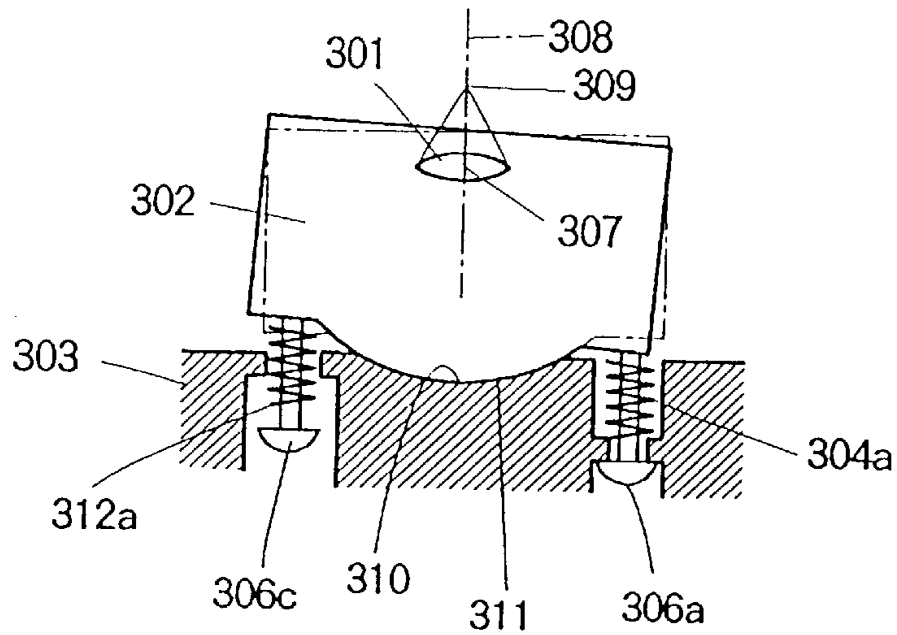
FIG. 23 PRIOR ART
