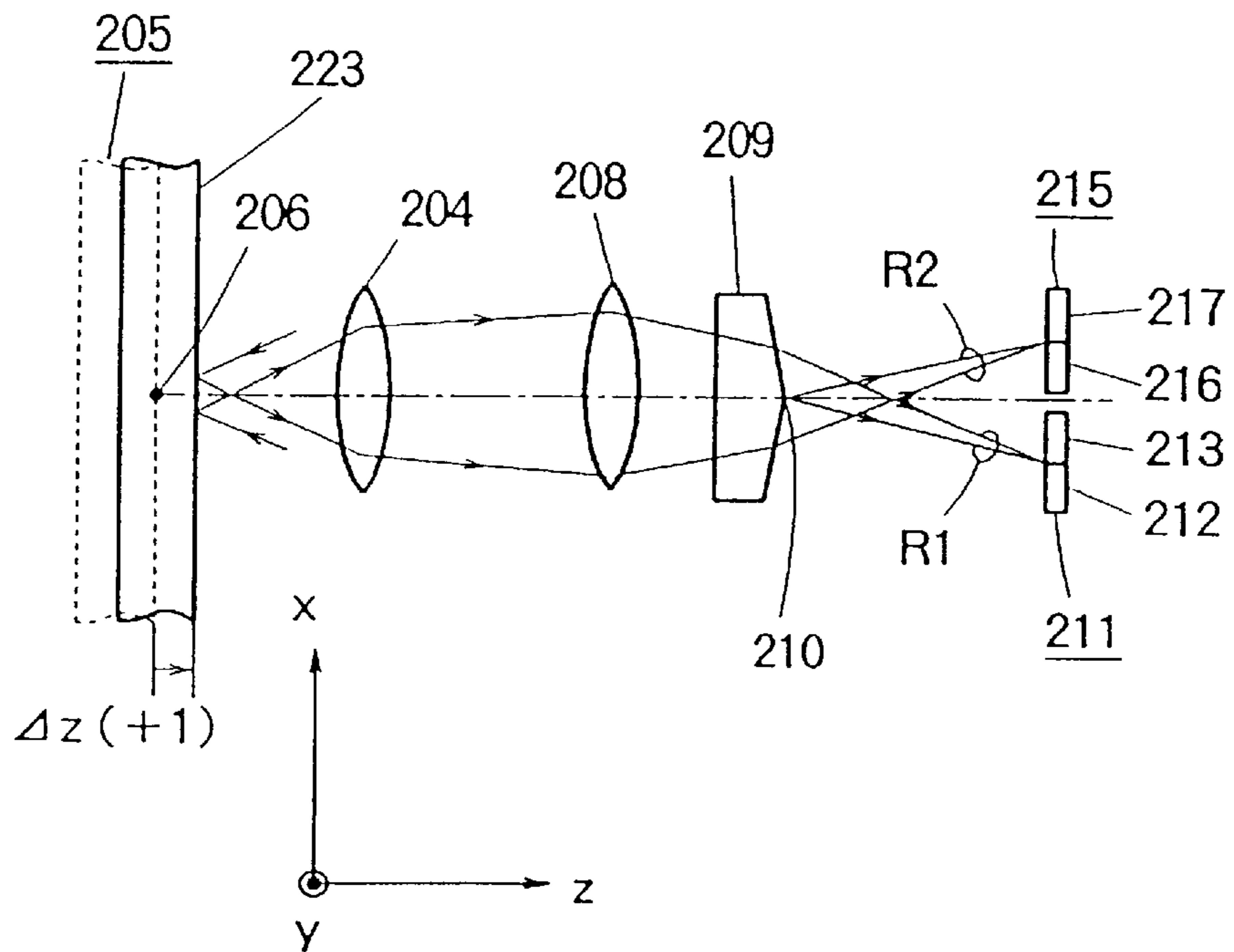
FIG. 18 PRIOR ART
