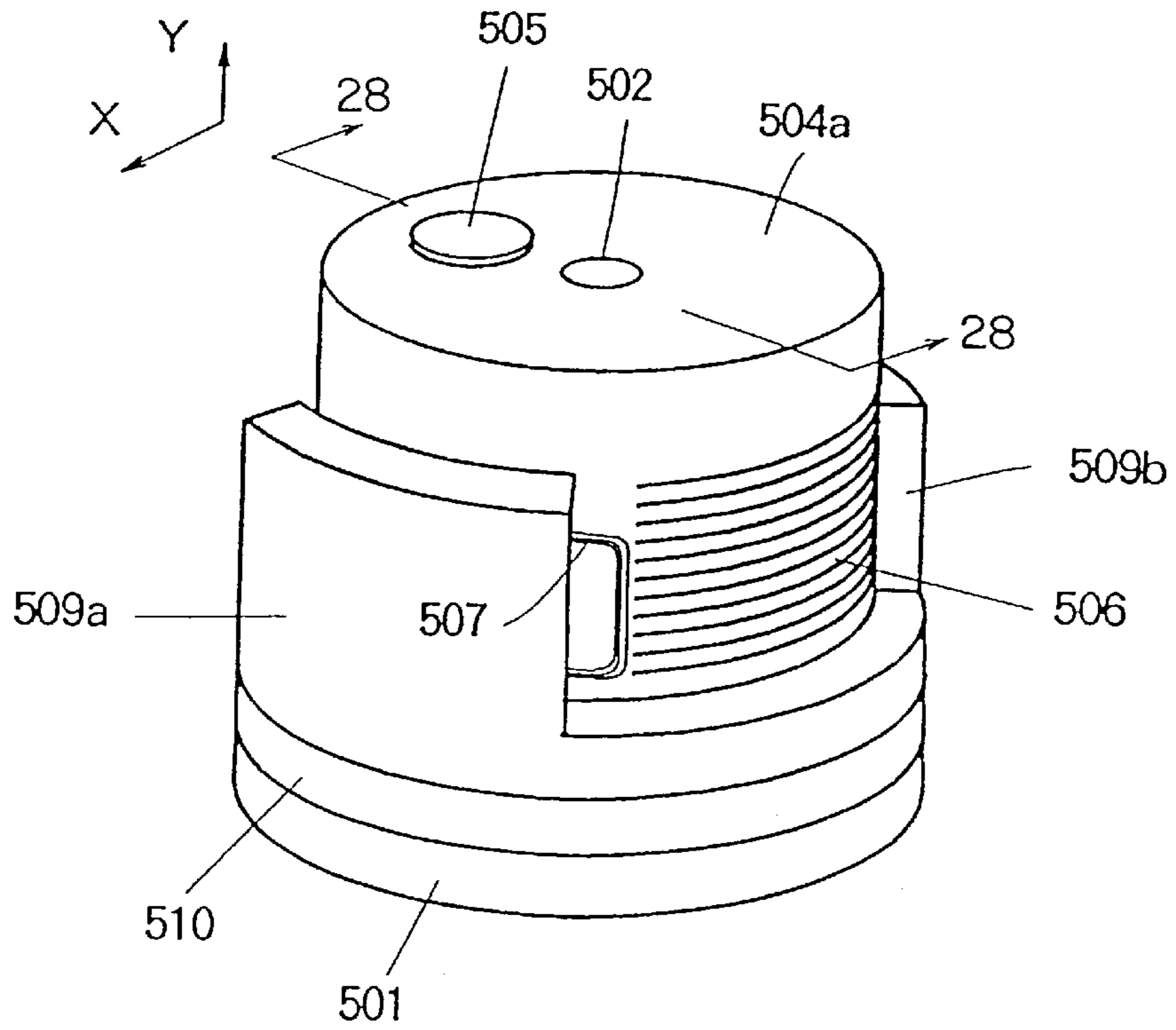
FIG. 27 PRIOR ART
