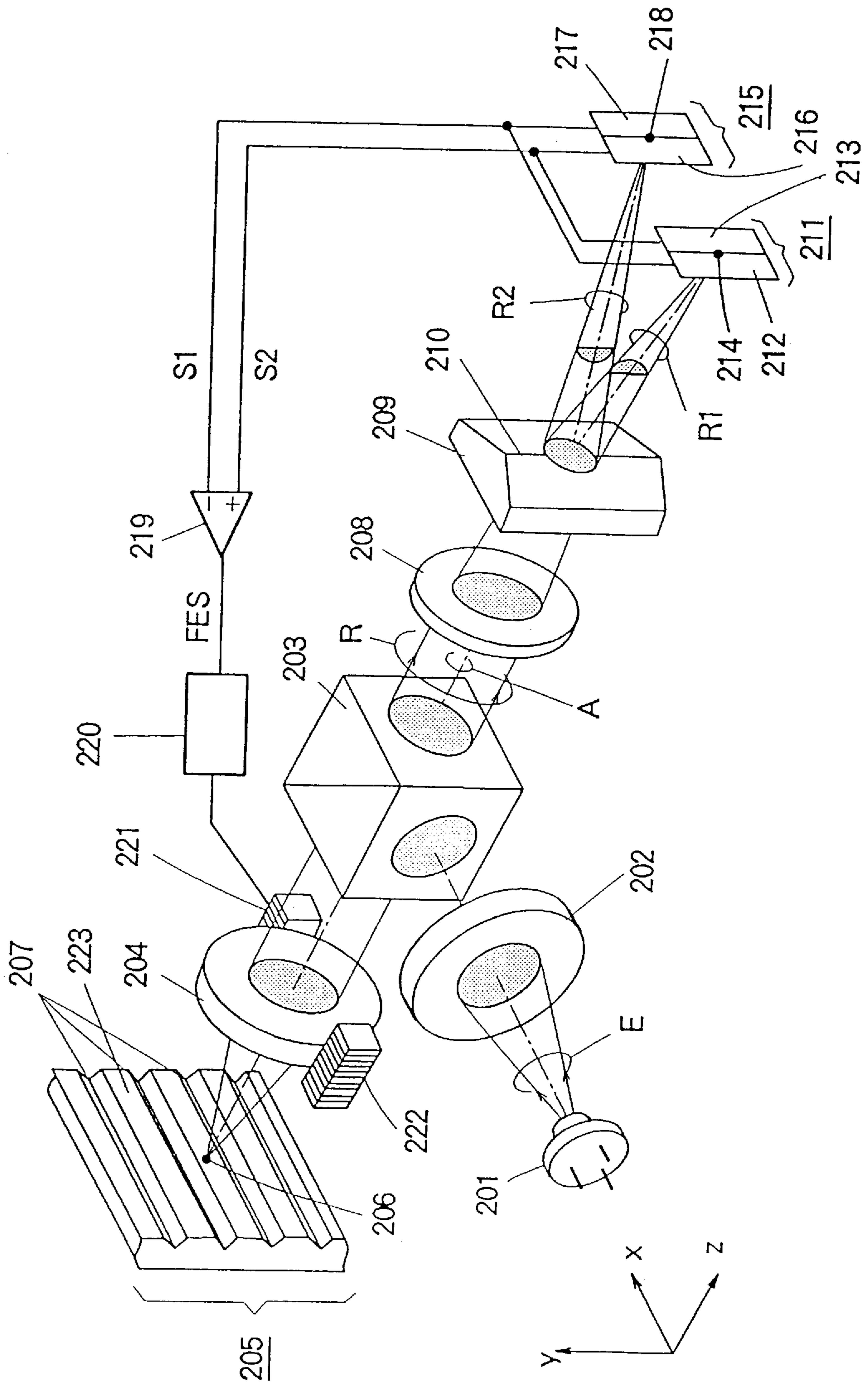
FIG. 16 PRIOR ART
