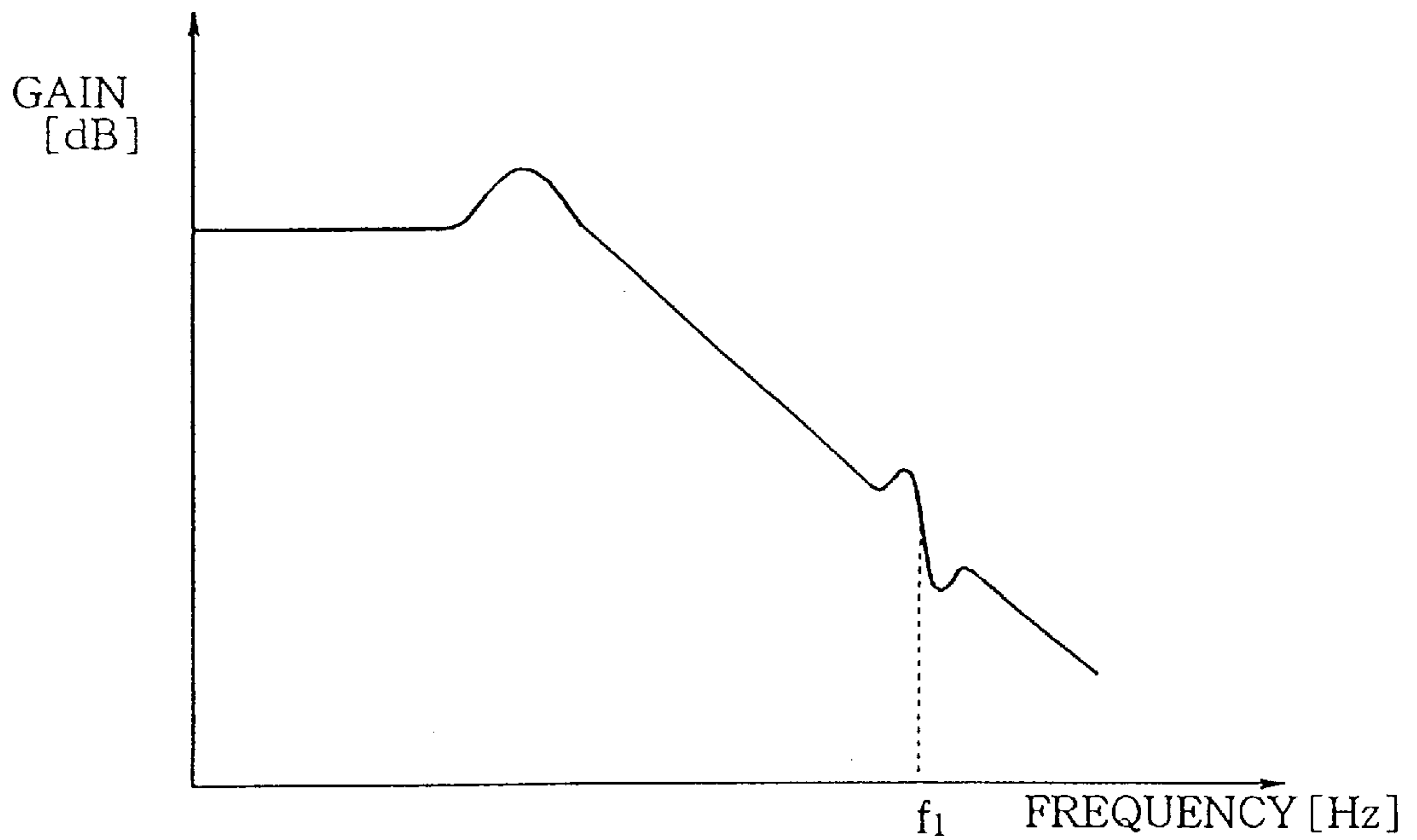
FIG. 26 PRIOR ART
