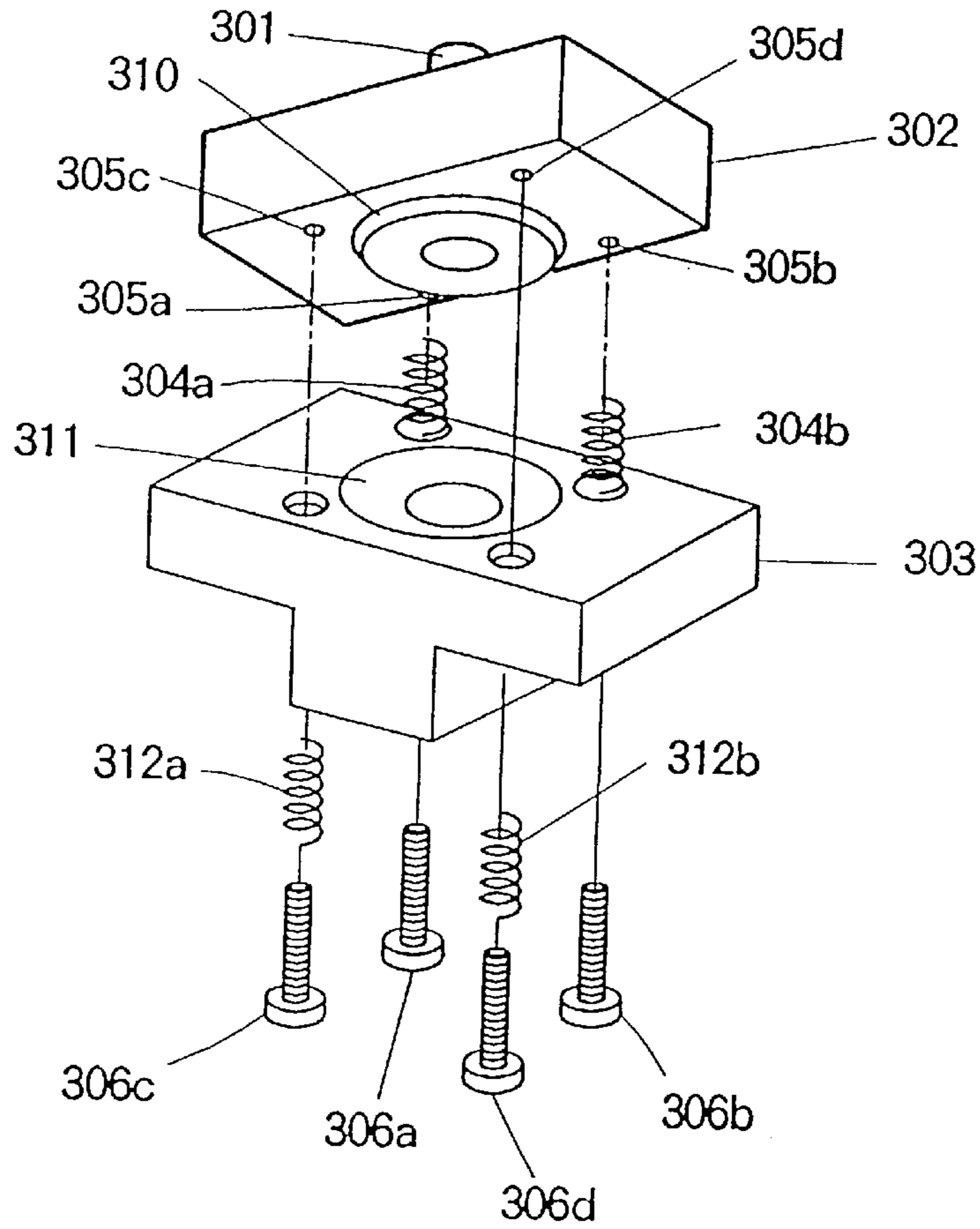
FIG. 22 PRIOR ART
