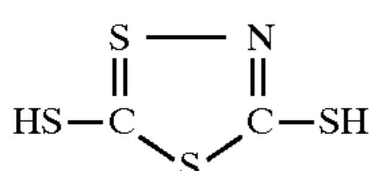
3,4-dimercapto-1,2,5-thiadiazole
