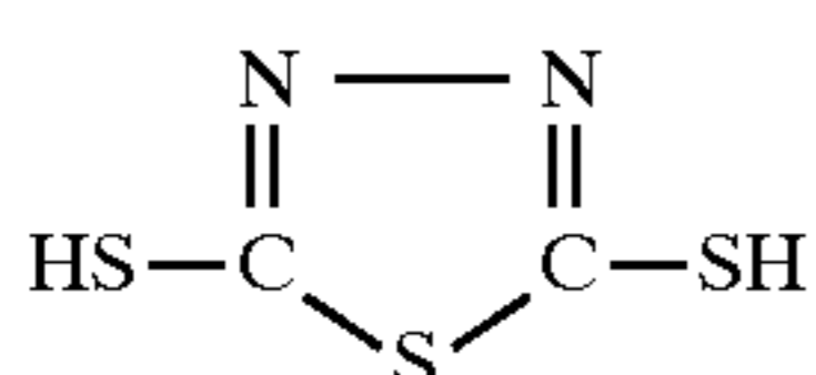
3,5-dimercapto-1,2,4-thiadiazole
