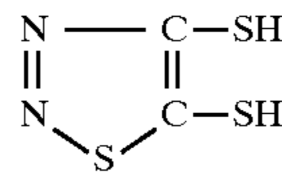
4,5-dimercapto-1,2,3-thiadiazole
