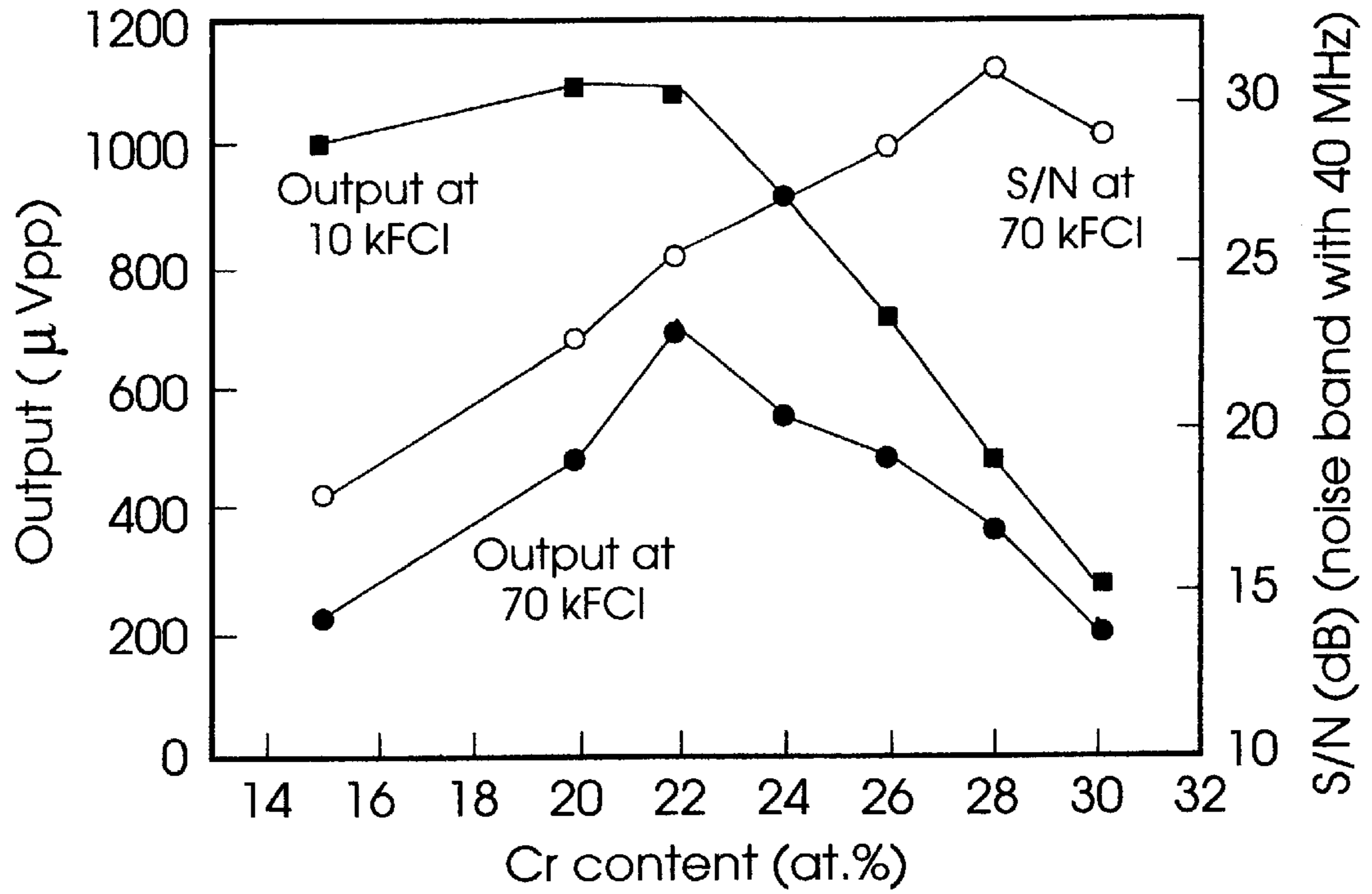
Dependencies of the output and S/N on the Cr content
