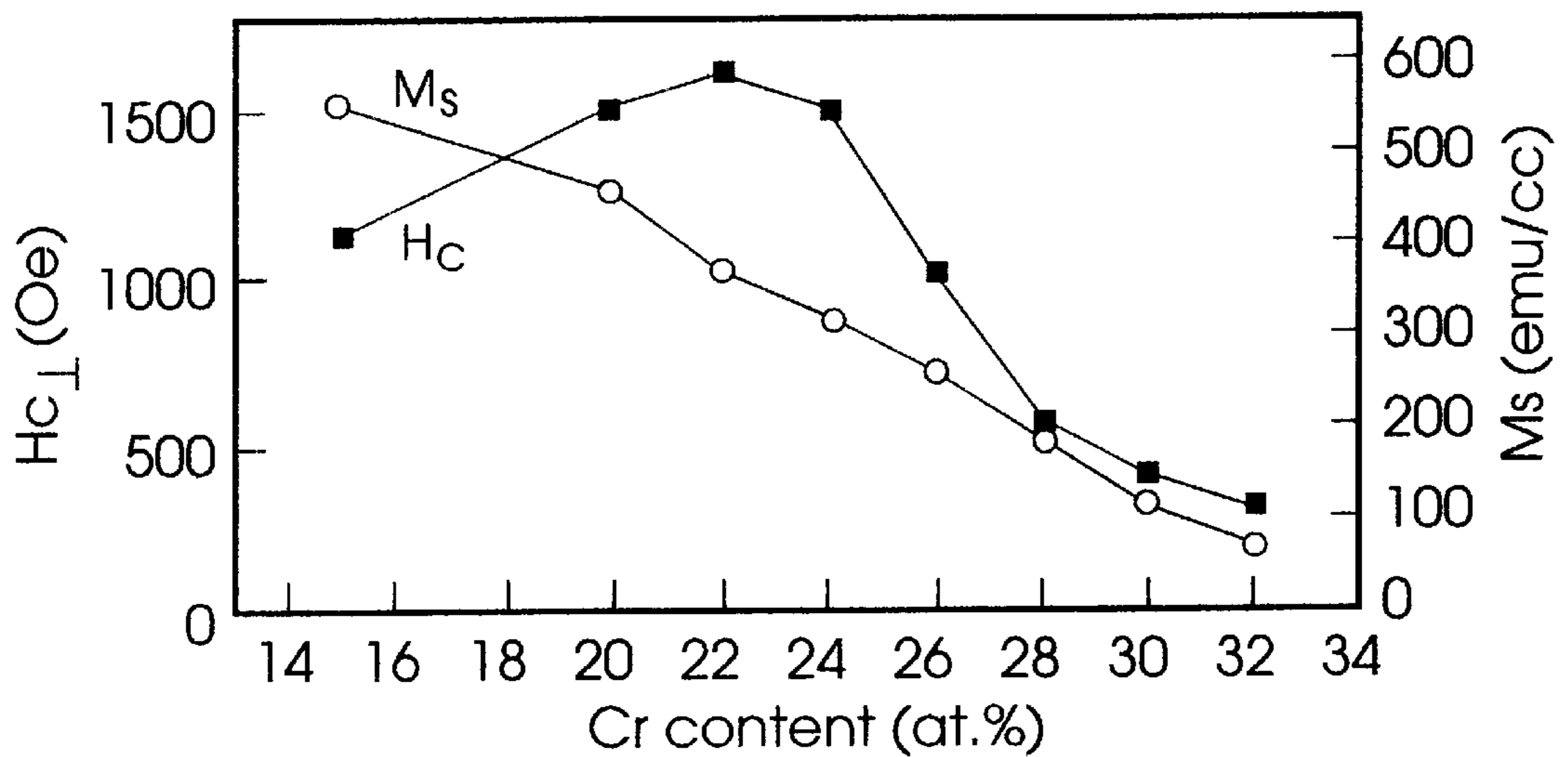
Hc ⊥ and Ms dependencies on the Cr content
