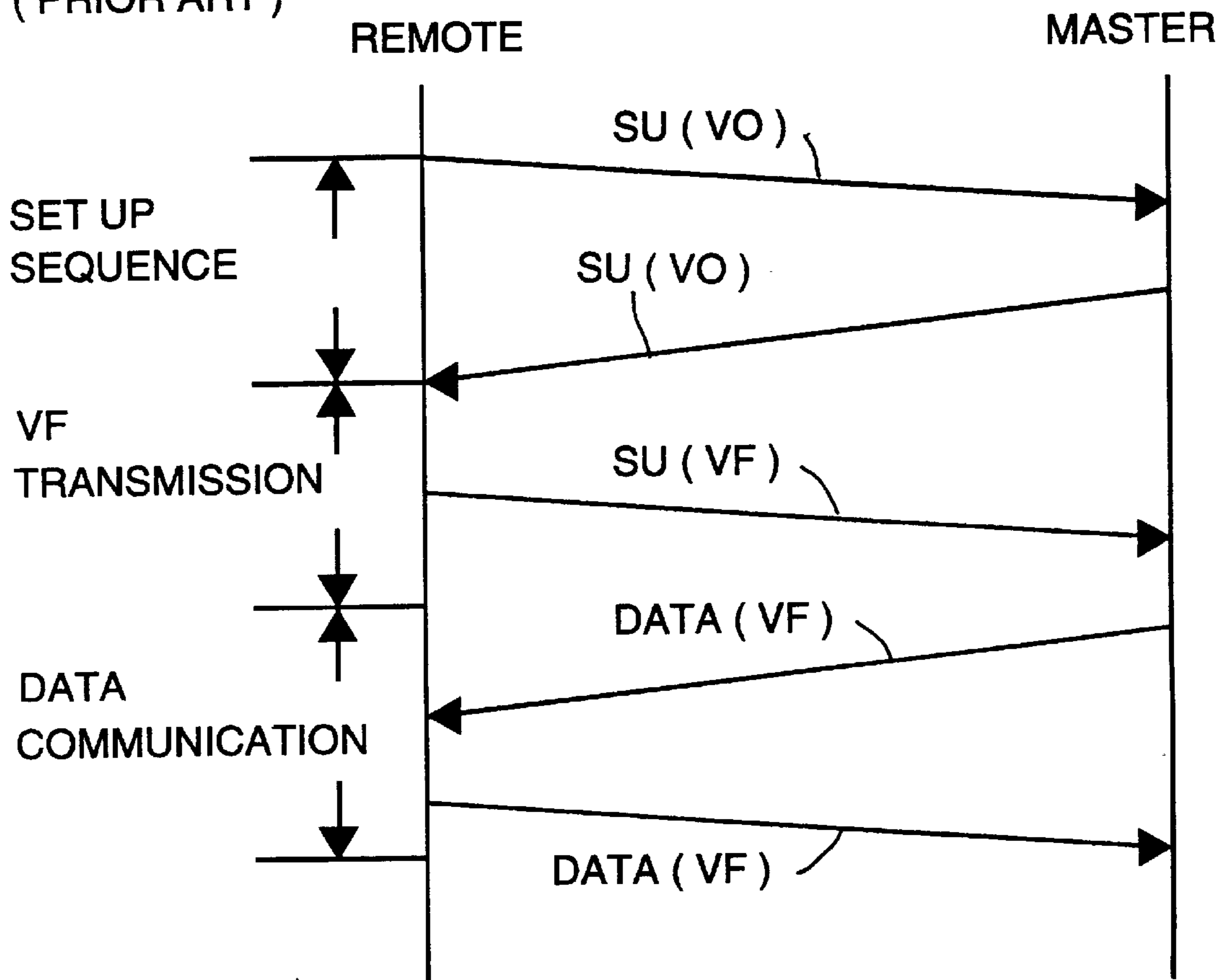
FIG. 4 (PRIOR ART)
