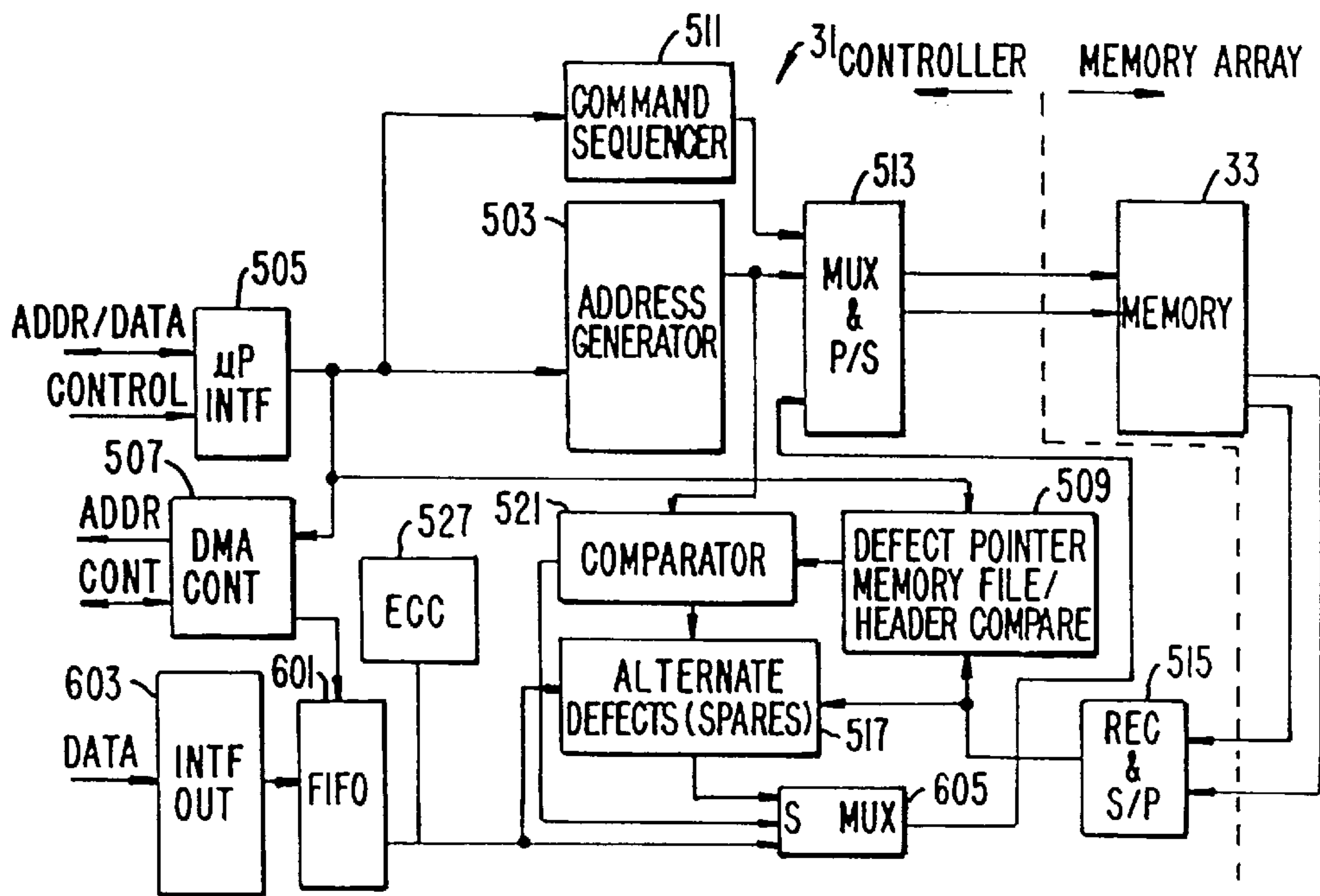
WRITE DATA PATH CONTROL FIG. 7.
