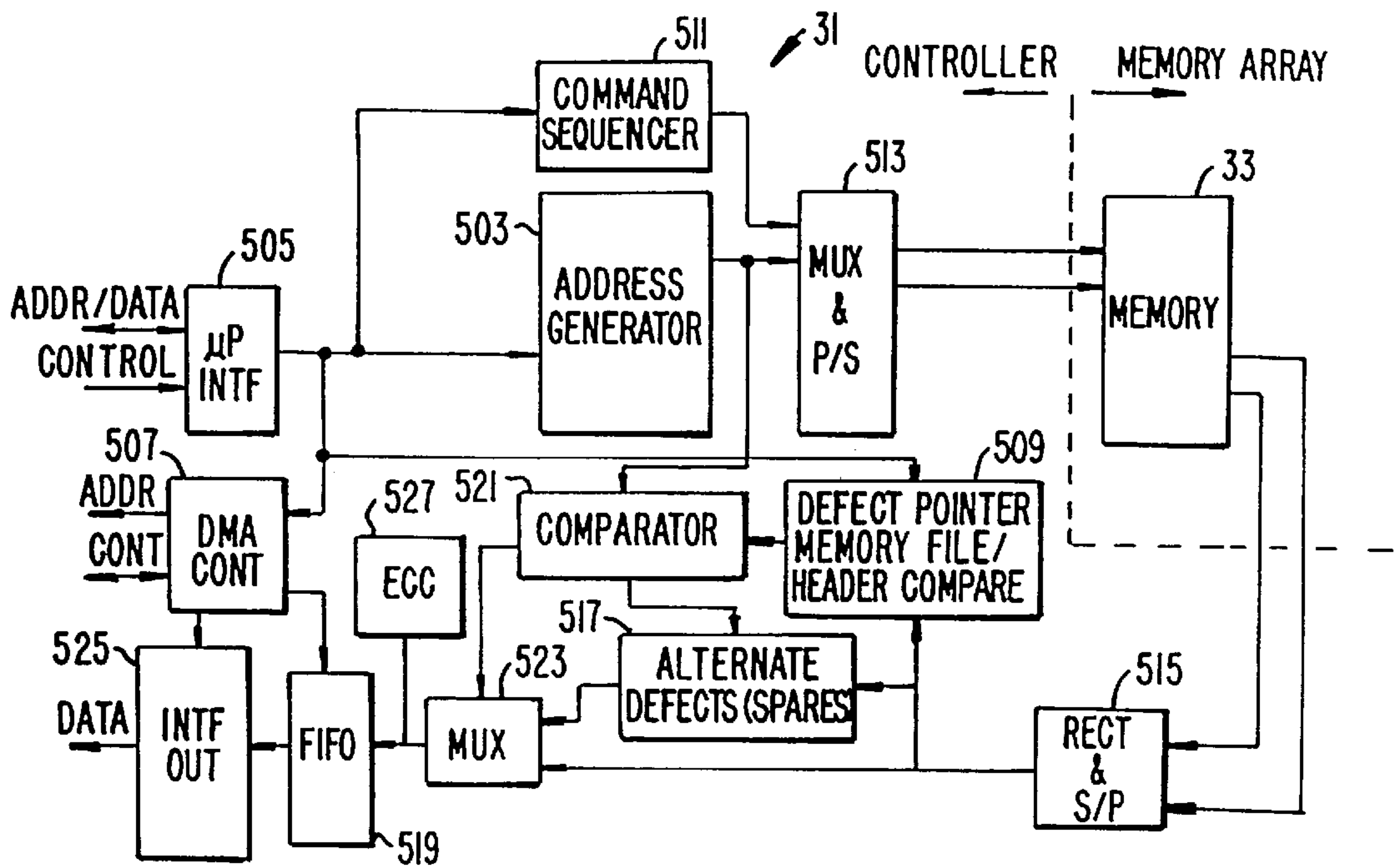
READ DATA PATH CONTROL FIG. 6.
