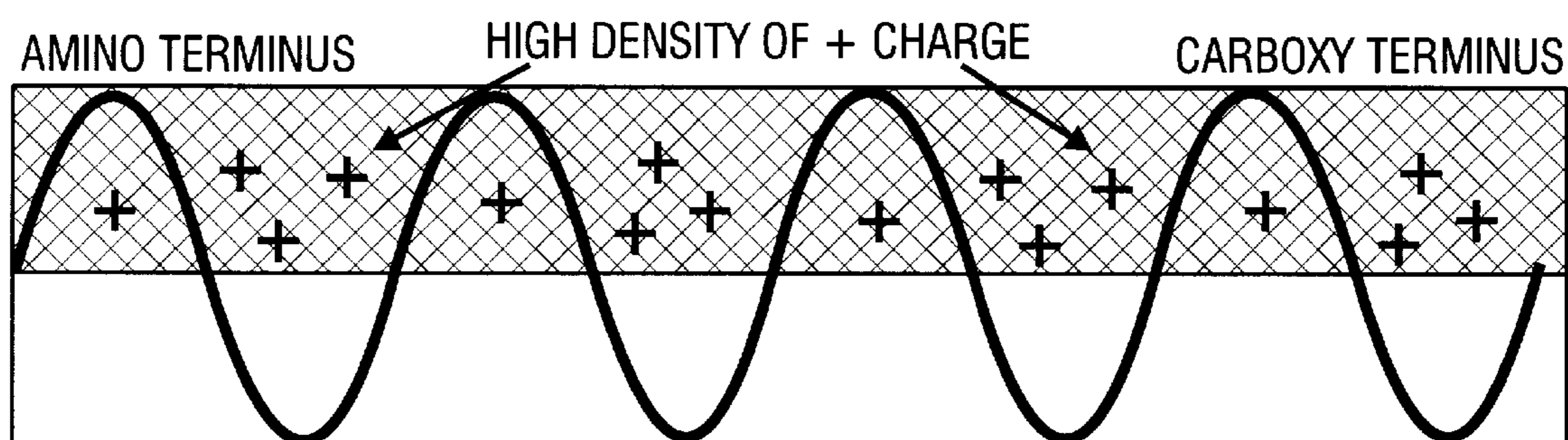
AMPHIPATHIC ALPHA HELIX Anubis Series
