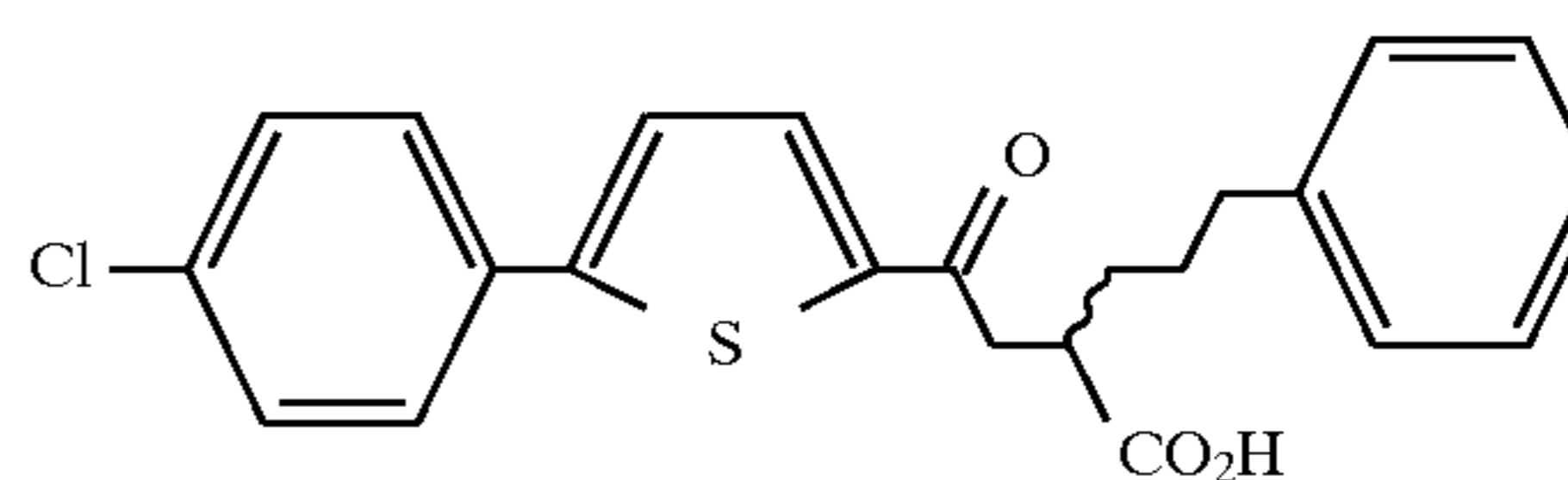
Example 250
