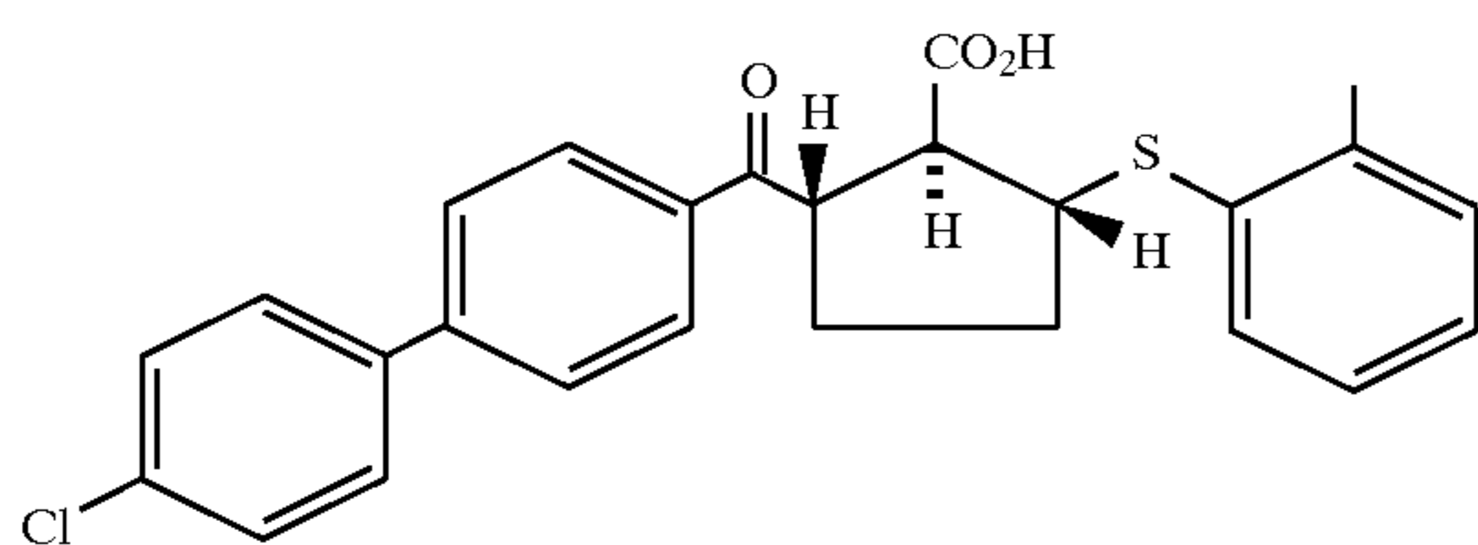
Example 216 (racemate)
