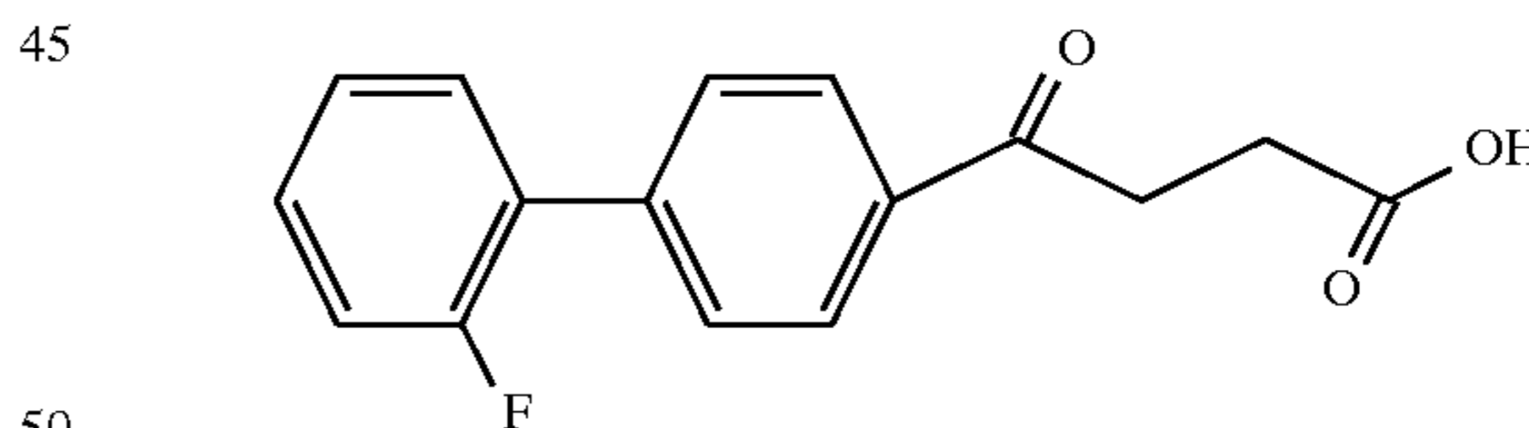
Example 9
