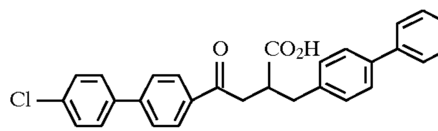
Example 110
