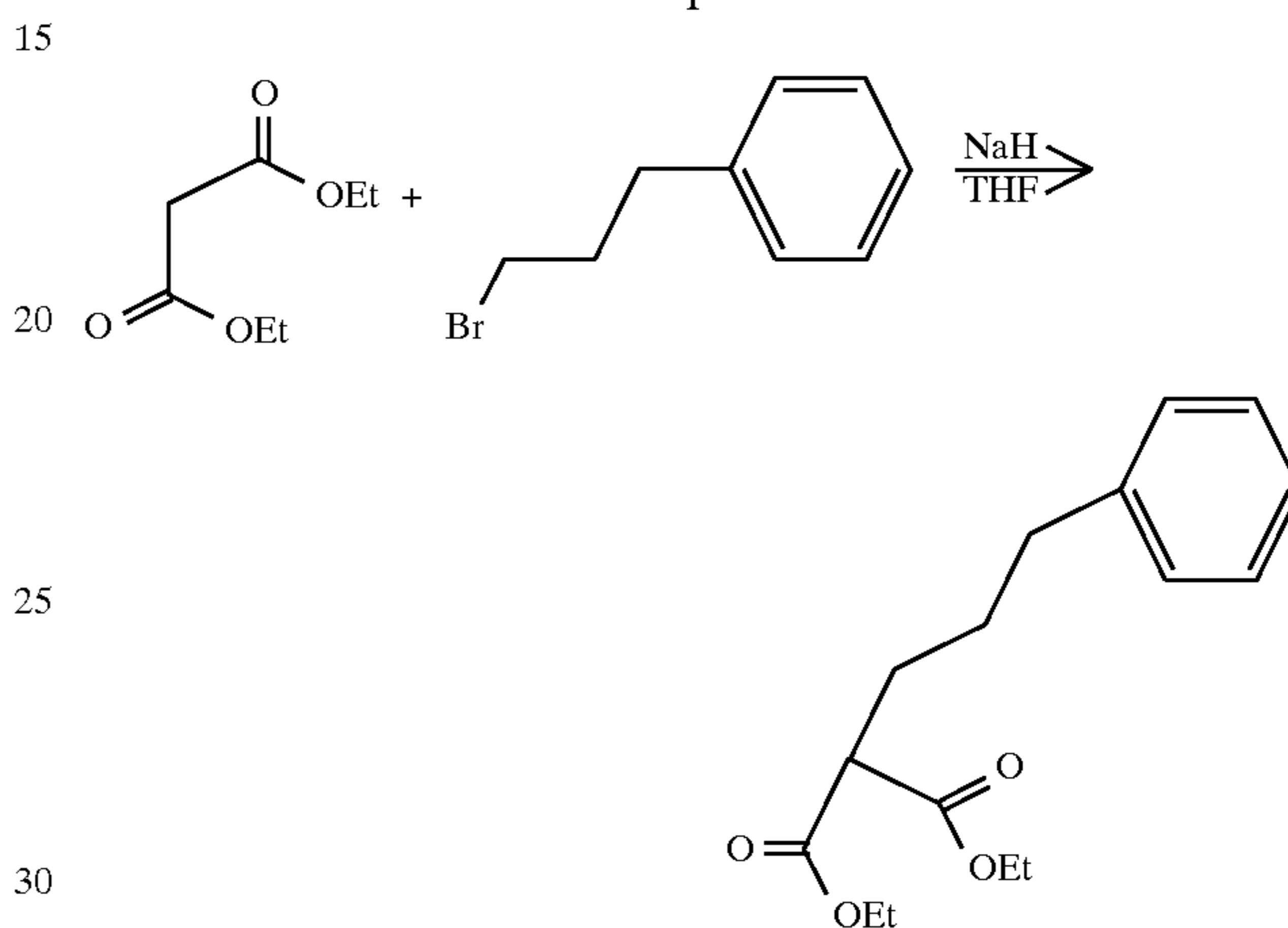
Example 87
