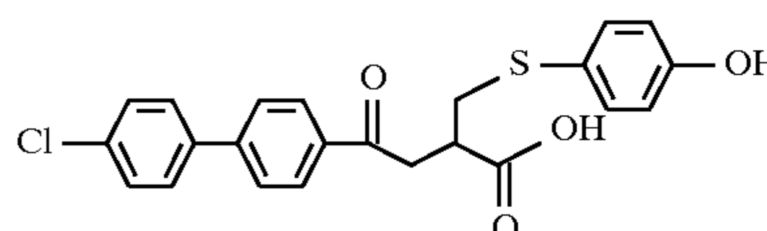
Example 134
