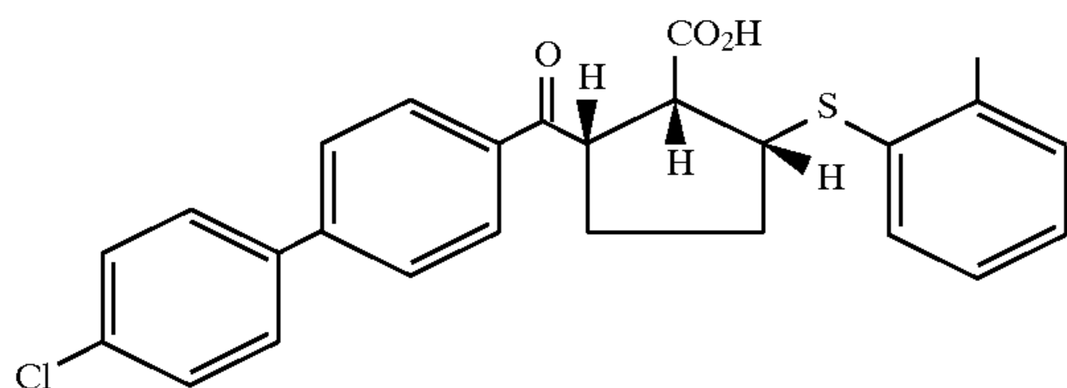
Example 217 (racemate)
