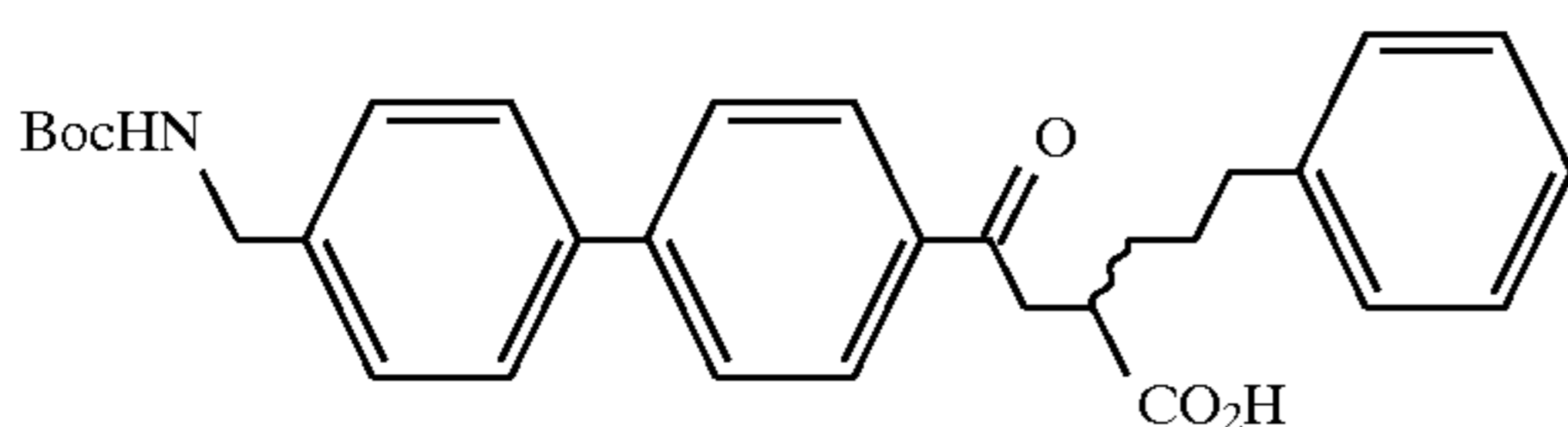
Example 49
