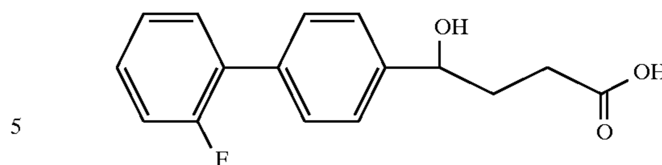
Example 39
