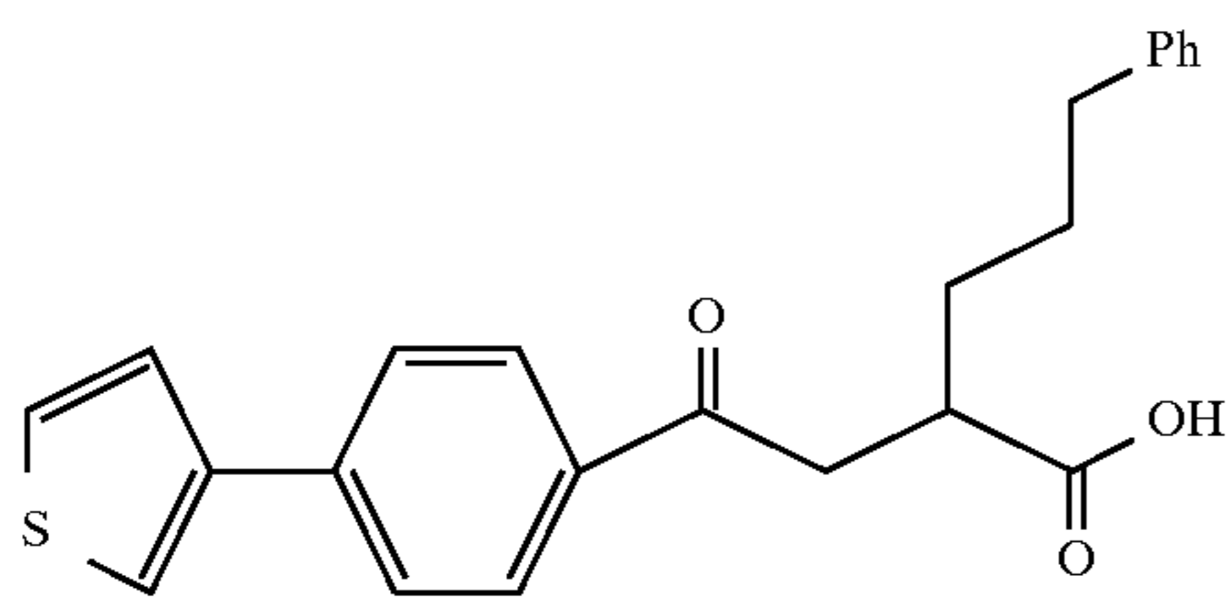
Example 72
