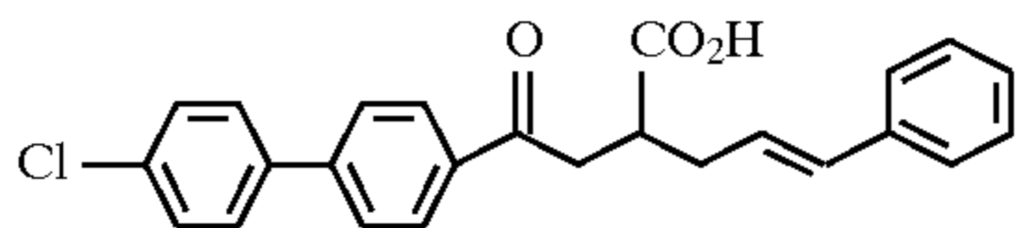
Example 111
