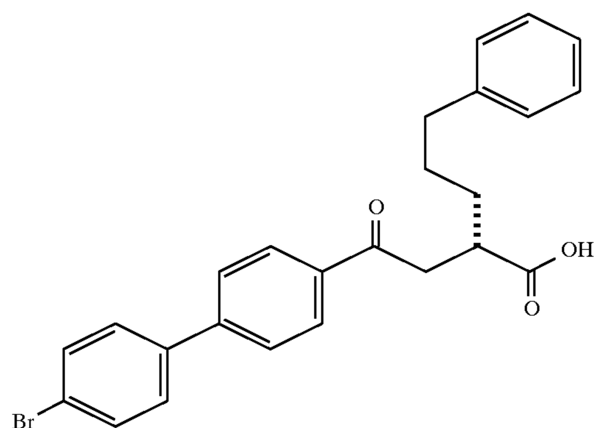
Example 90
