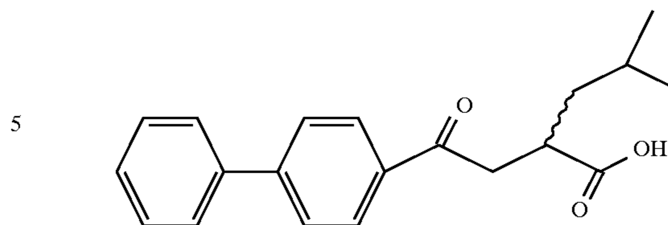
Example 13
