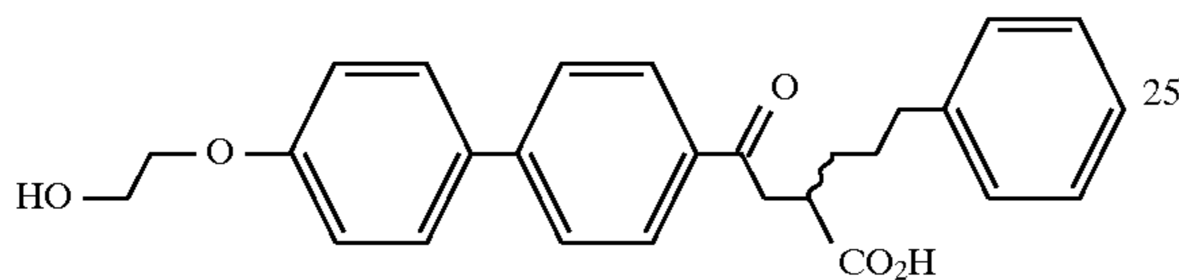
Example 54
