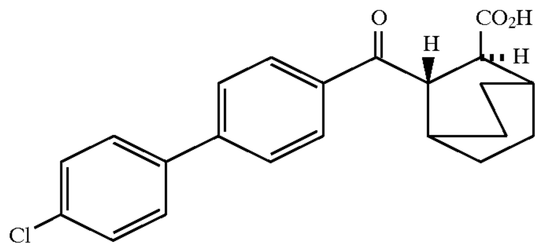
Example 232 (racemate)
