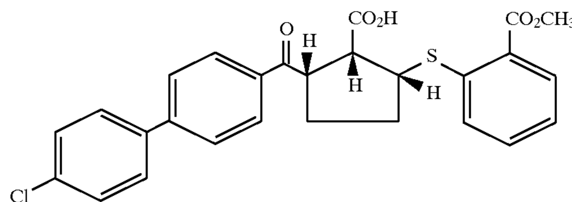
Example 220 (racemate)
