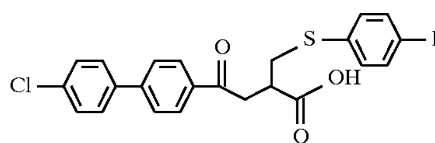
Example 138
