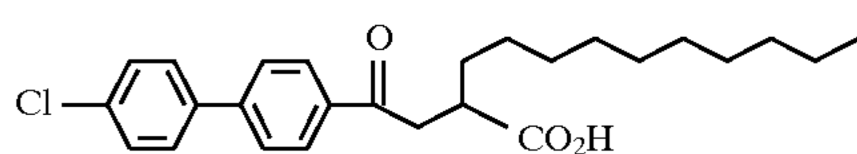
Example 98
