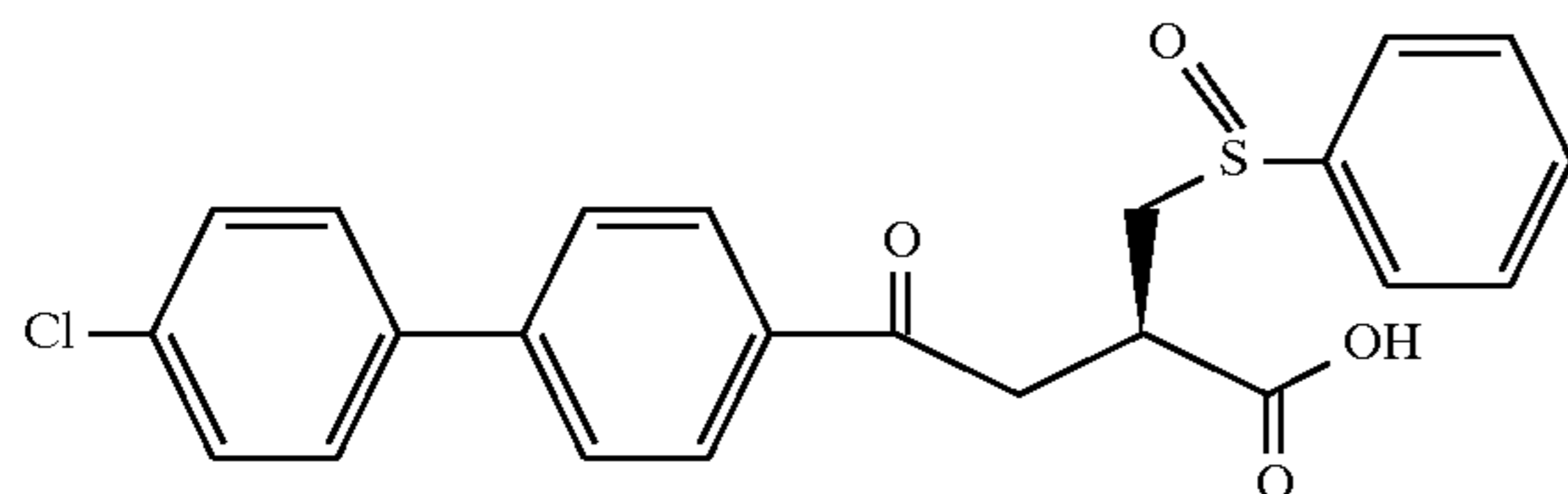
Example 126
