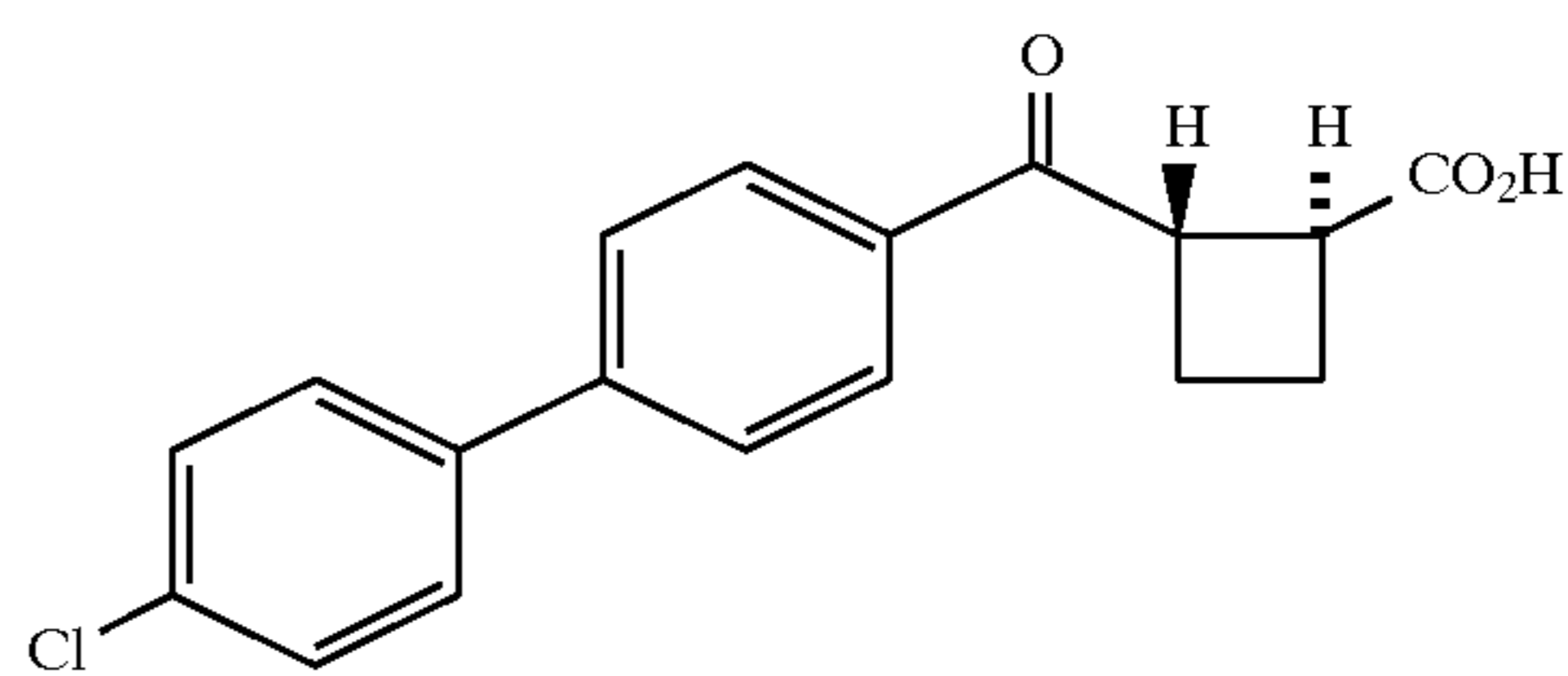
Example 206 (racemate)
