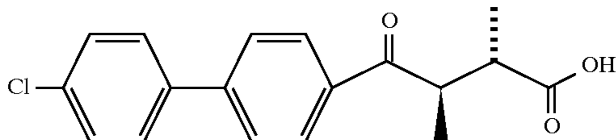
Example 199 (racemate)
