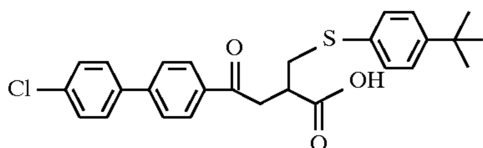
Example 143
