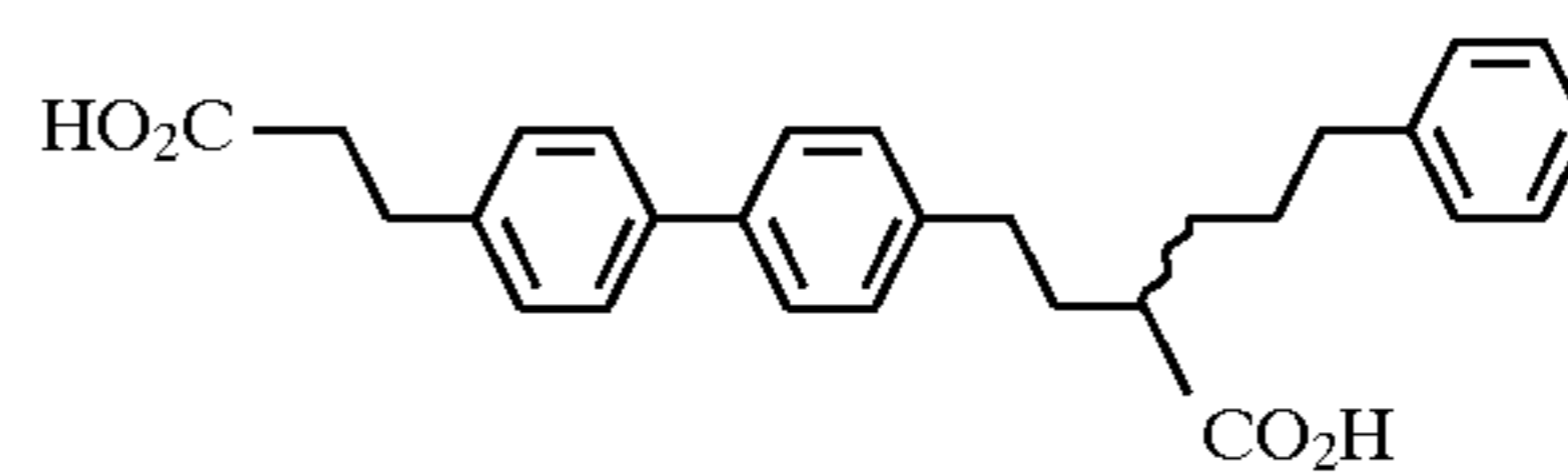
Example 45
