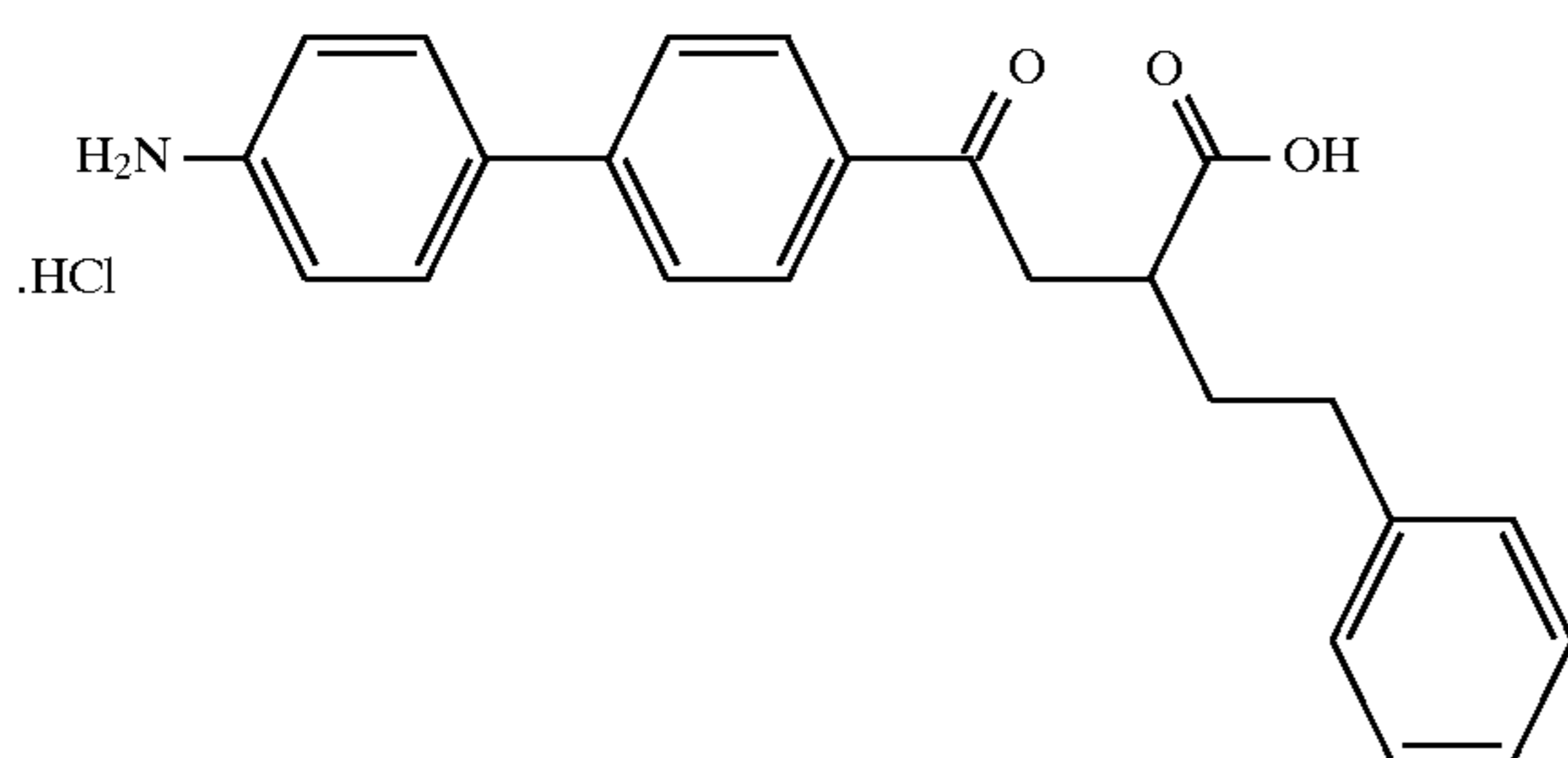
Example 100
