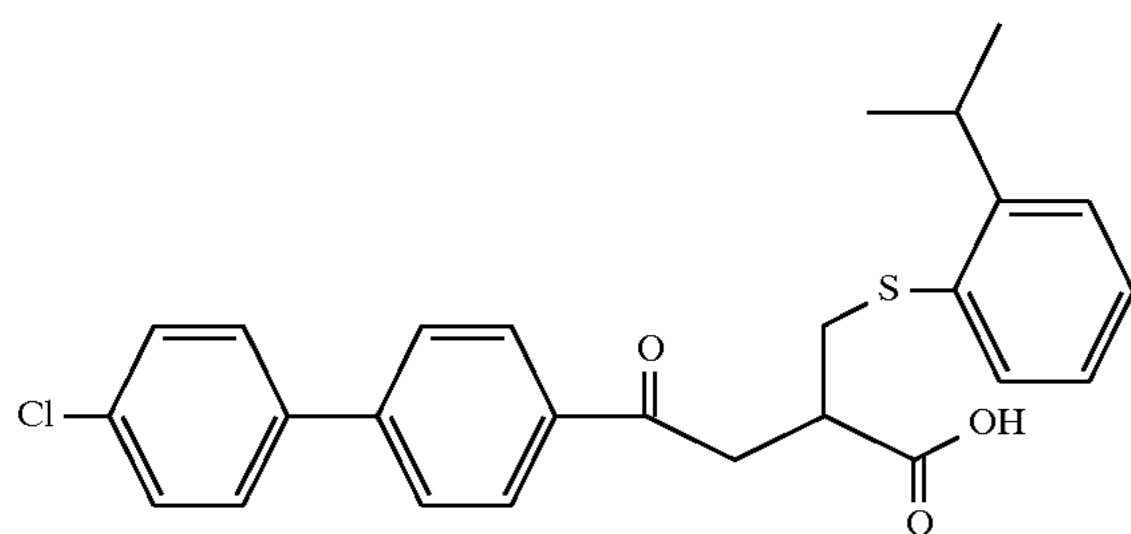
Example 151
