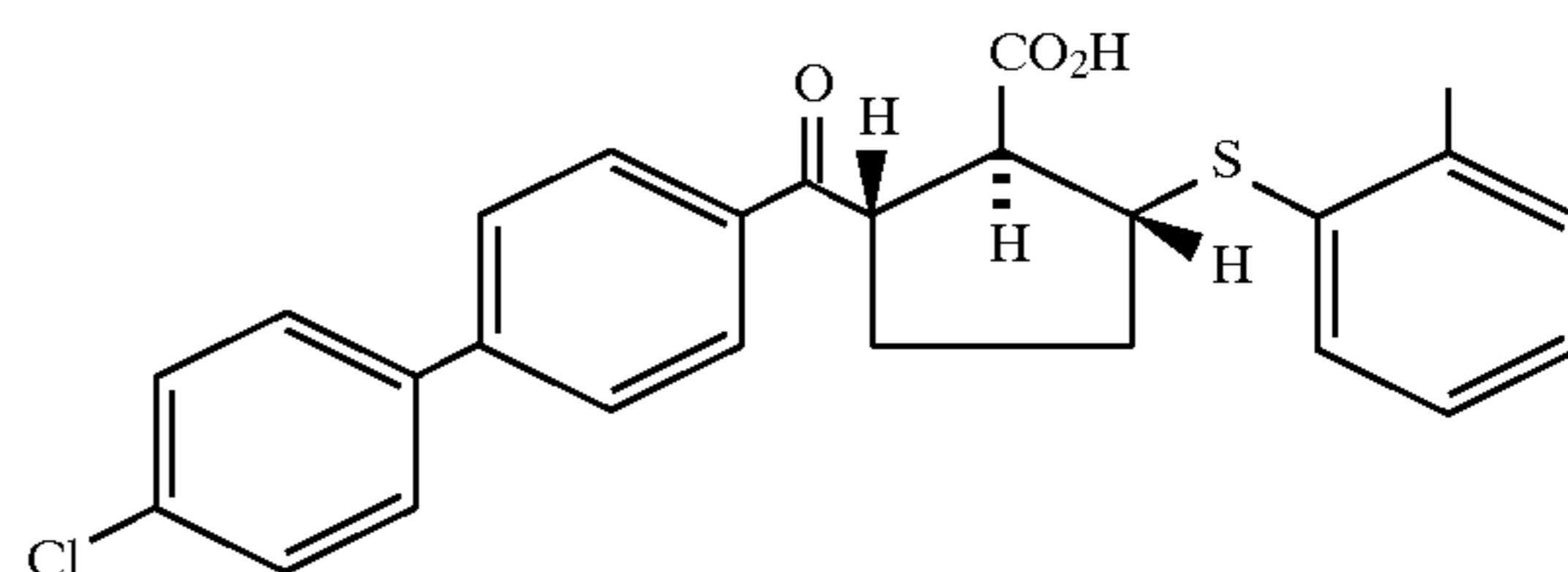
Example 219 (racemate)
