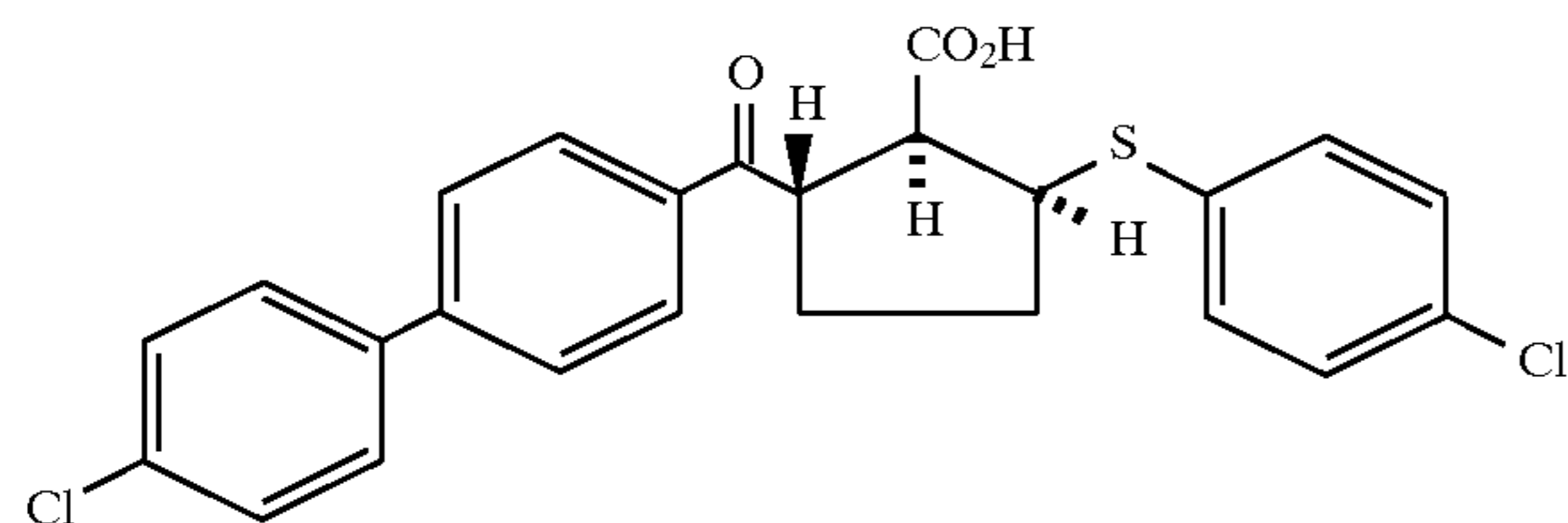
Example 223 (racemate)
