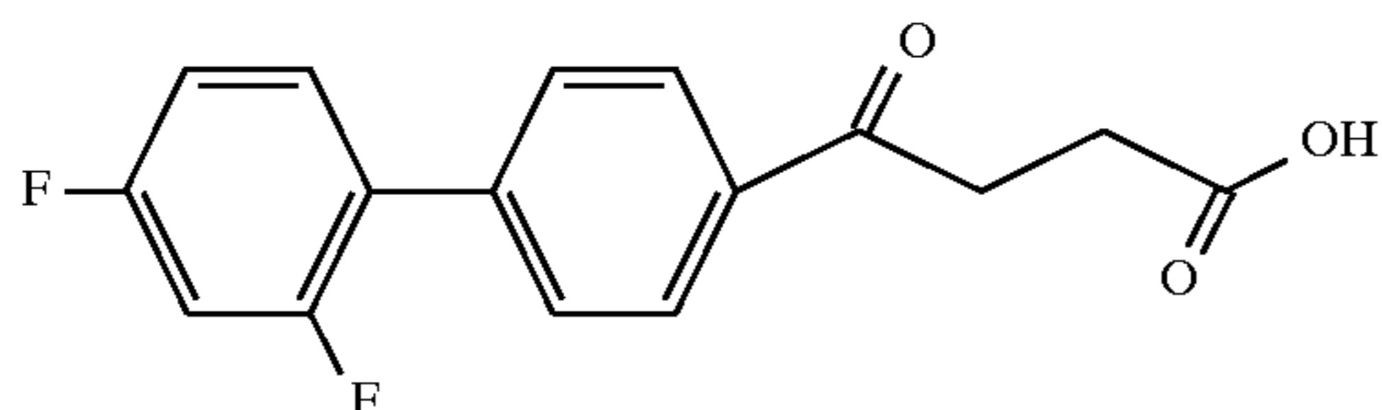
Example 11
