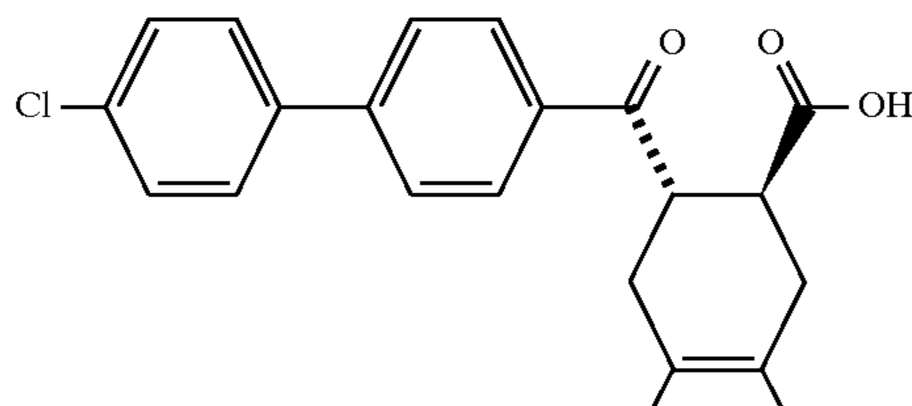
Example 228 (racemate)
