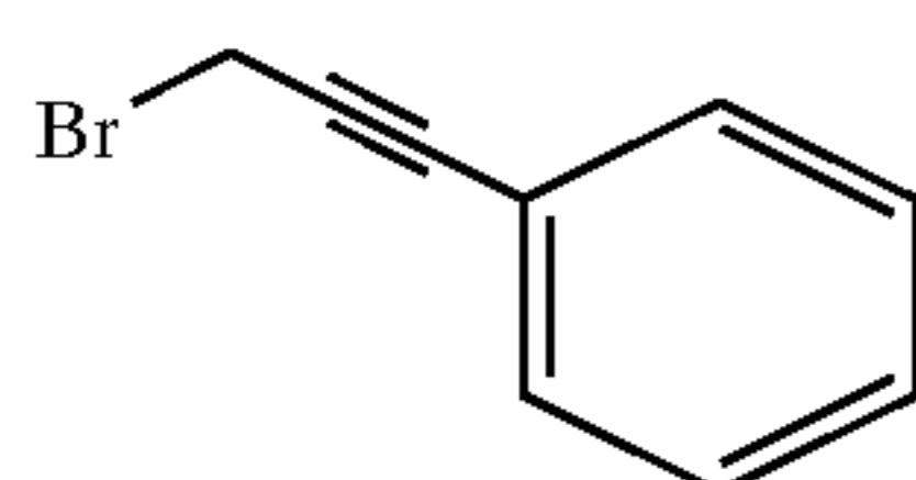
1-phenyl-3-bromo-1-propyn
