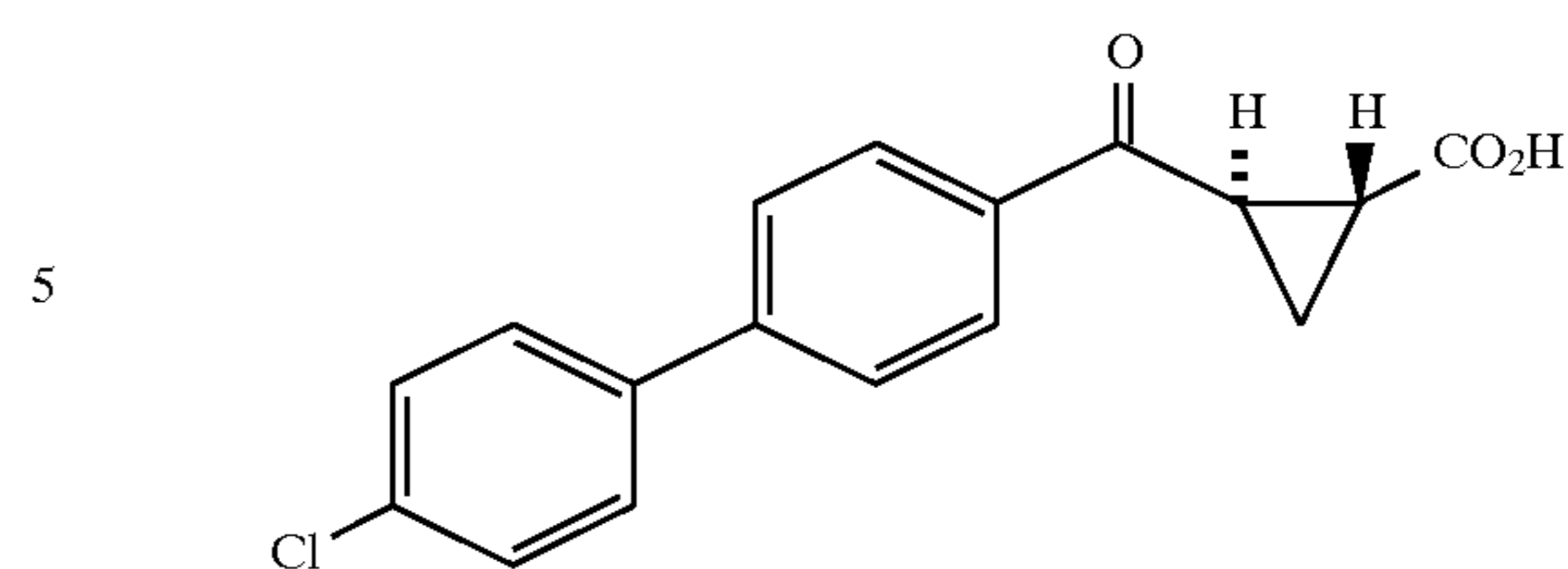
Example 208 (racemate)
