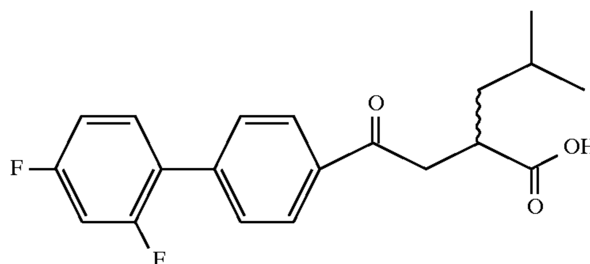
Example 20
