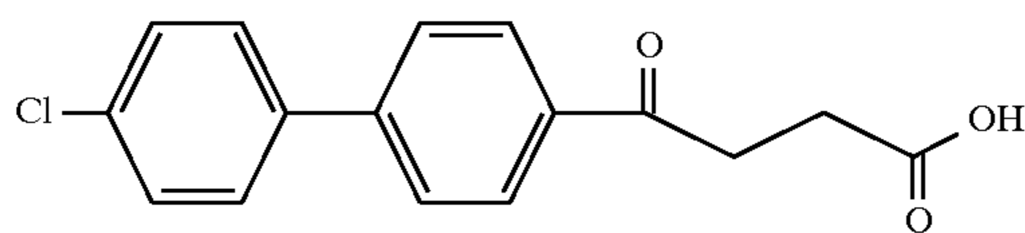
Example 6
