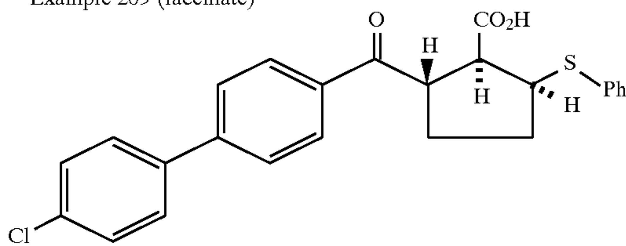
Example 210 (racemate)
