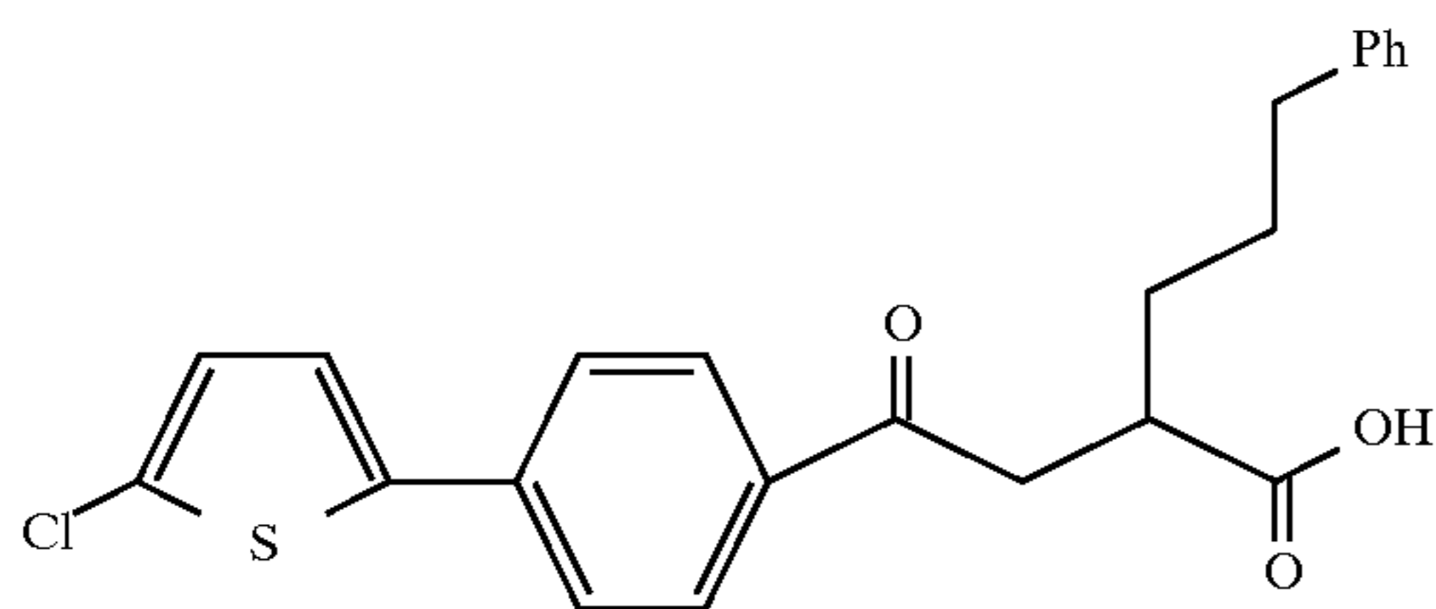
Example 68
