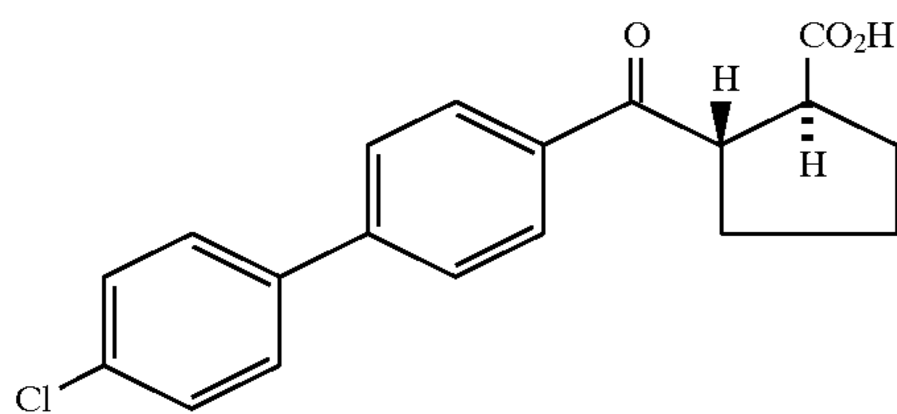
Example 204 (racemate)
