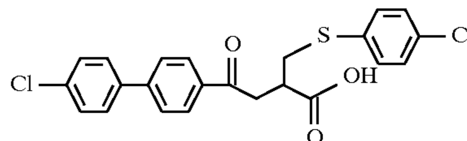
Example 139
