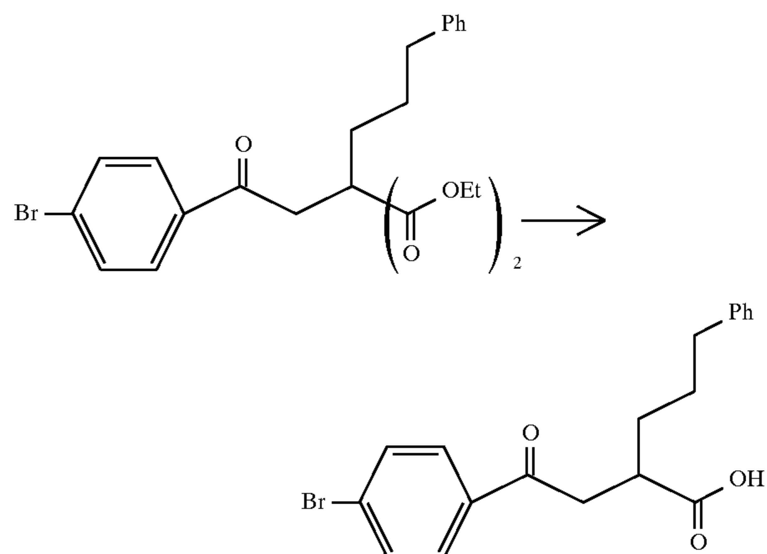
Example 65
