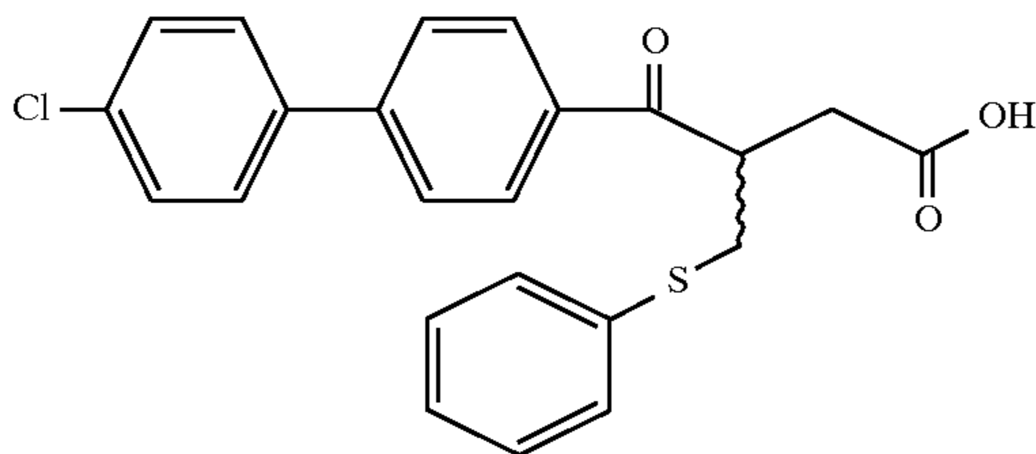
Example 181
