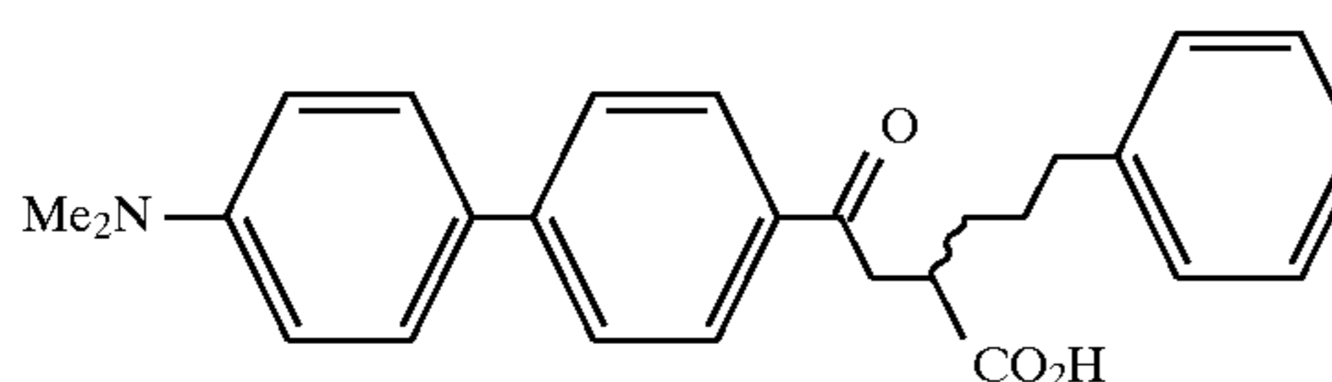
Example 60
