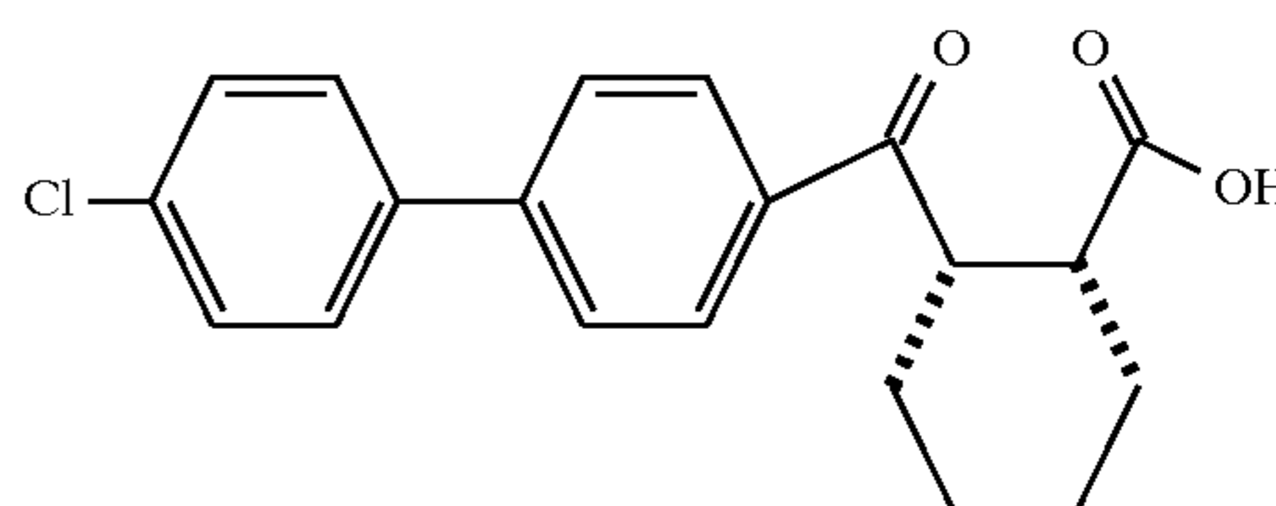
Example 201 (racemate)
