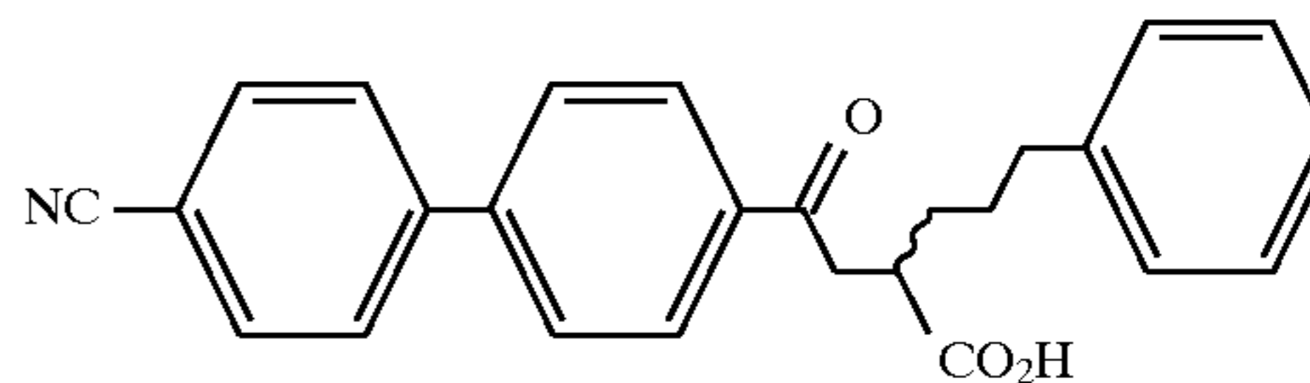
Example 56
