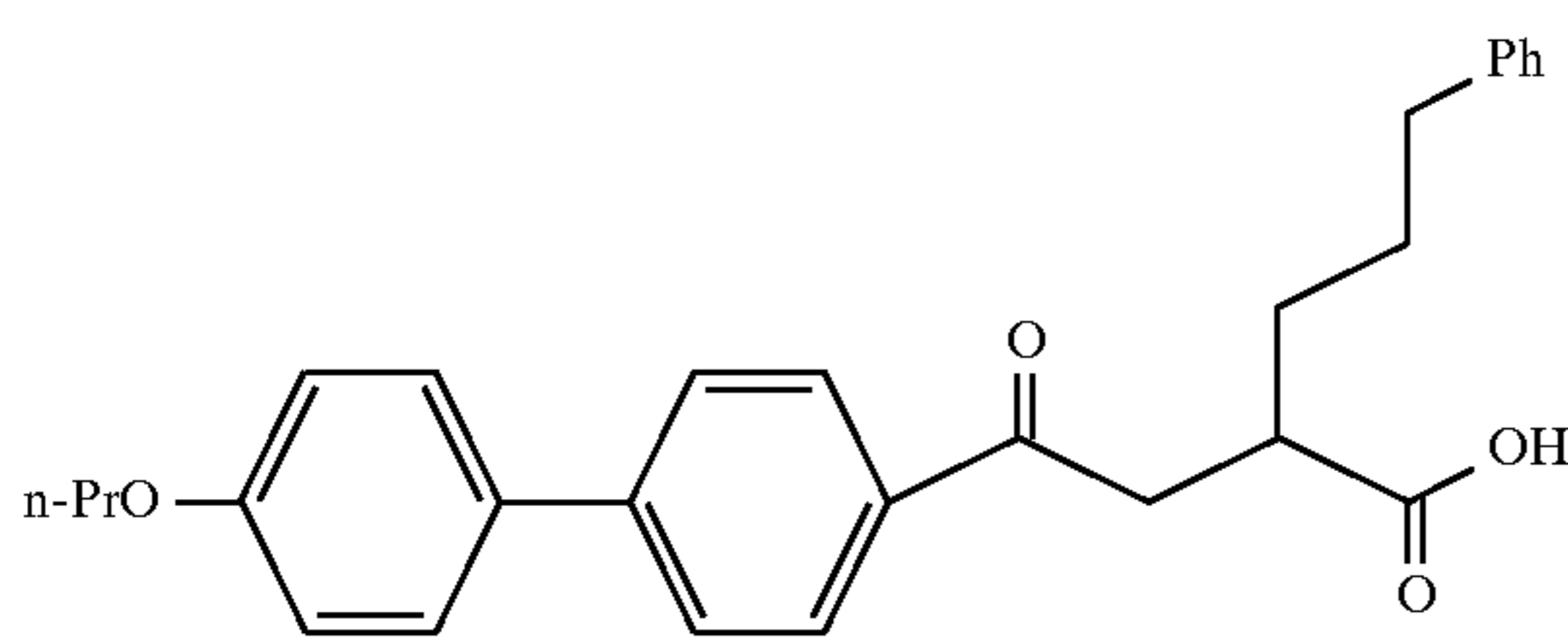
Example 80
