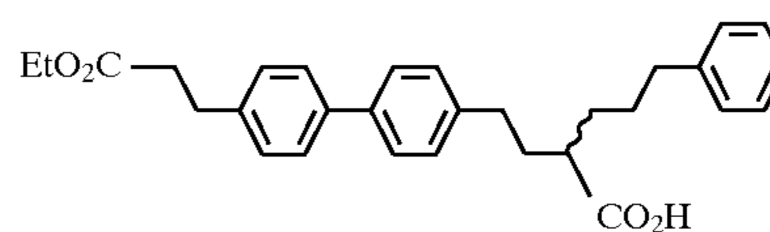
Example 44
