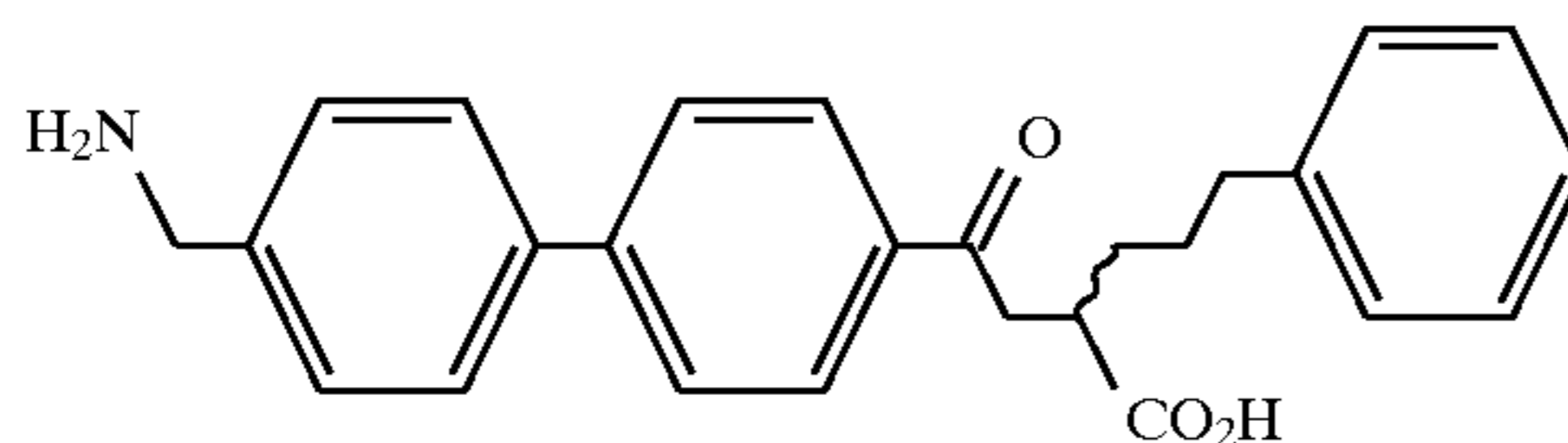
Example 59
