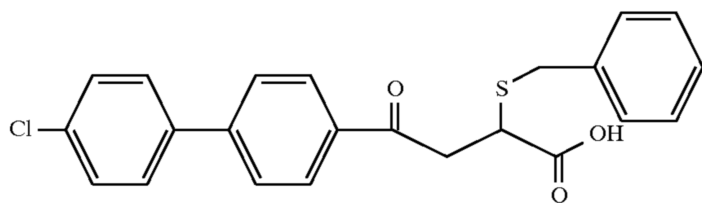
Example 177
