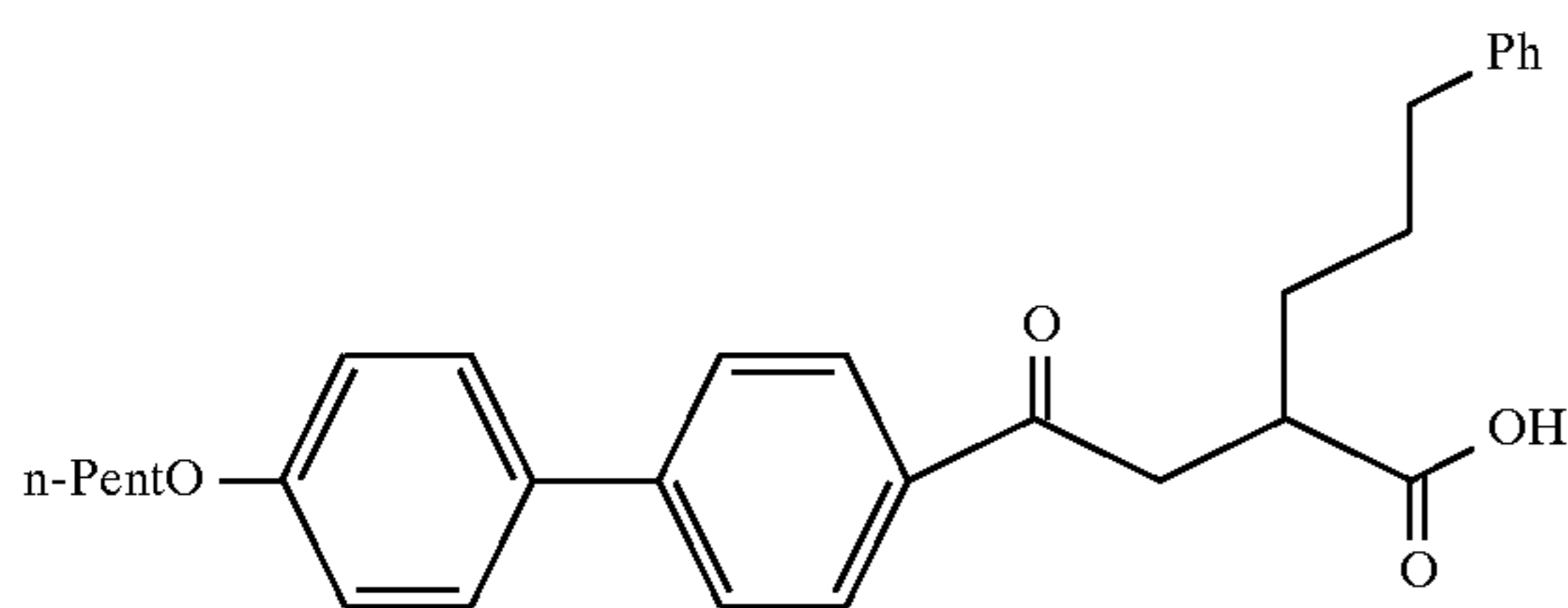
Example 81
