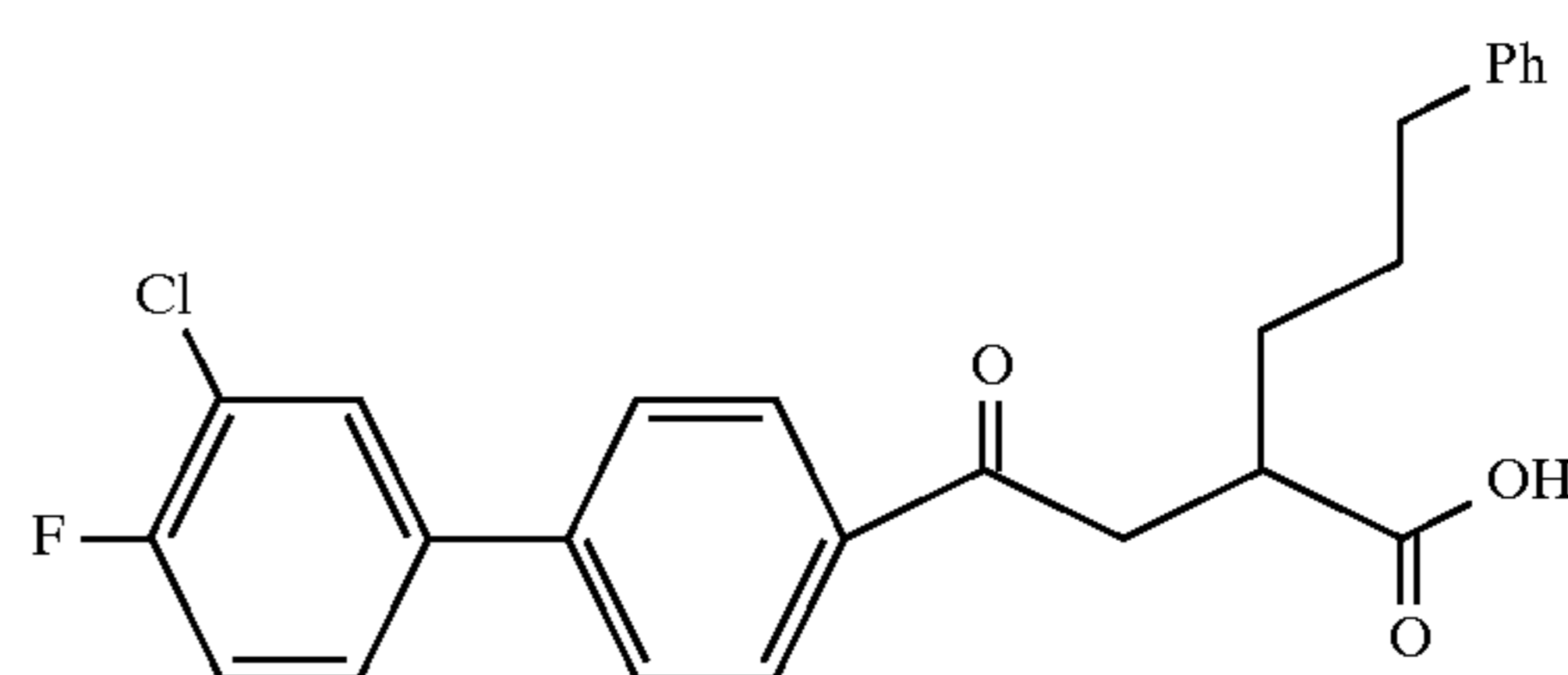
Example 70
