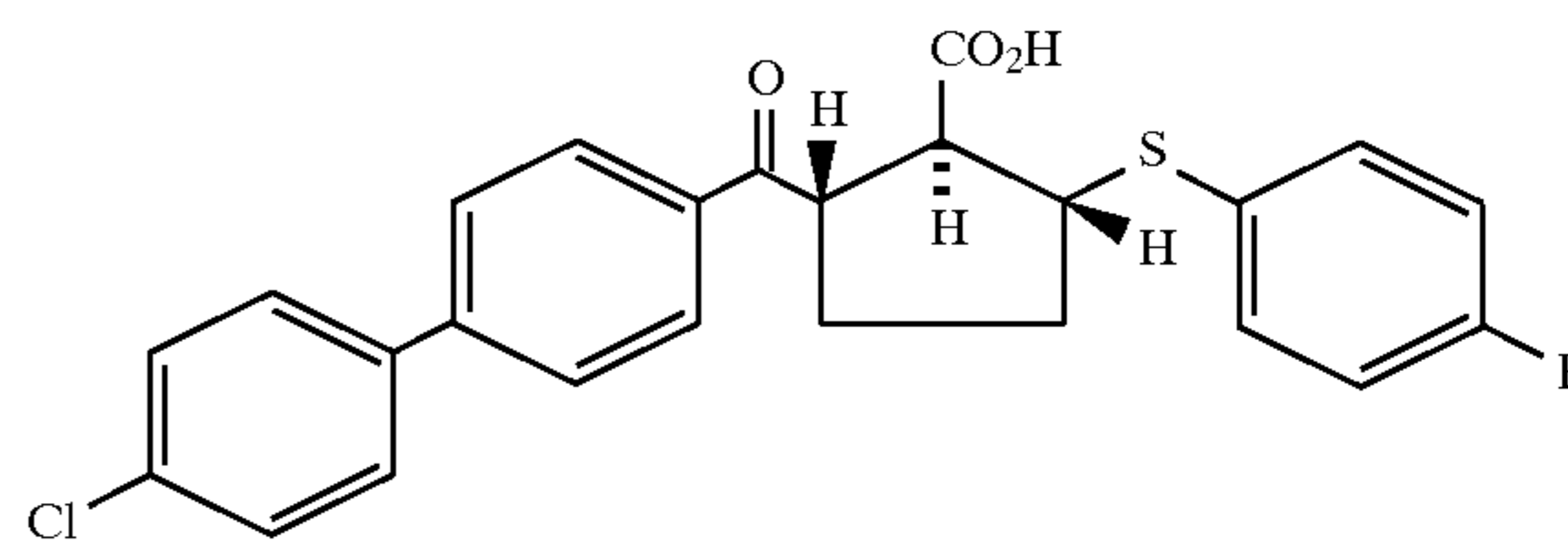
Example 213 (racemate)
