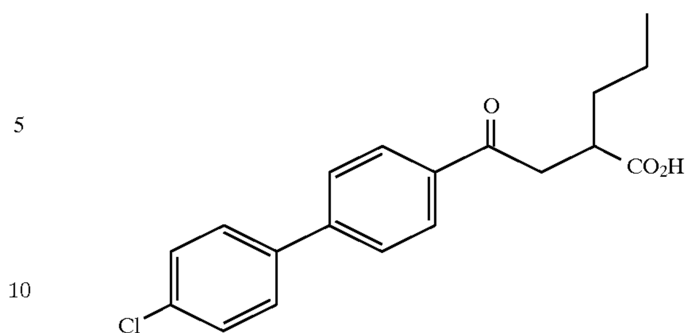
Example 93
