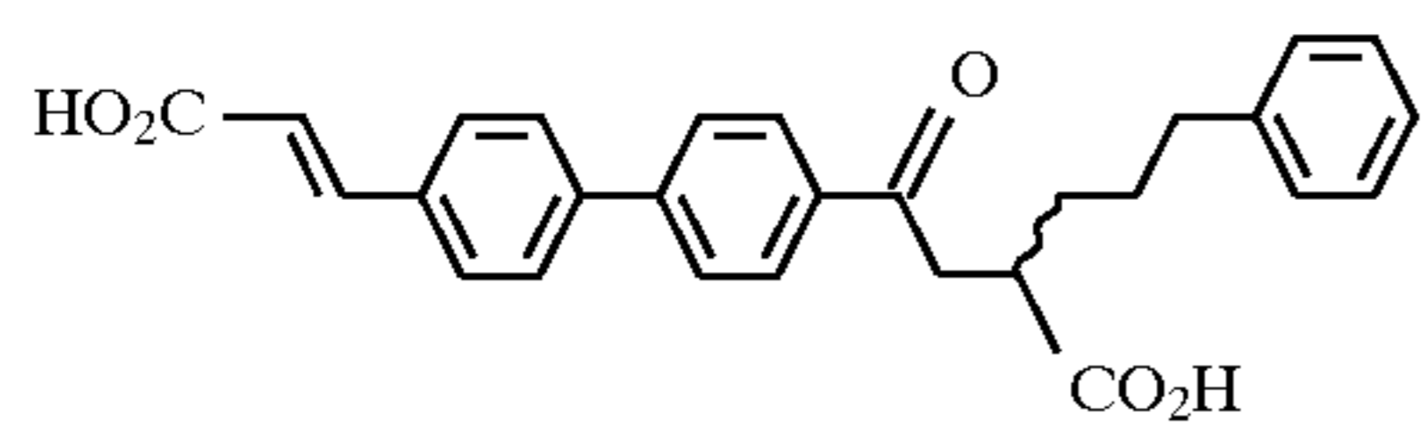
Example 43
