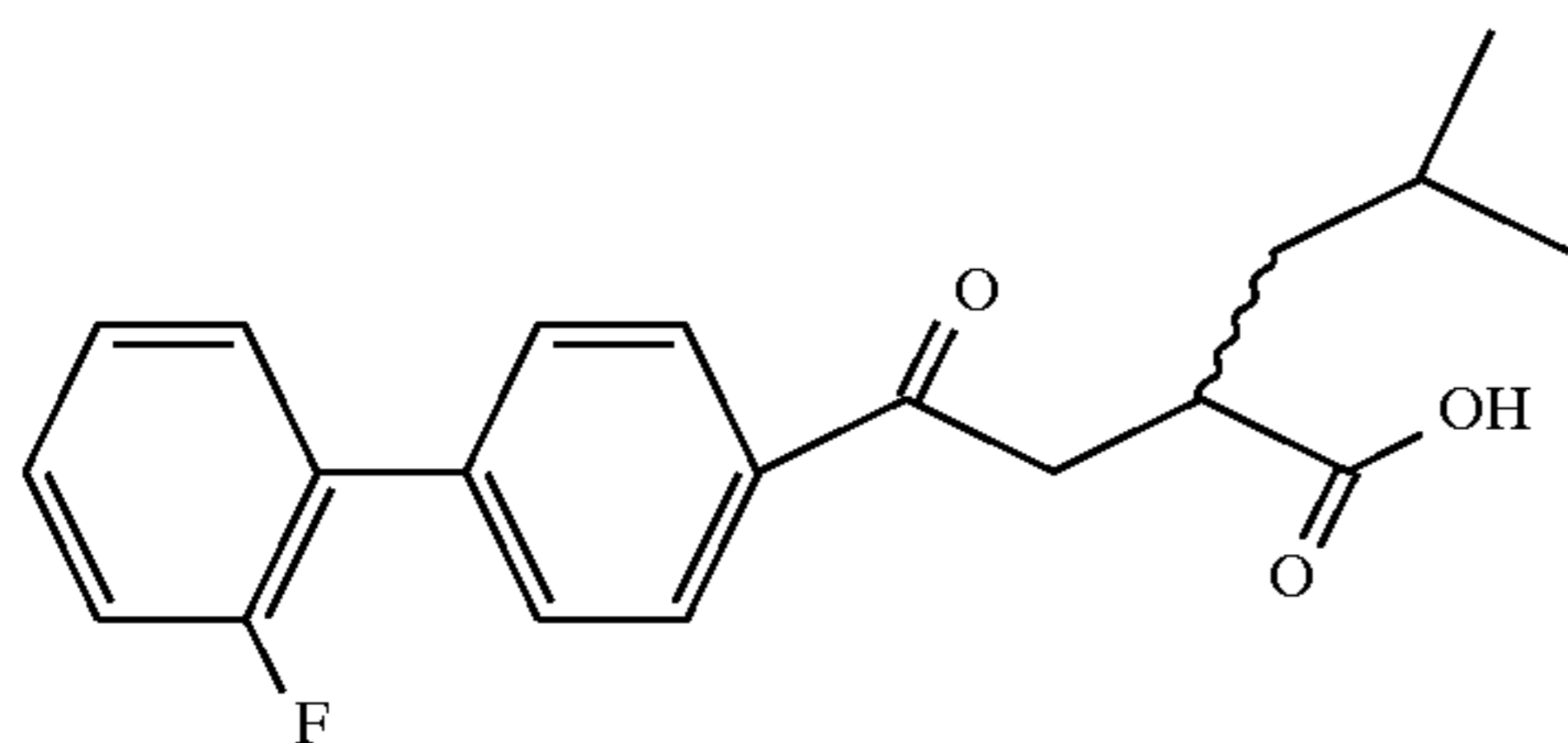
Example 17
