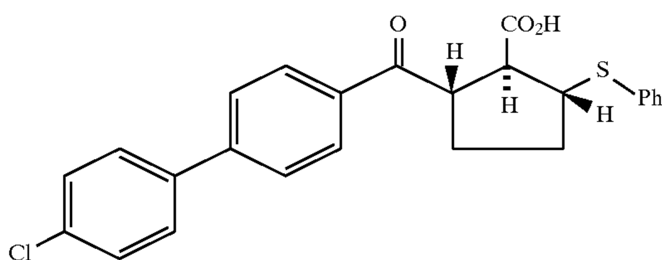
Example 209 (racemate)
