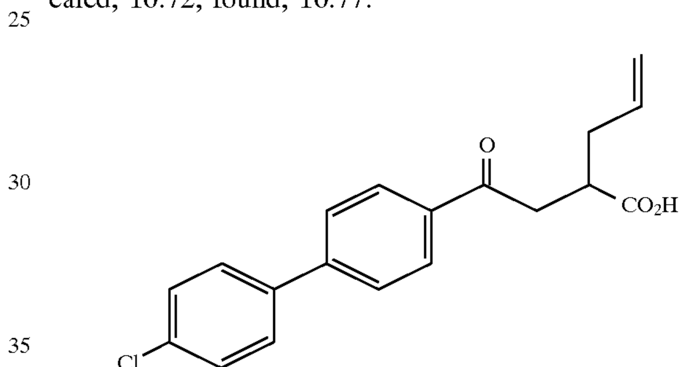
Example 94
