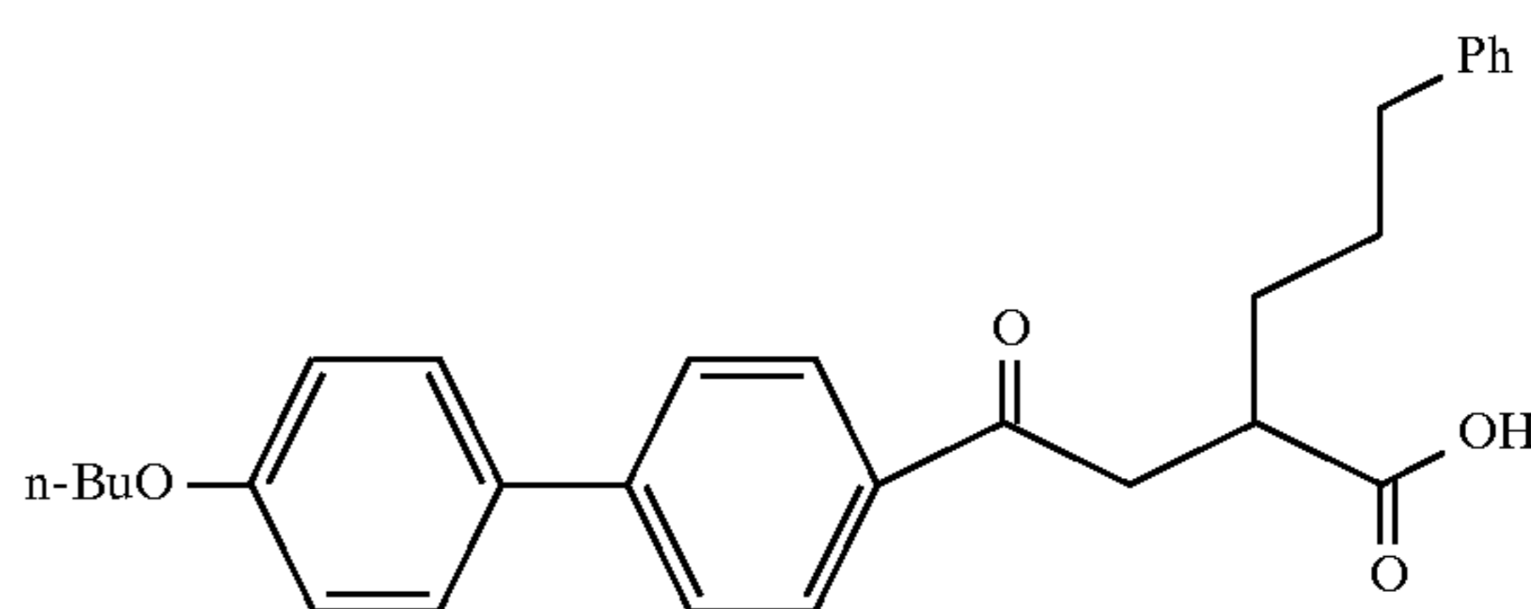
Example 83
