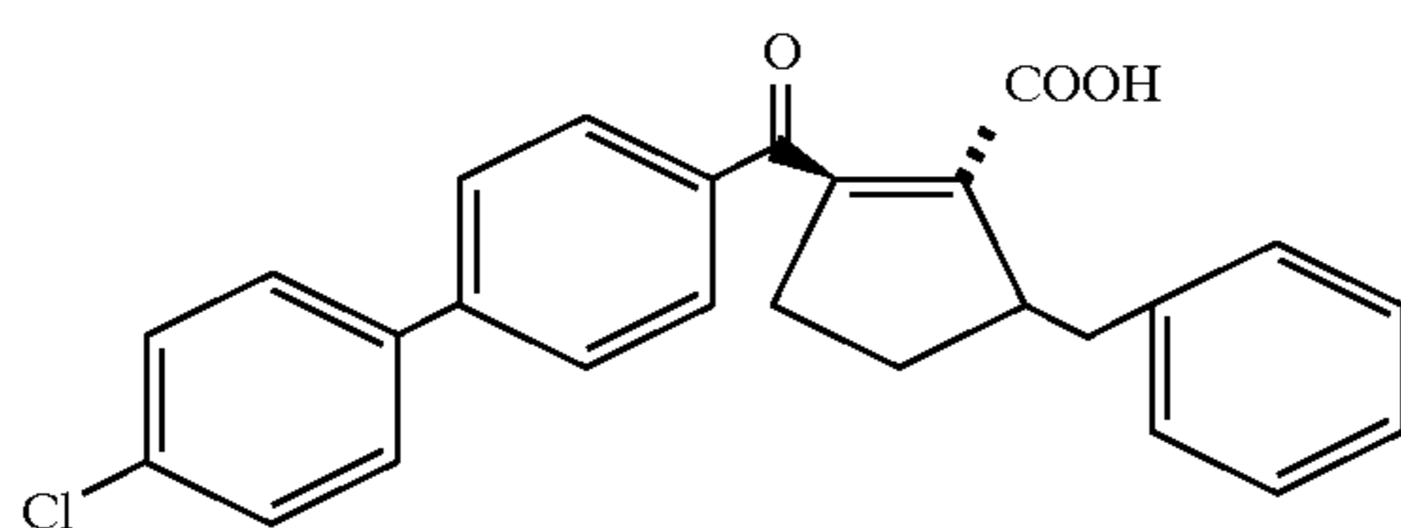
Example 227 (racemate)
