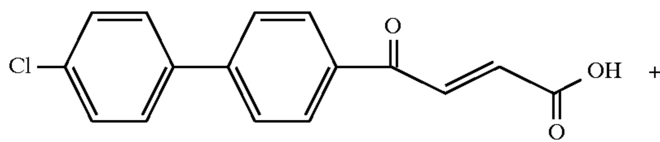
Example 34
