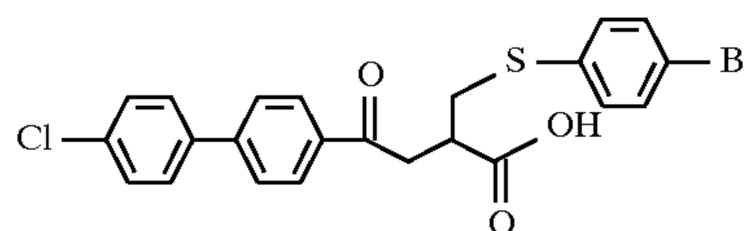
Example 140
