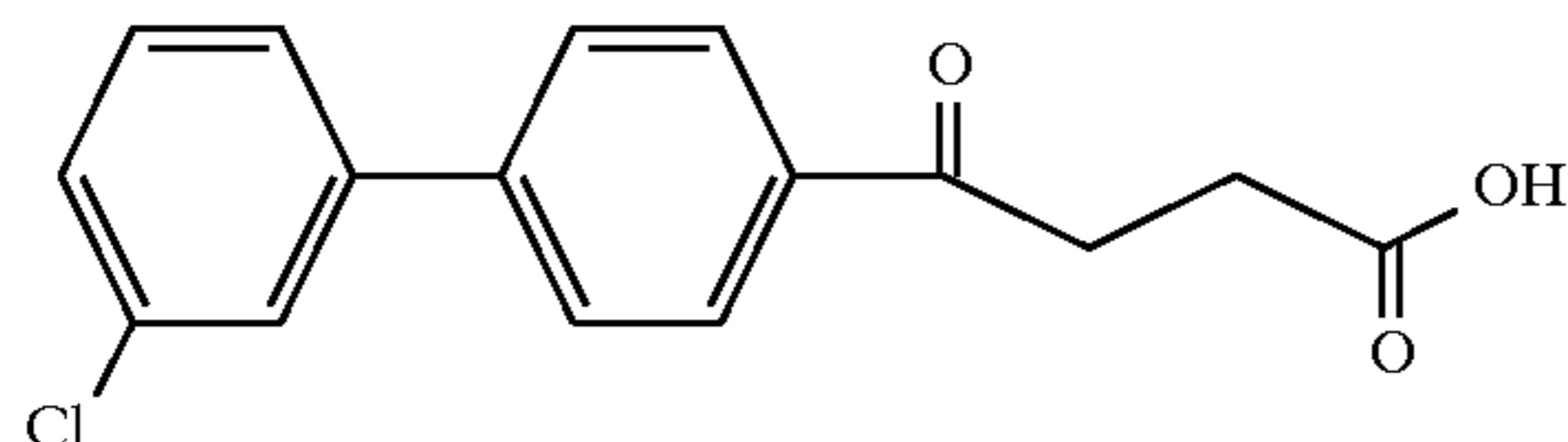
Example 12
