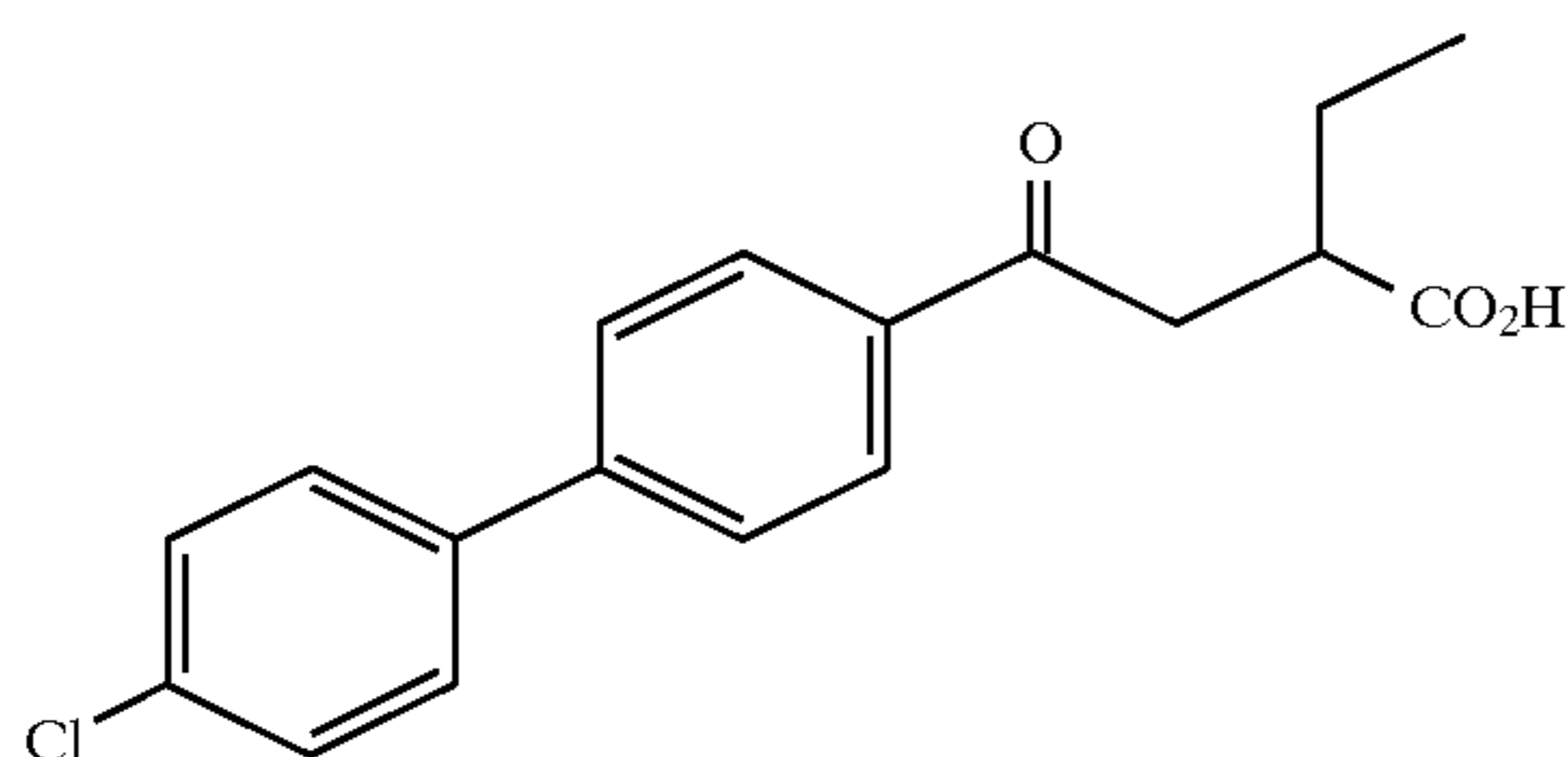
Example 92
