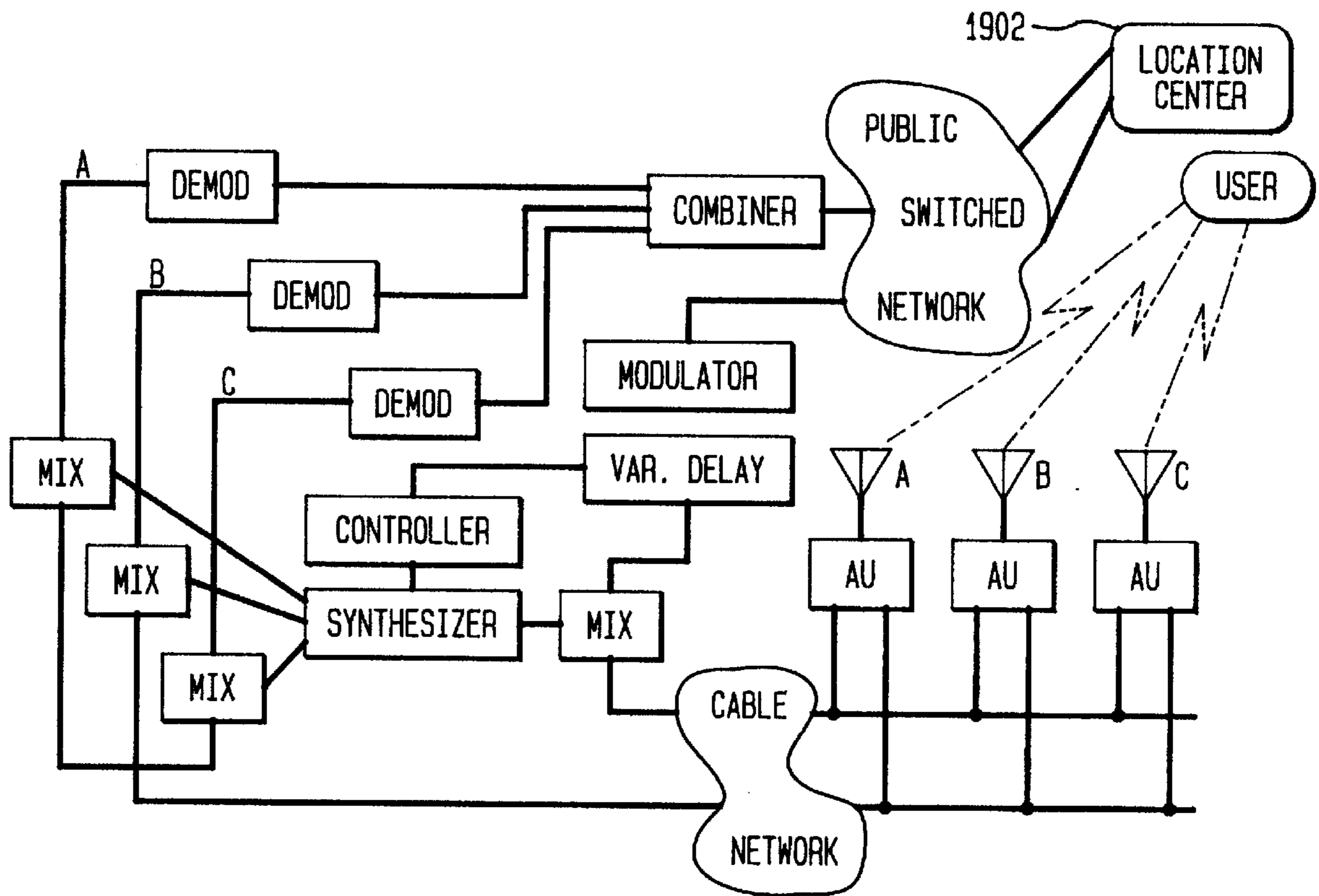
LOCATION CENTER EXTERNAL TO COMMUNICATION SYSTEM
