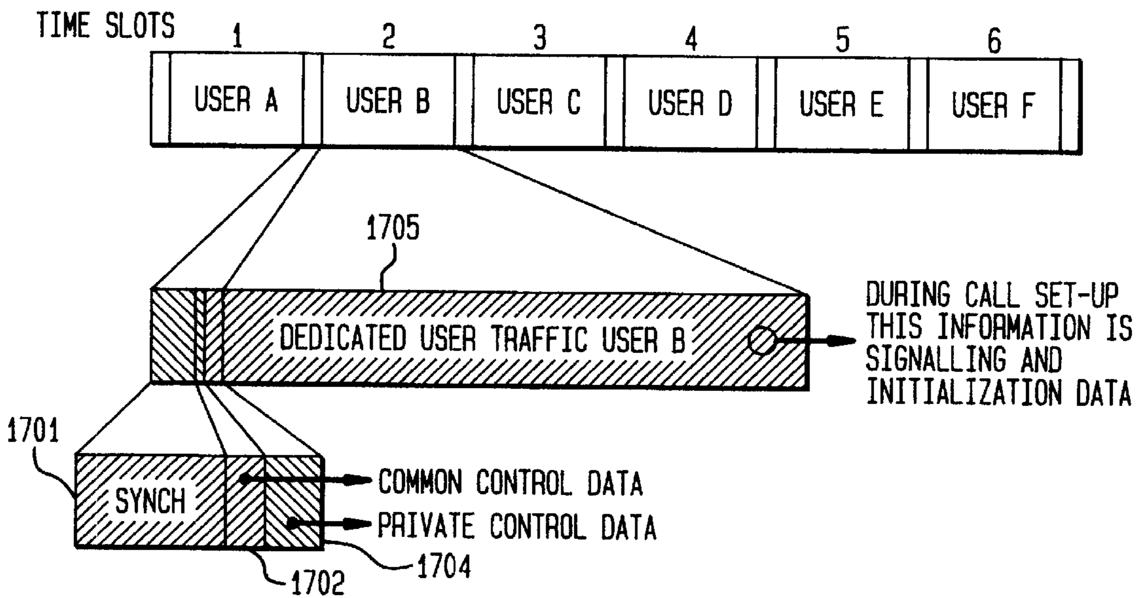
SYNCH AND CONTROL CHANNEL STRUCTURE
