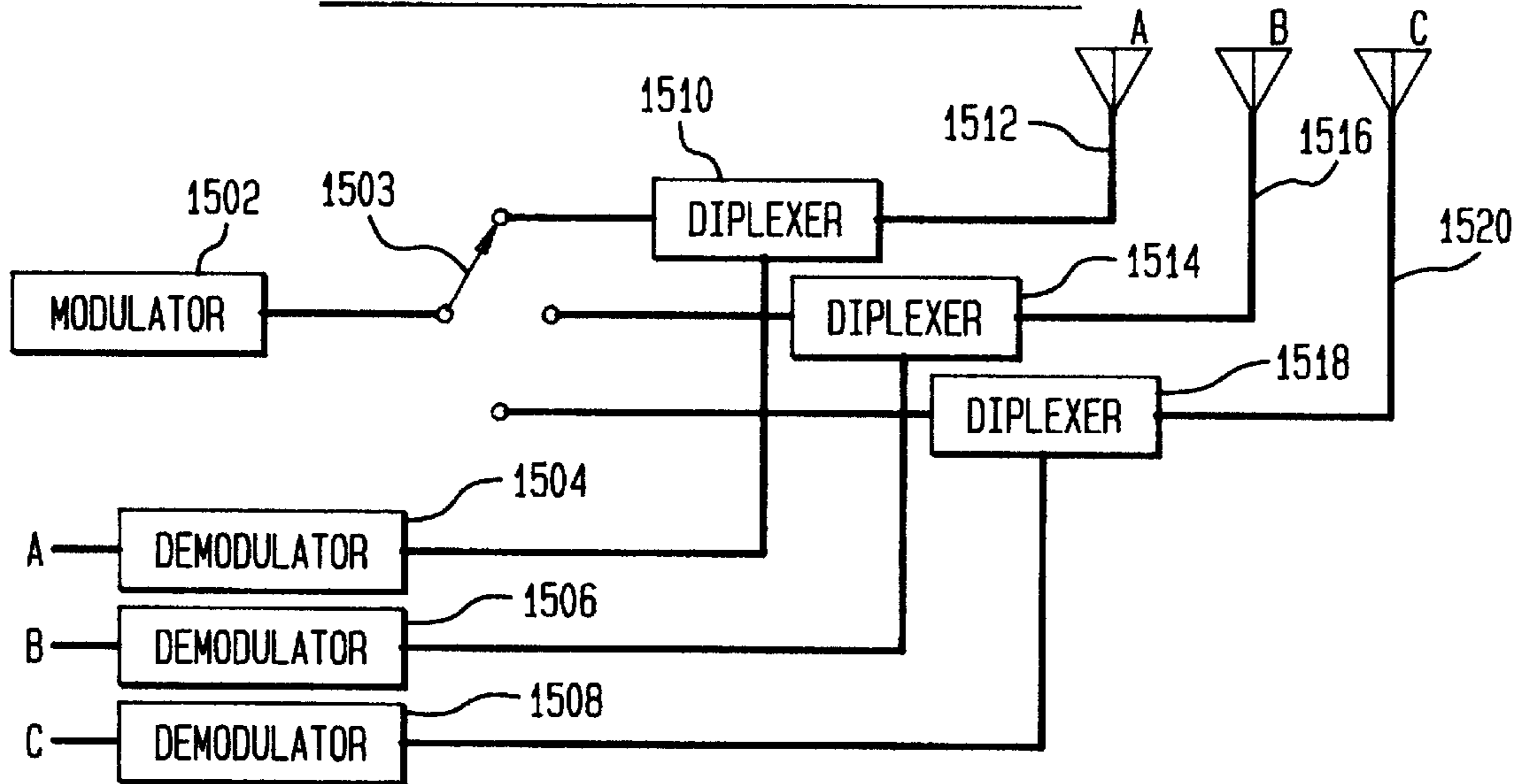
TRANSFER STATION ANTENNA IMPLEMENTATION
