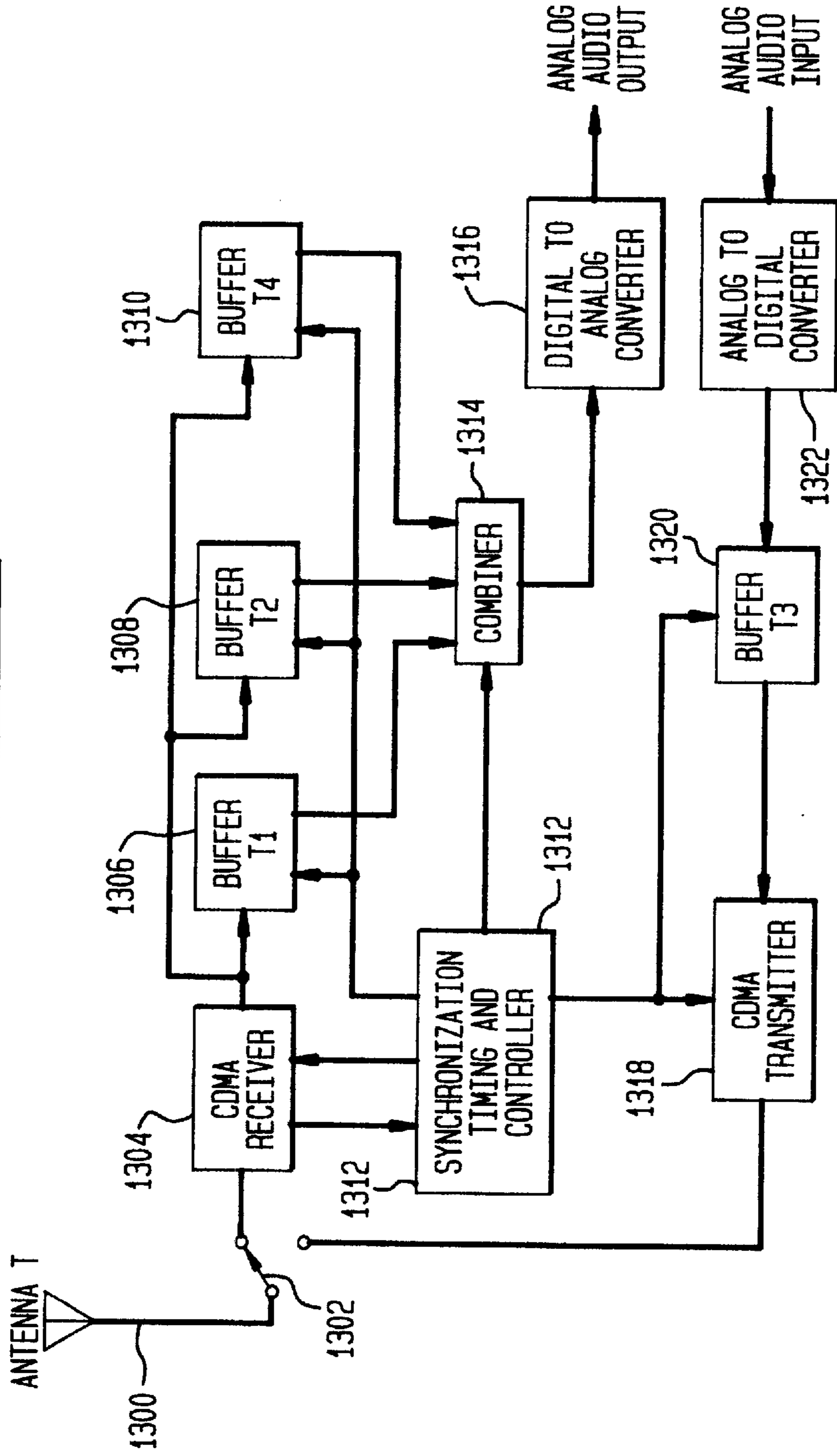
SUBSCRIBER STATION
