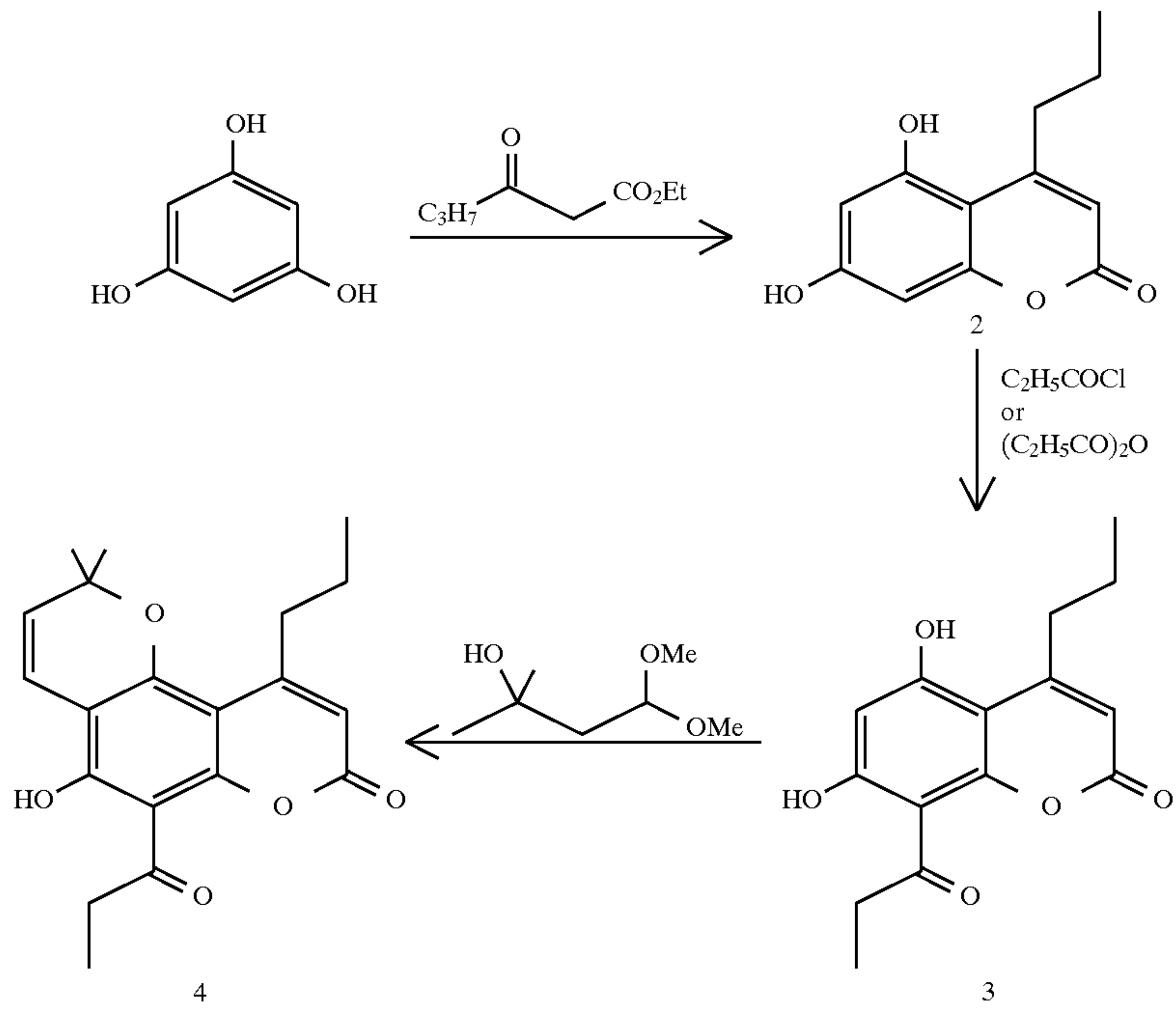
SCHEME I
