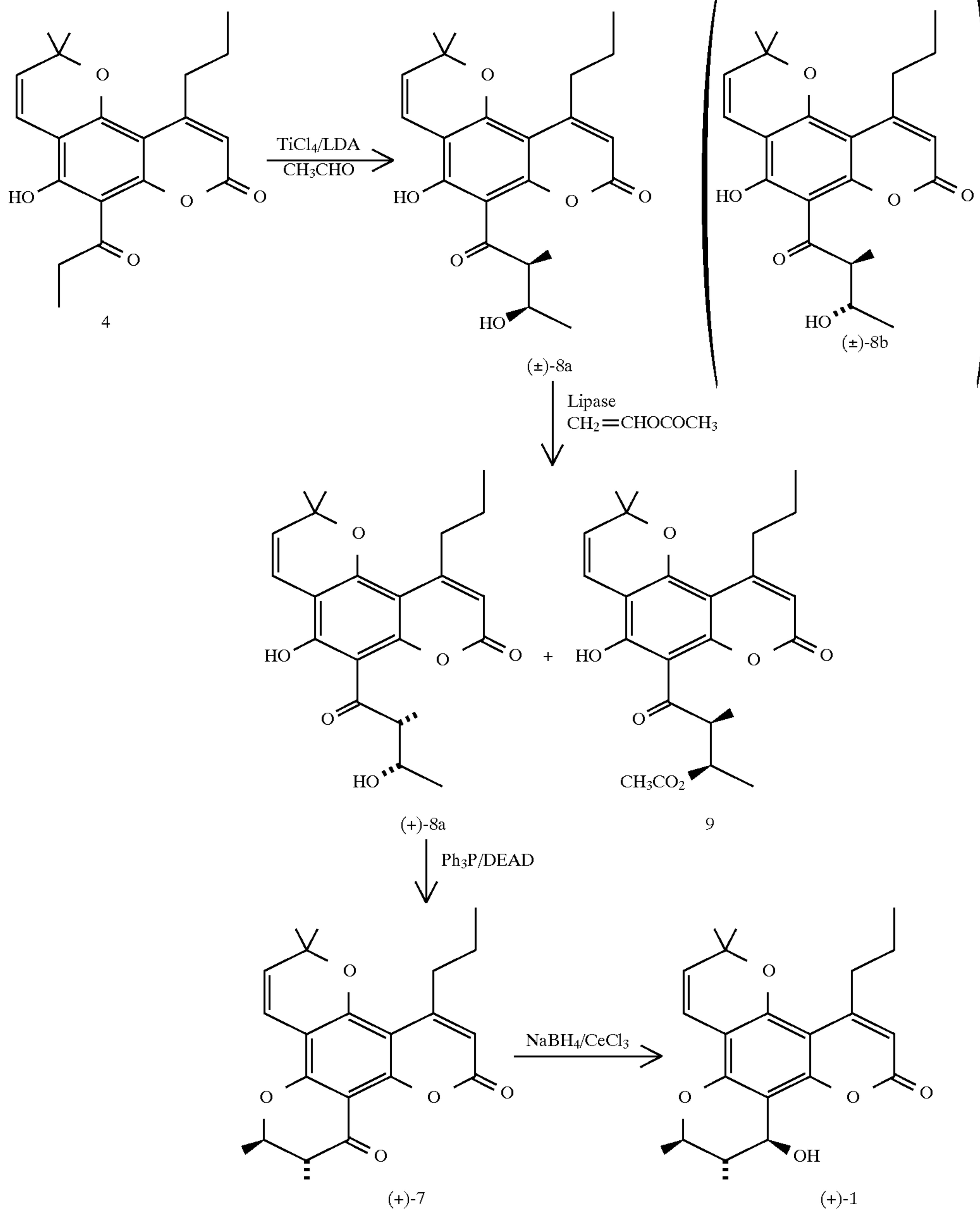
Scheme III
