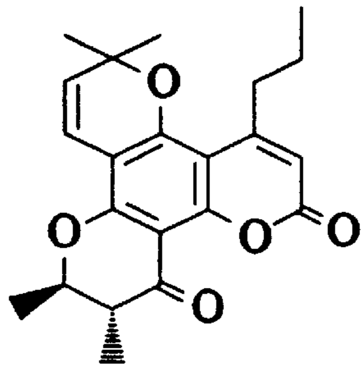
(±)-7
