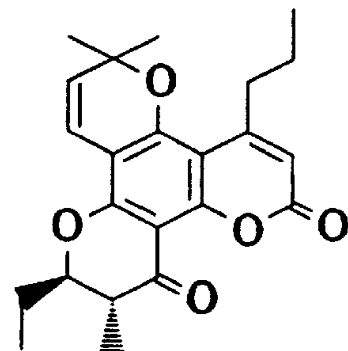
(±)-15c
