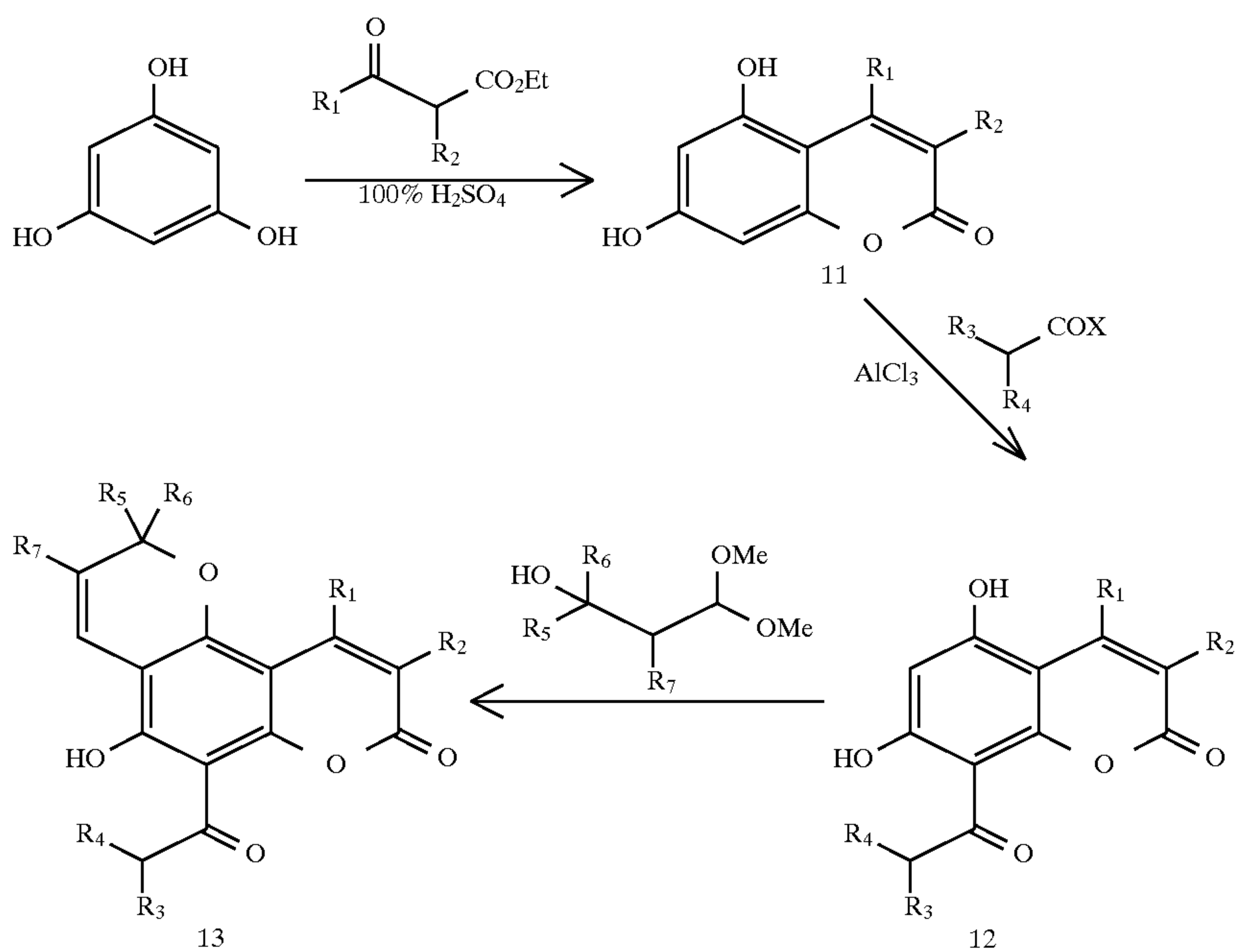
Scheme V
