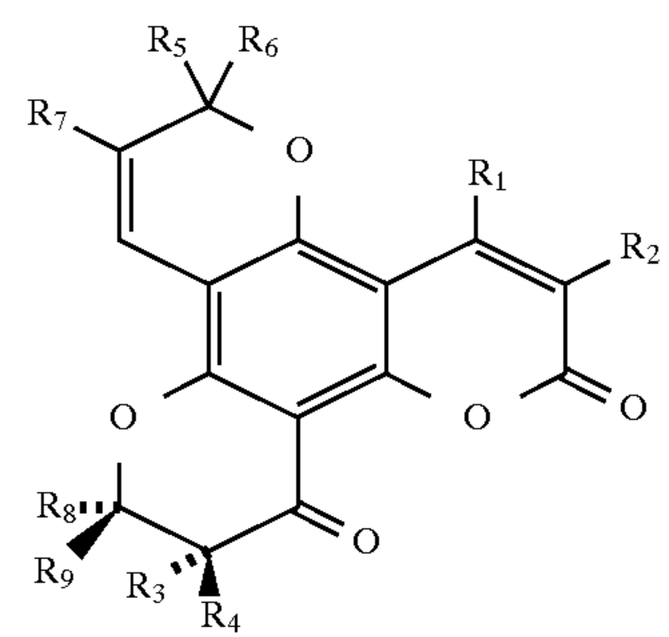
SCHEME VIII
