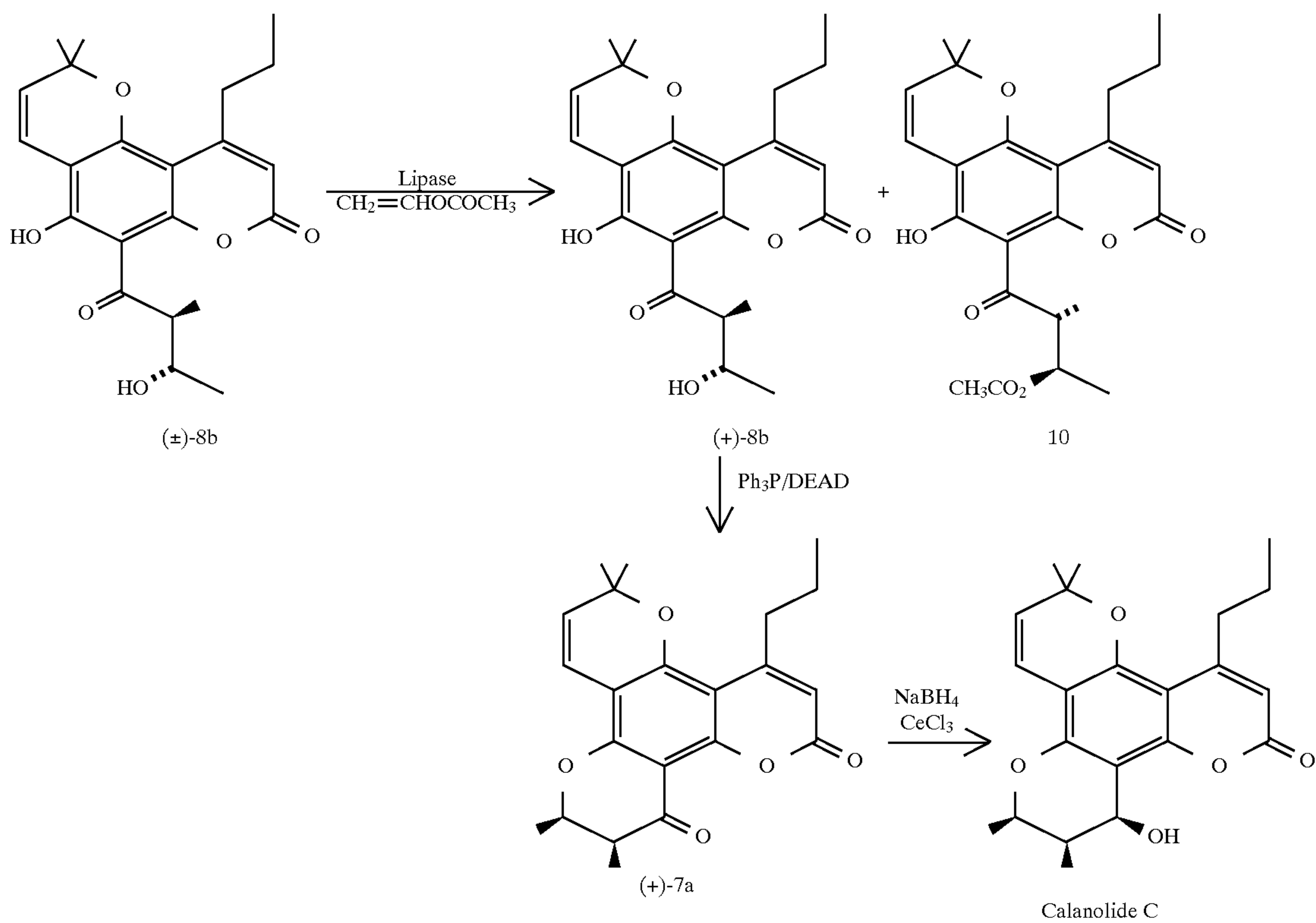
Scheme IV
