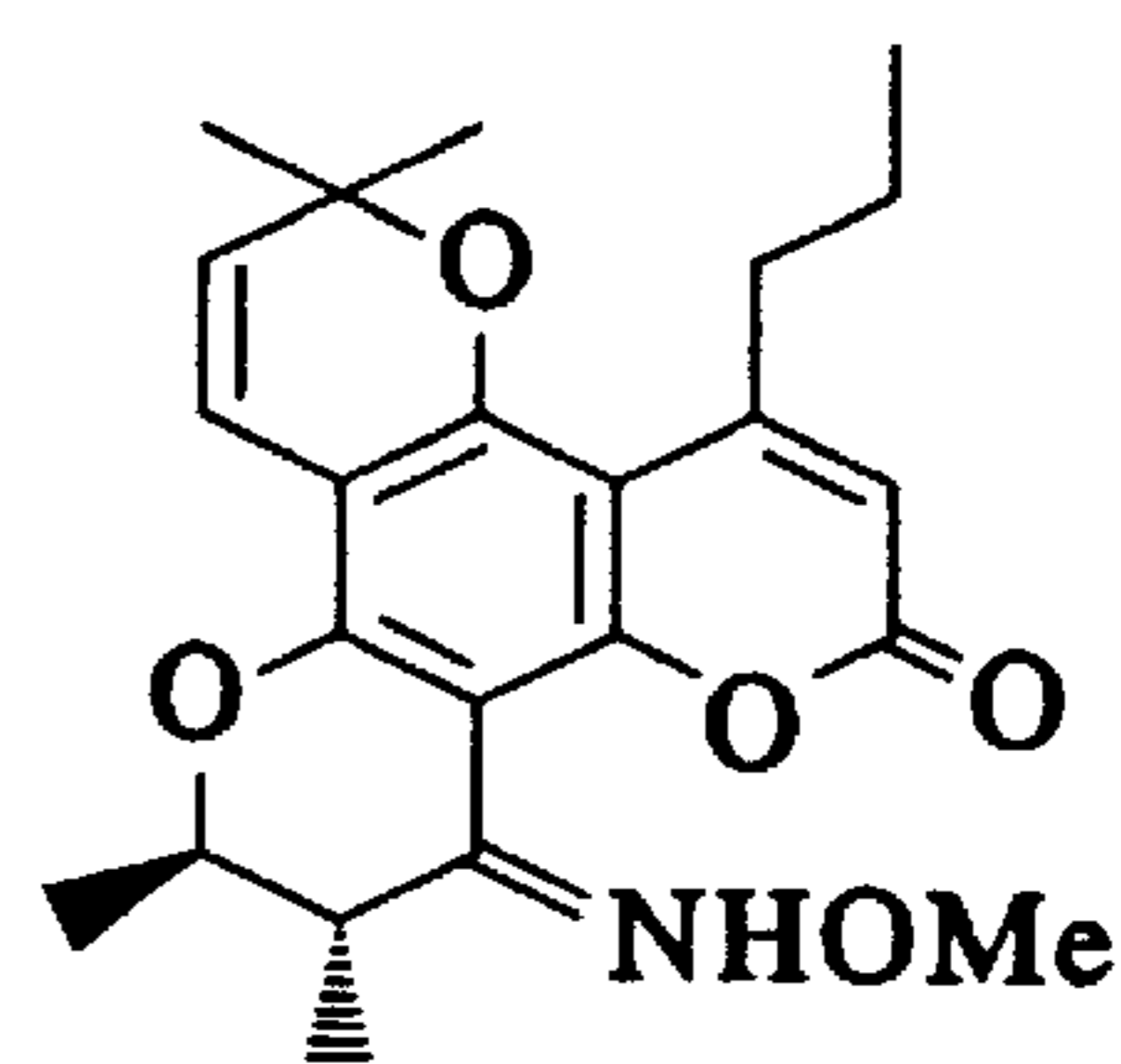
(±)-19b
