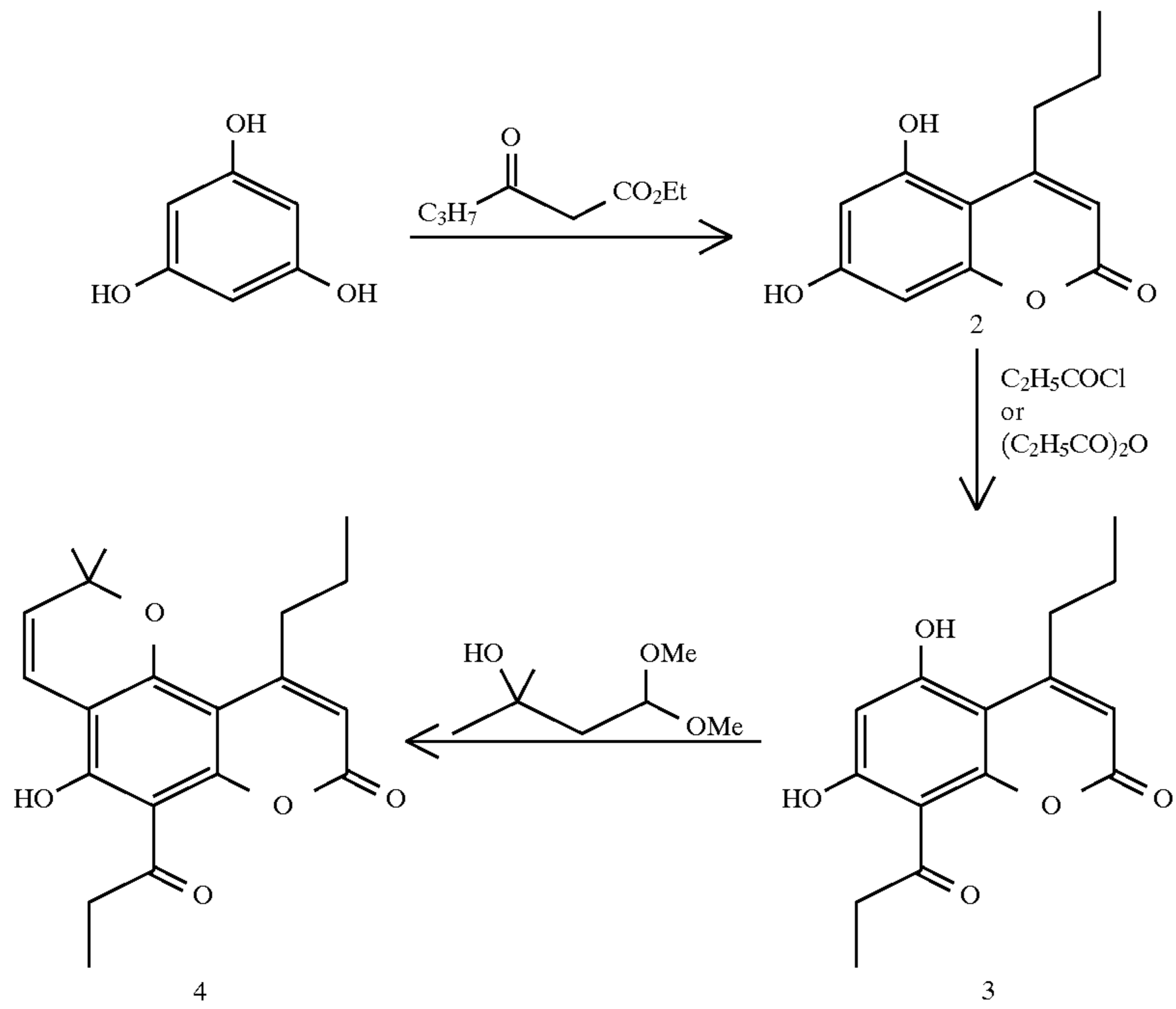
SCHEME I
