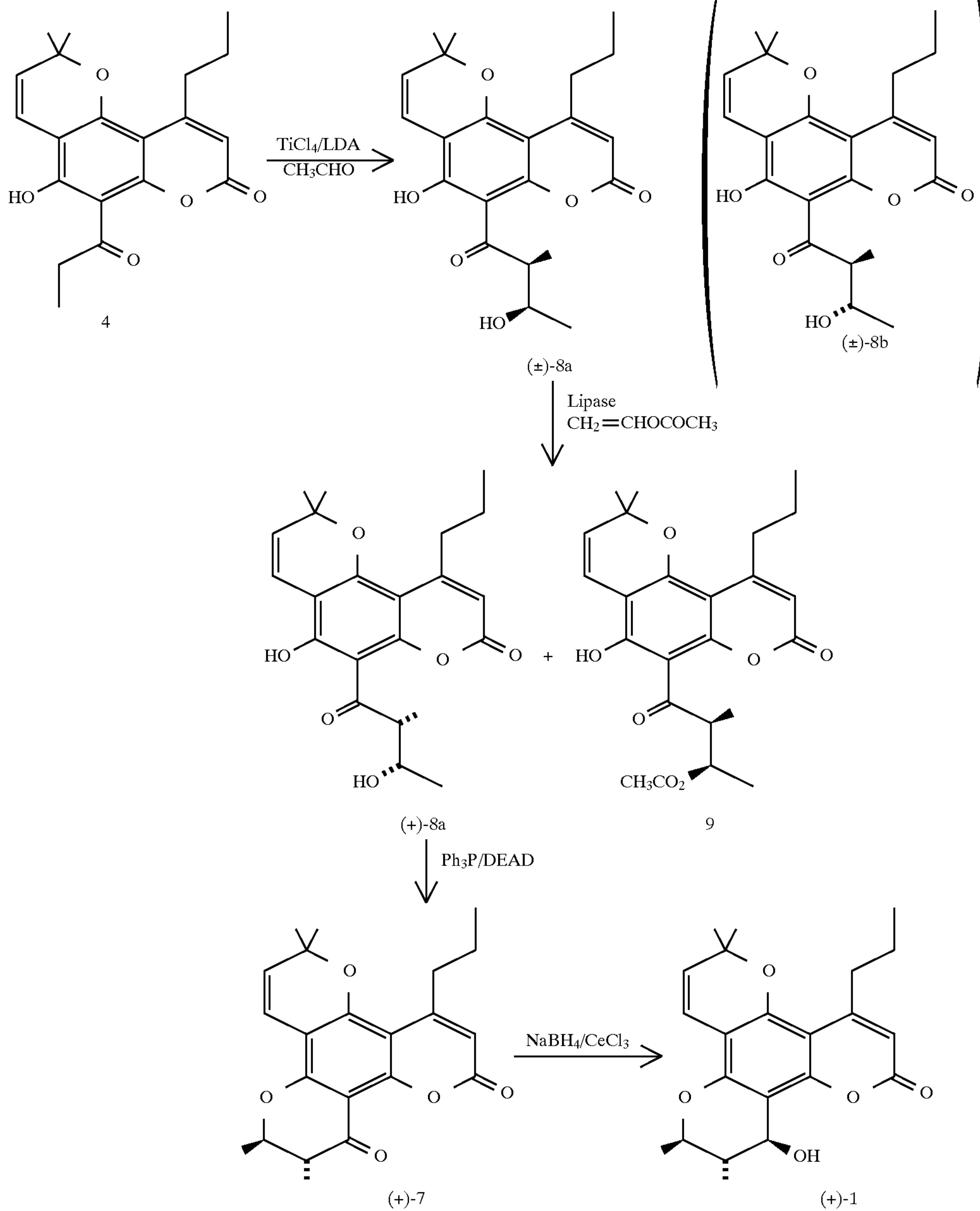
Scheme III
