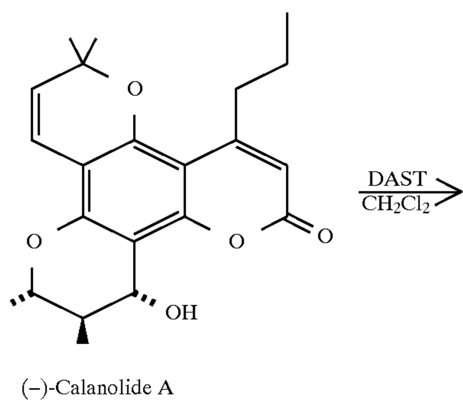
Scheme VII
