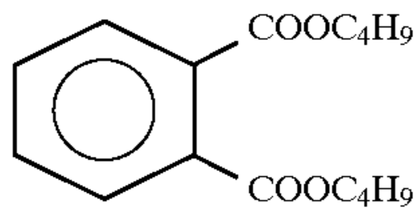
Solvent Solv-3
