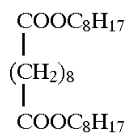
Solvent Solv-8
