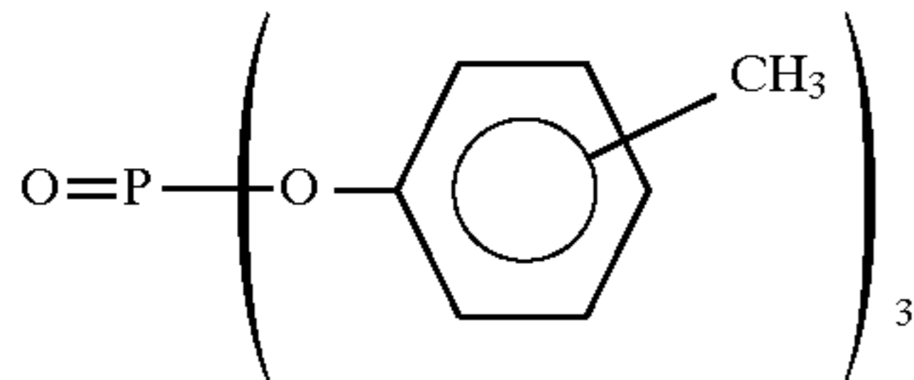
Solvent Solv-6
