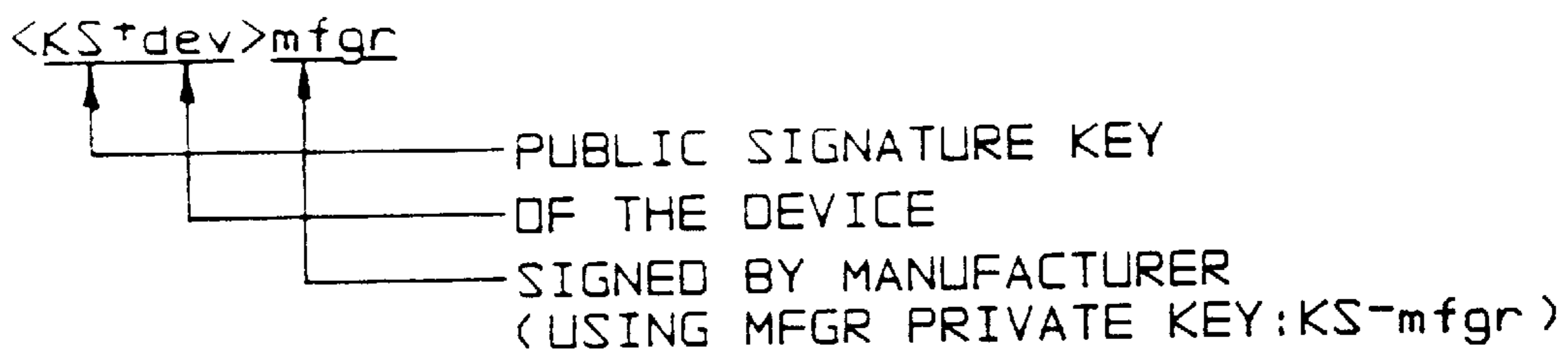
FIG. 1C PUBLIC KEY CERTIFICATE NOTATION (EXAMPLE)
