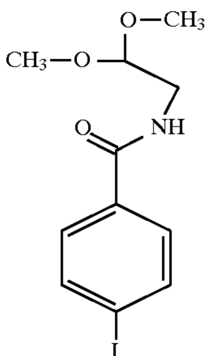
A. N-(2,2-Dimethoxyethyl)-4-iodobenzamide
