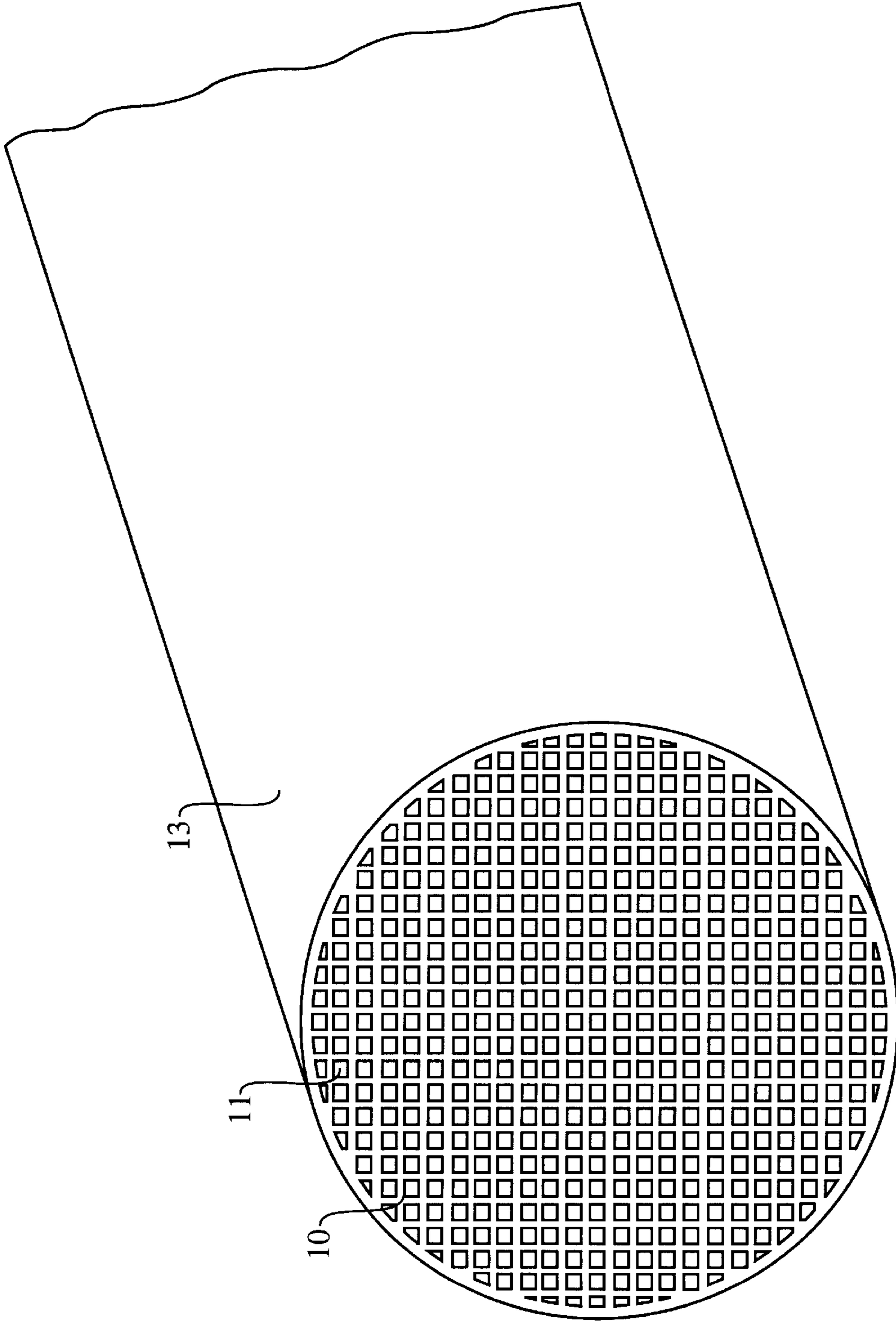
FIG. 4 PRIOR ART
