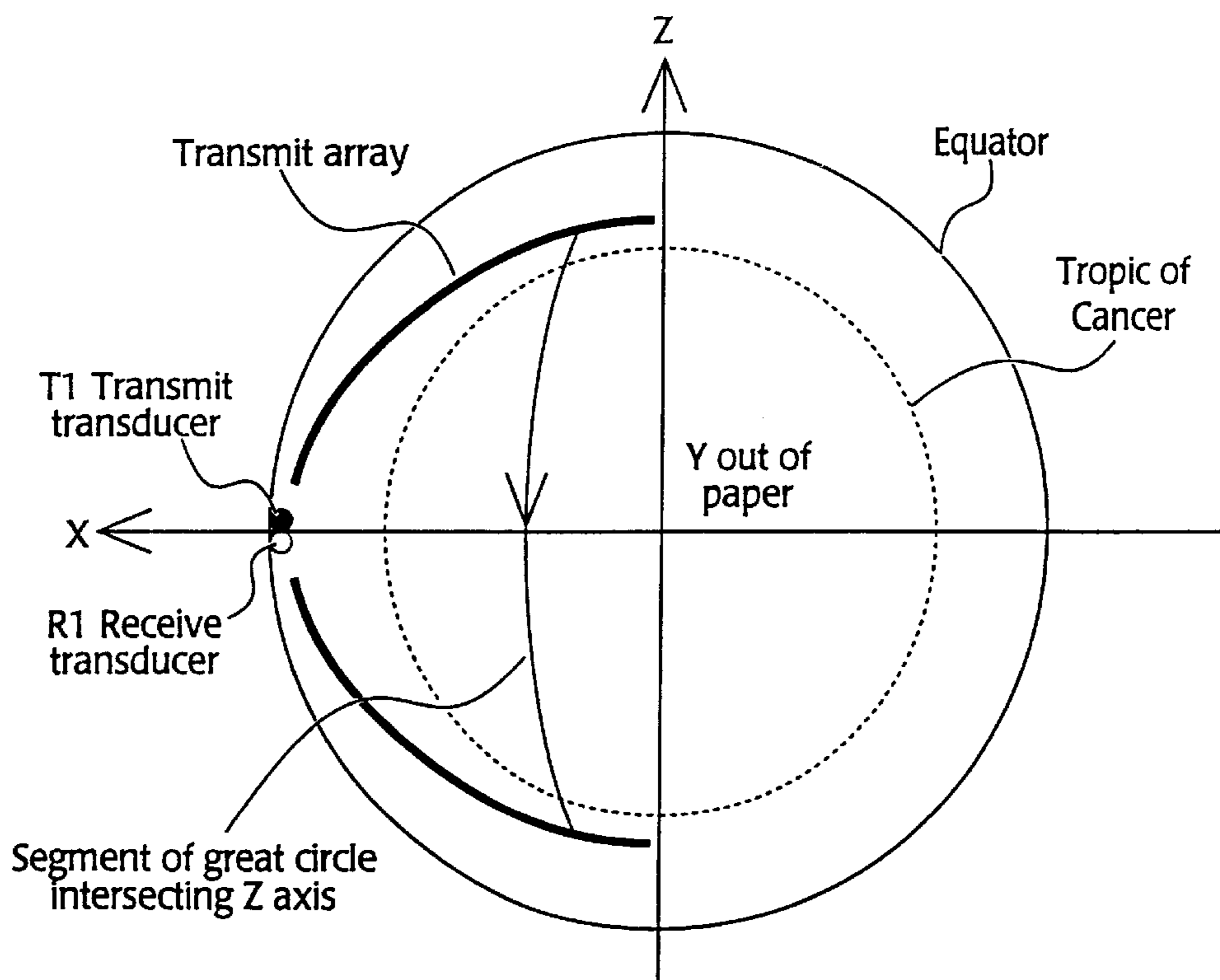
Fig. 21 (d) Top view of first sensor subsystem of alternate spherical sensor layout
