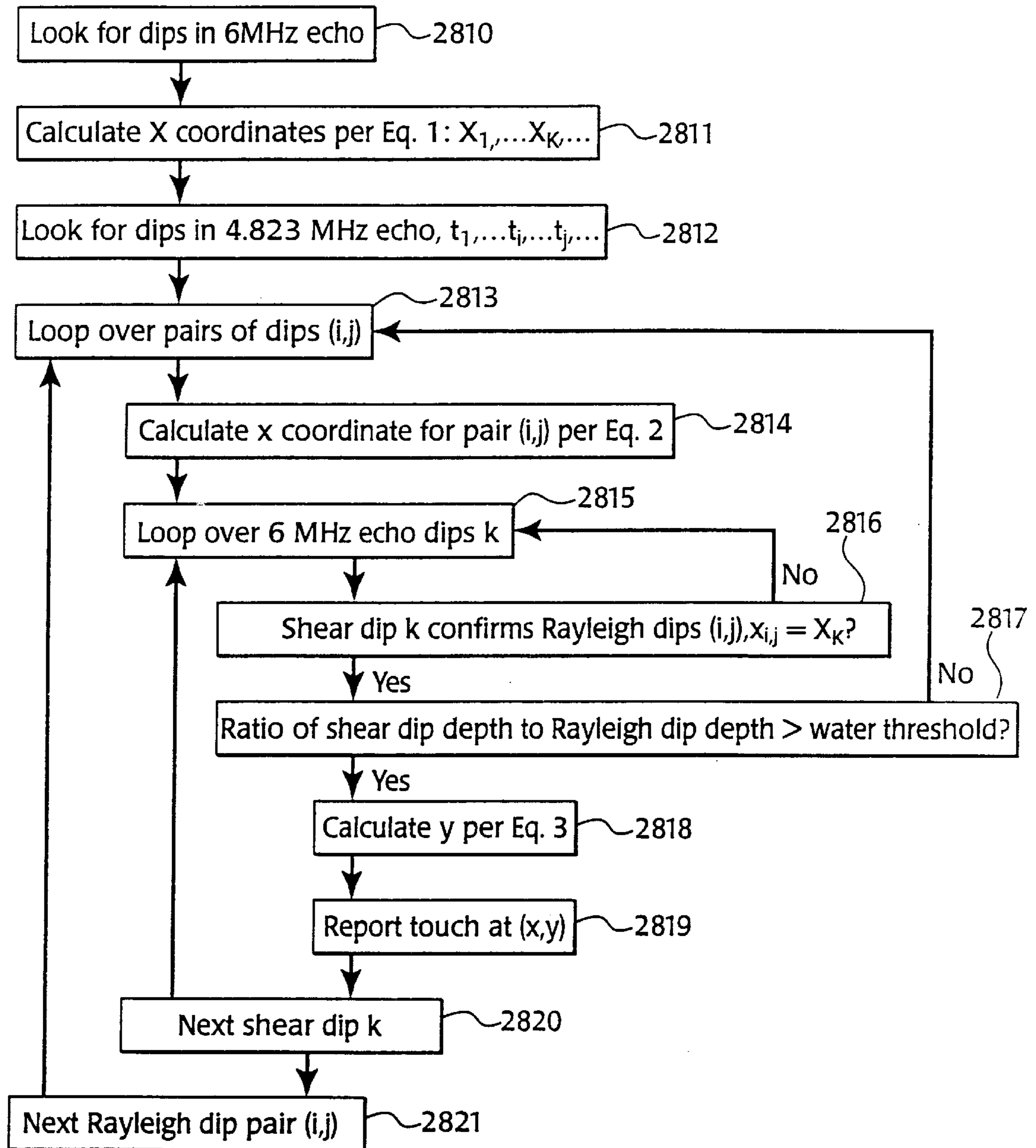
Algorithm flow chart for single-transducer two-frequency sensor
