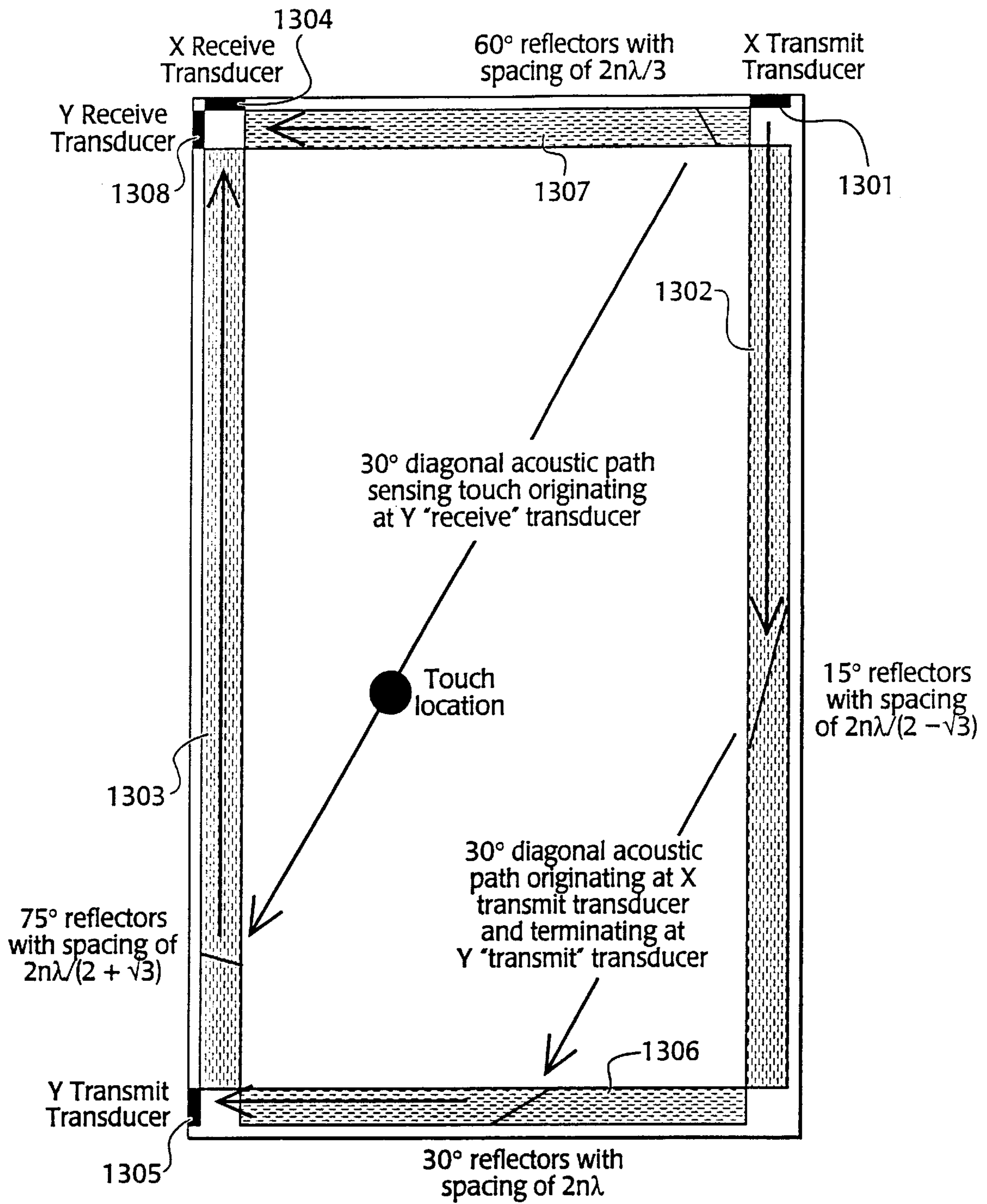
Figure 14 - V Subsystem of X, Y, U, V Sensor
