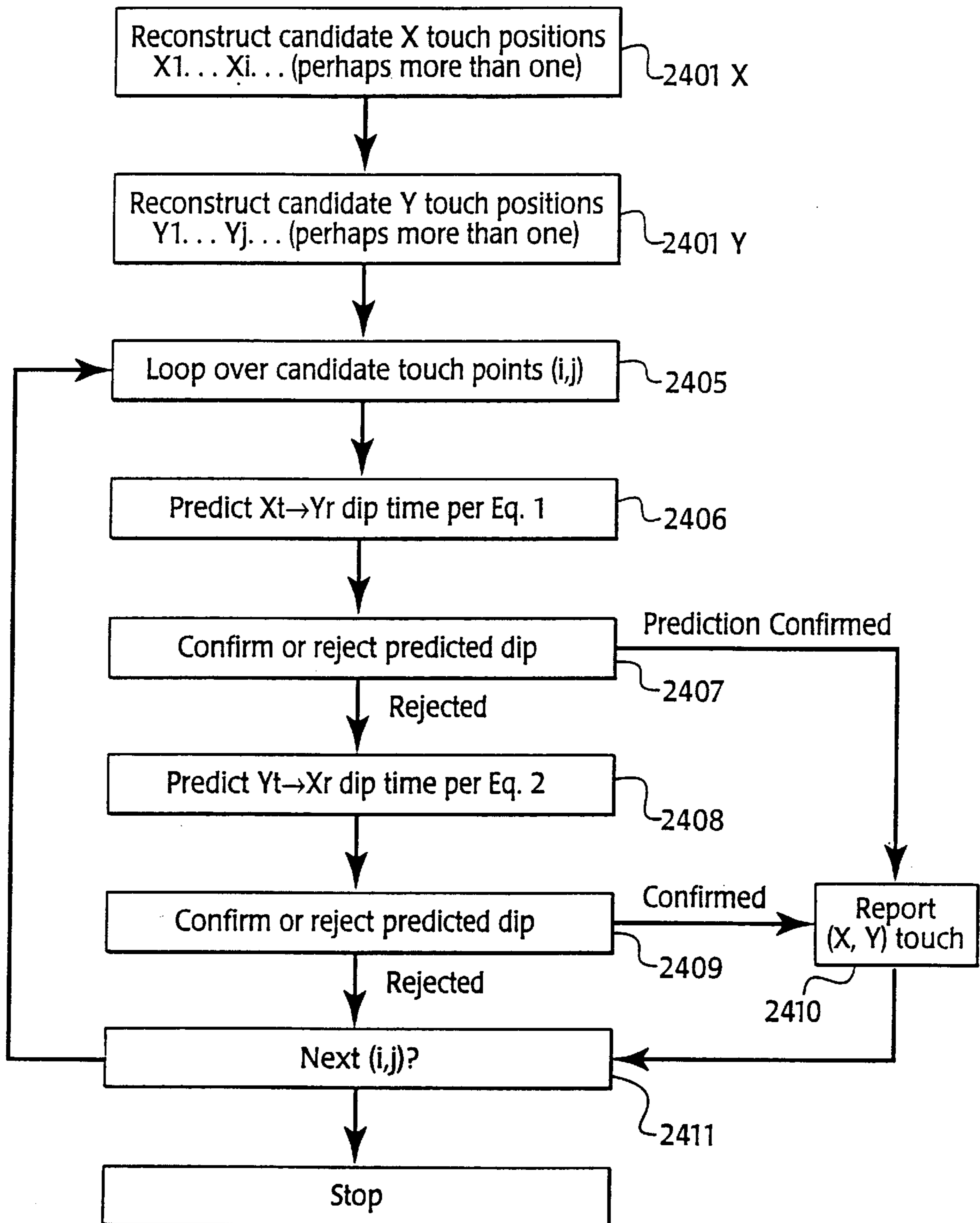
Multiple-Touch/Redundancy-Check Algorithm Flow Chart
