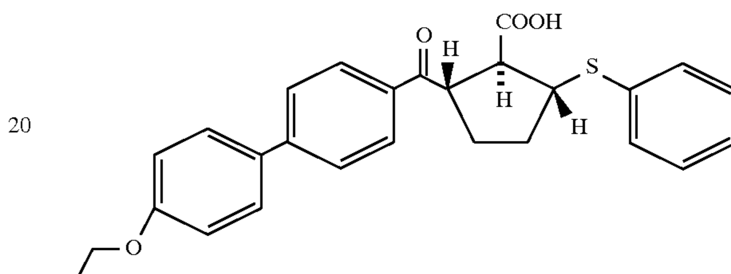
Example 224 (racemate)
