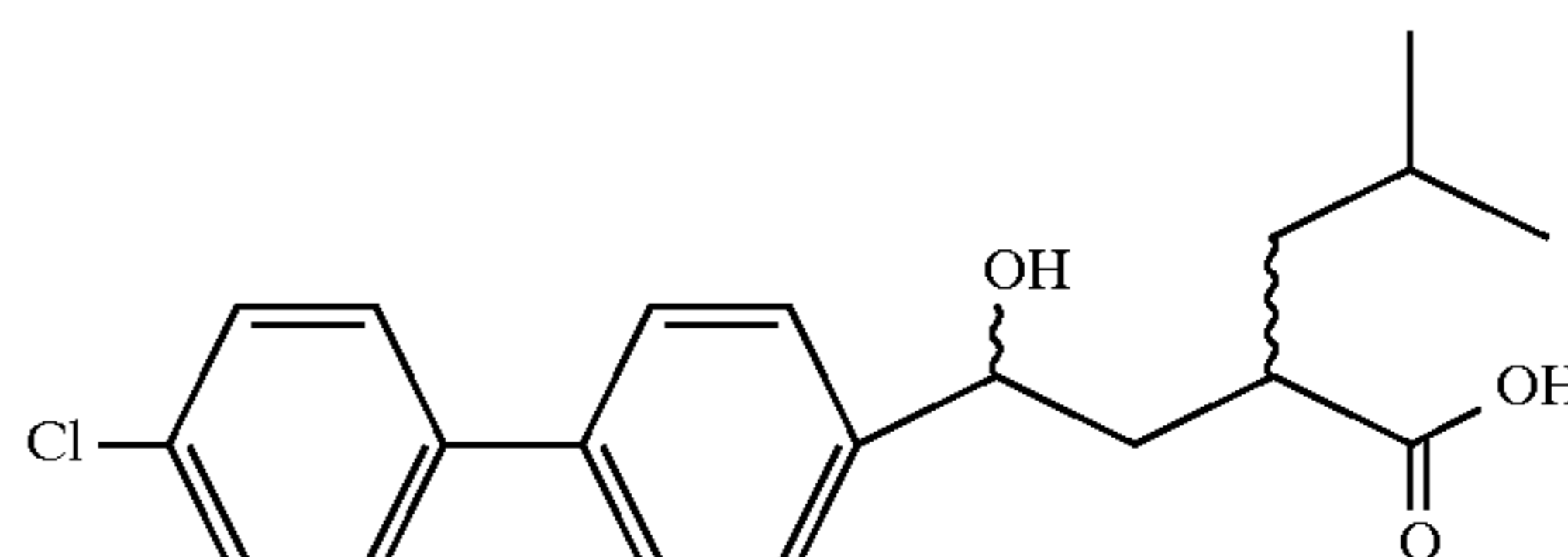
Example 26 Isomer A - First off chromatography column Example 27 Isomer A - Second off chromatography column
