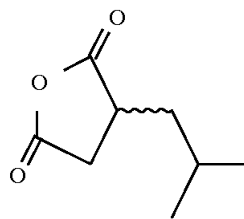
Dihydro-3-(2-methylpropyl)-2,5-furandione
