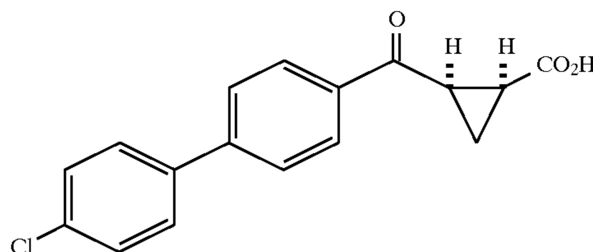
Example 207 (racemate)
