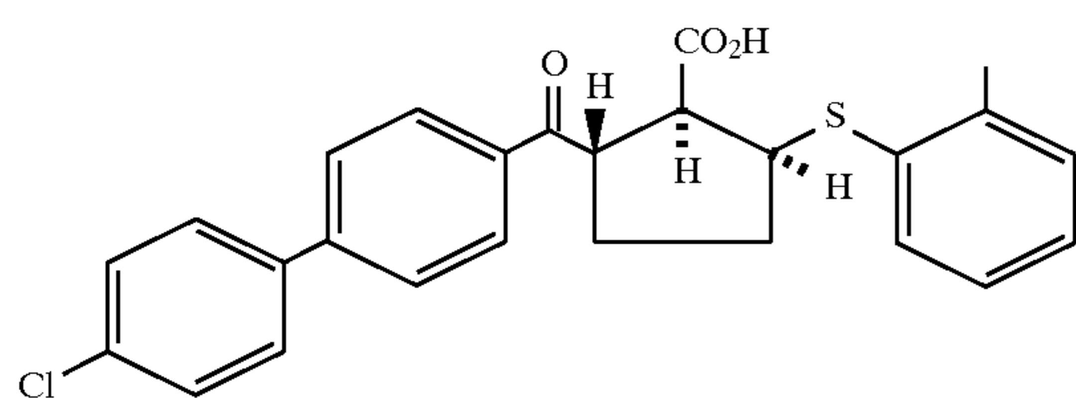
Example 218 (racemate)
