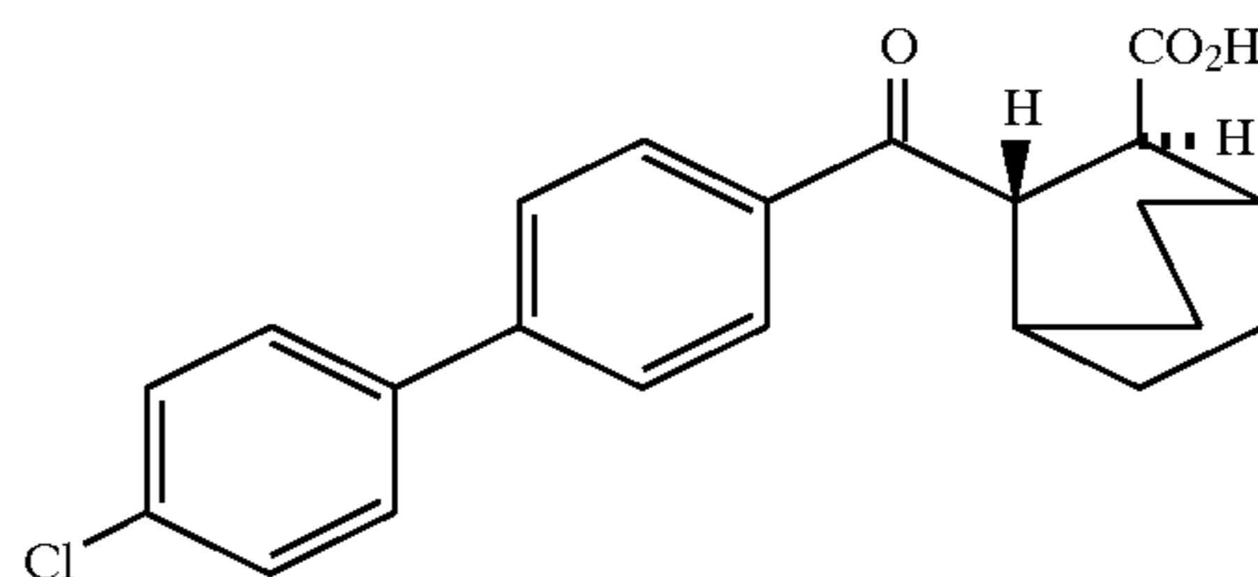
Example 232 (racemate)
