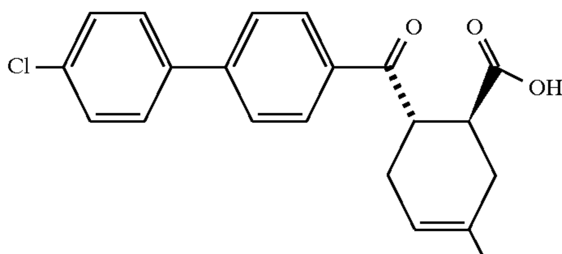
Example 230 (racemate)
