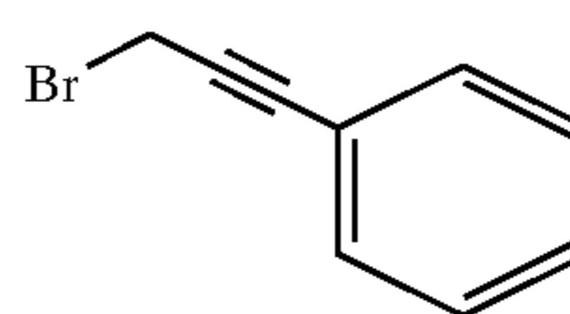
1-phenyl-3-bromo-1-propyn
