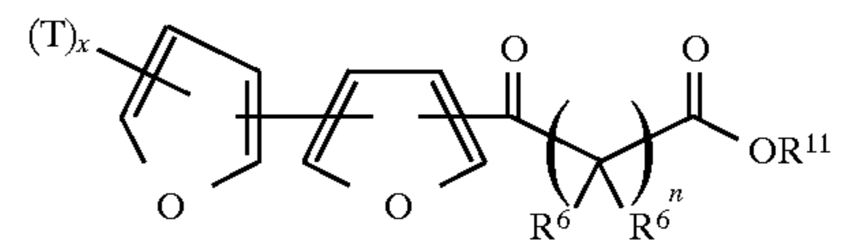
I-H-4
