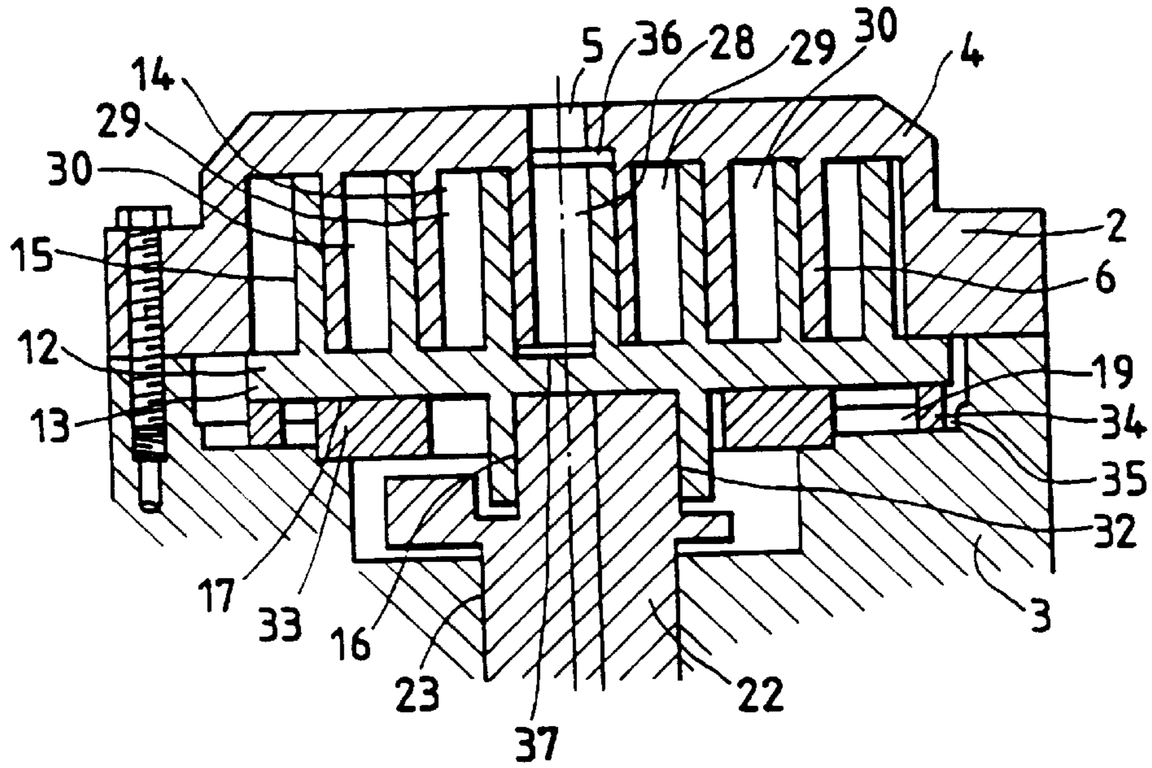
FIG. 17 PRIOR ART
