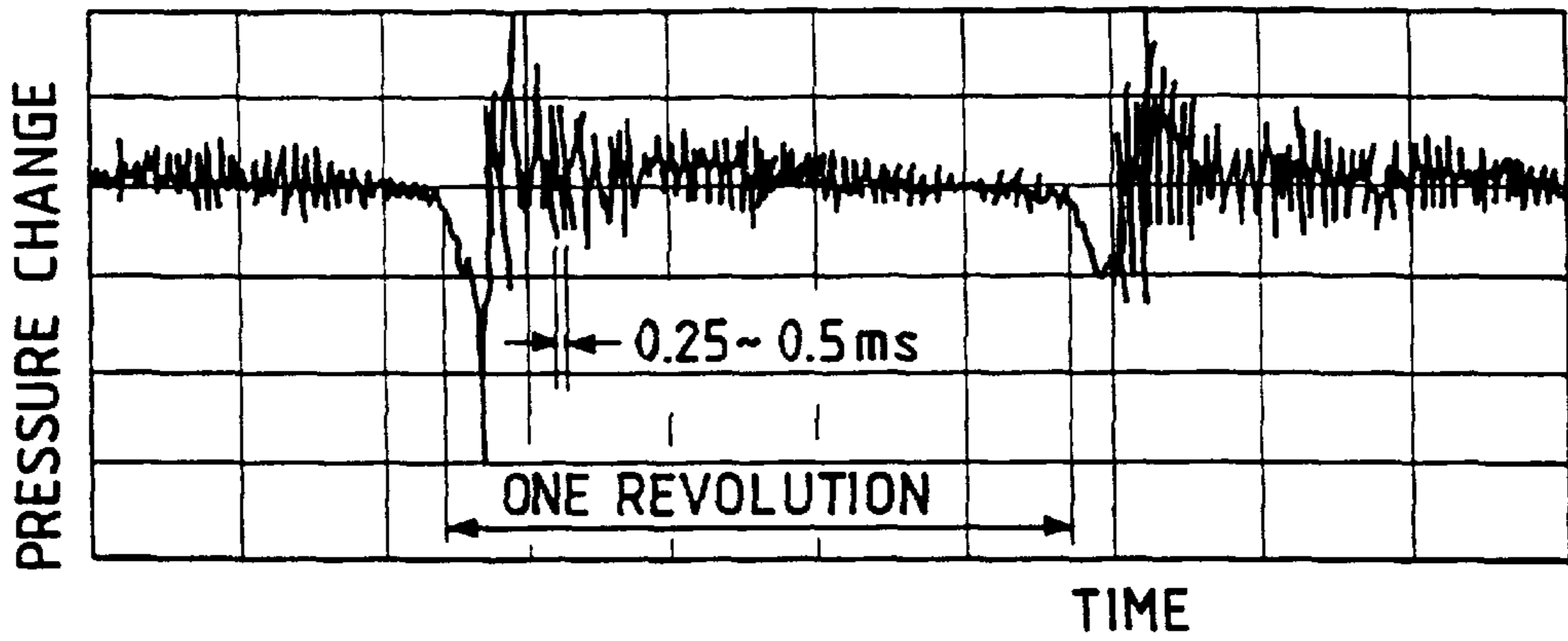
FIG. 9 PRIOR ART
