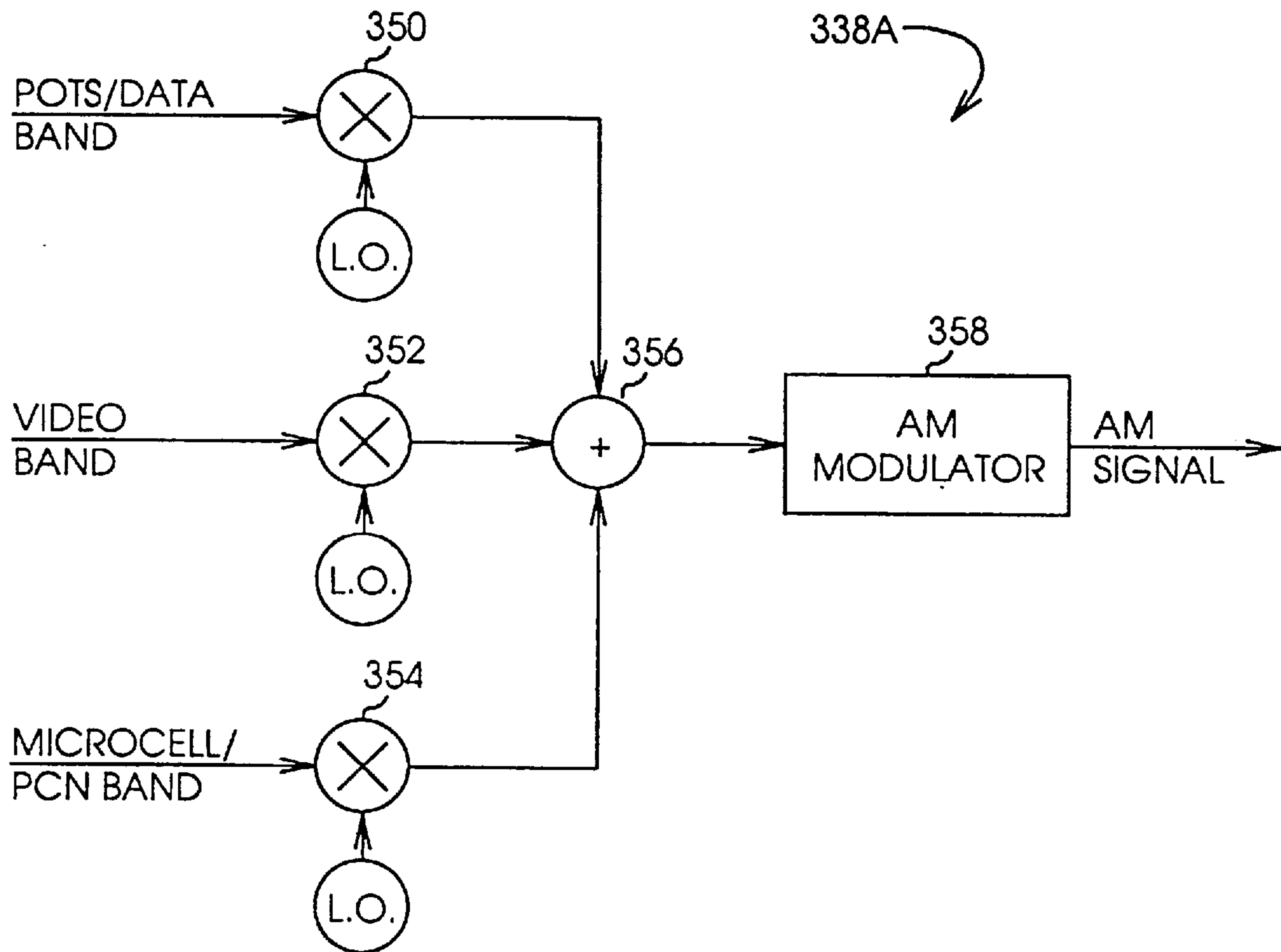
AM Modulator
