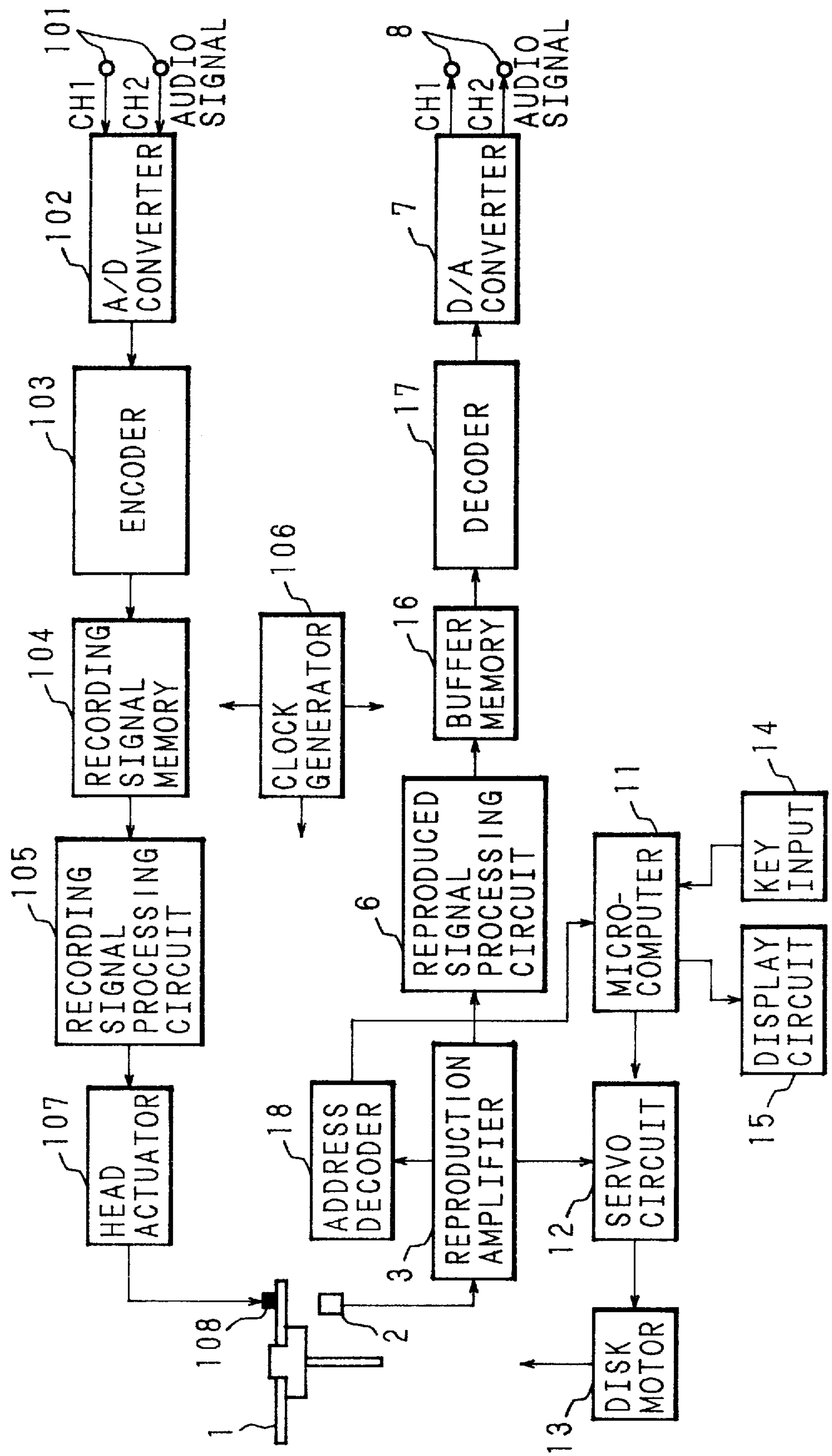
Fig. 1 Prior Art
