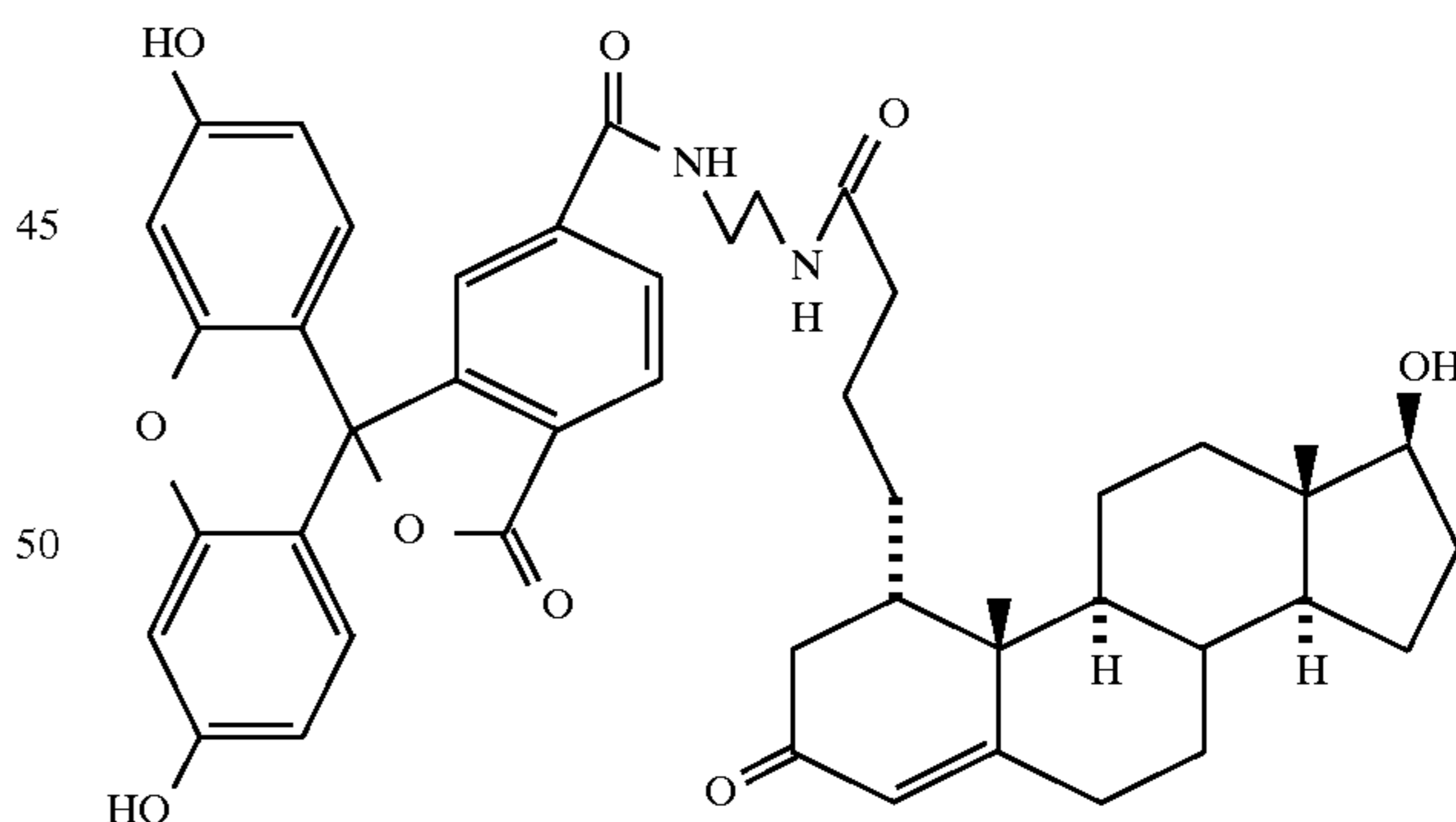
FORMULA 3 STRUCTURE OF THE PREFERRED FLUORESCHEIN-LABELED TESTOSTERONE REAGENT
