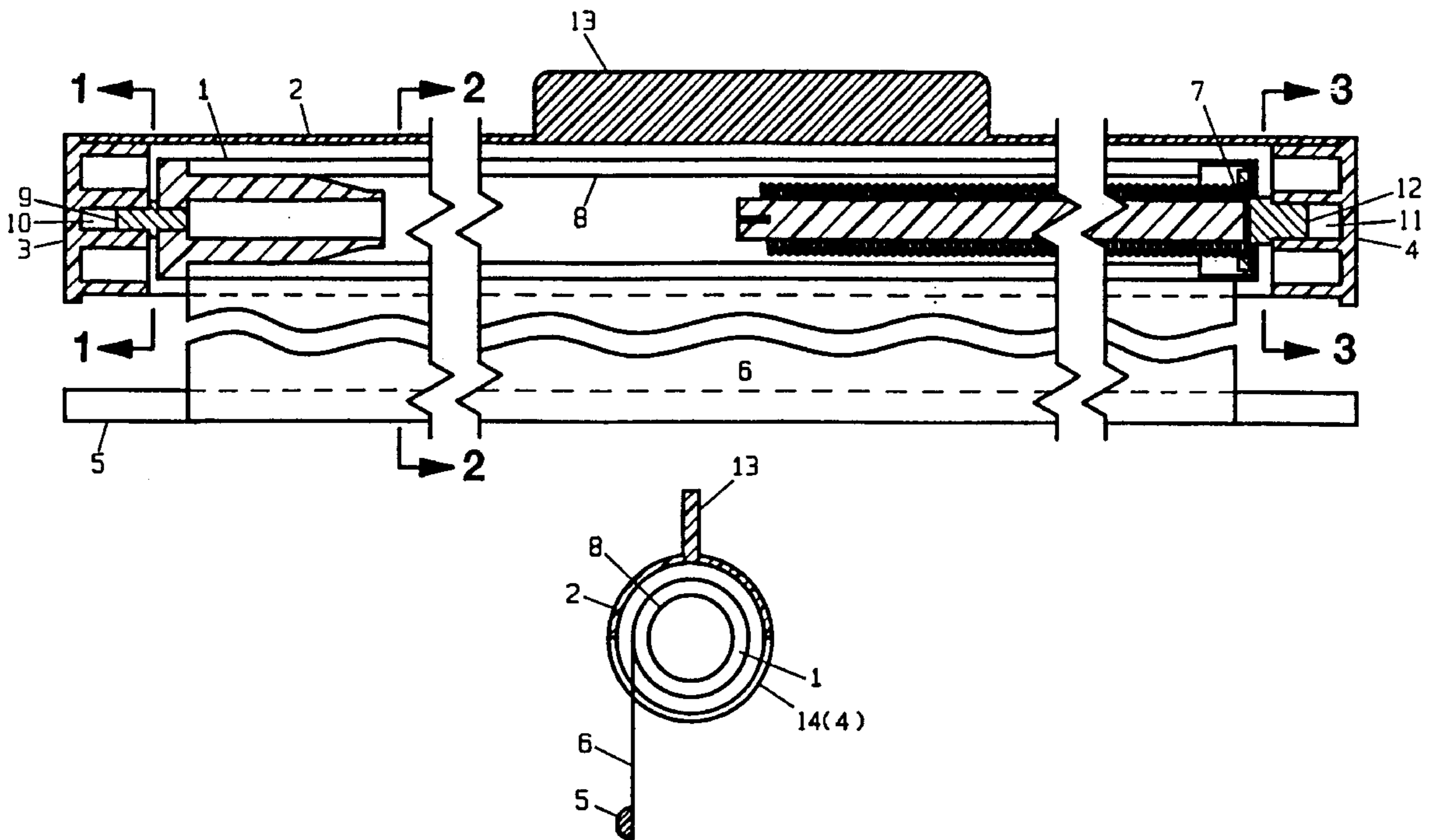
SECT. 2-2
