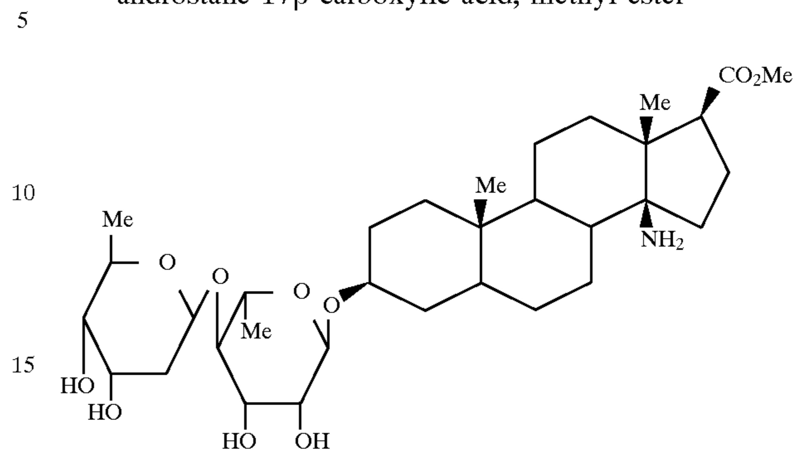
14 \beta -amino-3 \beta -[4''-O-acetyl-2'',3''-O-isopropylidene- \beta -(L)-rhamnopyranosyloxy-(1 \rightarrow 4)-2',3'-O-isopropylidene- \alpha -(L)-rhamnopyranosyloxy]-5 \beta -androstane-17 \beta -carboxylic acid, methyl ester
