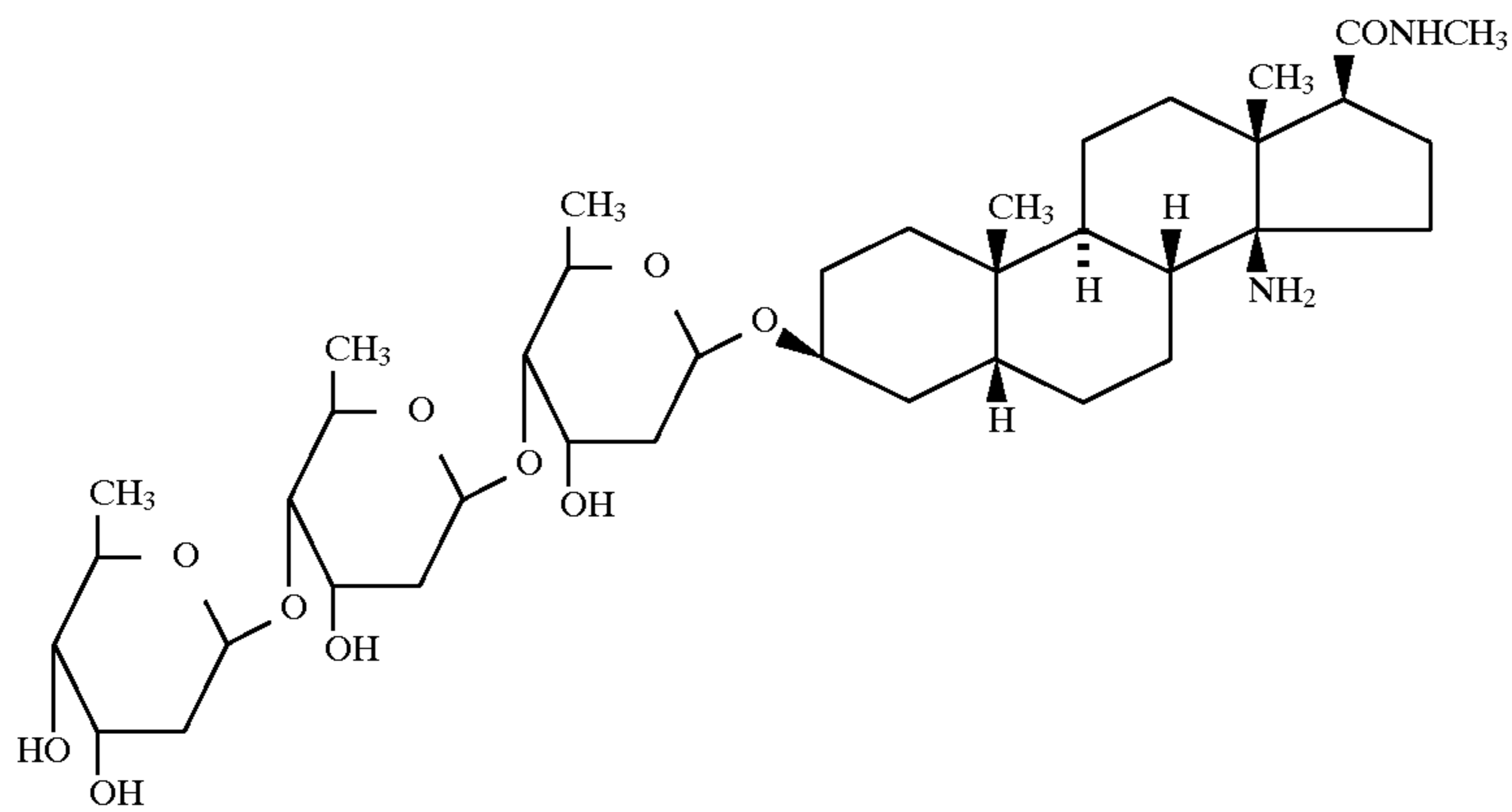
(3 \beta ,5 \beta ,14 \beta ,17 \beta )-14-Amino-3-[(0-2,6-dideoxy- \beta -D-ribo- hexopyranosyl-(1 \rightarrow 4)-0-2,6-dideoxy- \beta -D-ribo- 20 hexopyranosyl(1 \rightarrow 4)-2,6-dideoxy- \beta -D-ribo- hexopyranosyl)oxy]-N-methylandrostande-17- carboxamide
