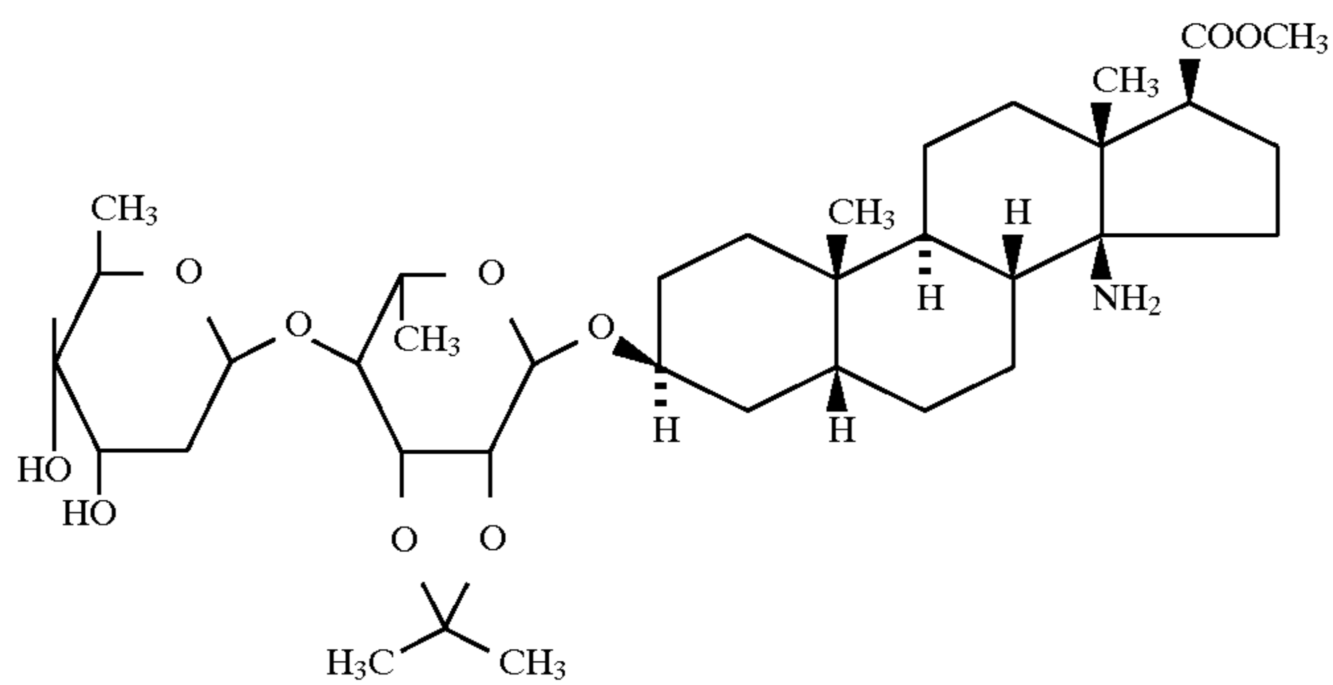
(3 \beta ,5 \beta ,14 \beta ,17 \beta )-14-Amino-3-[[0-2,6-dideoxy- \beta -D-ribo- 40 hexopyranosyl-(1 \rightarrow 4)-6-deoxy-2,3-O-(1- methylethylidene)- \alpha -L-mannopyranosyl]oxy] androstande-17-carboxylic acid, methyl ester
