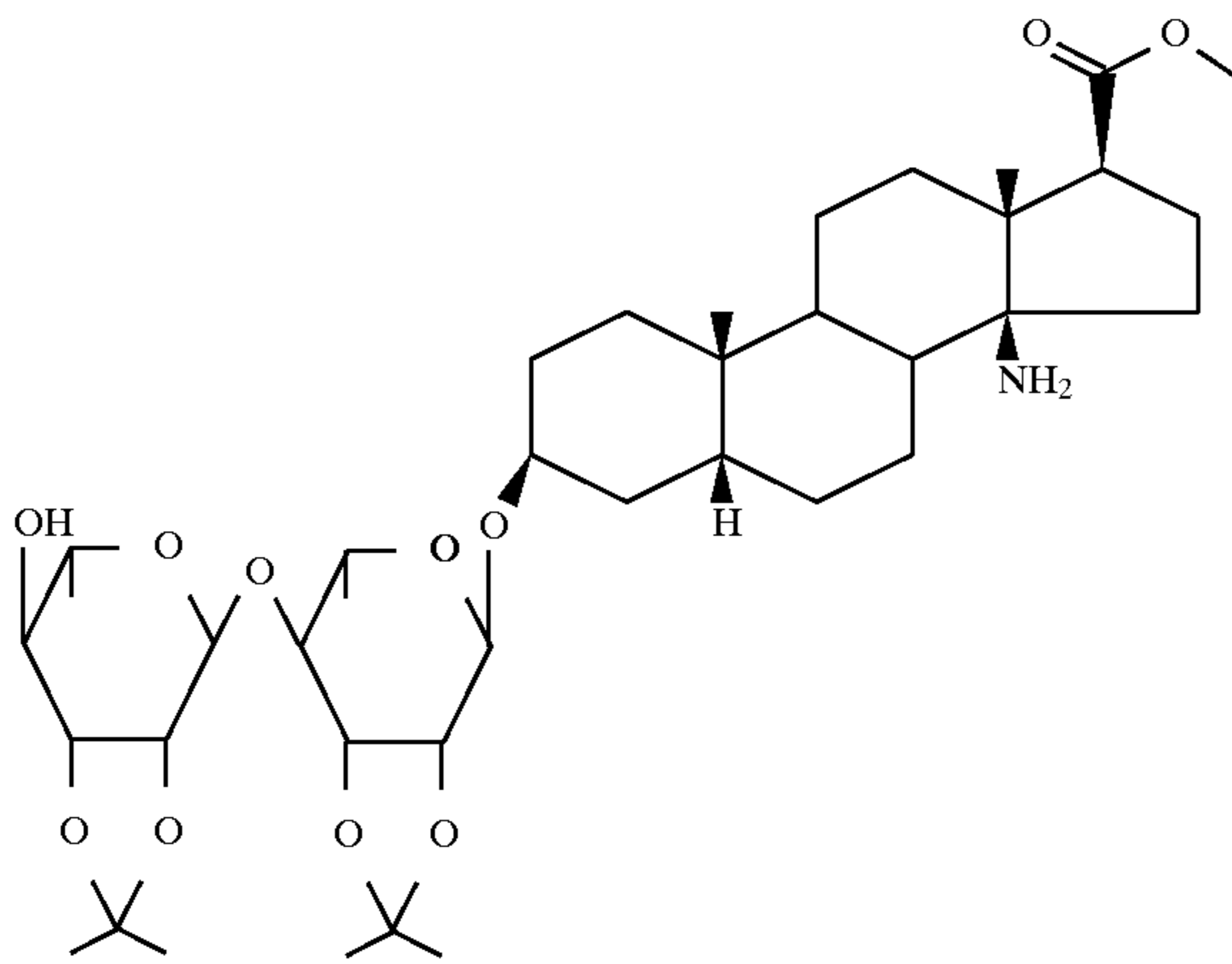
14 \beta -amino-3 \beta -[2'',3''-O-isopropylidene- \beta -(L)-rhamnopyranosyl-oxy-(1 \rightarrow 4)-2',3'-O-isopropylidene- \alpha -(L)-rhamnopyranosyloxy]-5 \beta -androstane-17 \beta -carboxylic acid, methyl ester
