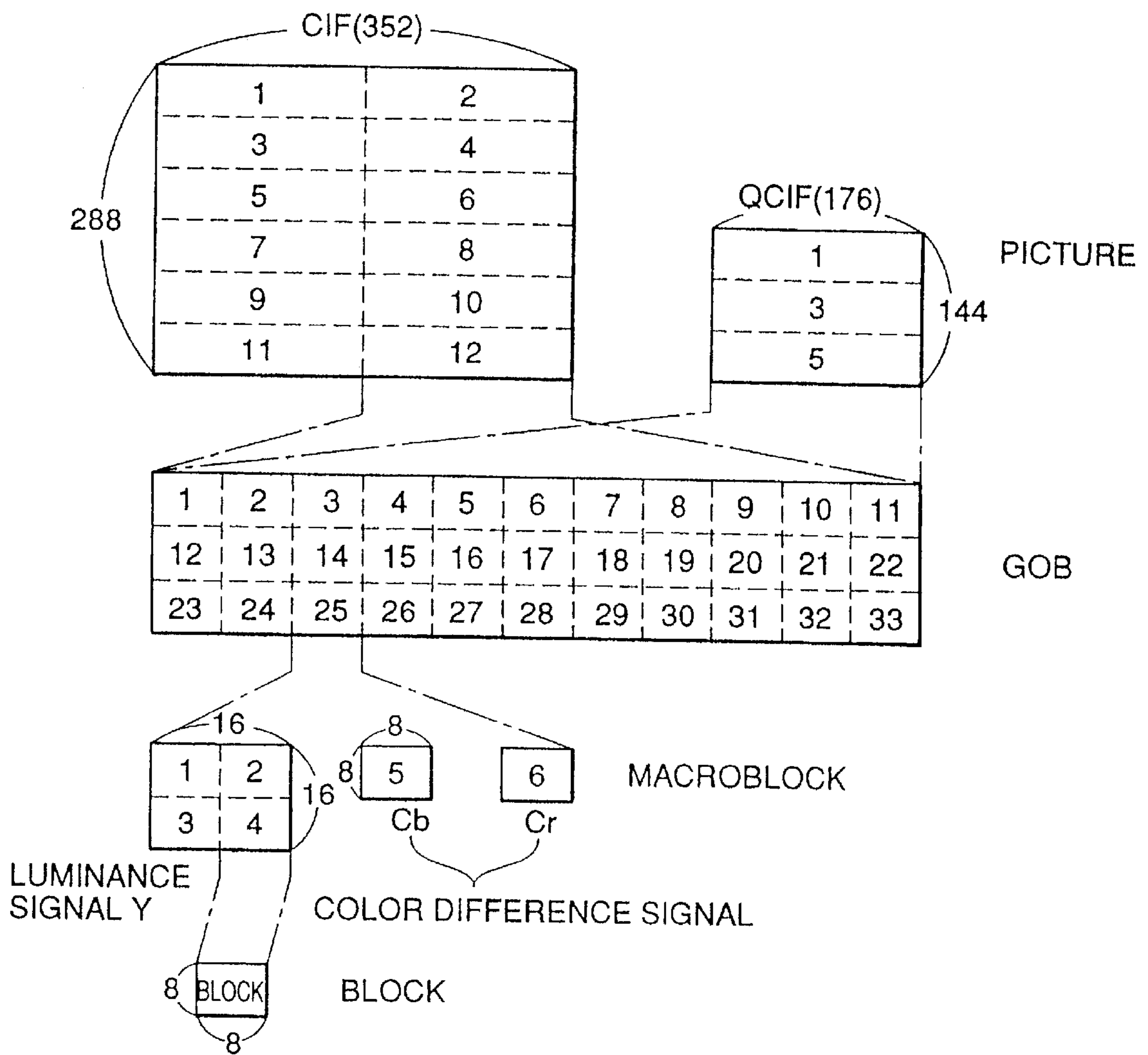
HIERARCHIAL DIVISIONS OF MOVING IMAGE DATA
