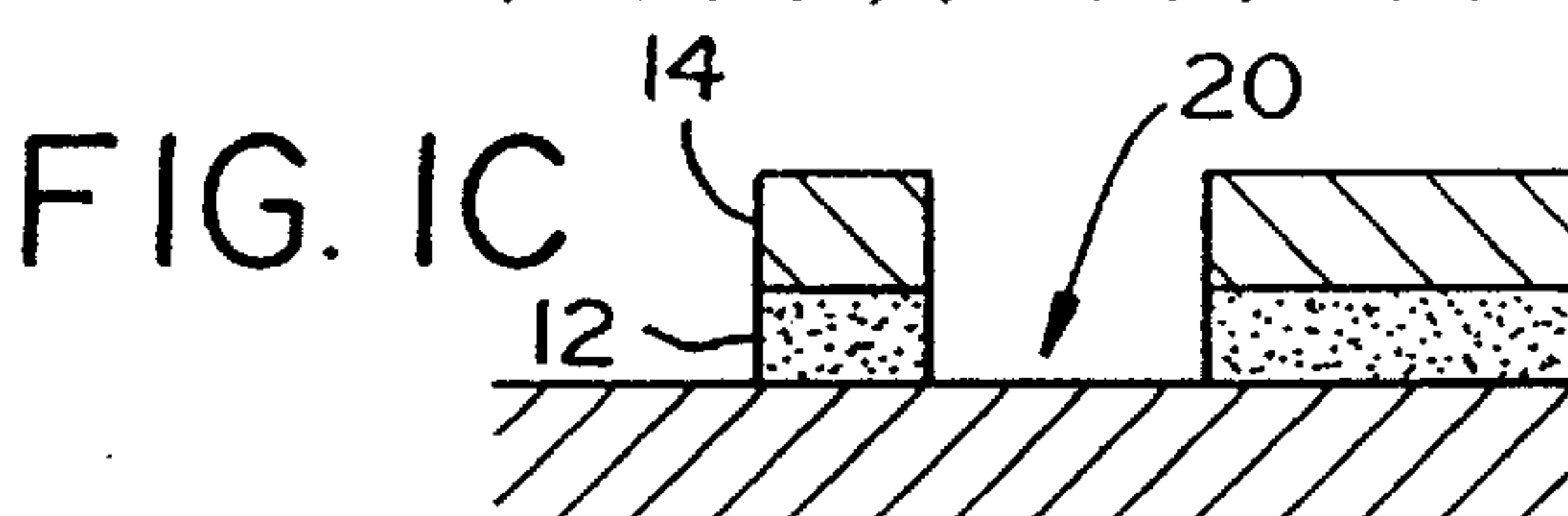
Step 3: Transfer Pattern
