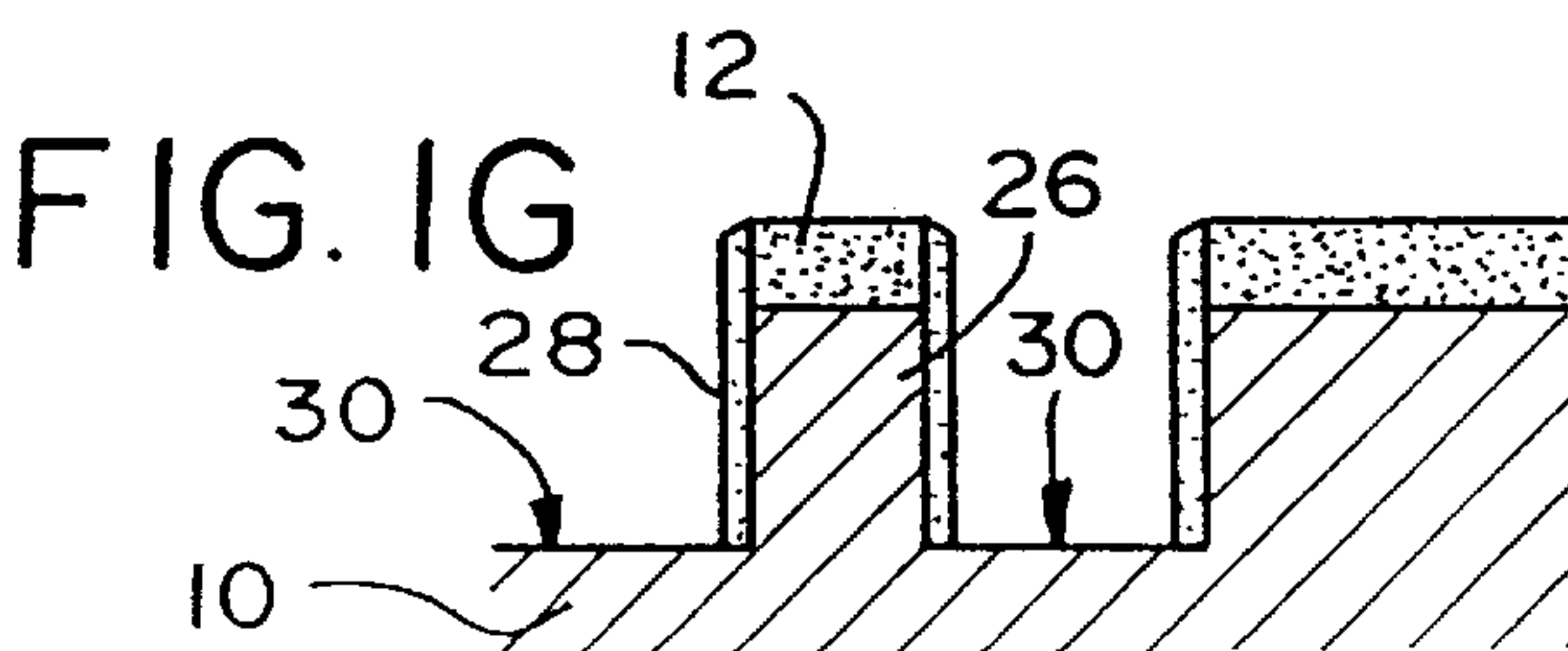
Step 7: Vertical Oxide Etch
