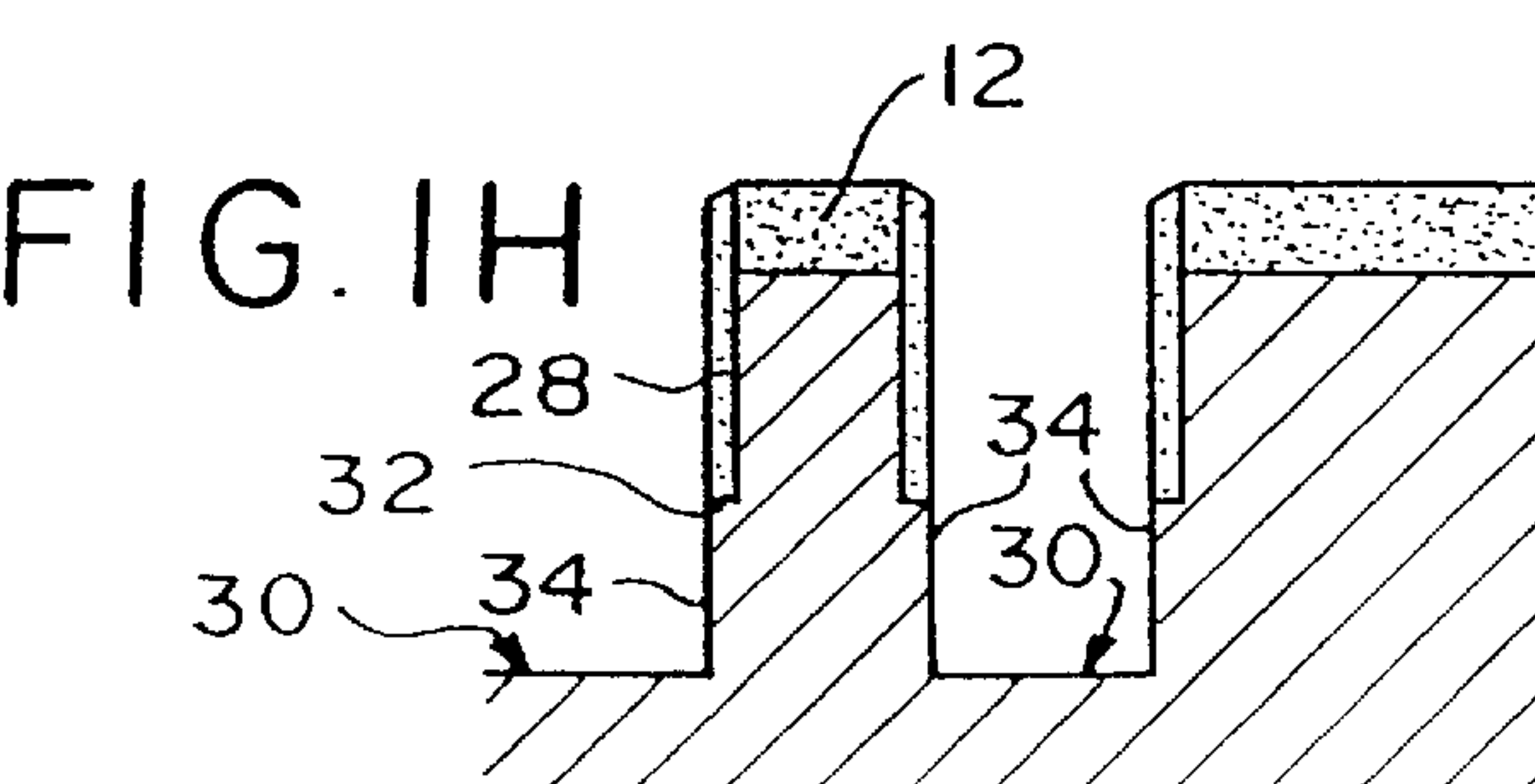
Step 8: Silicon Etch #2
