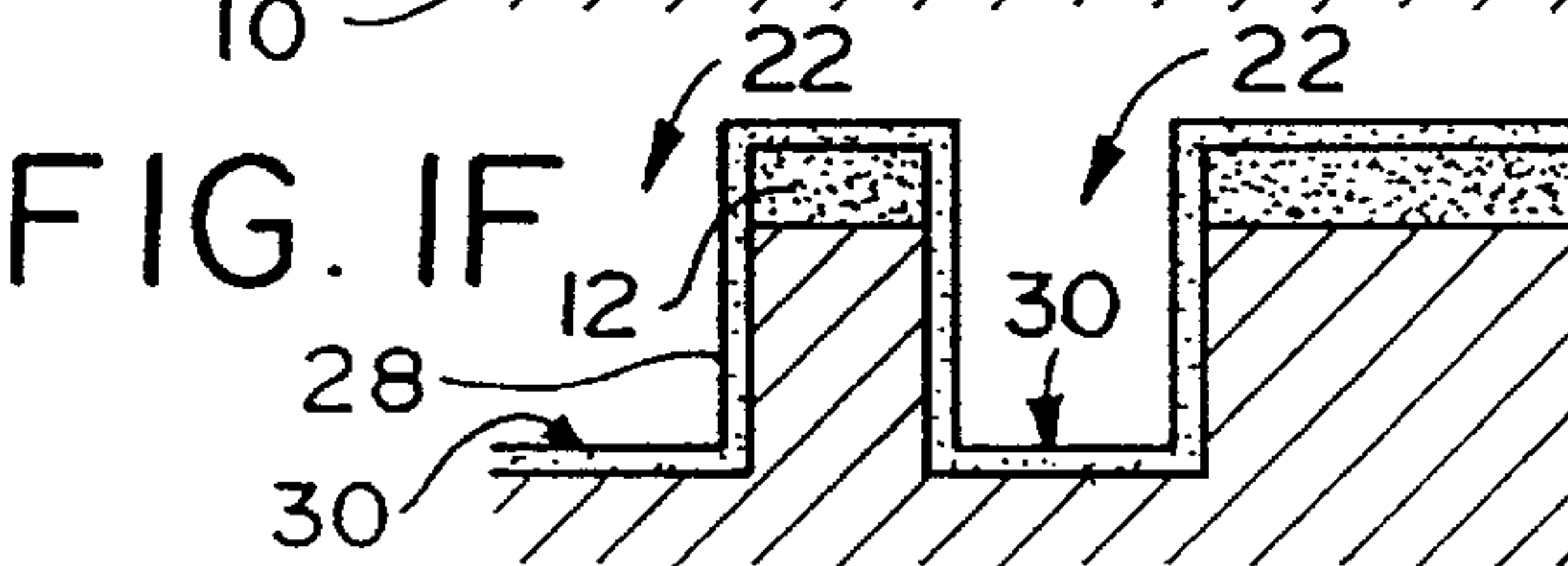
Step 6: Deposit PECVD Oxide
