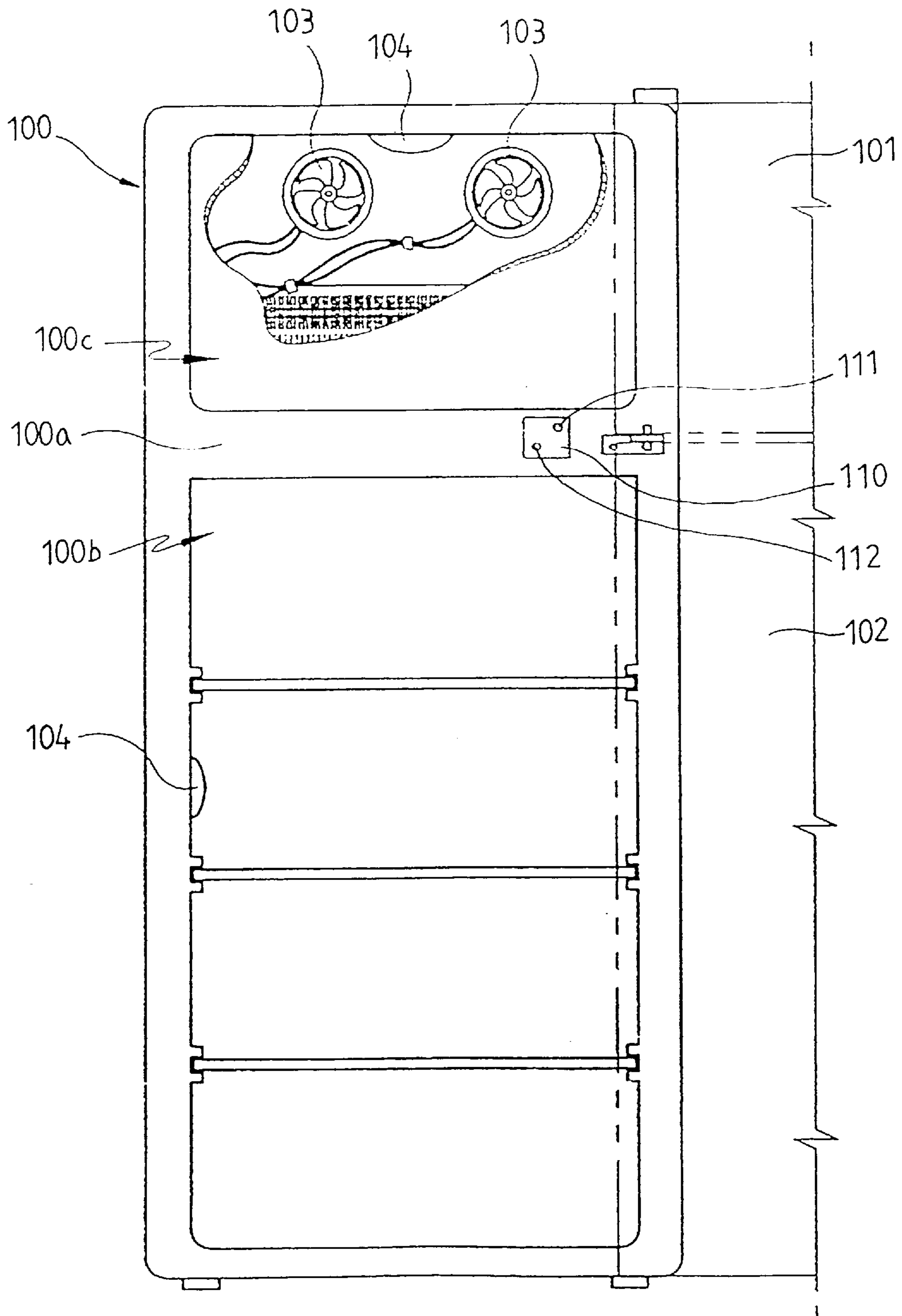
FIG. 5 (PRIOR ART)
