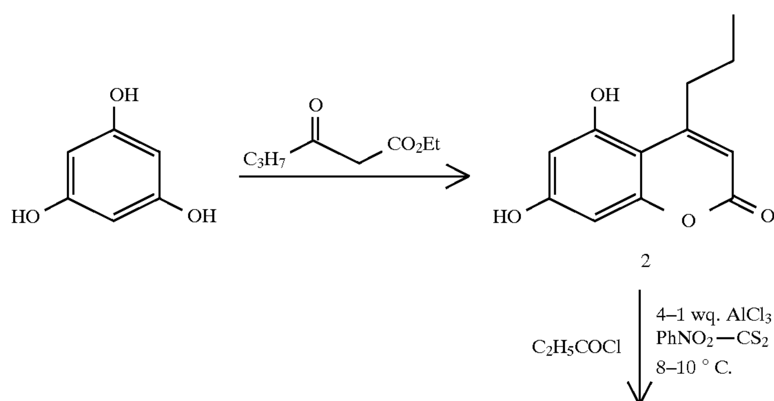
SCHEME I
