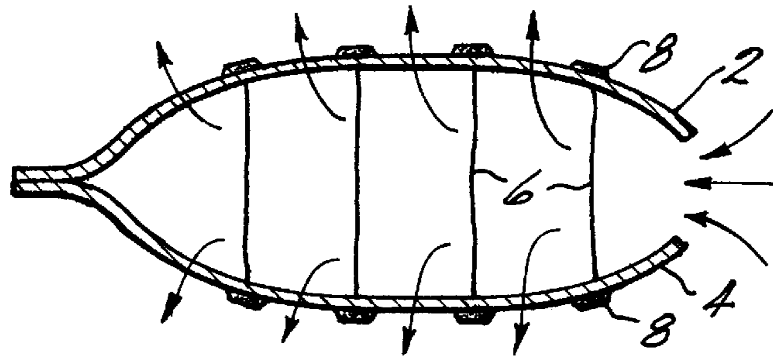
FIG. 2 (PRIOR ART)
