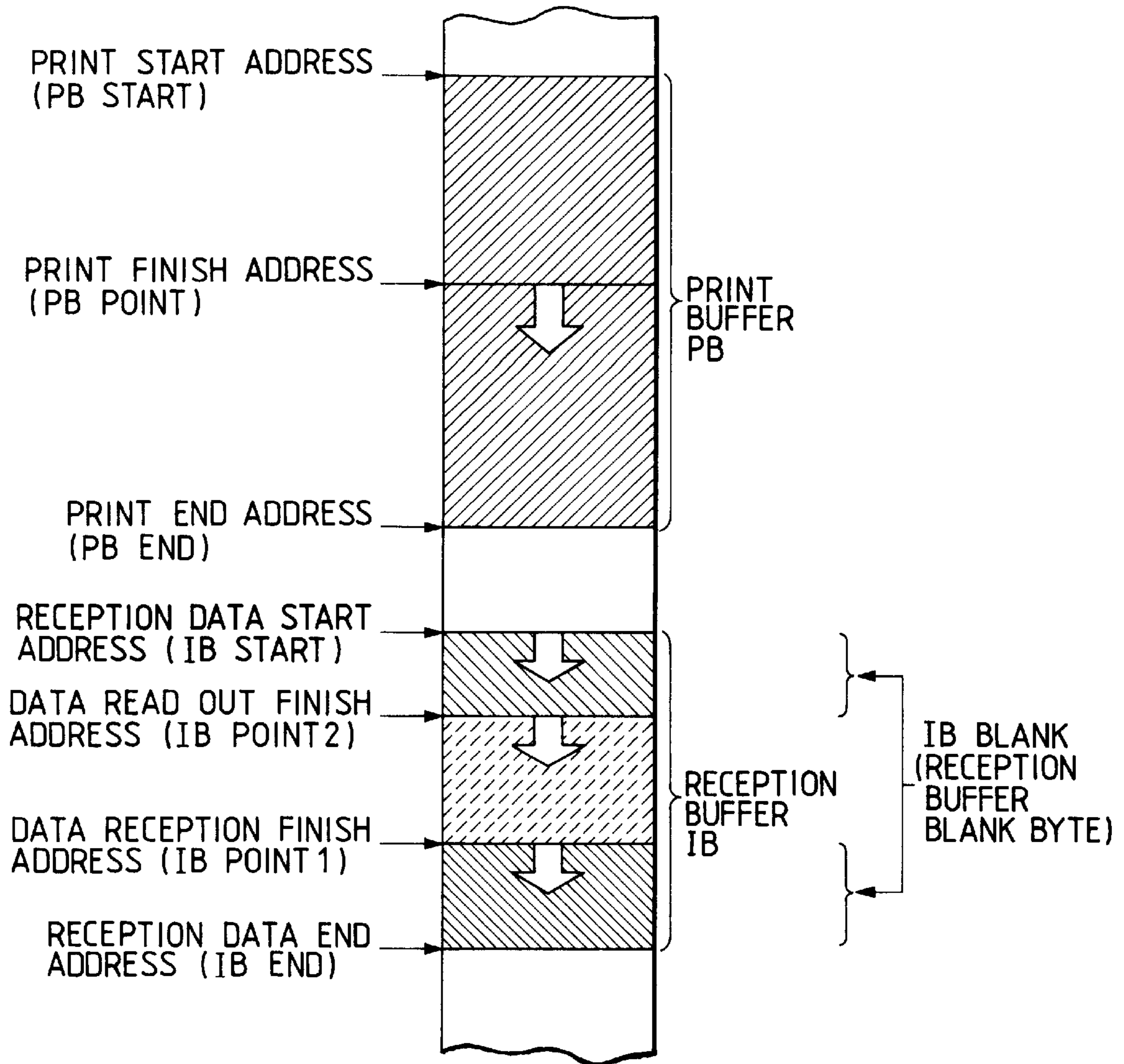
RAM-P ADDRESS MAP
