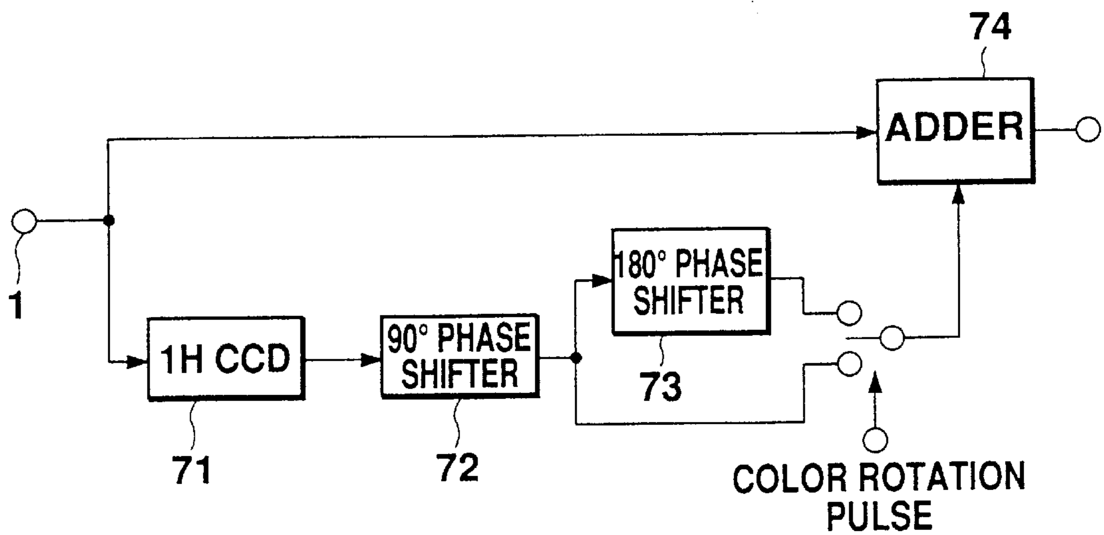
Fig. 20 PRIOR ART
