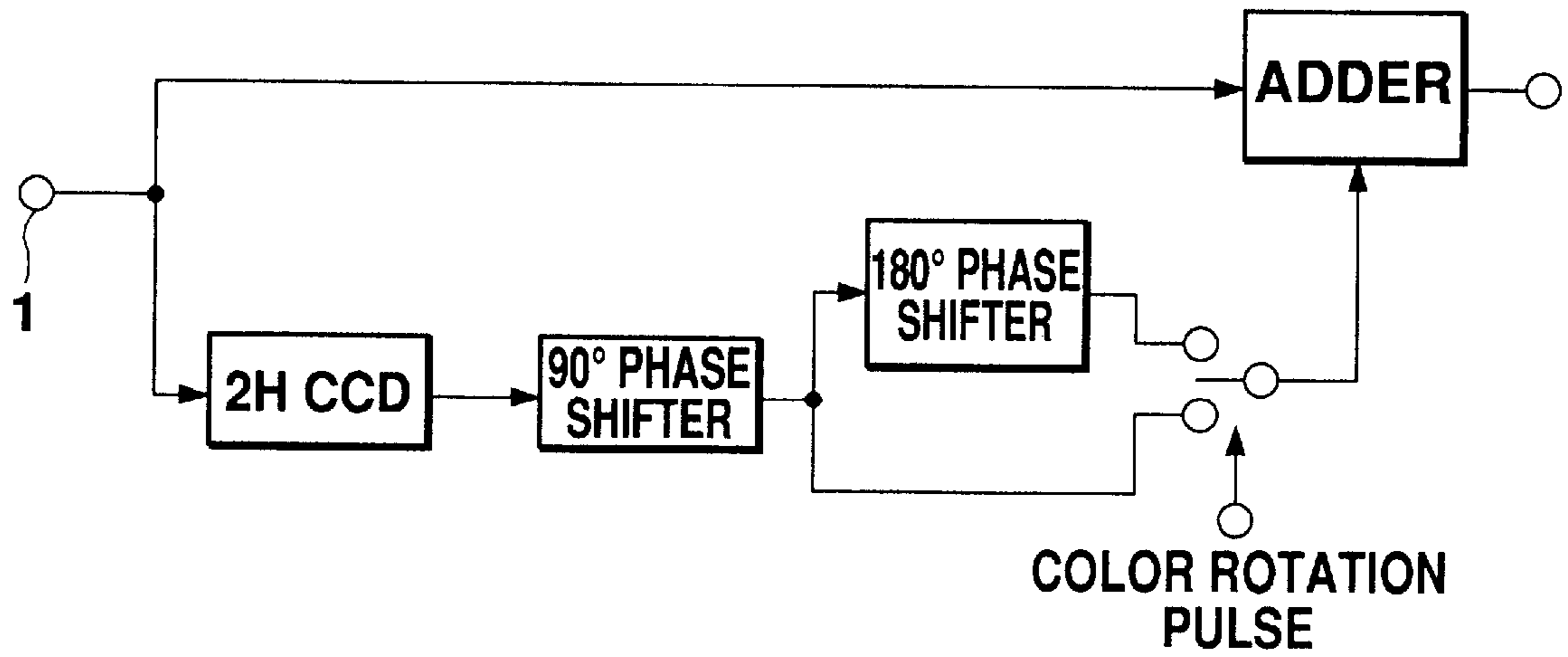
Fig. 27 PRIOR ART
