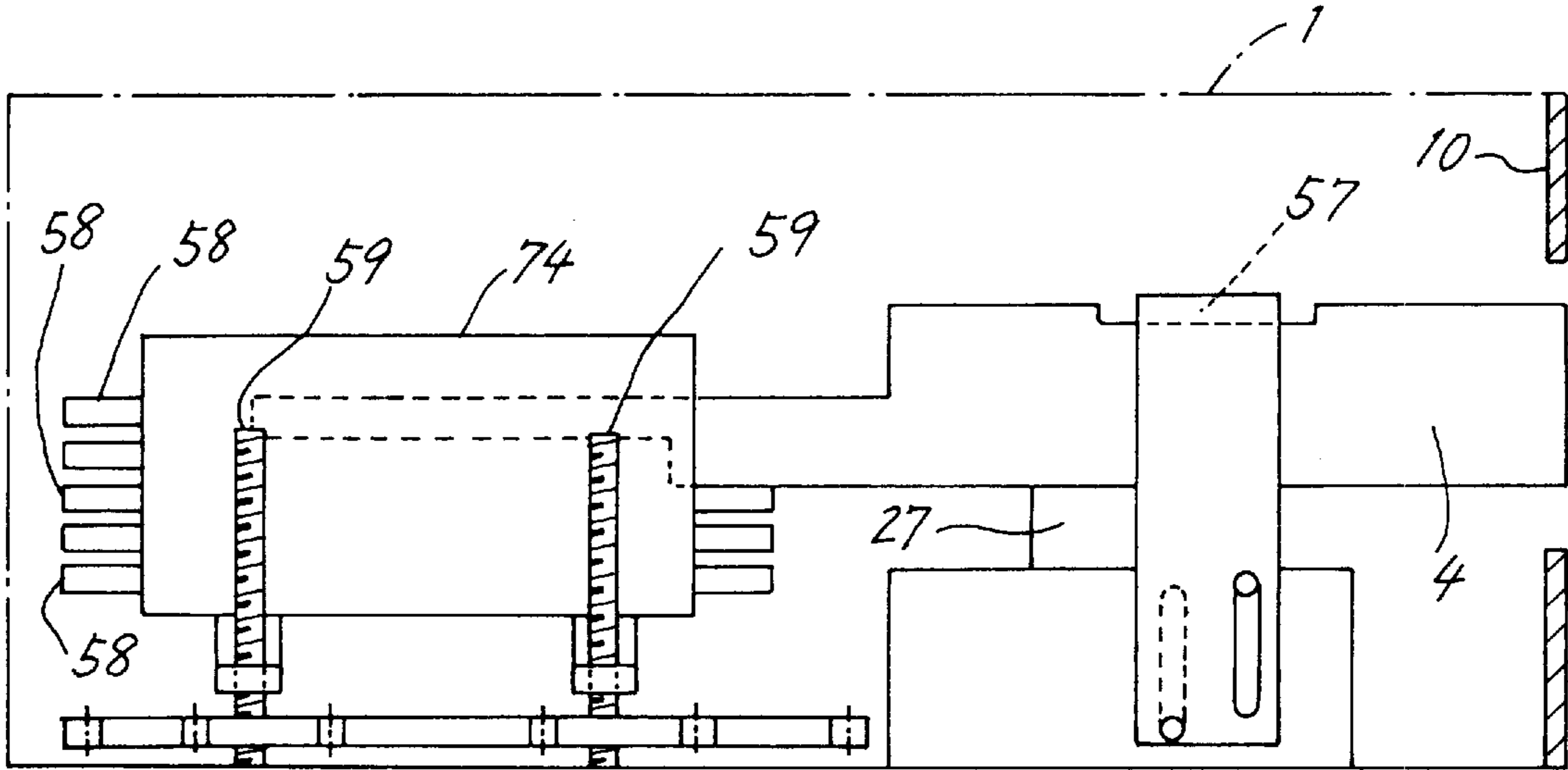
FIG. 41 PRIOR ART
