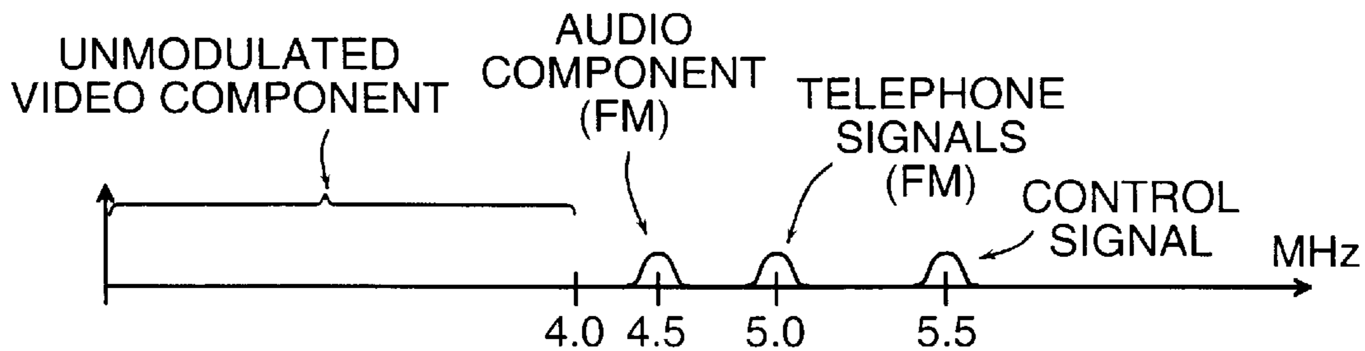
SPECTRUM OF AN NTSC SIGNAL TRANSMITTING AT BASEBAND
