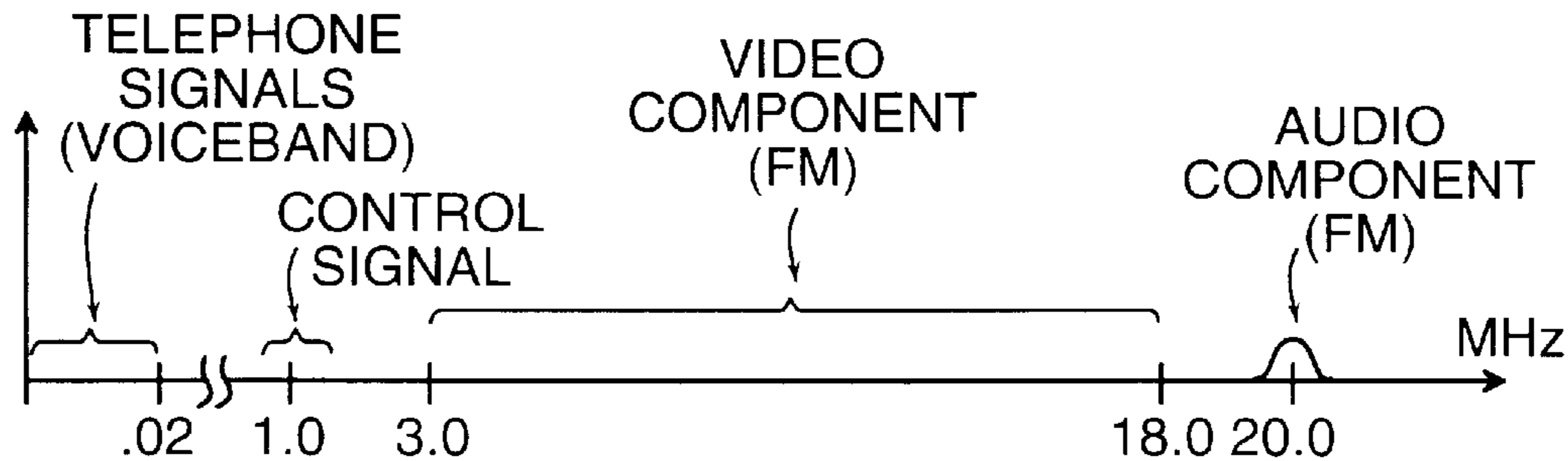
SPECTRUM OF AN FM NTSC SIGNAL NEAR VOICEBAND
