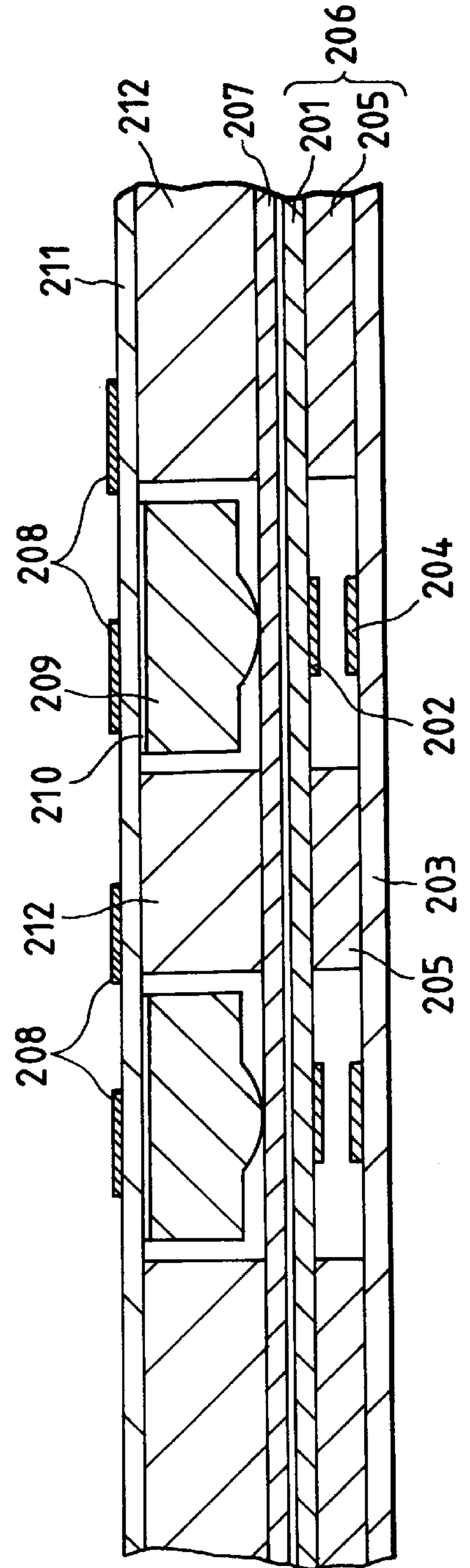
FIG. 14 PRIOR ART
