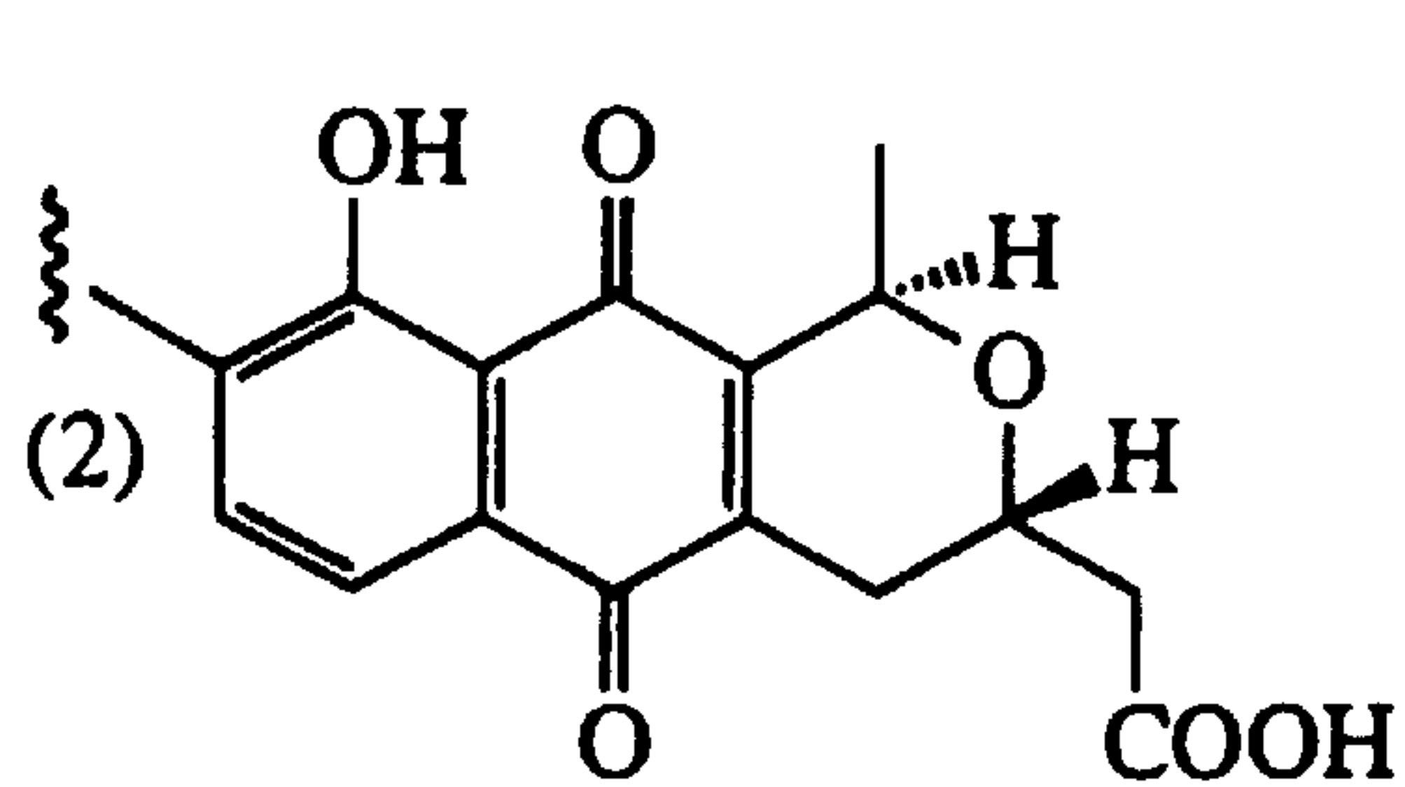
ACTINORHODIN (3)
