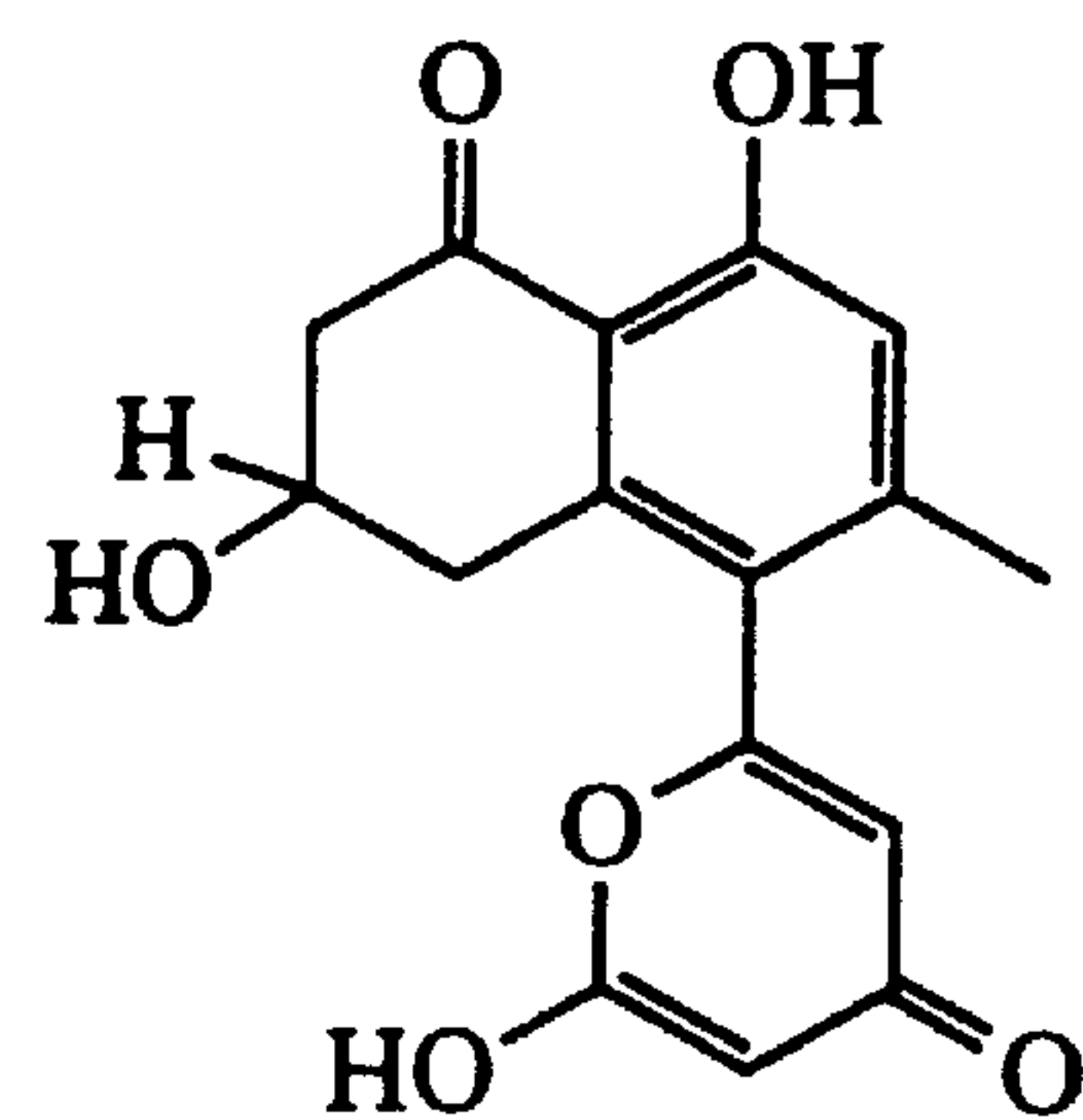
MUTACTIN (6)
