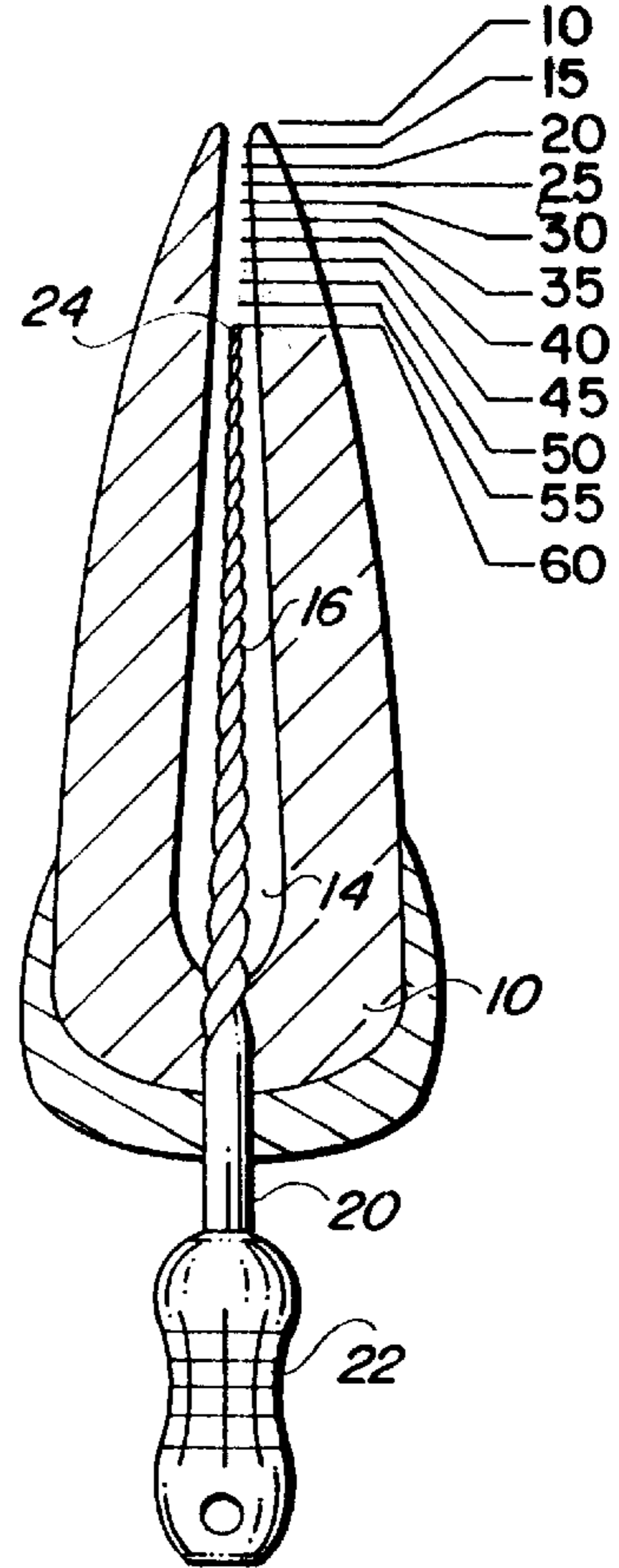
FIG. 2 (PRIOR ART)
