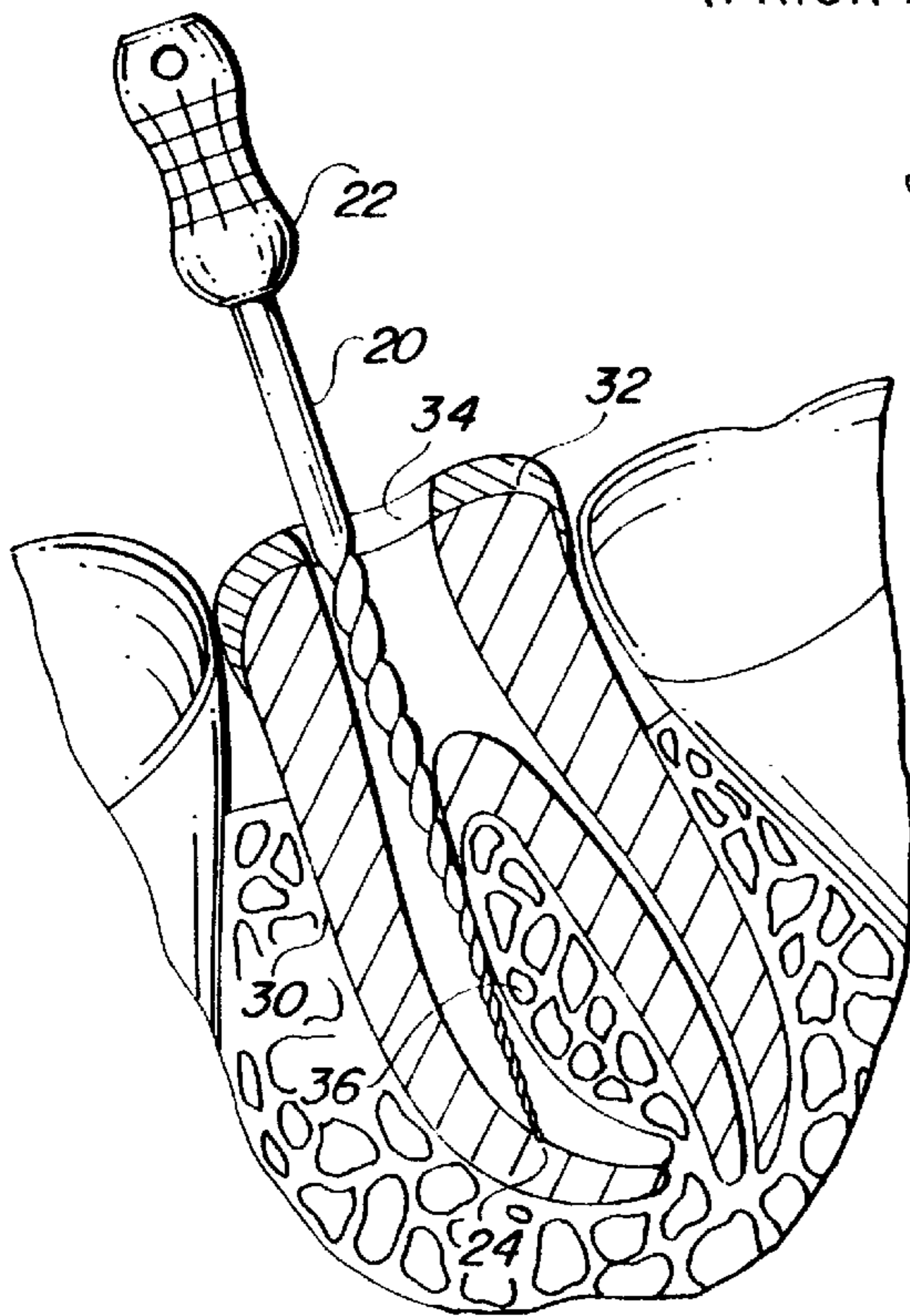
FIG. 3 (PRIOR ART)
