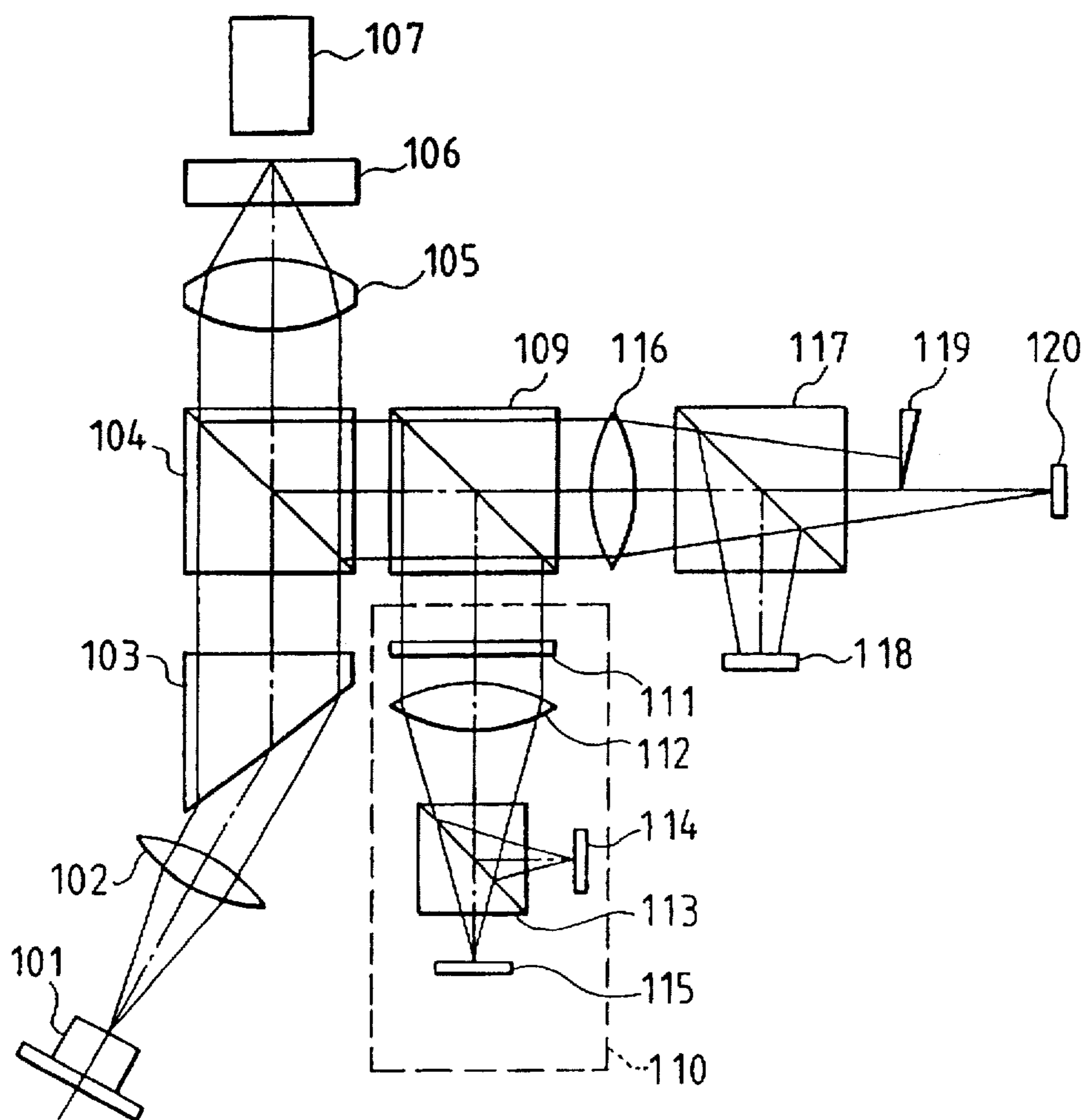
FIG. 1 PRIOR ART
