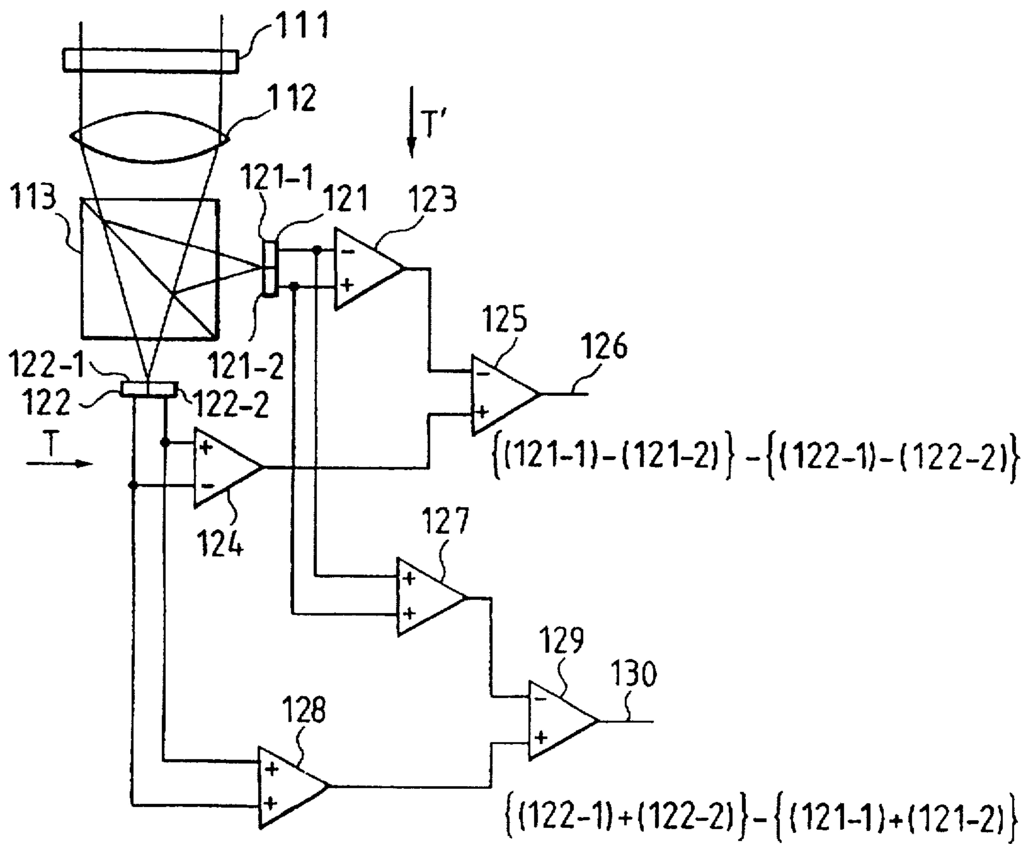
FIG. 6 PRIOR ART
