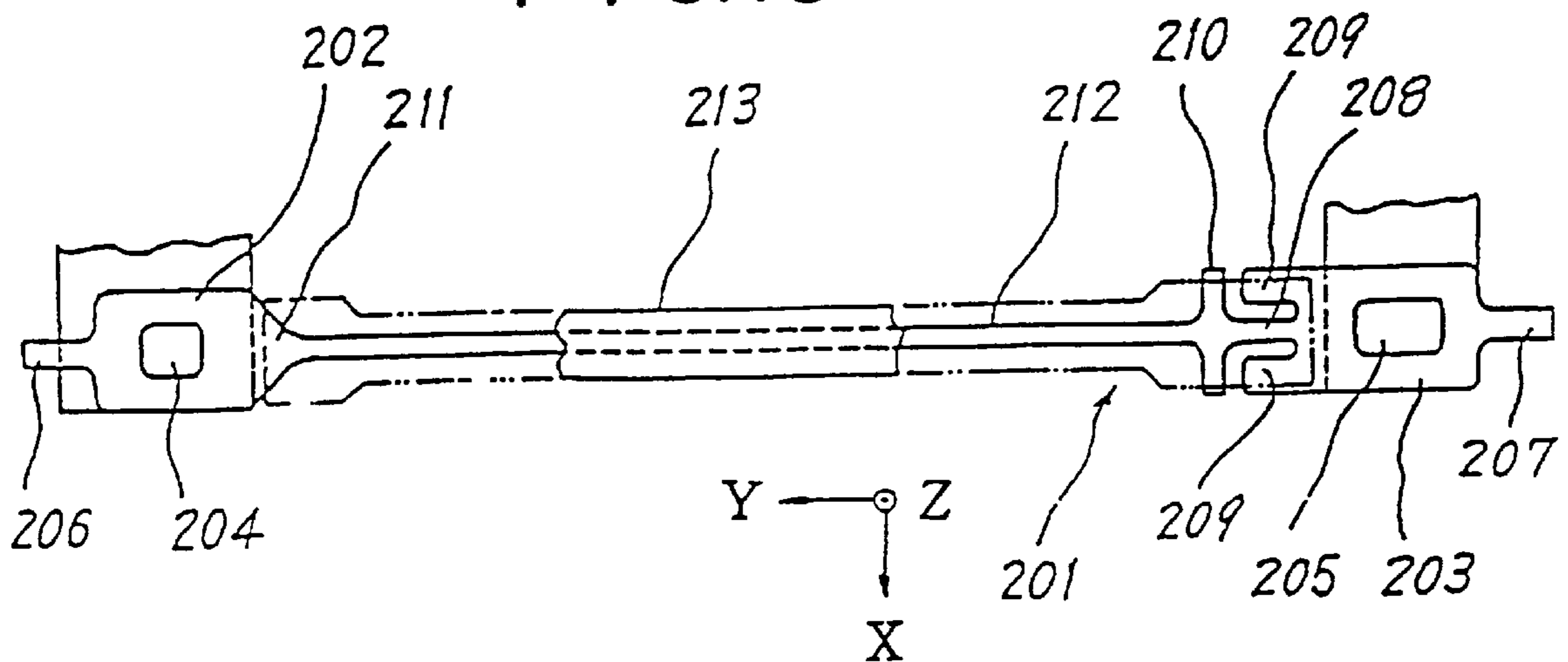
FIG. 15 PRIOR ART
