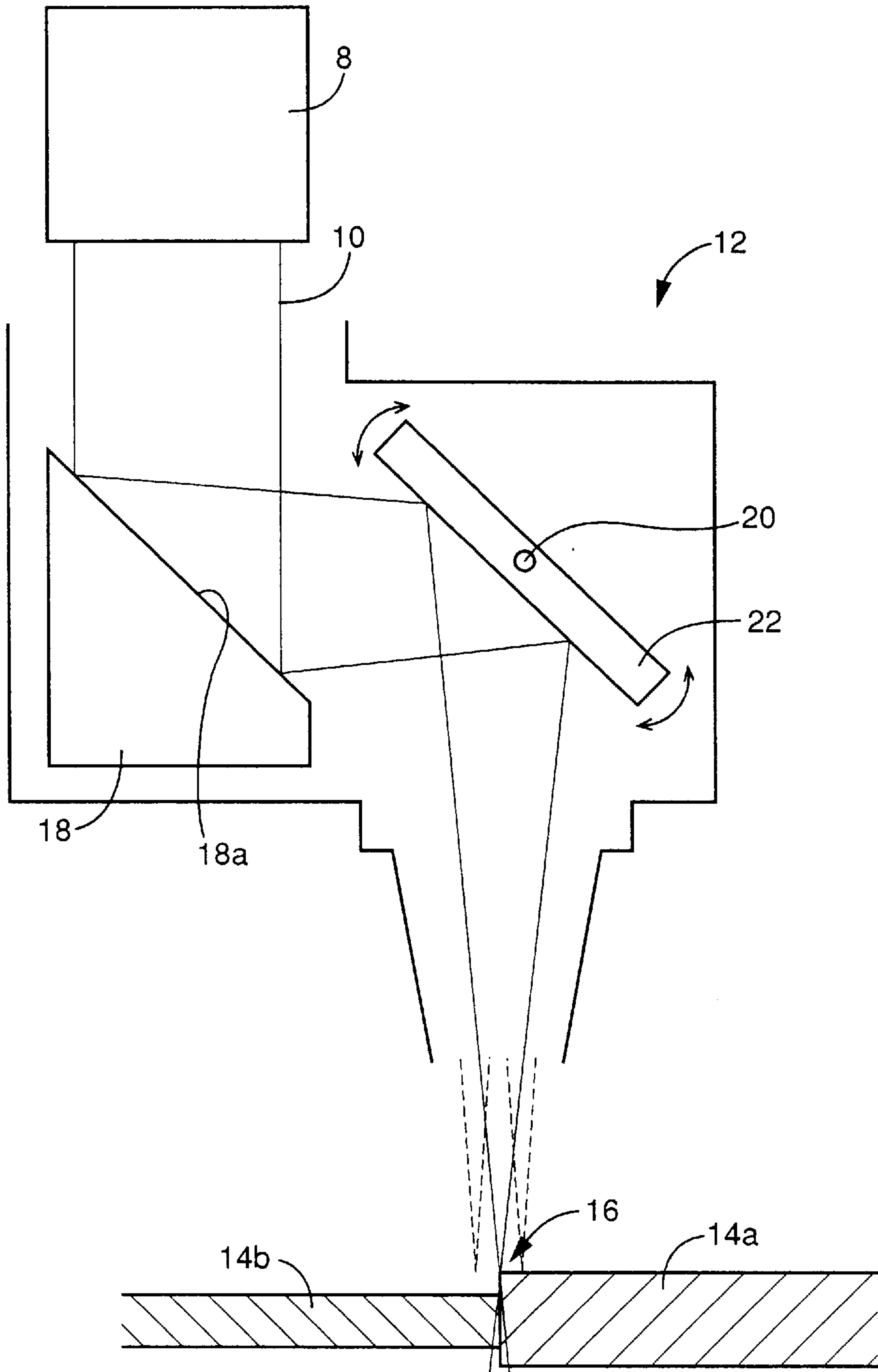
FIG. 9 PRIOR ART
