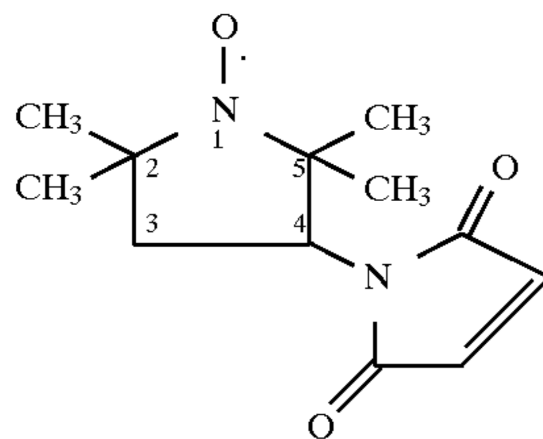
3-Maleimido-PROXYL
