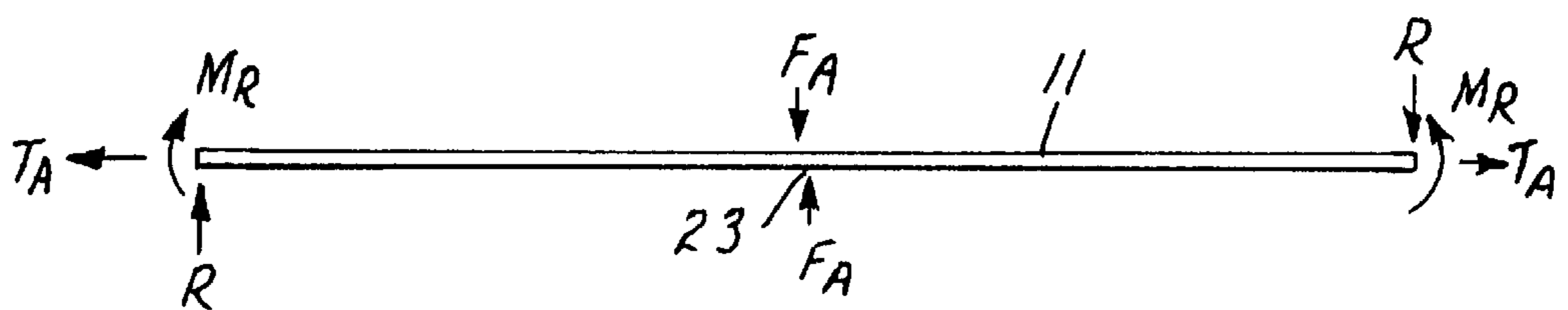
FIG. 2C PRIOR ART
